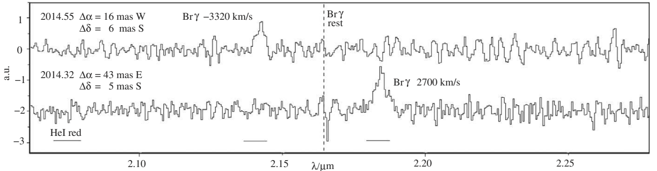
Figure 8. Summary spectra at the pre- and post-peribothron positions for the 2014 April and June epoch; see details in text.
