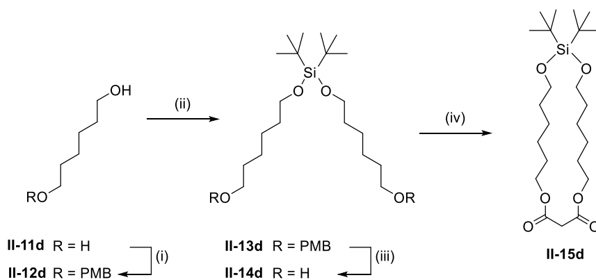
Scheme II-4. Reagents and conditions: (i) PMBCl, Ag_2O , CH_2Cl_2 , 48 h (92%); (ii) tBu_2Si(OTf)_2 , DMF, imidazole, rt, 12 h (59%); (iii) DDQ, CH_2Cl_2 , H_2O , rt, 6 h (82%); (iv) malonyl chloride, DMAP, CH_2Cl_2 , rt, 48 h ( II-15d : 38%).
