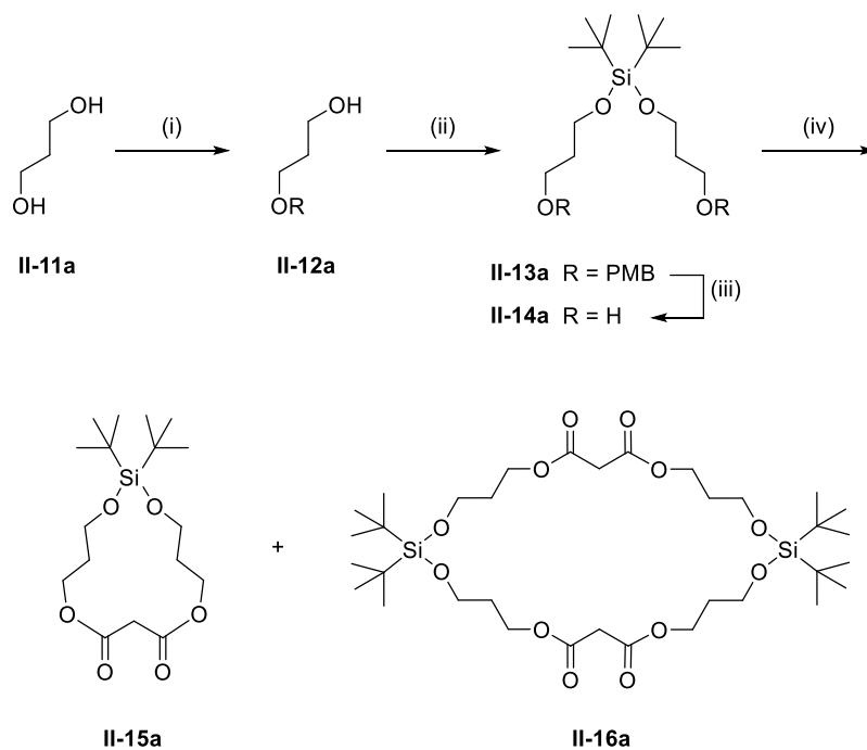
Scheme II-3. Reagents and conditions: (i) PMBCl, Ag_2O , CH_2Cl_2 , 48 h (80%); (ii) tBu_2Si(OTf)_2 , DMF, imidazole, rt, 12 h (68%); (iii) DDQ, CH_2Cl_2 , H_2O , rt, 6 h (86%); (iv) malonyl chloride, DMAP, CH_2Cl_2 , rt, 48 h ( II-15a : 24%; II-16a : 15%).
