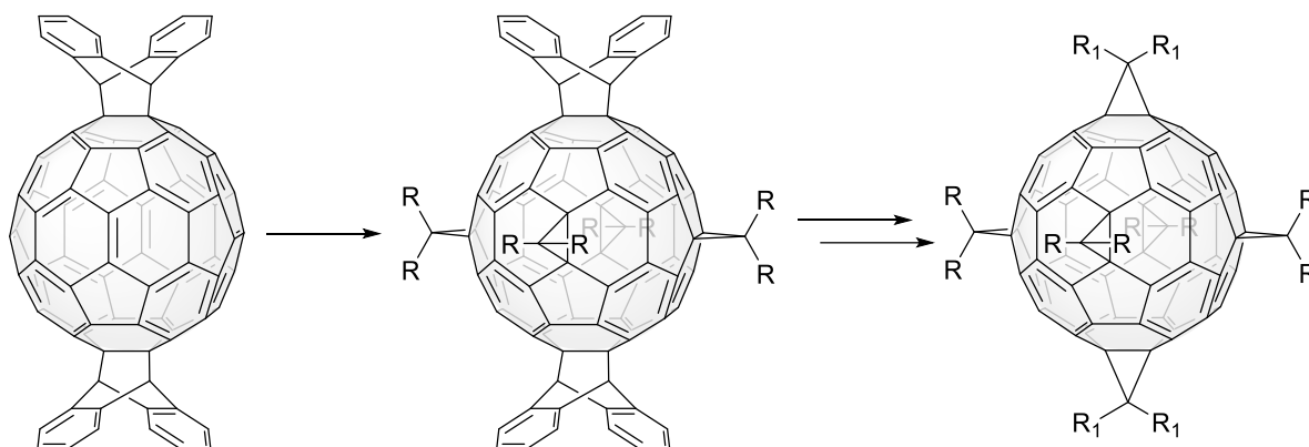
Figure IV-3 : Template strategy for the formation of type II [4:2] hexa-adducts.
