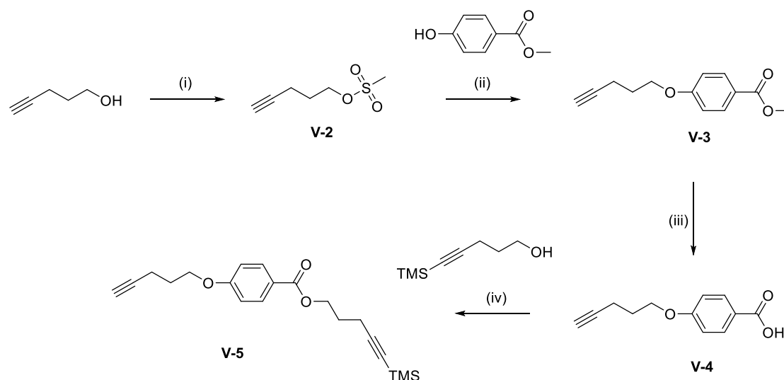
Scheme V-1. Reagents and conditions: (i) MeSO 2 Cl, trimethylamine, CH 2 Cl 2 , rt, 1 h (96%); (ii) K 2 CO 3 , crown 18C6 (cat.), acetone, reflux, 1.5 d (83%); (iii) KOH, THF/EtOH, reflux, 2.5 h (96%); (iv) DCC, DMAP, CH 2 Cl 2 , 0 °C to rt, 12 h (65%).
