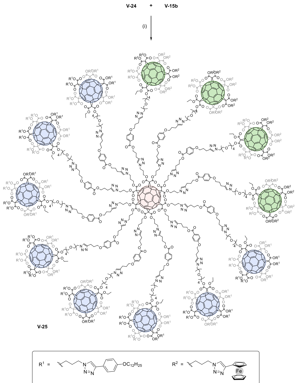
Scheme V-9. Reagents and conditions: (i) CuSO 4 ·5H 2 O, sodium ascorbate, CH 2 Cl 2 /H 2 O, 37 °C, 7 d (72%).
