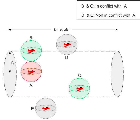
Figure 5.14 – Conflict cylinder
