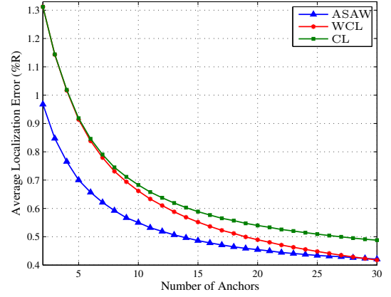
(b) Mobile anchors ( v = 1m/s )
