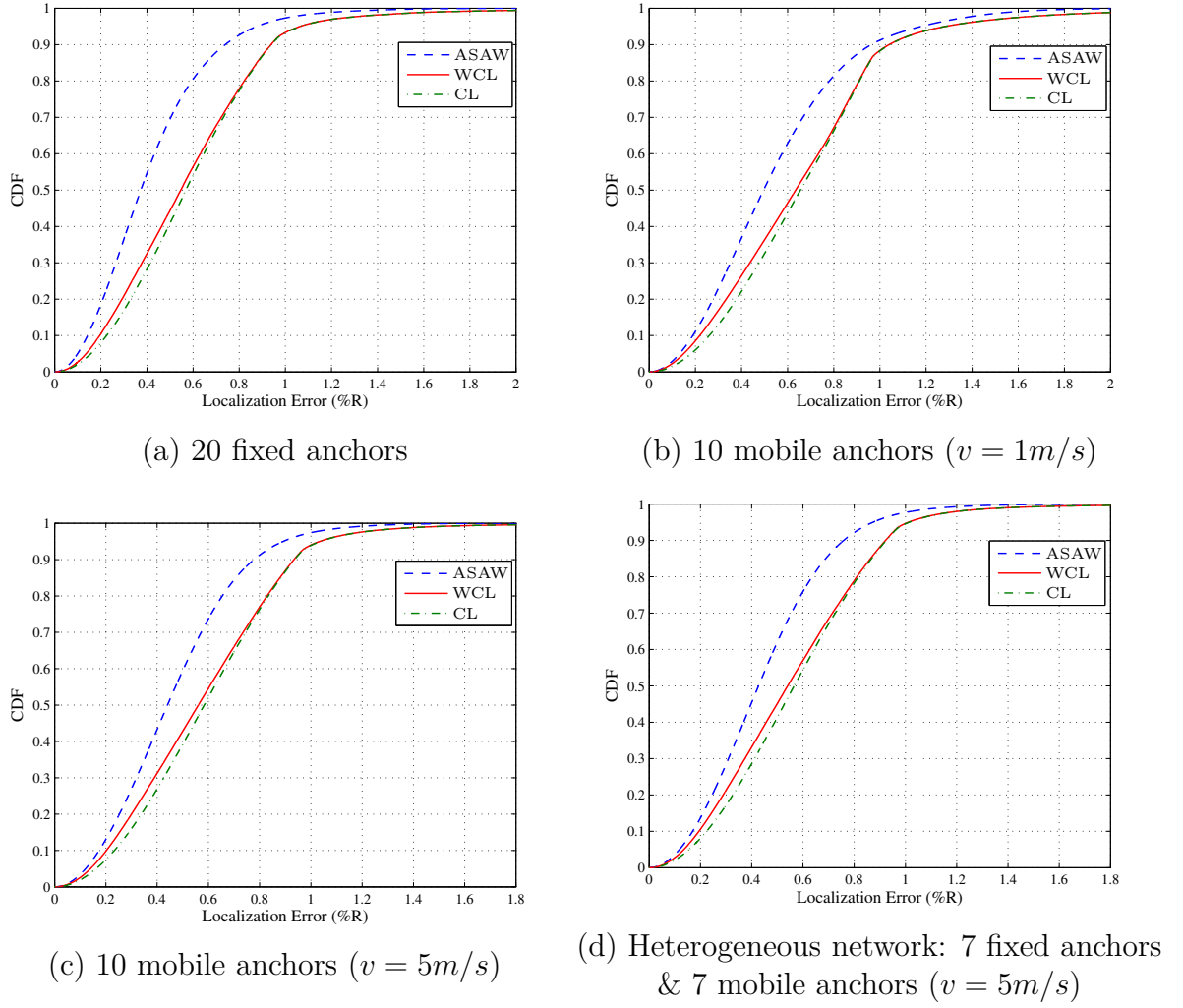
Figure 3.3 – CDF of localization errors
