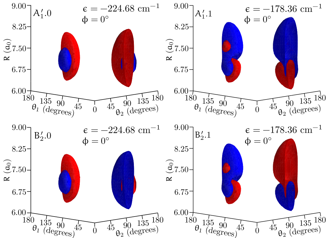
Figure 8.3: Left panel: 3D plot of the ground state quasi-degenerate wave functions. Right panel: 3D plot of the quasi-degenerate vibrational wave function of \text{MIN1} (0,0,1,0) level. The A'_1 wave function is the symmetrical combination of the two wave functions localized in the equivalent \text{MIN1} structures. The B'_2 wave function is the corresponding antisymmetrical combination.
