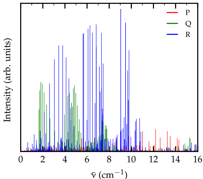
Figure 4.4: Rovibrational spectrum of He–C 3 N − at the temperature of 10 K
