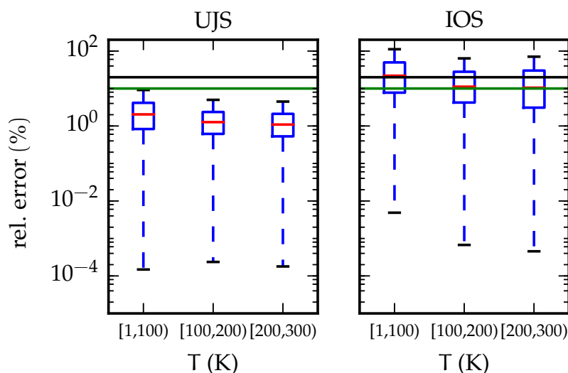
Figure 5.7: IOS and UJS relative error for selected temperature ranges. See the caption of Fig. 5.6 for the details of data representation.
