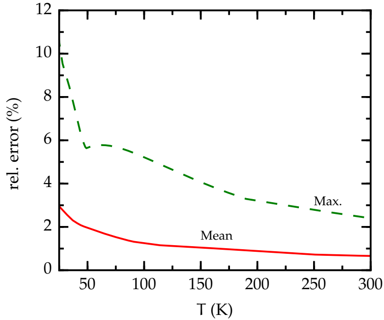
Figure 7.2: Error on the calculation of para -H 2 rate coefficients by using the UJS procedure as a function of temperature.
