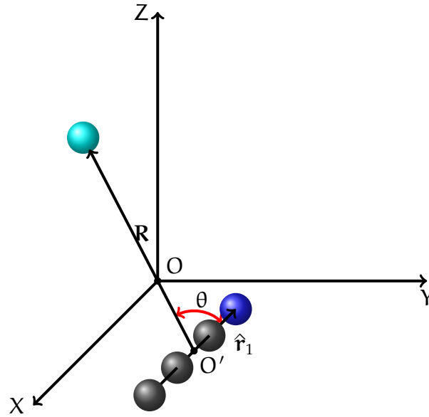
Figure 5.1: Space-fixed axes and Jacobi coordinates used to describe the interaction between He and C_3N^- . O' is the center of mass of C_3N^- and O is the center of mass of the whole system
