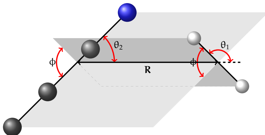
Figure 6.1: Body-fixed Jacobi coordinates used to describe the interaction between H_2 and C_3N^- .
