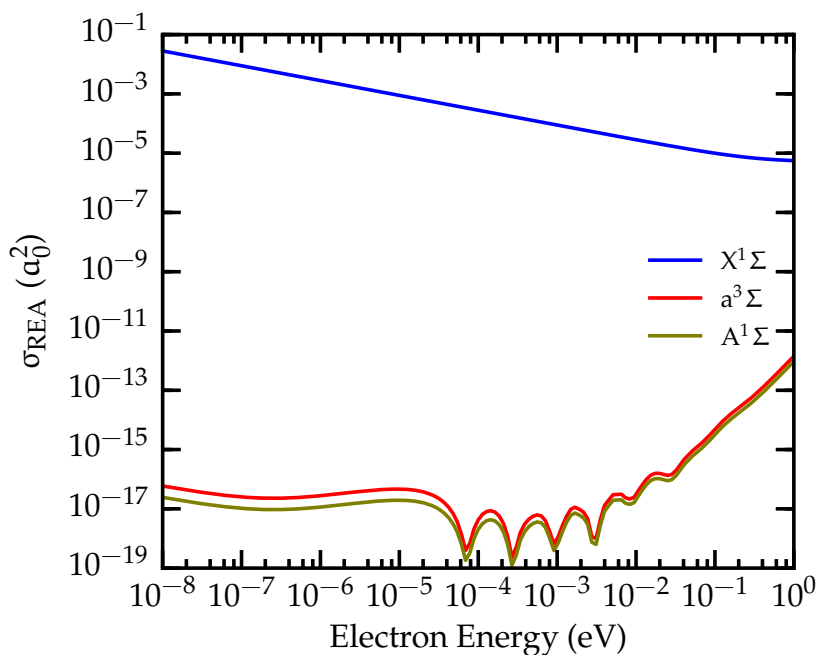
Figure 3.3: REA cross section of C_3N . The curves are labeled by the electronic state of the C_3N^- anion.
