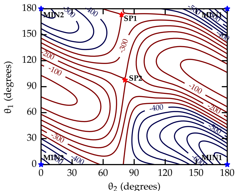
Figure 6.2: 2D contour plot of the H_2 - C_3N^- PES for \phi = 0^\circ and R relaxed. Contour lines are equally spaced by 50 \text{ cm}^{-1}
