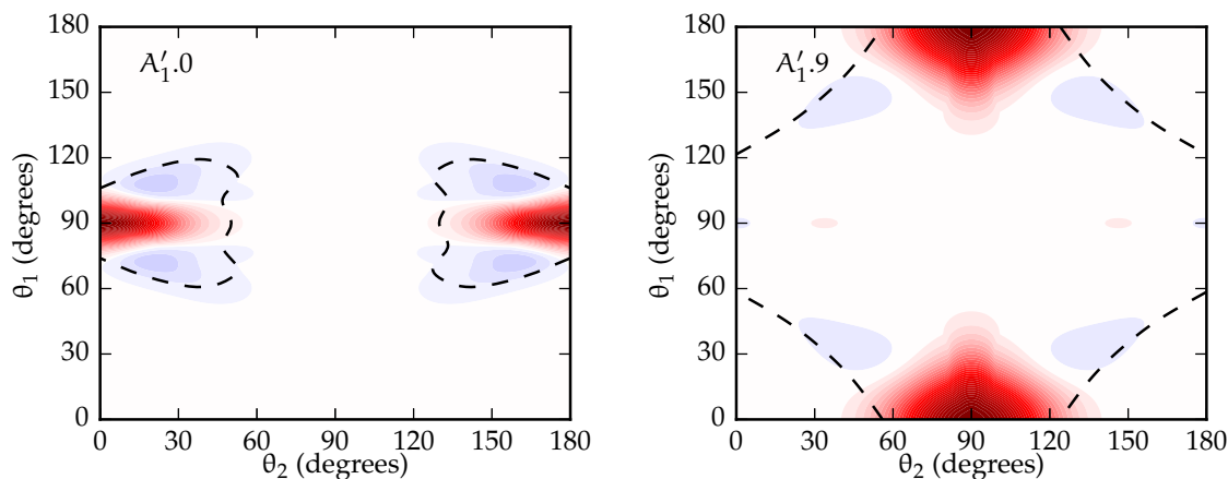
Figure 8.5: Left panel: 2D contour plot for the ground state wave function of MIN1. The black dashed line is the potential isoline equal to the energy of the ground state. Right panel: 2D contour plot for the ground state wave function of MIN2. For each point (\theta_1, \theta_2) , both the wave function and the potential energy have been calculated with the values of \phi and R which minimize the potential energy. The black dashed line is the potential isoline equal to the energy of the bound state.
