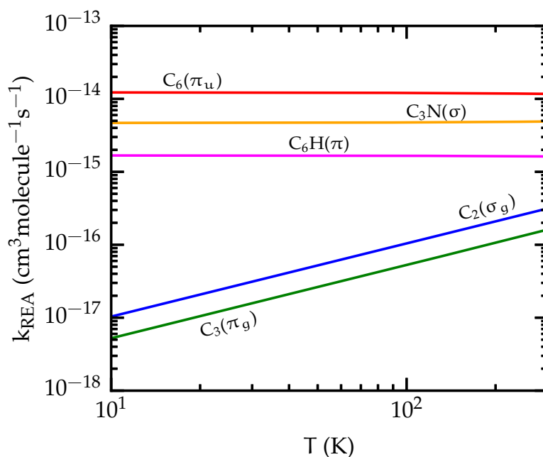
Figure 3.2: REA rate coefficient as a function of the temperature for selected linear chains. The curves are labeled by molecule and symmetry type of the Dyson orbital.
