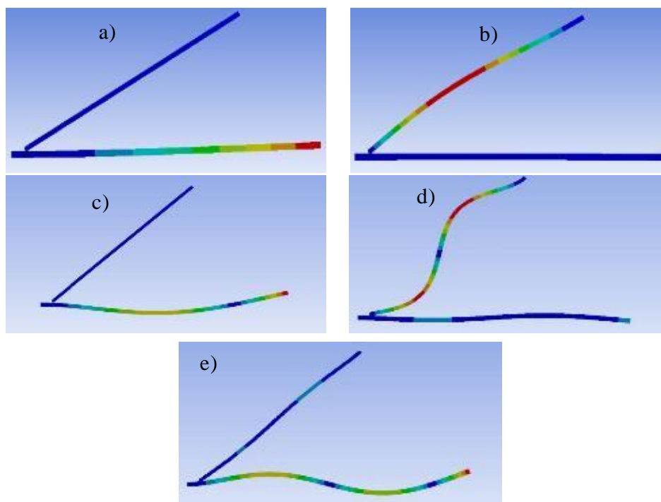
Fig. IV-1: deformation shapes for 1 st (a), 2 nd (b), 3 th (c), 4 th (d), and 5 th (e) natural frequency, with s=5 mm
