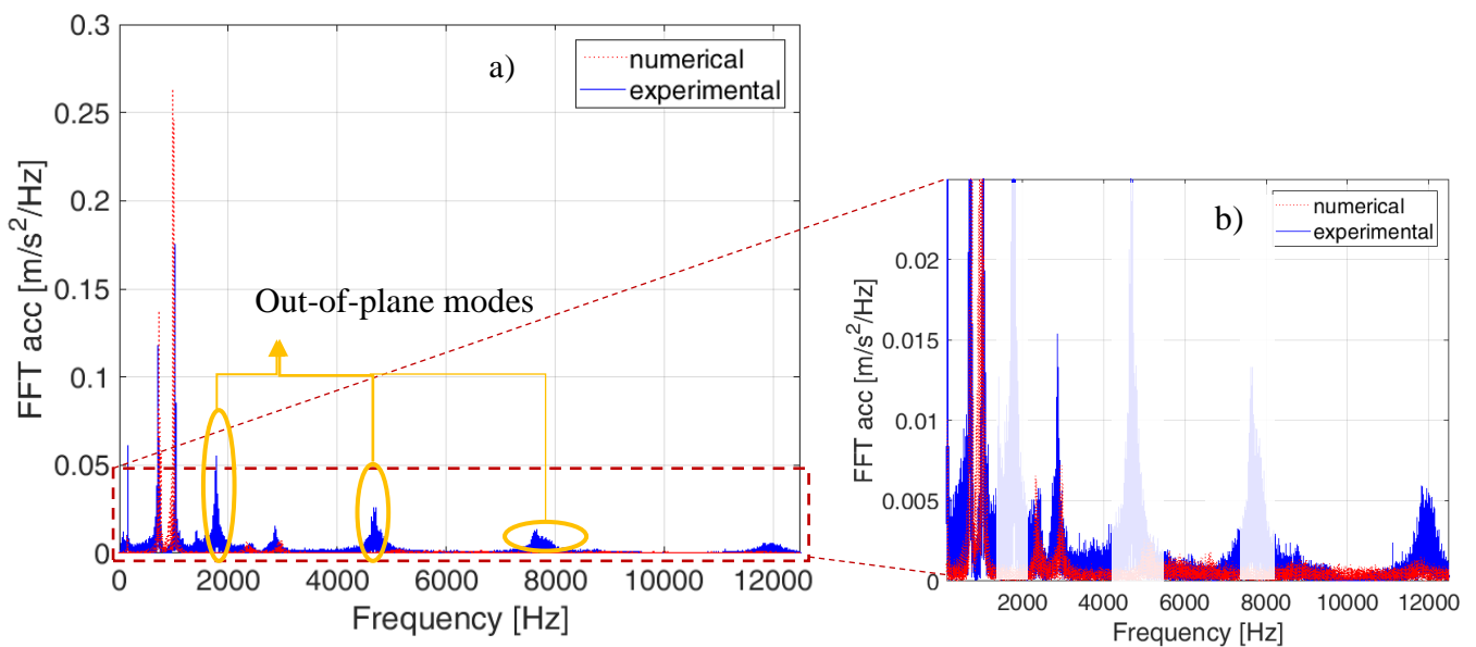
Fig. V-12 a) superposition of the experimental (blue) and the numerical (red) spectral distribution (FFT) of the acceleration; b) magnification of the spectral evolution with focus on the higher frequency band. The signal chosen for the perturbative term is the one retrieved from the inverse method, choosing the surface roughness R320.
