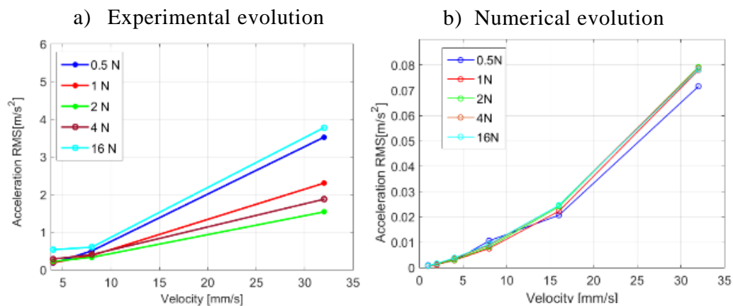
Fig. IV-6: a) experimental evolution of the acceleration RMS with respect to the sliding velocity, for a surface roughness R120; b) numerical evolution of the acceleration RMS with respect to the sliding velocity. Classical friction law with 0.45 as friction coefficient.
