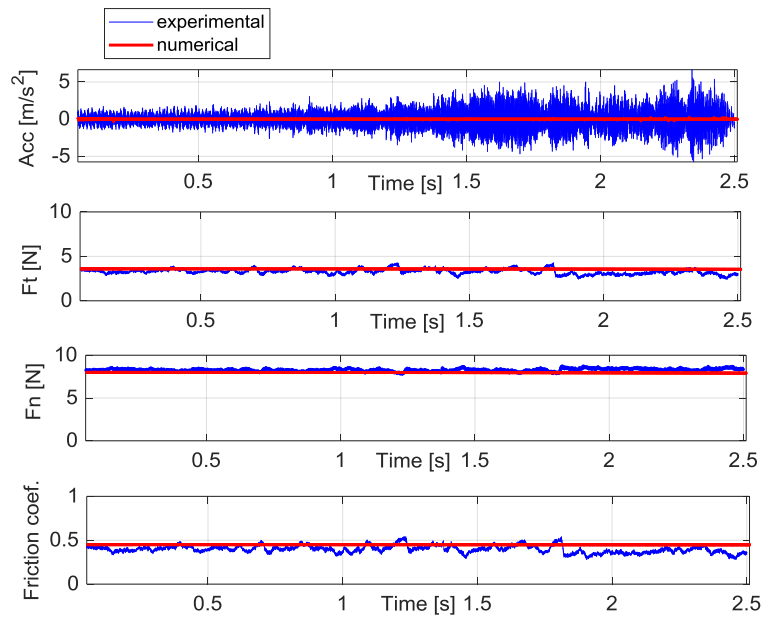
Fig. IV-8: Superposition of the numerical (red curve) and the experimental (blue curve) evolution of the acceleration, tangential (Ft) and normal force (Fn), and friction coefficient, during the 20mm of relative sliding.
