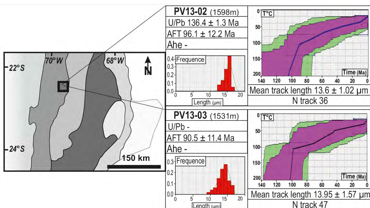
Figure 4.14 – Low-temperature thermochronological modelling of the samples from the coastal range with HeFty, U/Pb, AFT and AHe ages and fission track lengths data (number and mean track length).
