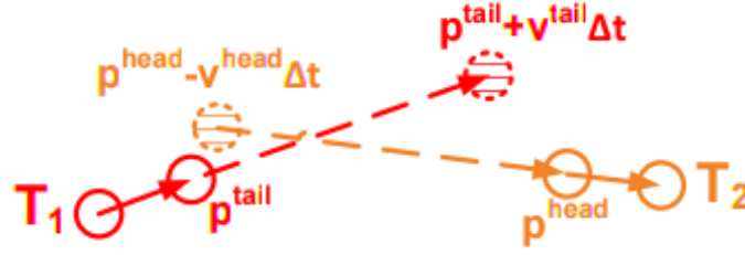
Figure 2.3: Illustration of linear motion model presented in [113] where \mathbf{T} standing for Target, \mathbf{p} standing for Position, \mathbf{v} standing for Velocity of the target.
