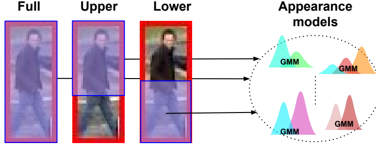
Figure 6.2: Tracklet representation.
