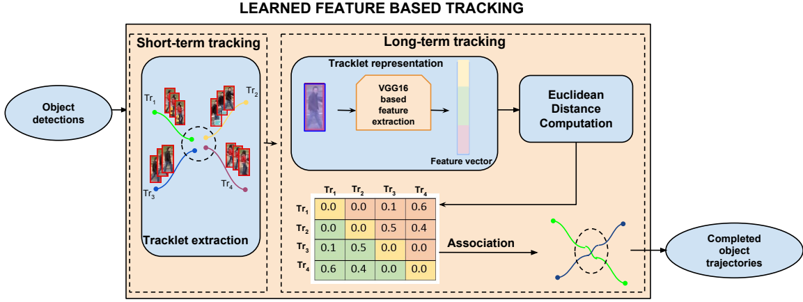
Figure 6.5: The proposed learned feature based MOT framework.
