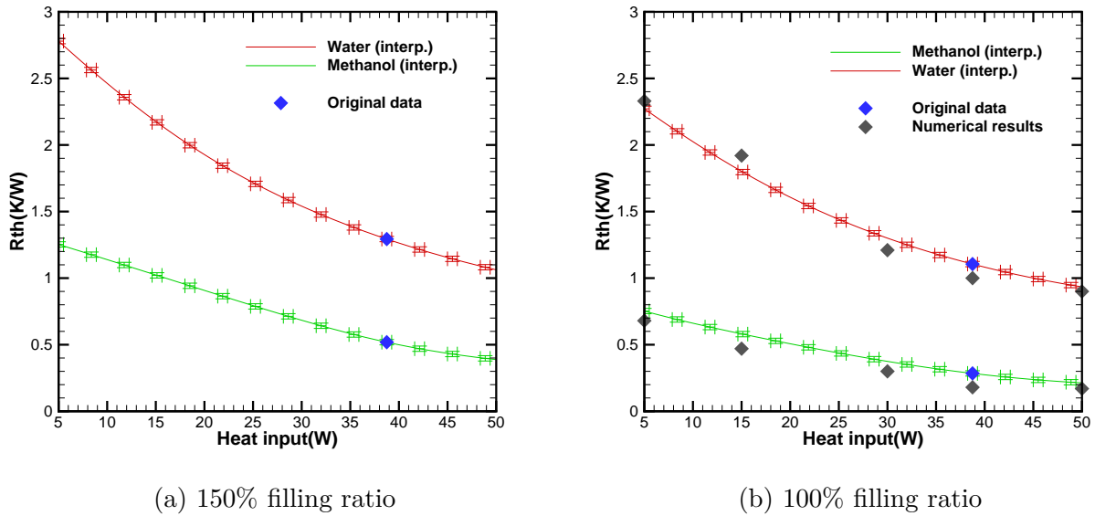
FIGURE 5.23 – Variations of the thermal resistance versus the heat input for different working fluids under condenser temperature, 37°C, and inclination angle, 63°.
