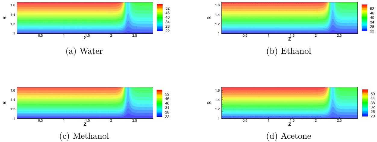
FIGURE B.1 – Temperature field in the porous medium expressed in °C for different working fluids using sintered steel (case I).
