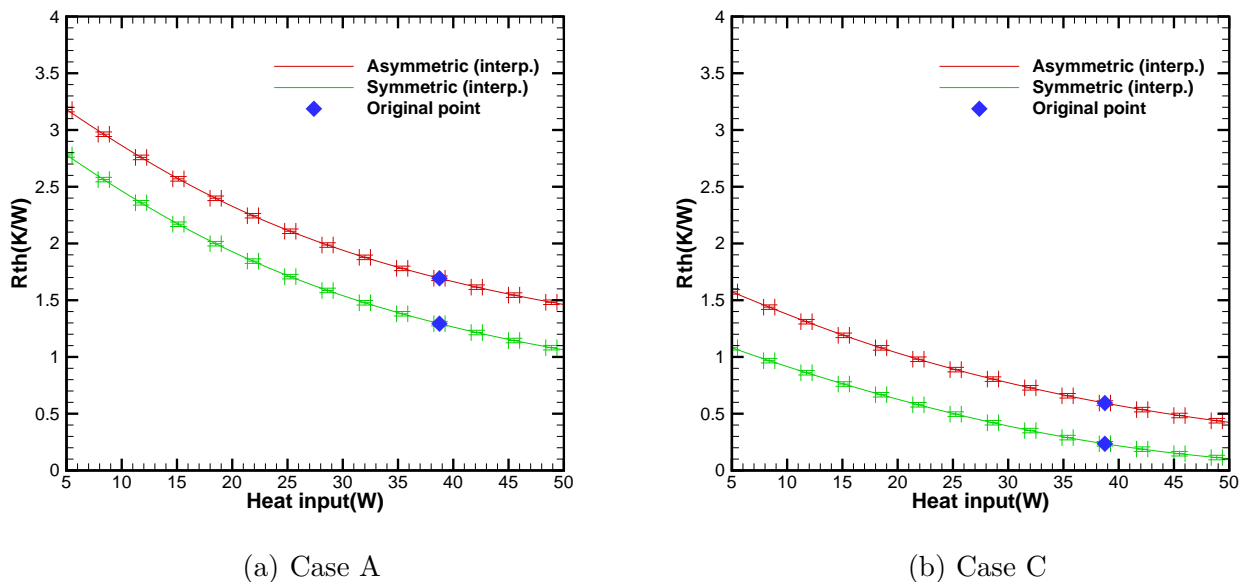
FIGURE 5.40 – Variations of the thermal resistance versus the heat input for water with 150% filling ratios using symmetric and asymmetric configurations under condenser temperature, 37^{\circ}\text{C} , and inclination angle, 63^{\circ} .
