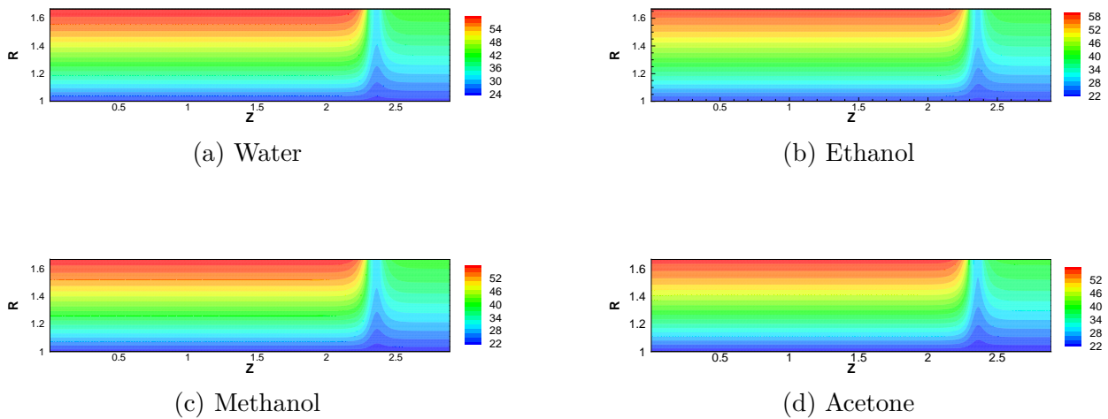
FIGURE B.2 – Temperature field in the porous medium expressed in °C for different working fluids using copper screen (case II).
