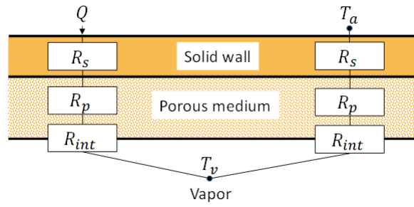
FIGURE 5.18 – Resistance circuit equivalent to the heat pipe.
