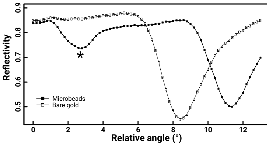
Figure 3.21 – Plasmon curves of surfaces with and without microbeads in culture media (RPMI 1640). The SPR angle on gold (surface without microbeads) was set as 0^\circ . In case of the WGM phenomena, the valley associated to this optical effect are marked with an asterisk (*).
