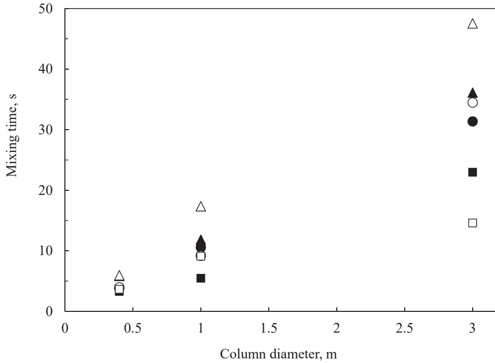
Figure 4.18: Mixing time as a function of the column diameter. Comparison between two different turbulence models: RNG k-\varepsilon ( \blacktriangle 0.09 m/s, \bullet 0.16 m/s and \blacksquare 0.25 m/s) and k-\omega ( \triangle 0.09 m/s, \circ 0.16 m/s and \square 0.25 m/s).
