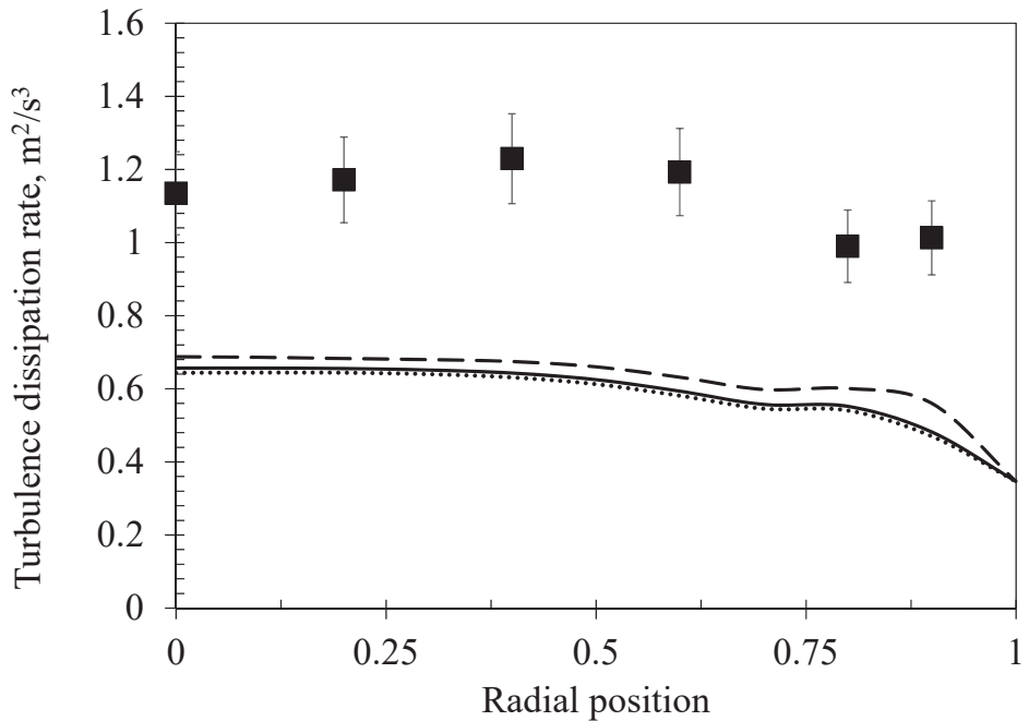
Figure C.5: Radial profile of the turbulence dissipation rate for a superficial gas velocity of 0.16 m/s at H/D=2.5. Experimental data (■) versus CFD results obtained by considering the Reynolds average (solid line) and the Favre-like average seen by the bubbles (dashed line) and the liquid (dotted line).
