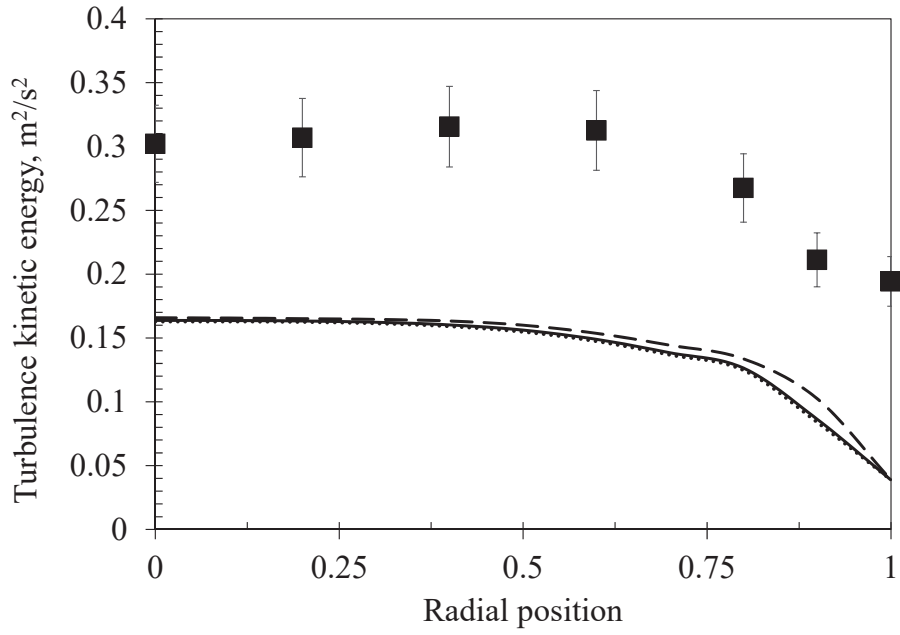
Figure C.4: Radial profile of the turbulence kinetic energy for a superficial gas velocity of 0.16 m/s at H/D=2.5. Experimental data (■) versus CFD results obtained by considering the Reynolds average (solid line) and the Favre-like average seen by the bubbles (dashed line) and the liquid (dotted line).
