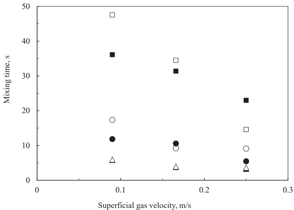
Figure 4.19: Mixing time as a function of the superficial gas velocity. Comparison between two different turbulence models: RNG k-\varepsilon ( \blacktriangle \phi 0.4 m, \bullet \phi 1 m and \blacksquare \phi 3 m) and k-\omega ( \triangle \phi 0.4 m, \circ \phi 1 m and \square \phi 3 m).
