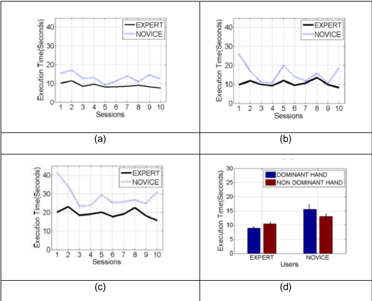
Figure 117 – ANOVA results on time (a) left hand (b) right hand (c) both hands and (d) time differences between users (© 2017 IEEE).
