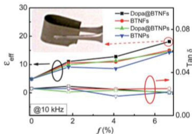
Fig. 2-10 Variation of dielectric constant and loss with the volume fraction of BaTiO 3 nanofillers for epoxy nanocomposites [83].
