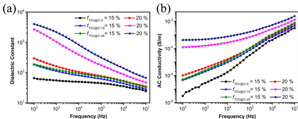
Fig. 6-7 Frequency dependence of the (a) dielectric constant and (b) AC conductivity values of the TiO 2 @C-5 NWs/PVDF, TiO 2 @C-15 NWs/PVDF, and TiO 2 @C-45 NWs/PVDF nanocomposites at different filler loadings (15 vol. % and 20 vol. %).
