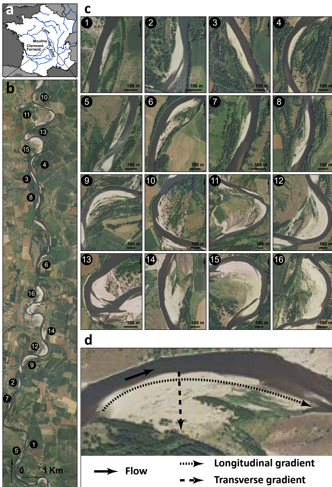
Figure 37. The study reach of the Allier River and the 16 alluvial bars ranked from 1 to 16 according to increasing lateral erosion rate (1.45, 1.61, 1.74, 1.78, 1.93, 2.01, 3.13, 4.37, 5.26, 5.57, 7.59, 7.61, 8.65, 10.10, 16.49 \text{m}^2/\text{m}/\text{y} ) calculated from aerial photographs taken in 2005 and 2013.
