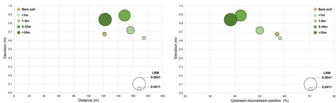
Figure 35. Vegetation height classes distribution along two connectivity gradients (distance from main channel, upstream-downstream gradient of energy) and their elevation from main channel. The surface of the circles is proportional to the mean value of local relief model (LRM).
