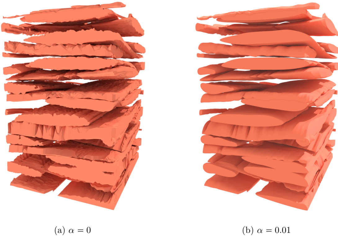
Figure 5.11 3D geometry kriging reconstructions for (a) \alpha = 0 ; (b) \alpha = 10^{-2} .
