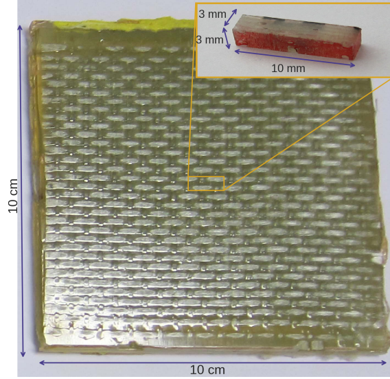
Figure 6.8 Geometry of the composite specimen and location of the sample used in the microtomographic study.
