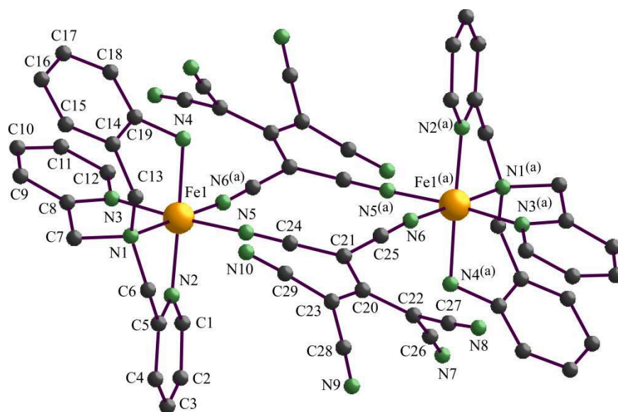
Each iron (II) metal ion presents a distorted FeN 6 octahedral environment assumed by four nitrogen atoms (N1, N2, N3, N4) arising from the tmpa neutral ligand and by two nitrogen atoms of two equivalent (tcpd) 2- anions (N5 and N6 (a) ). As indicated in table 4 , compounds 1 and 2 display different crystallographic parameters, and consequently different crystal packing are expected (see below). However, despite this difference, the structure of 2 is built from similar asymmetrical unit described above for 1 , leading to a dinuclear molecular structure of the formula [Fe 2 (andmpa) 2 (μ 2 -tcpd) 2 ]•2CH 3 OH, similar to that described for 1 ( Figure 2 ).
