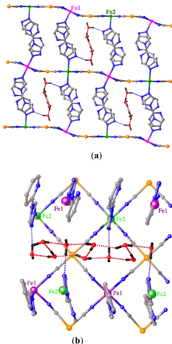
Figure 4. 3D crystal packing of 1 at ambient temperature (296 K): (a) View along the [0 1 0] direction; (b).view along the [2 0 -1] direction showing the hydrogen-bonding network between Fe2 sites. Dashed lines show the hydrogen-bonding network
