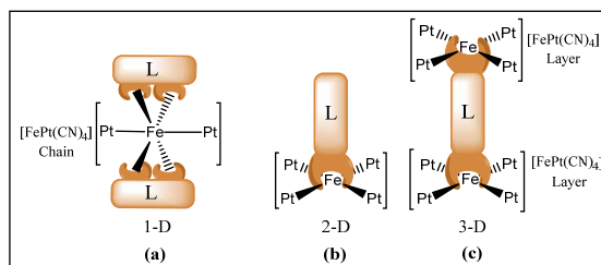
Scheme 1. Coordination modes of the ancillary L ligands for the design of bimetallic coordination polymers, including 2-D and 3-D Hoffman-type Metal-Organic Frameworks (MOFs).
