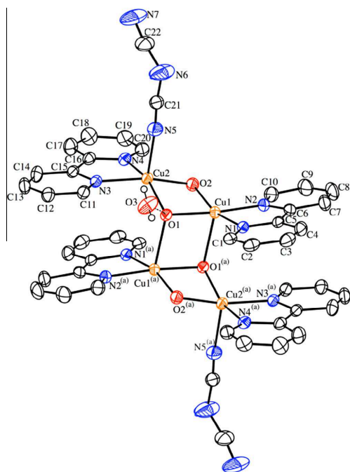
Fig. 4. Thermal ellipsoid drawing [41] (30% probability ellipsoids) of compound 2 showing the labelling scheme of the asymmetric unit and some symmetrically equivalent atoms (a) = 1 - x, -y, 1 - z . Uncoordinated dca anion and bipyridine are omitted for clarity.
