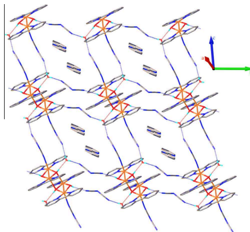
Fig. 5. Crystal packing of compound 2 along the [30\ -1] lattice vector.
