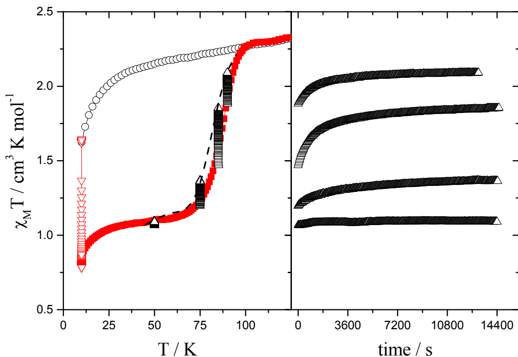
Figure S12. Left) Thermal evolution of the \chi_m T product from high temperature to low temperature in the dark (o), under 830 nm light irradiation at 10 K ( \nabla ), and in the dark after irradiation ( \square ). Isothermal relaxations from the LS-LS state, recorded at 50, 75, 85 and 90 K ( \Delta ). Right) temporal evolution of the \chi_m T product of the corresponding kinetics at 50, 75, 85 and 90 K ( \Delta ).
