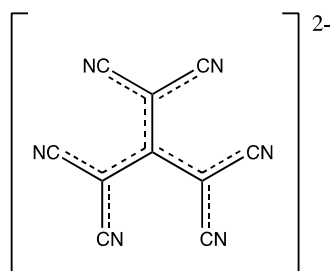
Figure I.13 Ligands (\text{tcpd})^{2-}
