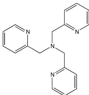
Figure II.3 Ligands tmpa
