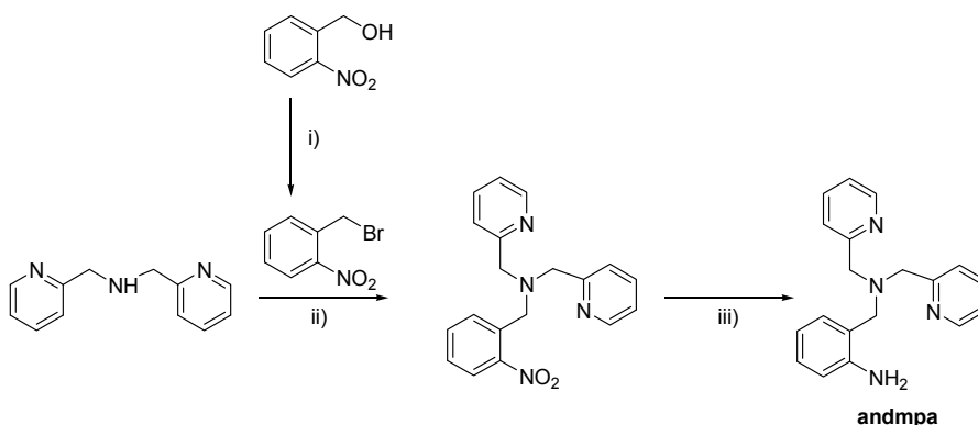
Scheme 2. Synthesis of the ligand andmpa i) 1.1 eq PBr 3 , Et 2 O, 0°C, 2h ; ii) K 2 CO 3 , CH 3 CN, reflux, 5 days; iii) NH 2 NH 2 -H 2 O, EtOH, activated charcoal, 48h.
