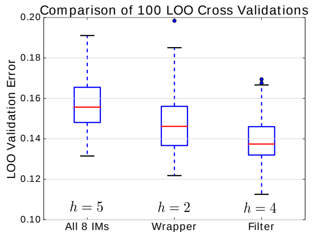
Figure 3.10: LOO cross-validation results for different ANNs
