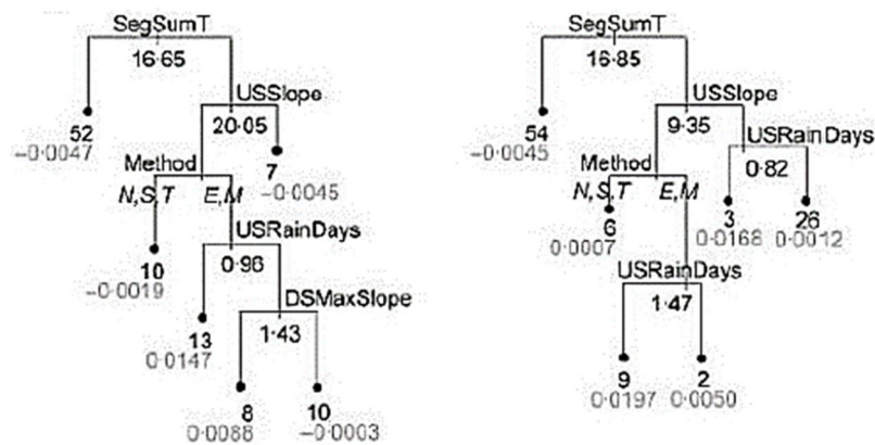
Fig. 2.19. An example of boosted regression tree used to model short-finned eels ( Anguilla australis ) occurrence. Each name (SegSumT – summer air temperature; USSlope – average slope in the upstream catchment; Method – Fishing method; USRainDays – days per month with rain >25 mm; DSMaxSlope – maximum downstream slope) represent an environmental variable that allowed to split the parent dataset (node). Split values are displayed under the split, and terminal nodes show percentage of sites in that node (black) and prediction in logit space (grey). From Elith et al. (2008).
