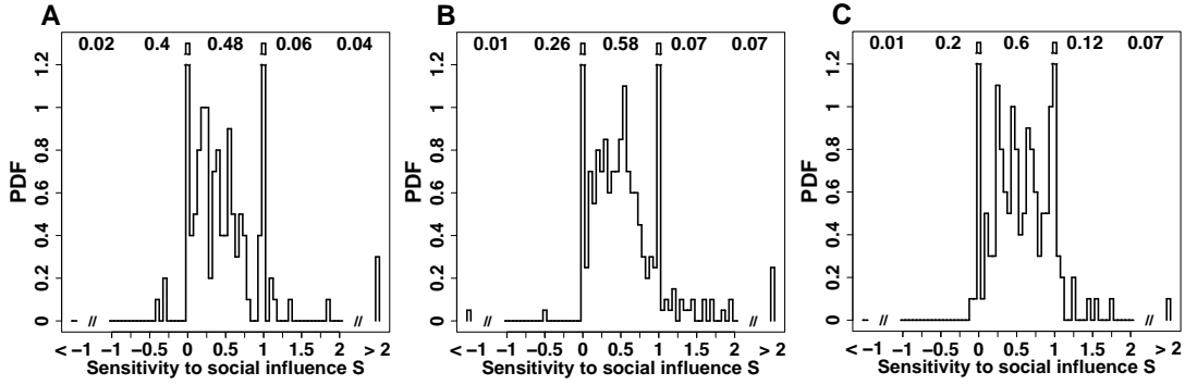
Figure 1.9: PDF of the sensitivity to social influence S , for questions 25 to 29 in the first experiment in France, in the following cases: A. confident subjects, defined as the quarter of each subgroup of 8 subjects minimizing \langle |S_q| \rangle_q , where q is the index for questions 1 to 24 (the subjects who were on average closest to S = 0 ); B. “average” subjects, defined as being neither confident nor follower; C. followers , defined as the quarter of the group minimizing \langle |1 - S_q| \rangle_q (the ones who were on average closest to S = 1 ). In A, the peak at S = 0 is almost 7 times higher than the one at S = 1 , whereas in B, it is less than 4 times, and in C, less than twice.
