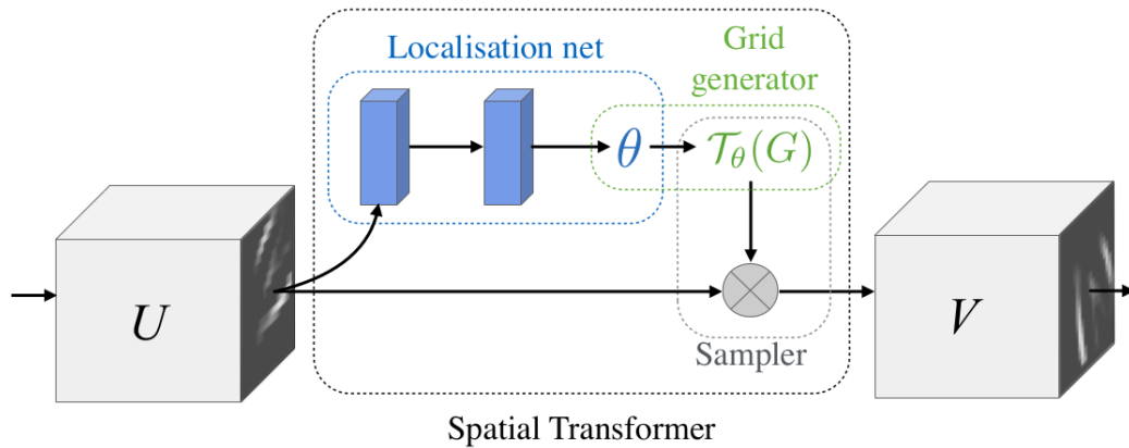
FIGURE 5.2 – Architecture d'un module ST (illustration provenant de [40]).
