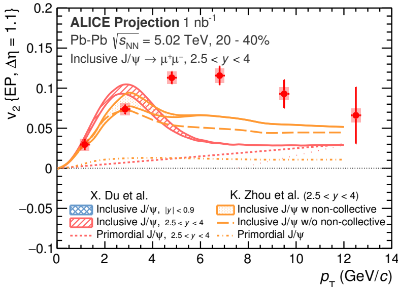
Figure 6.13 – Projection for J/\psi v_2 measurements with ALICE in Pb–Pb collisions at \sqrt{s_{\text{NN}}} = 5.02 \text{ TeV} for the full run 2 period. Calculations from [DR15] and [ZXXZ14] are shown
