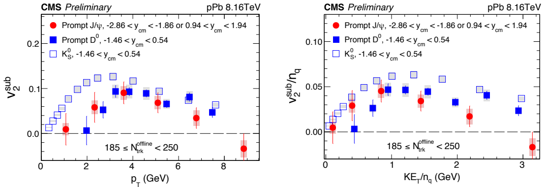
Figure 6.12 – (Top) Measurement of J/\psi elliptic flow in high-multiplicity p–Pb collisions at \sqrt{s_{NN}} = 8.16 TeV by CMS compared to D^0 and K_s^0 mesons, (Bottom) values as a function of the transverse kinetic energy ( KE_T ) and scaled by the number of constituent quarks n_q
