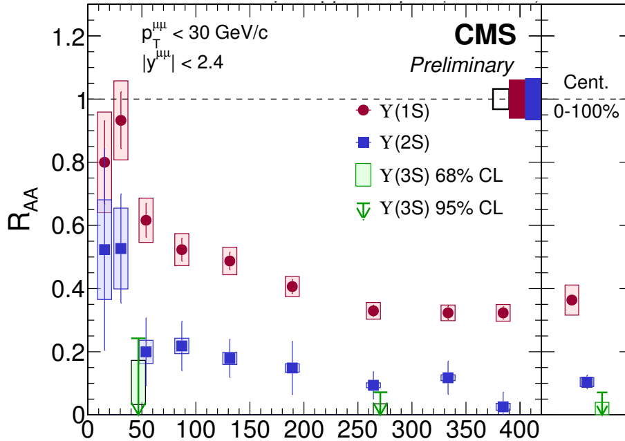
Figure 4.6 – Nuclear modification factor of \Upsilon(1S) , \Upsilon(2S) and \Upsilon(3S) states as a function of the number of participants measured by the CMS experiment at \sqrt{s_{NN}} = 5.02 TeV[S + 18b]
