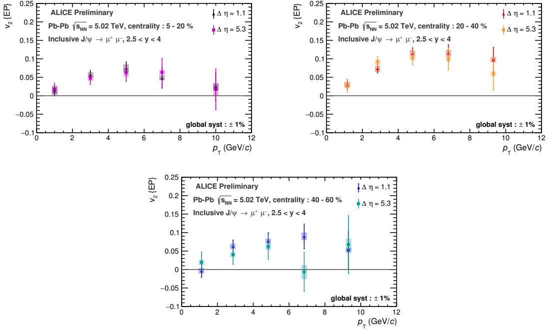
Figure 5.22 – Comparison of the results obtained with the mean v_2 method (from left to right: in the centrality classes 5–20 %, 20–40 % and 40–60 %) using the V0A ( \Delta\eta = 5.3 ) and the SPD ( \Delta\eta = 1.1 ) as event plane detector and the mean v_2 method. Boxes for systematic uncertainty contain signal extraction only.
