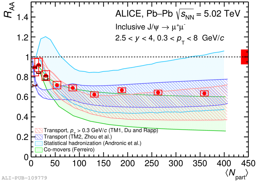
Figure 4.18 – Inclusive J/\psi R_{AA} in Pb-Pb collisions (in the 0–90 % centrality range) measured by ALICE at \sqrt{s_{NN}} = 5.02 \text{ TeV} compared to several theoretical predictions [A + 17d]
