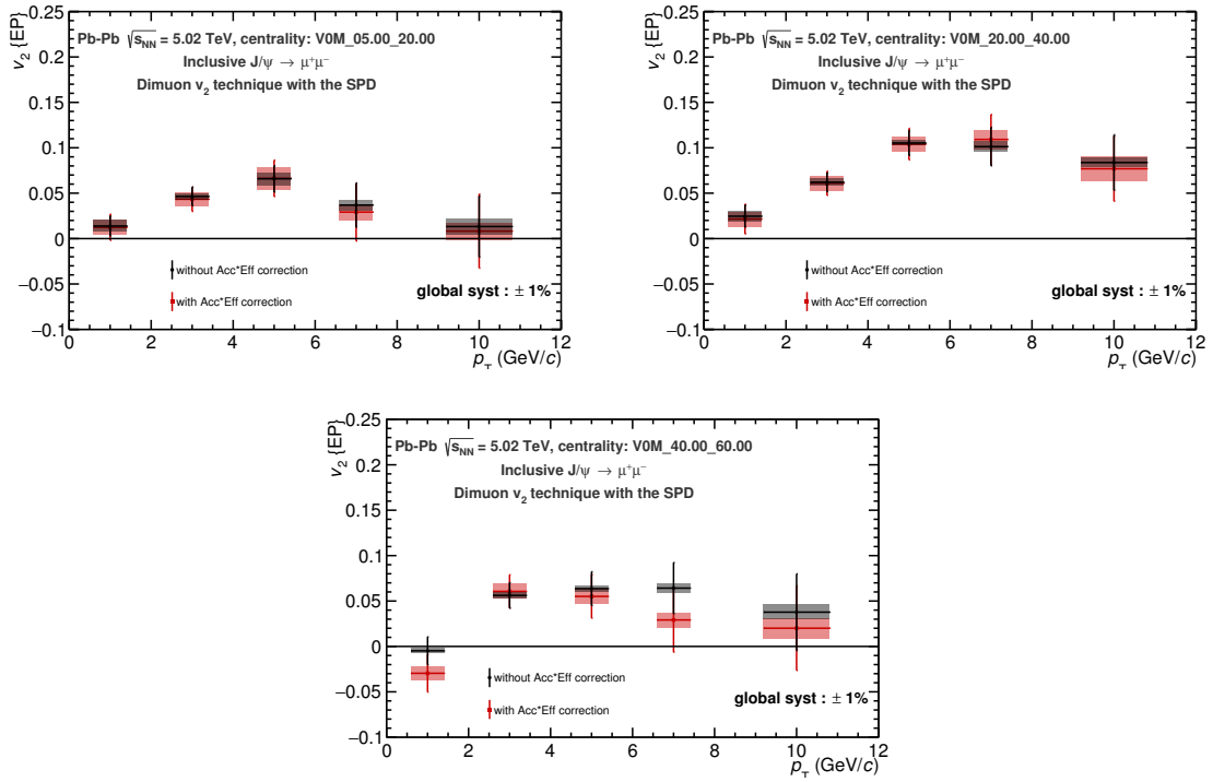
Figure 5.14 – Effect of the A\epsilon correction on results obtained with the mean v_2 method using the SPD as EP detector for different centrality ranges (from left to right: 5–20 %, 20–40 %, and 40–60 %). Boxes for systematic uncertainty contain signal extraction only.
