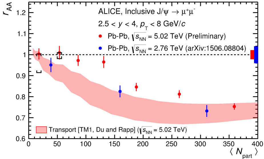
Figure 4.10 – J/\psi r_{AA} as a function of the number of participants measured by ALICE in Pb–Pb collisions at \sqrt{s_{NN}} = 2.76\text{ TeV} and \sqrt{s_{NN}} = 5.02\text{ TeV} . A comparison to a transport model is proposed [ZR11]
