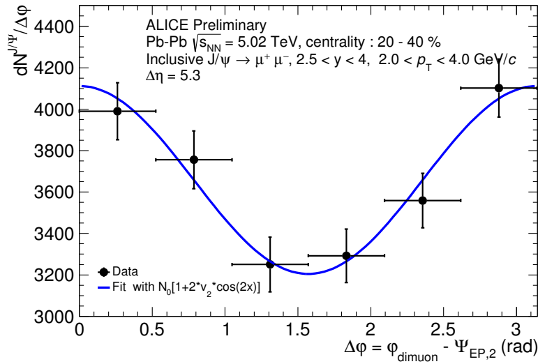
Figure 5.8 – Example of J/\psi v_2 extraction with the event plane method (SPD) for 2 < p_T < 4 \text{ GeV}/c and 2.5 < y < 4 in the centrality range 20–40% (the horizontal error bars stand for the bin widths)
