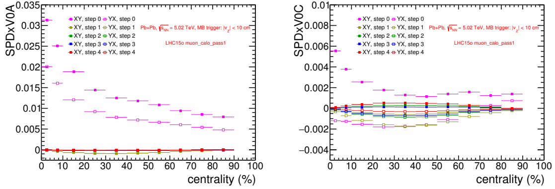
Figure 5.17 – (Left) \langle Q_{2,x}^{\text{SPD}} Q_{2,y}^{\text{V0A}} \rangle and \langle Q_{2,y}^{\text{SPD}} Q_{2,x}^{\text{V0A}} \rangle as a function of centrality after each calibration pass. (Right) \langle Q_{2,x}^{\text{SPD}} Q_{2,y}^{\text{V0C}} \rangle and \langle Q_{2,y}^{\text{SPD}} Q_{2,x}^{\text{V0C}} \rangle as a function of centrality after each calibration pass.
