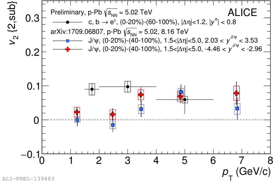
Figure 6.11 – Elliptic flow of HF-decay electrons in p–Pb at \sqrt{s_{NN}} = 5.02 TeV compared to J/\psi average at \sqrt{s_{NN}} = 5.02 TeV and at \sqrt{s_{NN}} = 8.16 TeV
