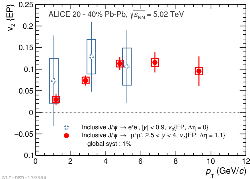
Figure 6.3 – Comparison of rapidity measurement for J/\psi v_2 in Pb–Pb collisions at \sqrt{s_{NN}} = 5.02 TeV
