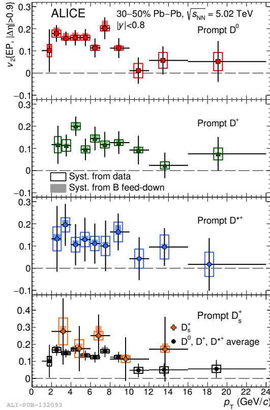
Figure 3.11 – Elliptic flow measurements in Pb–Pb collisions at \sqrt{s_{NN}} = 5.02 TeV by ALICE for D^0 , D^+ , D^{*+} , and D_s^+ mesons as a function of p_T in semi-central collisions (30–50% centrality class)
