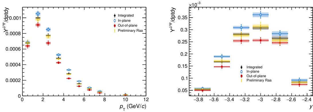
Figure B.14 – Yields comparison between in-, out-of-plane and integrated samples and previous analysis as a function of (Left) p_T and (Right) rapidity
