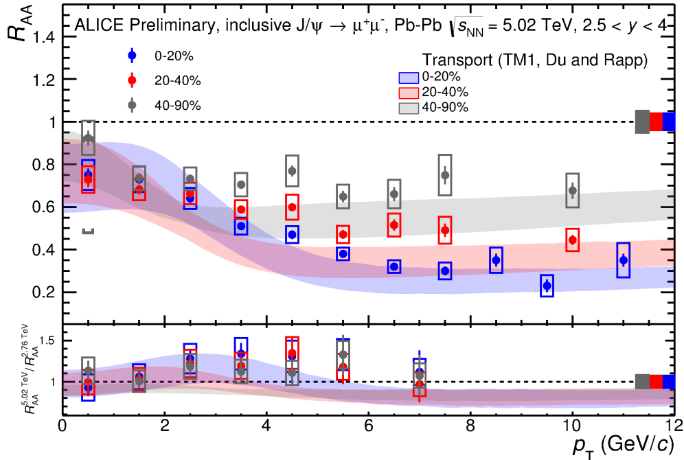
Figure 4.11 – J/\psi R_{AA} as a function of p_T measured by ALICE in Pb–Pb collisions at \sqrt{s_{NN}} = 5.02\text{ TeV} for three centrality ranges. A comparison to a transport model is proposed [DR15]
