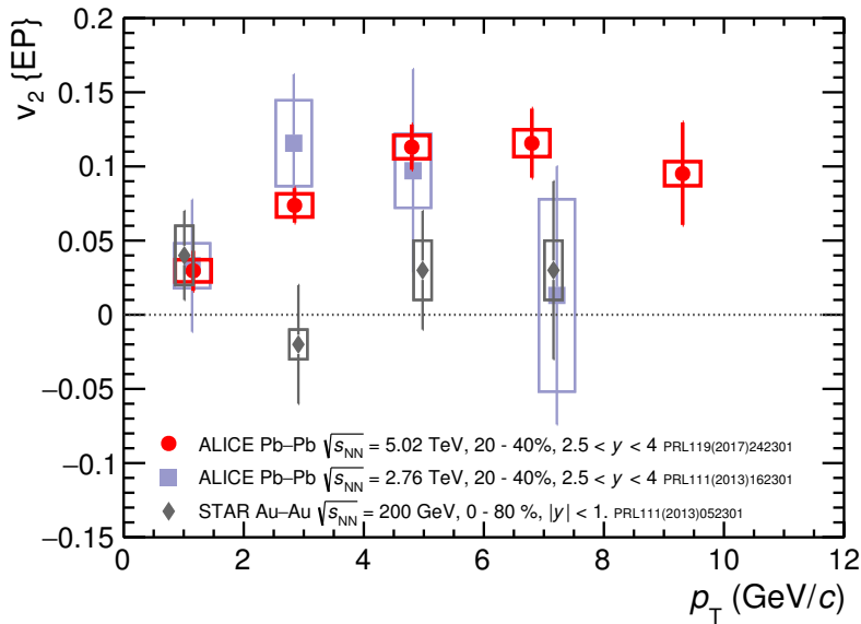
Figure 6.5 – Comparison of J/\psi v_2 measurements at the LHC by ALICE and at RHIC by STAR
