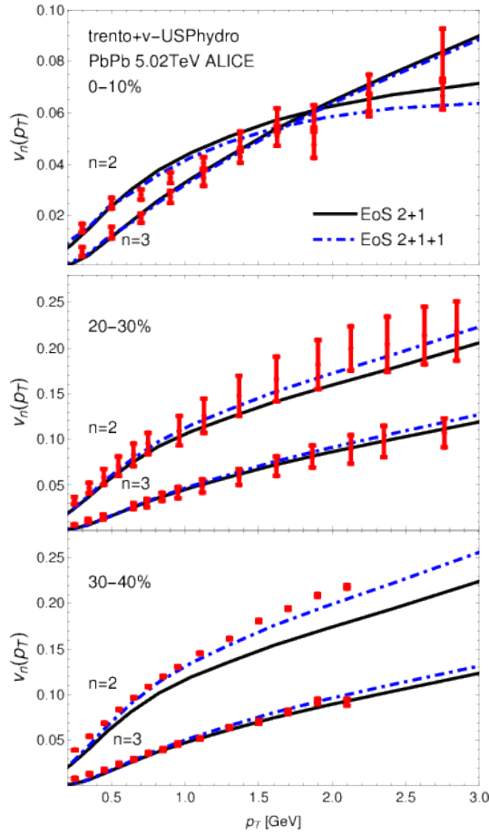
Figure 3.14 – v_n(p_T) calculations of [NHR18] in Pb–Pb collisions at \sqrt{s_{\text{NN}}} = 5.02 TeV for charged particles for the 2+1-flavour [BFH + 14] and 2+1+1-flavour [B + 16] equations of state, compared to the experimental data from ALICE [A + 16b, A + 18f]
