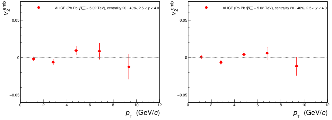
Figure 5.15 – J/\psi v_2 as a function of p_T measured in embedded MC events in the 20–40% centrality range using the V0A (Left) or the SPD (Right) as EP detector
