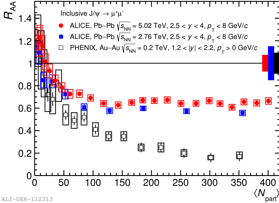
Figure 4.7 – Comparison of J/\psi nuclear modification factors as a function of the number of participants measured by PHENIX in Au–Au collisions at \sqrt{s_{NN}} = 200 GeV [A + 11c] and ALICE in Pb–Pb collisions at \sqrt{s_{NN}} = 2.76 TeV [A + 12c] and \sqrt{s_{NN}} = 5.02 TeV [A + 17d]
