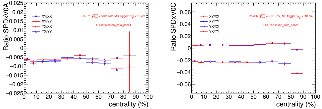
Figure 5.18 – (Left) Ratio of \langle Q_{2,x}^{\text{SPD}} Q_{2,y}^{\text{V0A}} \rangle and \langle Q_{2,y}^{\text{SPD}} Q_{2,x}^{\text{V0A}} \rangle by \langle Q_{2,x}^{\text{SPD}} Q_{2,x}^{\text{V0A}} \rangle and \langle Q_{2,y}^{\text{SPD}} Q_{2,y}^{\text{V0A}} \rangle , (Right) Ratio of \langle Q_{2,x}^{\text{SPD}} Q_{2,y}^{\text{V0C}} \rangle and \langle Q_{2,y}^{\text{SPD}} Q_{2,x}^{\text{V0C}} \rangle by \langle Q_{2,x}^{\text{SPD}} Q_{2,x}^{\text{V0C}} \rangle and \langle Q_{2,y}^{\text{SPD}} Q_{2,y}^{\text{V0C}} \rangle as a function of centrality
