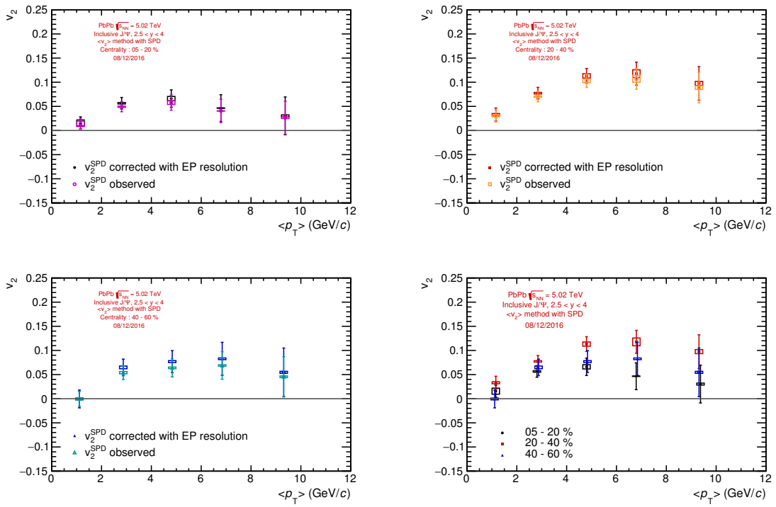
Figure 5.13 – Inclusive J/\psi v_2 as a function of p_T in the rapidity range 2.5 < y < 4 in 3 centrality classes using the mean v_2 method and the SPD as event plane detector. Boxes represent the systematic uncertainty from the signal extraction.
