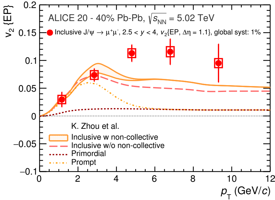
Figure 6.8 – Inclusive J/\psi v_2 at forward rapidity in semi-central Pb–Pb collisions at \sqrt{s_{\text{NN}}} = 5.02 TeV compared to TM2 [ZXXZ14] predictions
