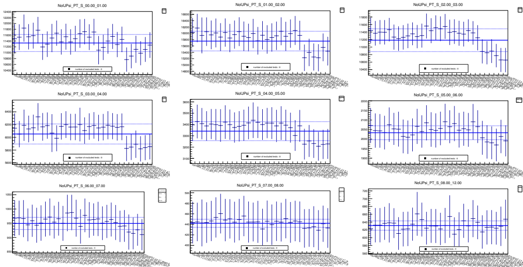
Figure B.9 – In-plane signal extraction tests for the 5-20% centrality class
