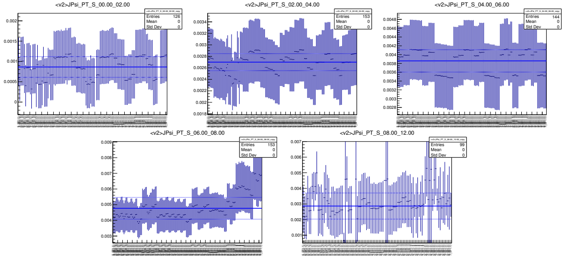
Figure B.7 – Systematics for J/\psi v_2 extraction in the centrality ranges 20-40% using the mean v_2 technique with the SP method and the VOA as EP detector
