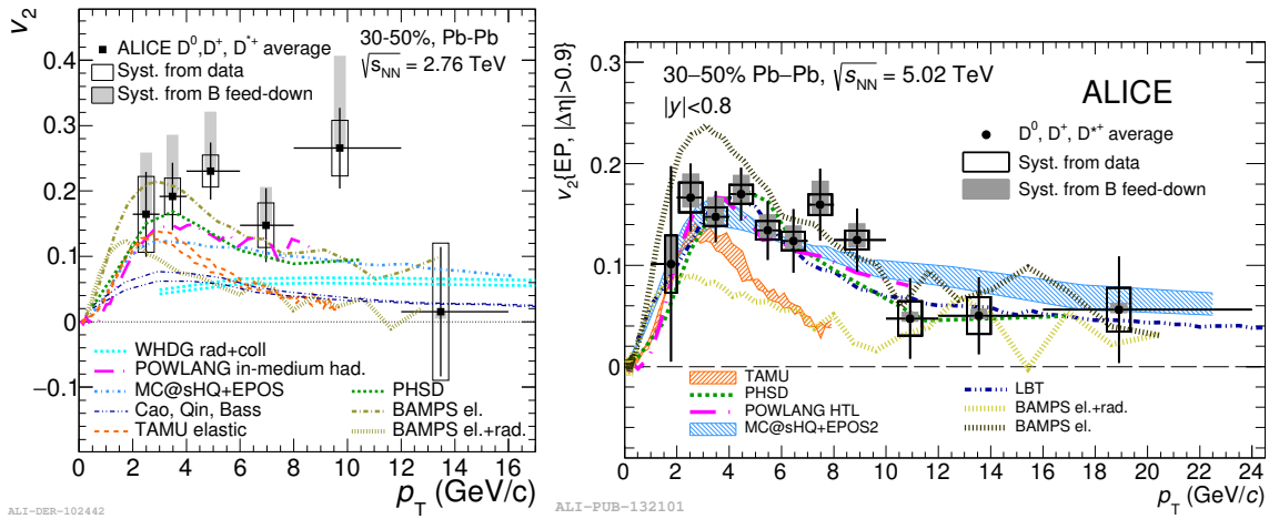
Figure 3.10 – Elliptic flow measurements in Pb–Pb collisions at \sqrt{s_{NN}} = 2.76 TeV by ALICE [A + 14e] and \sqrt{s_{NN}} = 5.02 TeV for D mesons in semi-central collisions (30–50% centrality class)
