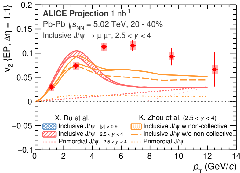
Figure 6.13 – Projection for J/\psi v_2 measurements with ALICE in Pb–Pb collisions at \sqrt{s_{\text{NN}}} = 5.02 \text{ TeV} for the full run 2 period. Calculations from [DR15] and [ZXXZ14] are shown
