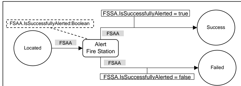
Figure 4.17 Branch Pattern Example
