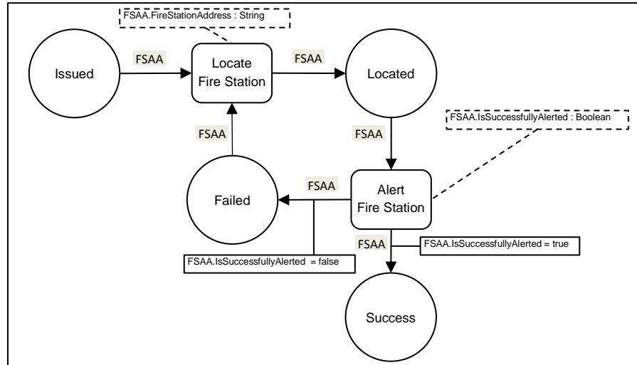
Figure 4.21 Rework Pattern Example
