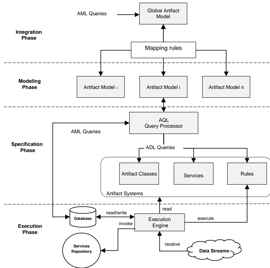
Figure 1.4. Artifact-centric process integration framework
