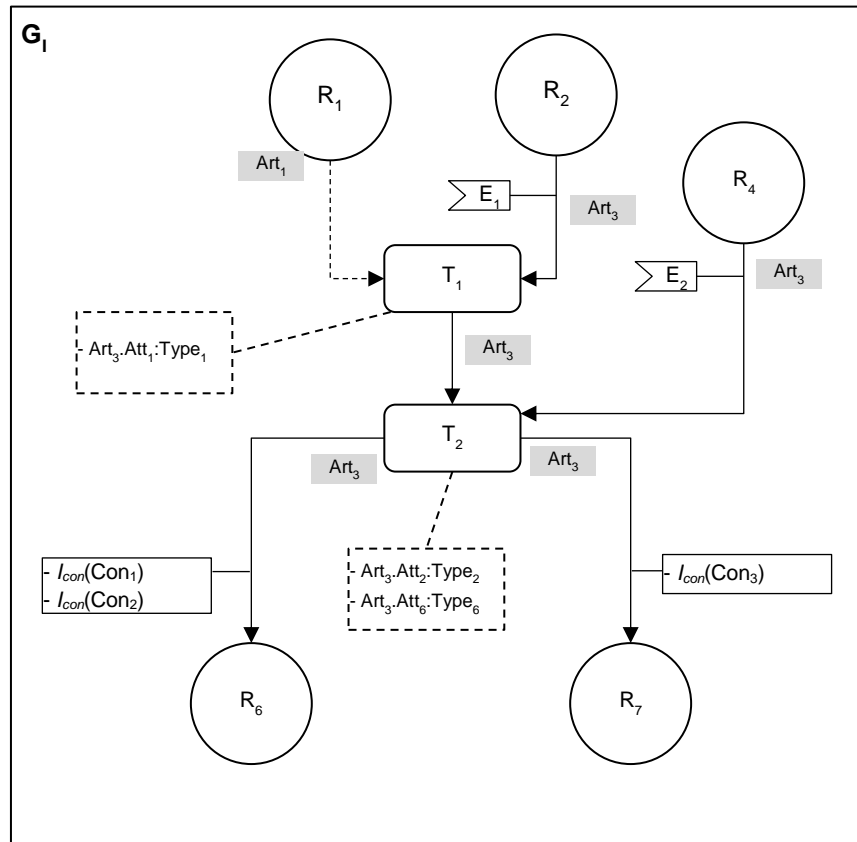
Figure 5.7 Generated global CAMs
