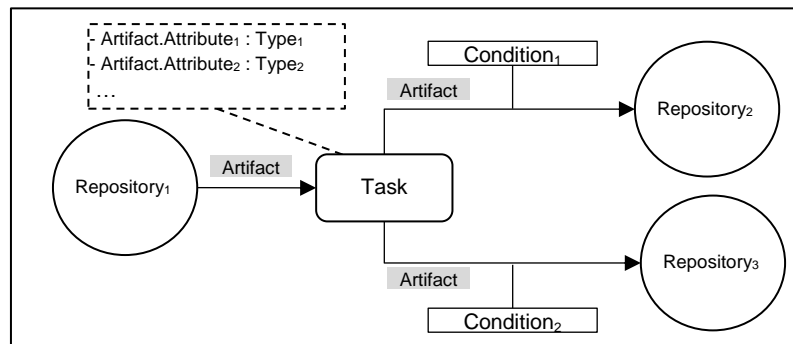
Figure 4.15 Task-centered Branch Pattern
