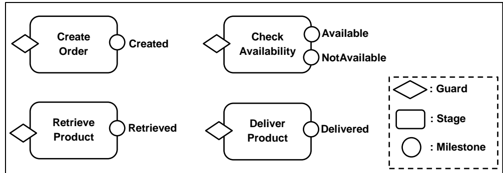
Figure 2.6 GSM representation of the Lifecycle of the Order Artifact
