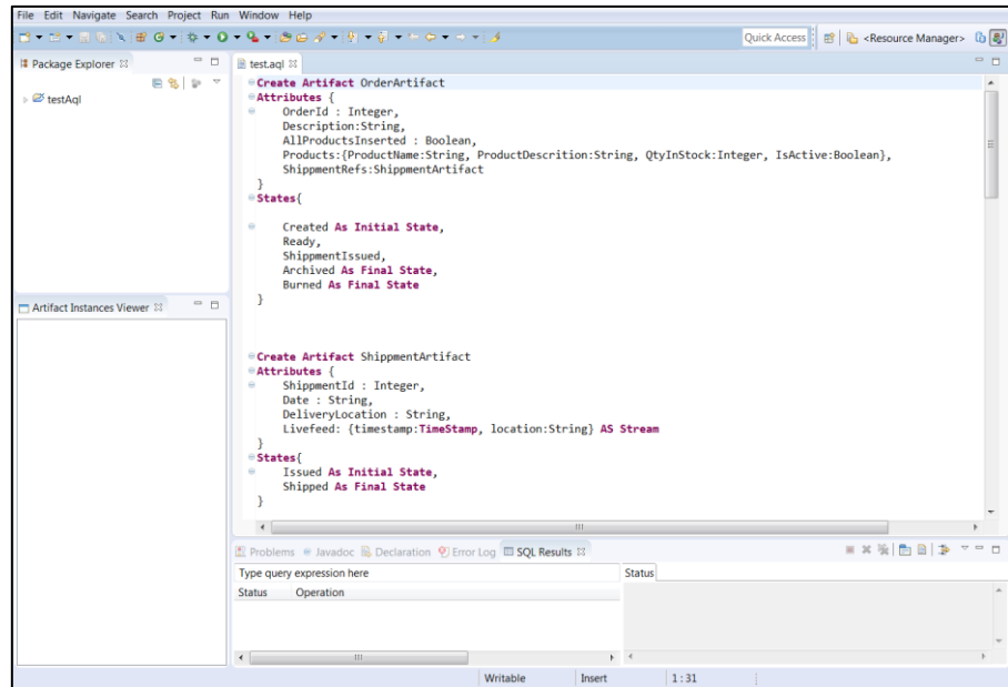
Figure 6.3 Graphical Interface of the AQL Editor
