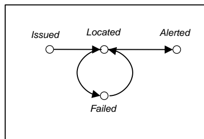
Figure 6.22 State Transitions of FireStationAlertArtifact
