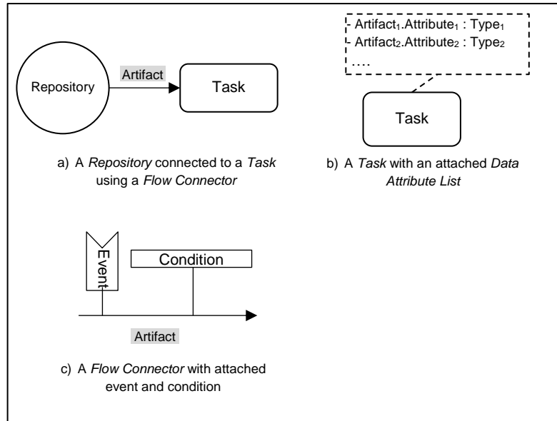
Figure 4.1 Examples of CAMN Combinations
