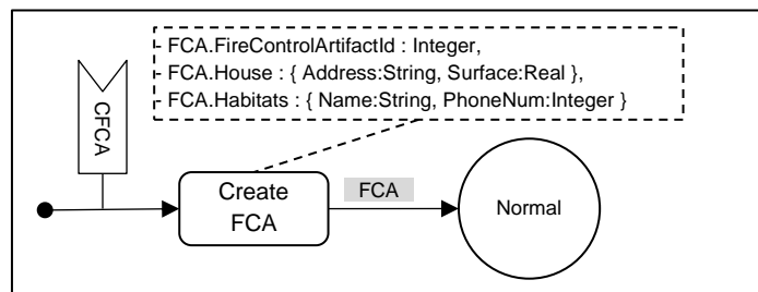
Figure 4.12 Parent Artifact Creation Pattern Example
