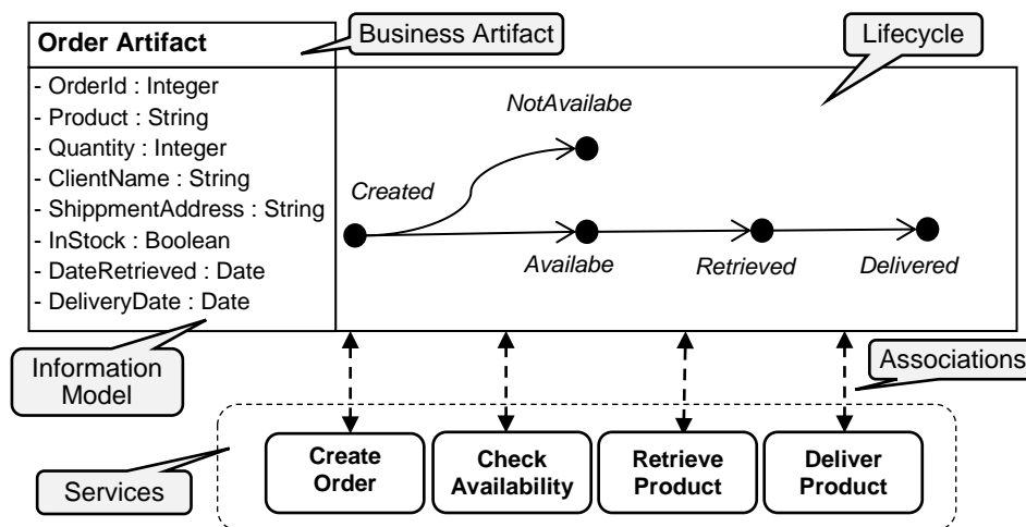
Figure 2.3 BALSA Framework example
