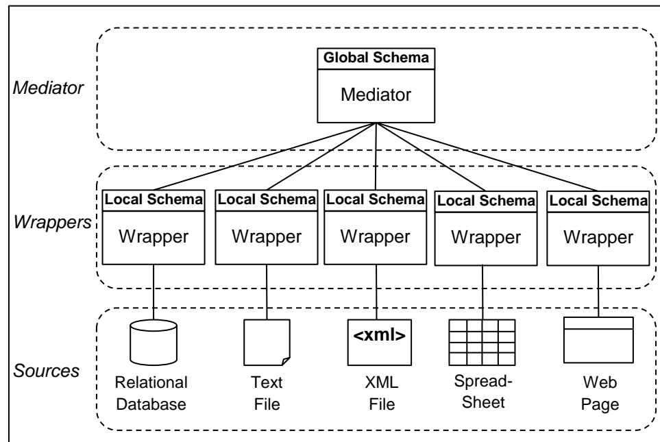
Figure 2.7 Artifact Integration System
