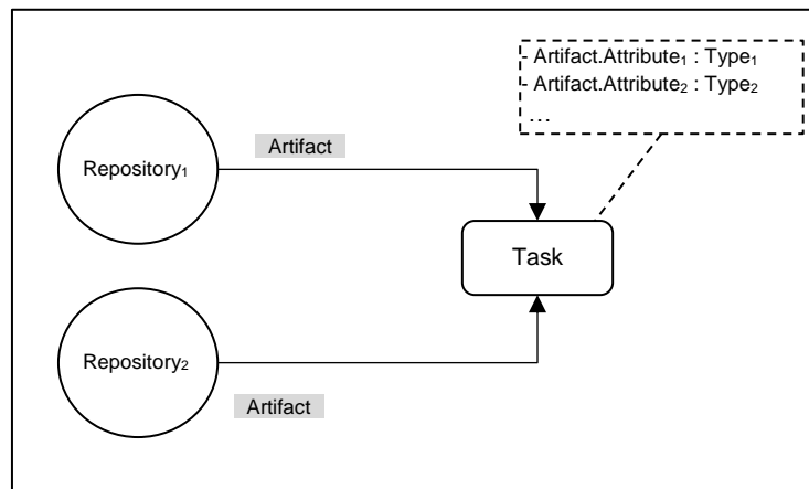
Figure 4.18 Task-centered Convergence Pattern
