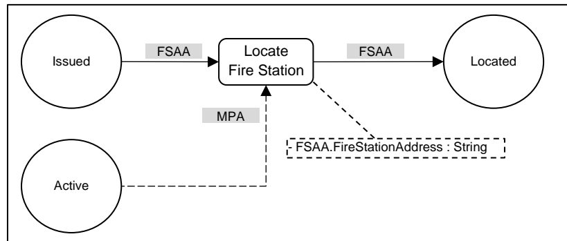
Figure 4.23 Synchronization Pattern Example
