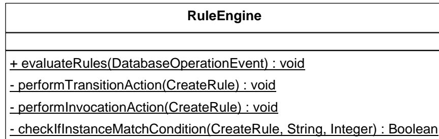
Figure 6.11 UML Class of RuleEngine
