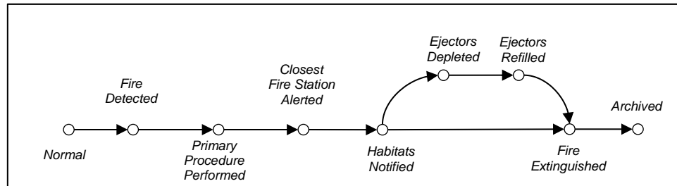
Figure 6.21 State Transitions of FireControlArtifact
