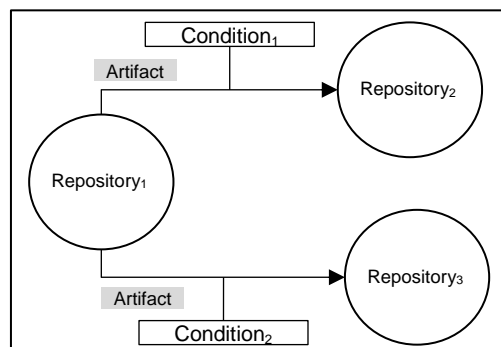
Figure 4.16 Repository-centered Branch Pattern
