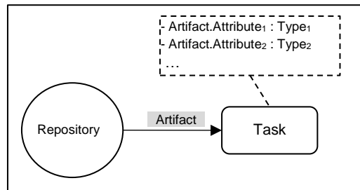
Figure 4.3 Repository-to-Task Transition Pattern
