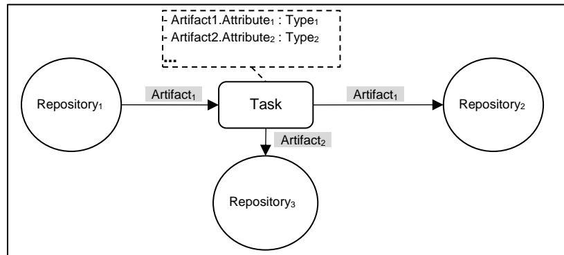
Figure 4.13 Child Artifact Creation Pattern
