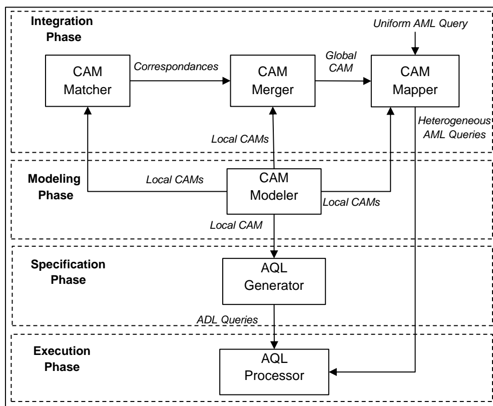
Figure 6.1 Main Modules of Artifact Integration Framework
