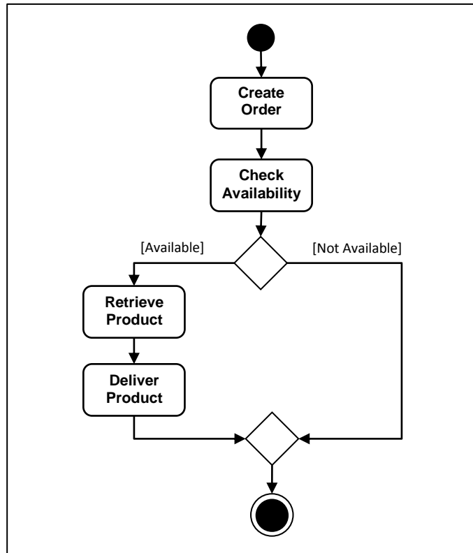
Figure 2.2 UML Activity Diagram example
