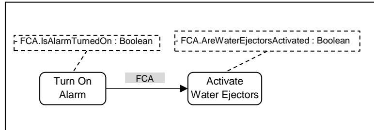
Figure 4.8 Task-to-Task Transition Pattern Example
