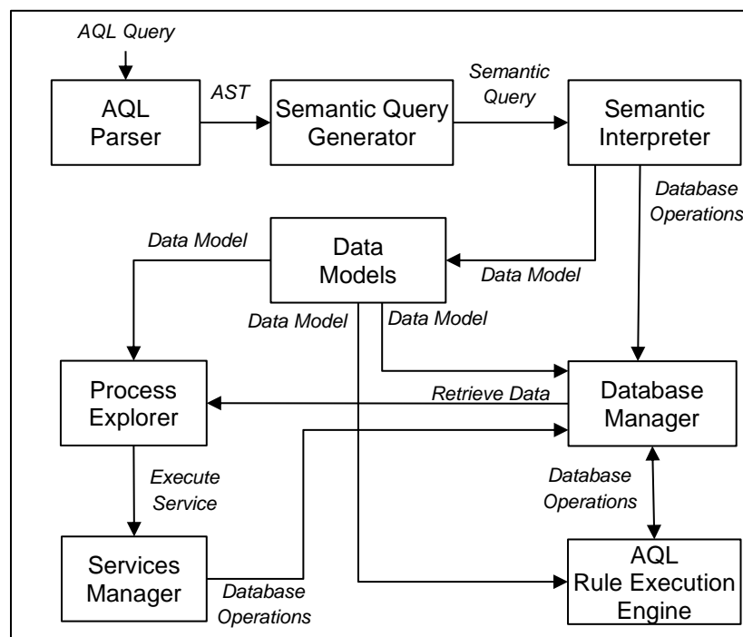
Figure 6.2 AQL Processor Architecture
