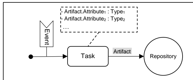
Figure 4.11 Parent Artifact Creation Pattern
