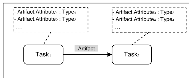
Figure 4.7 Task-to-Task Transition Pattern
