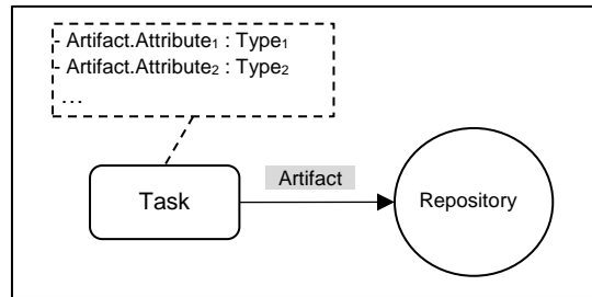
Figure 4.5 Task-to-Repository Transition Pattern
