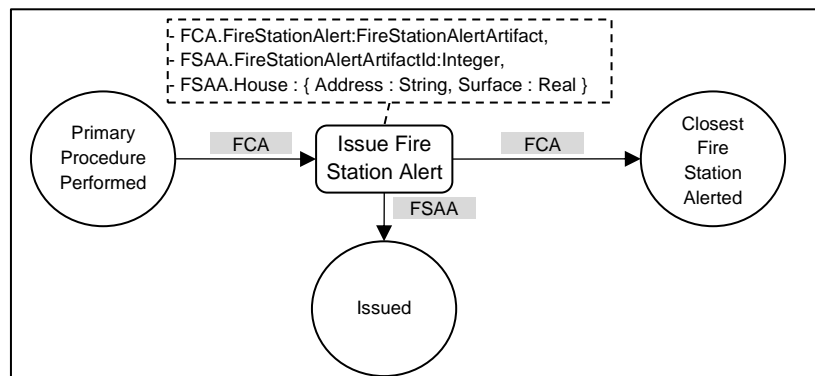
Figure 4.14 Child Artifact Creation Pattern Example
