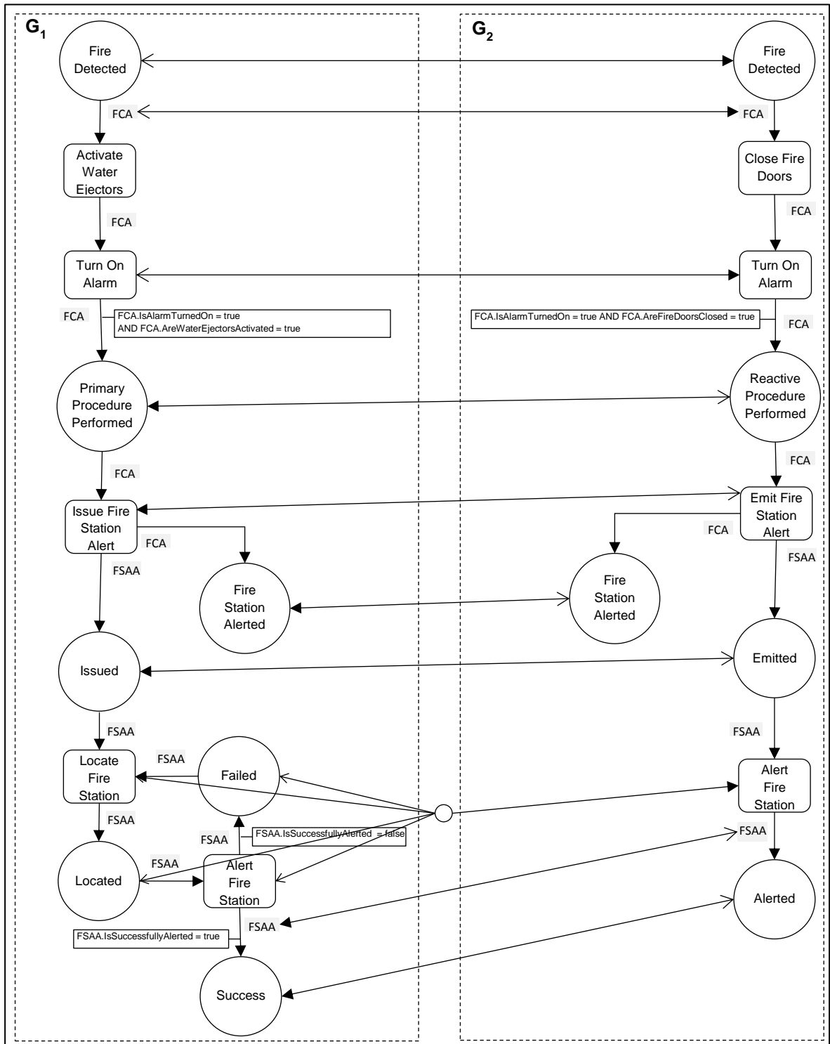
Figure 6.24 Fire Control Local CAMs Correspondences
