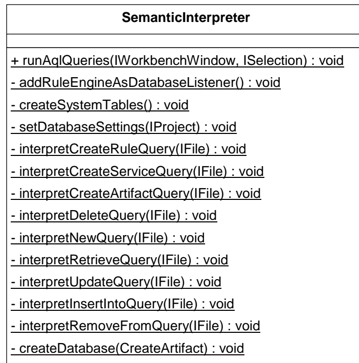
Figure 6.5 UML Class of SemanticInterpreter
