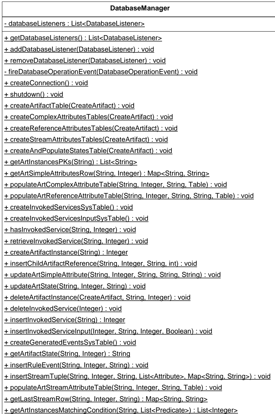
Figure 6.10 UML Class of DatabaseManager
