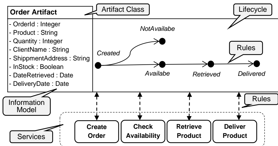
Figure 1.1 Artifact System example
