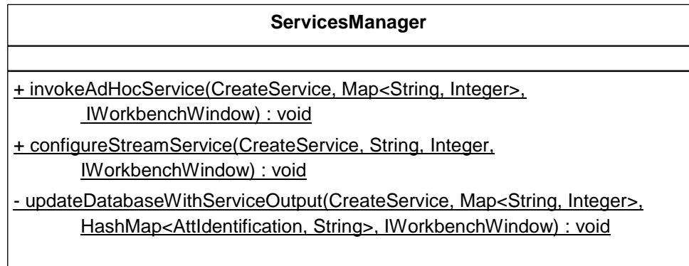
Figure 6.15 UML class of ServicesManager
