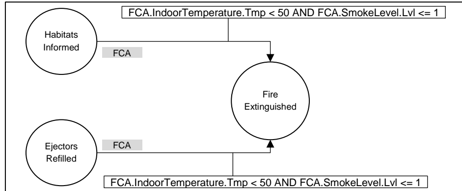
Figure 4.19 Repository-centered Convergence Pattern
