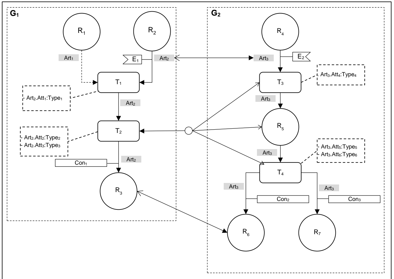
Figure 5.5 Merging Sub-Phase local CAMs example
