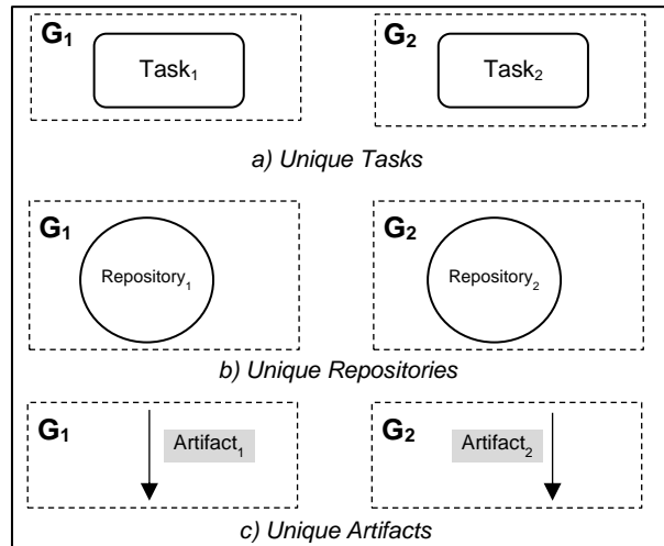
Figure 5.2 Uniqueness correspondence relationships for Tasks, Repositories, and Artifacts
