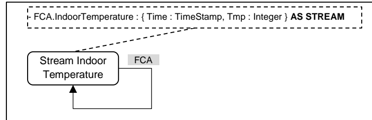
Figure 4.25 Streaming Pattern Example
