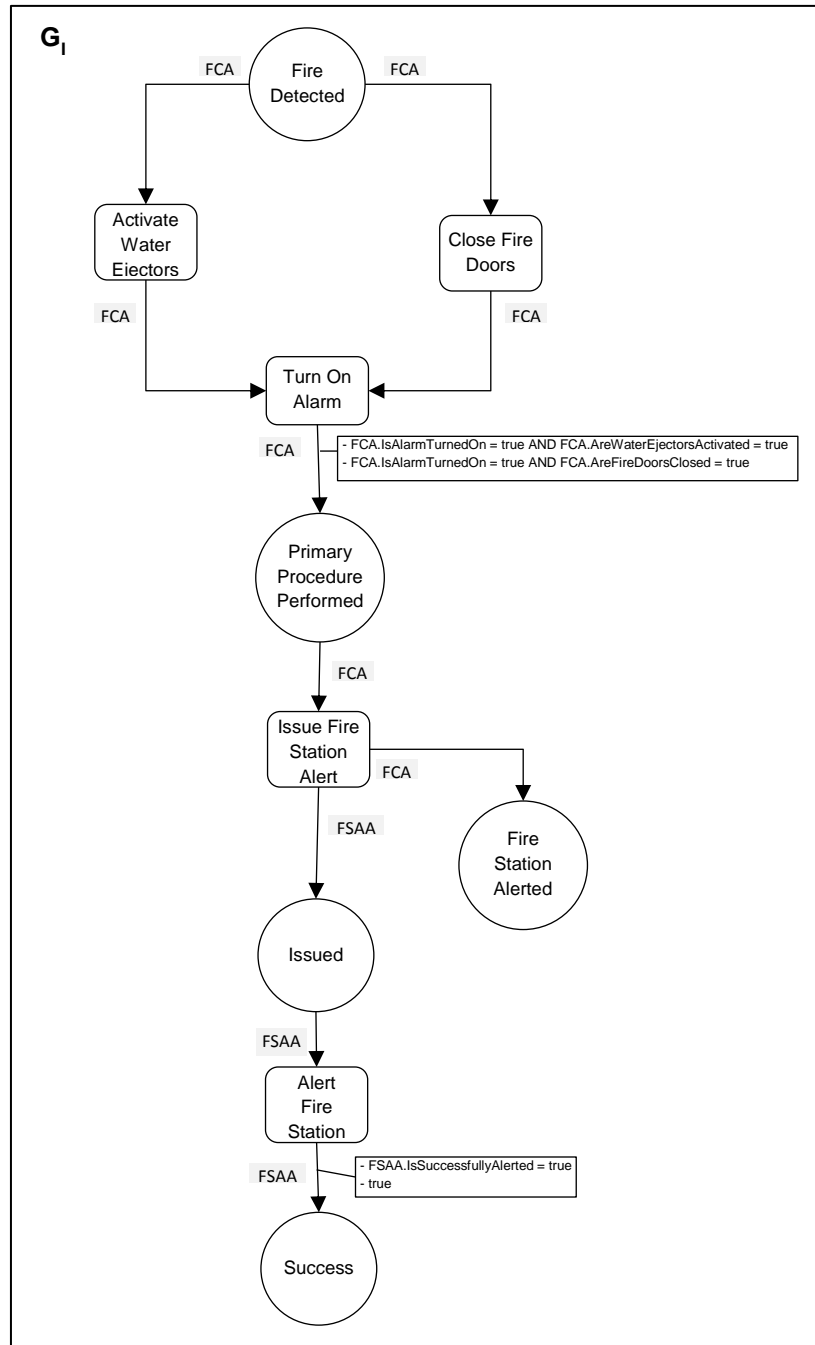
Figure 6.25 Fire Control Global CAM
