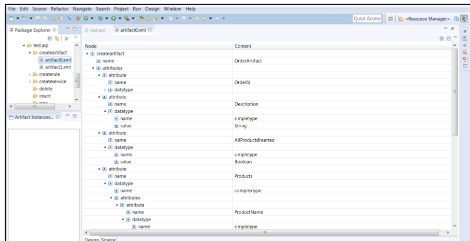
Figure 6.4 Generated XML Semantic Query
