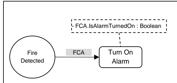
Figure 4.4 Repository-to-Task Transition Pattern Example
