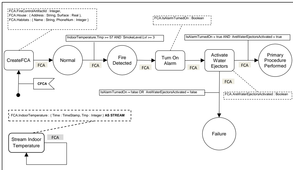
Figure 4.2 Part of Fire Control Conceptual Artifact Model
