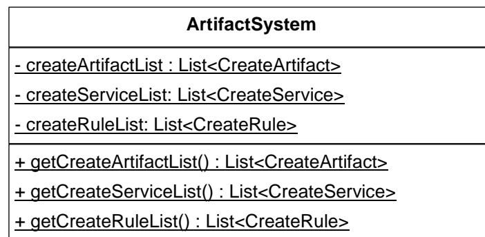
Figure 6.7 UML Class of ArtifactSystem
