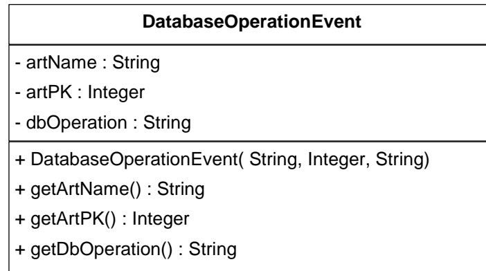
Figure 6.9 UML Class of DatabaseOperationEvent
