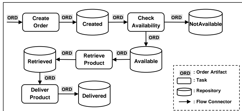
Figure 2.4 Lifecycle of Order artifact as Tasks, Repositories and Flow Connector
