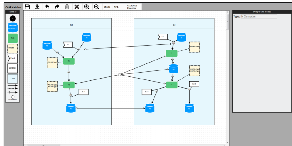
Figure 6.19 CAM Matcher Main Graphical Interface
