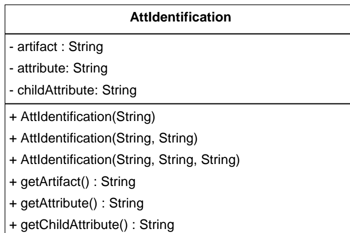
Figure 6.8 UML Class of AttIdentification
