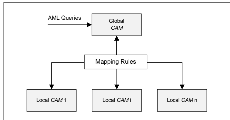
Figure 5.1 Artifact Integration System
