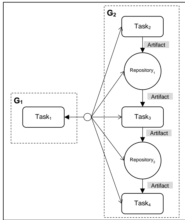
Figure 5.4 Composition correspondence relationship for Tasks
