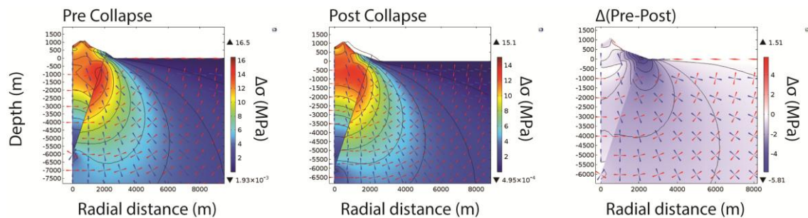
Figure 6.3 Stress field before and after the collapse. The oblique line separates volcano to the left and basement rocks to the right. The change in effective stress after the collapse would be up to 4 MPa and would reach a depth of 6 km.
