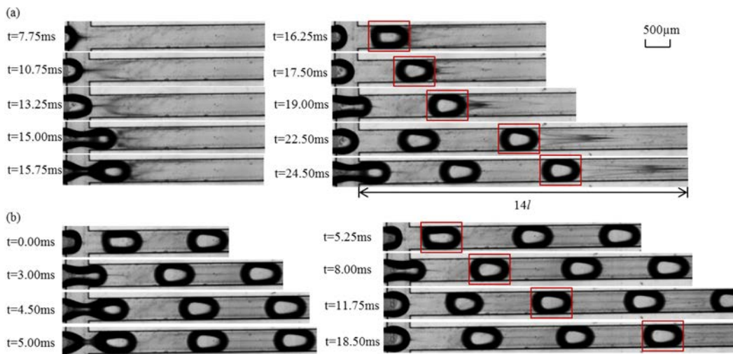
Fig. 3-3 Typical images of the mass transfer process ( j_G= 0.053 \text{ m} \cdot \text{s}^{-1} , j_L= 0.27 \text{ m} \cdot \text{s}^{-1} ). (a) just after the moment where both gas and liquid phases are injected in the microchannel (transient period). (b) when steady state is reached. The bubble in the red rectangle represents the bubble observed.
