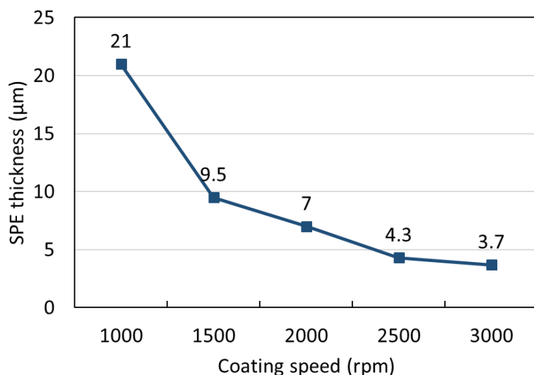
Fig. 14. Relationship between rotation speed of spin-coater for deposition of NBR/PEO and its resulting thickness
