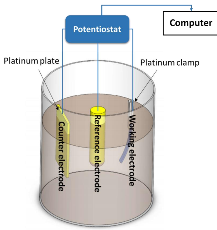
Fig. 4. Three-electrode system for setting the oxidation state of the PEDOT and for cyclic voltammetry analysis.
