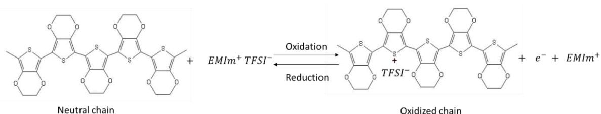
Fig. 2. Cation driven actuation in a PEDOT-based actuator.
