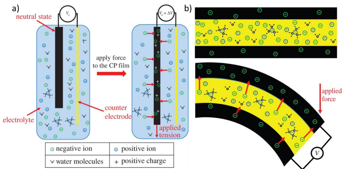
Fig. 1. a) Schematic of CP free-standing film sensing mechanism before and after subjected to a linear force, and b) Schematic of a bending trilayer sensor [4]
