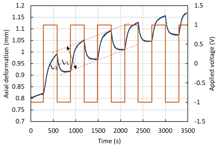
Fig. 18. Uniaxial deformation of the trilayer actuator under a step voltage
