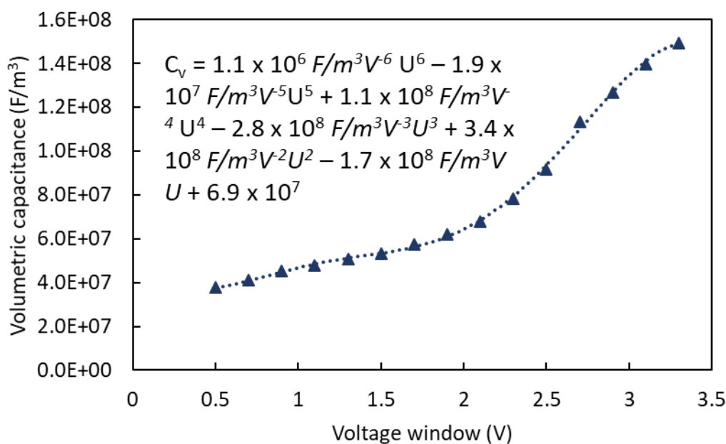
Fig. 8. Volumetric capacitance as a function of the voltage window from 0.5 Vpp to 3.3 Vpp.
