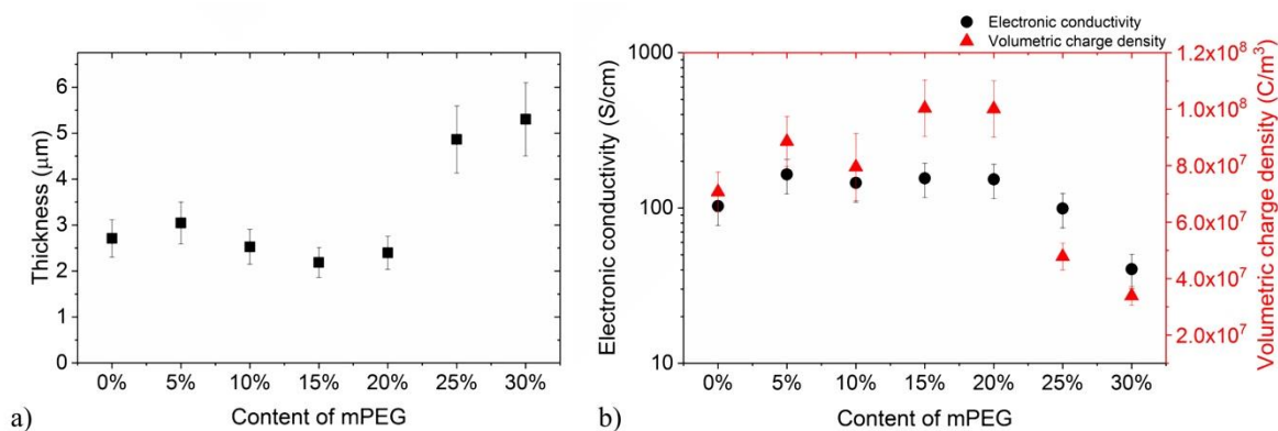
Fig. 1. Results of mPEG content in the oxidant solution: thickness (a-■), electronic conductivity (b-●), and volumetric charge density (b-▲) at a scan rate of 20 mV/s and a voltage window of 2 V. Spin coating speed/acceleration/duration of oxidant solution: 2500 rpm/1000 rpm \text{s}^{-1} /30 s; EDOT VPP time: 30 min; EDOT VPP temperature: 40 ^{\circ}\text{C} .
