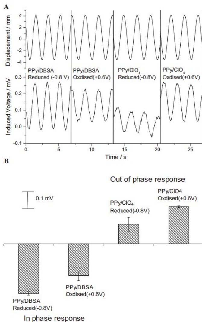
Fig. 2. Effect of counter-ion and redox state on the voltage output of polypyrrole mechanical sensor [2] (Reprinted with permission from John Wiley and Sons)
