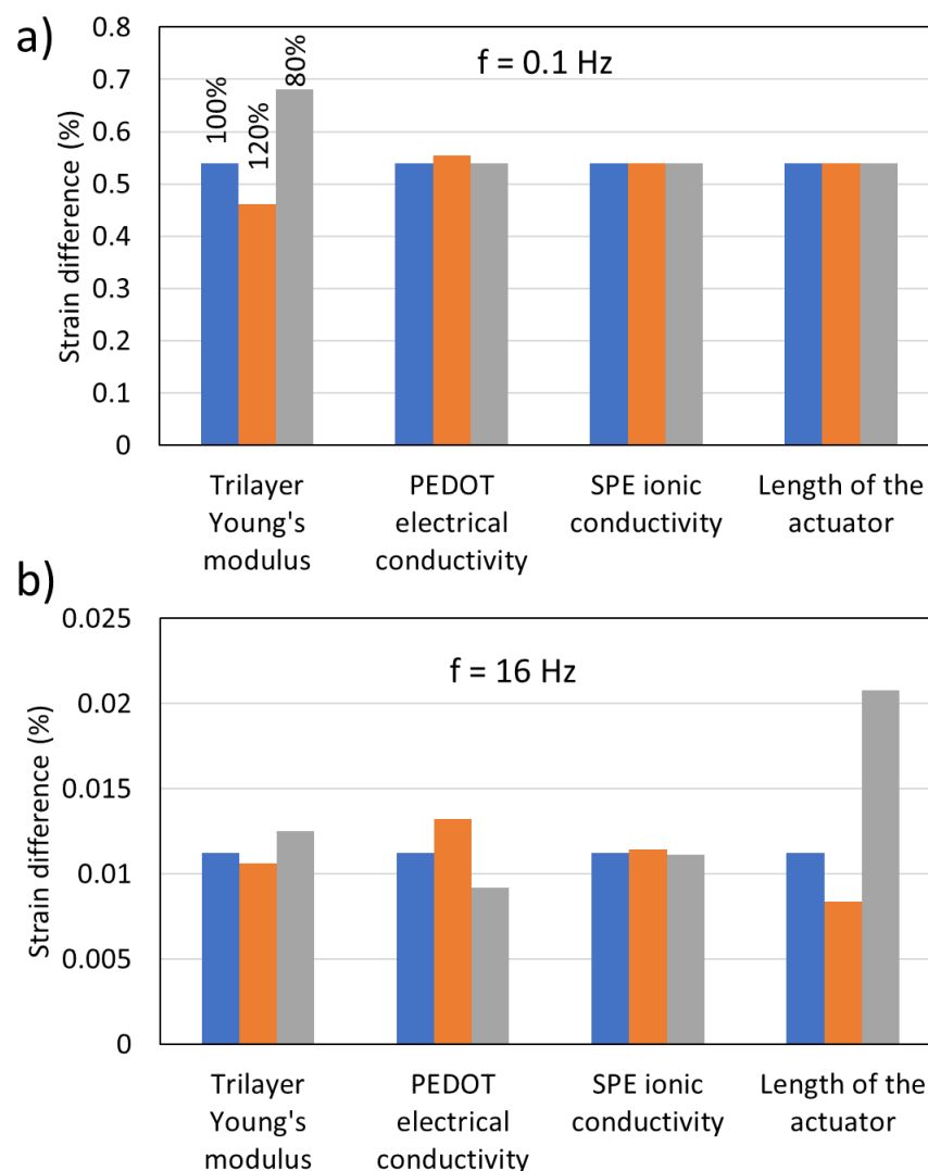
Fig. 22. Key factors affecting the actuator displacement under a square wave voltage ( V_{pp} = 2.4 V), a) at low frequency f = 0.1 Hz, and b) at high frequency f = 16 Hz. For each parameter,
