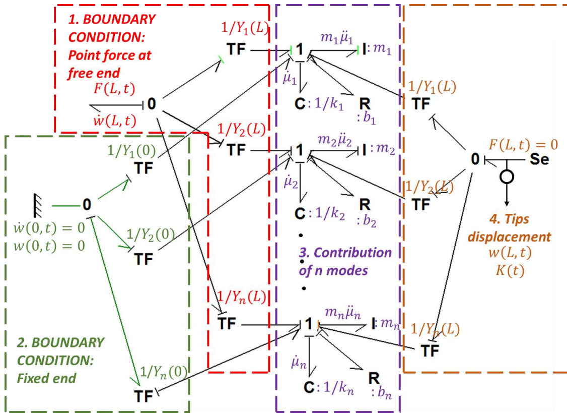
Fig. 10. BG representation of the mechanical model of the trilayer actuator, the block 1 (red color) indicates the point force F(L, t) obtaining from the electromechanical coupling matrix applying to the free end of the beam, the block 2 (green color) presents the boundary condition where one end of the beam is fixed, the block 3 (pink color) is a BG presentation of the equation (25), and finally the block 4 (orange color) introduces the method to extract the tips displacement of the beam w(L, t) .
