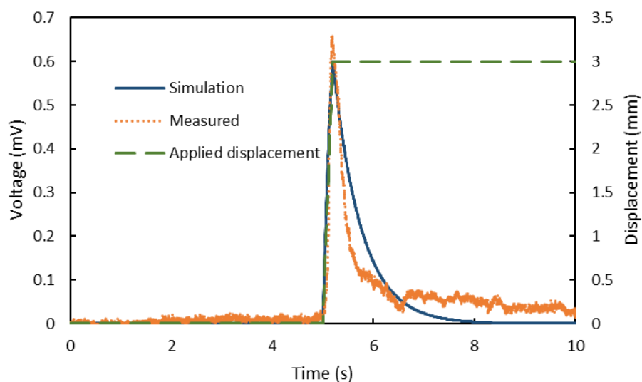
Fig. 11. Comparison between the simulation and measured voltage responding to an applied step displacement
