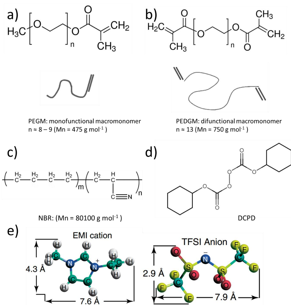
Fig. 9. Molecular formula of a) the precursor PEGM, b) PEDGM, c) the linear chain NBR, d) the initiator DCPD, and e) the ionic liquid EMITFSI [46] (Reprinted with permission from American Chemical Society, 2008.)
