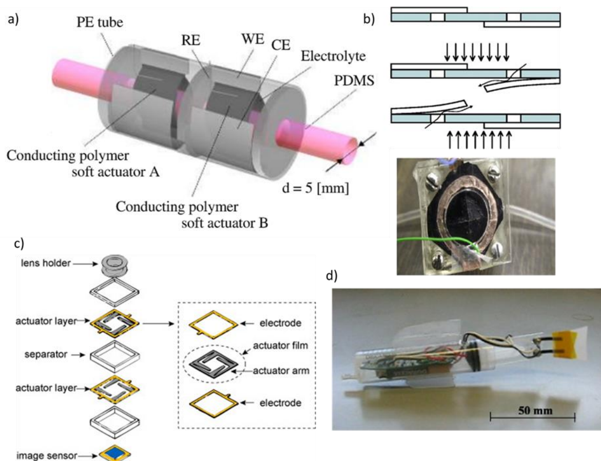
Fig. 5. a) Schematic of a micropump driven by a PPy-based CP actuator [12] (Reprinted with permission from John Wiley and Sons), b) A diagram pump: the mechanism of flap check valves and a bottom view of the assembled micropump [13] (Reprinted with permission from Elsevier), c) Micro autofocus lens actuator that uses bending conducting polymer actuators [14] (Reprinted with permission from Elsevier), d) A prototype of a robotic fish [15] (Reprinted with permission from IOP Publishing)
