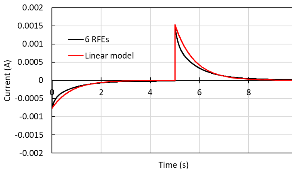
Fig. 14. Comparison between the output current of the linear model and nonlinear (6 RFEs) responses to a step voltage of 2 V_{pp} at f = 0.1 Hz
