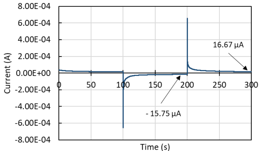
Fig. 9. The current response to an input step voltage at low frequency ( f = 0.005 Hz)
