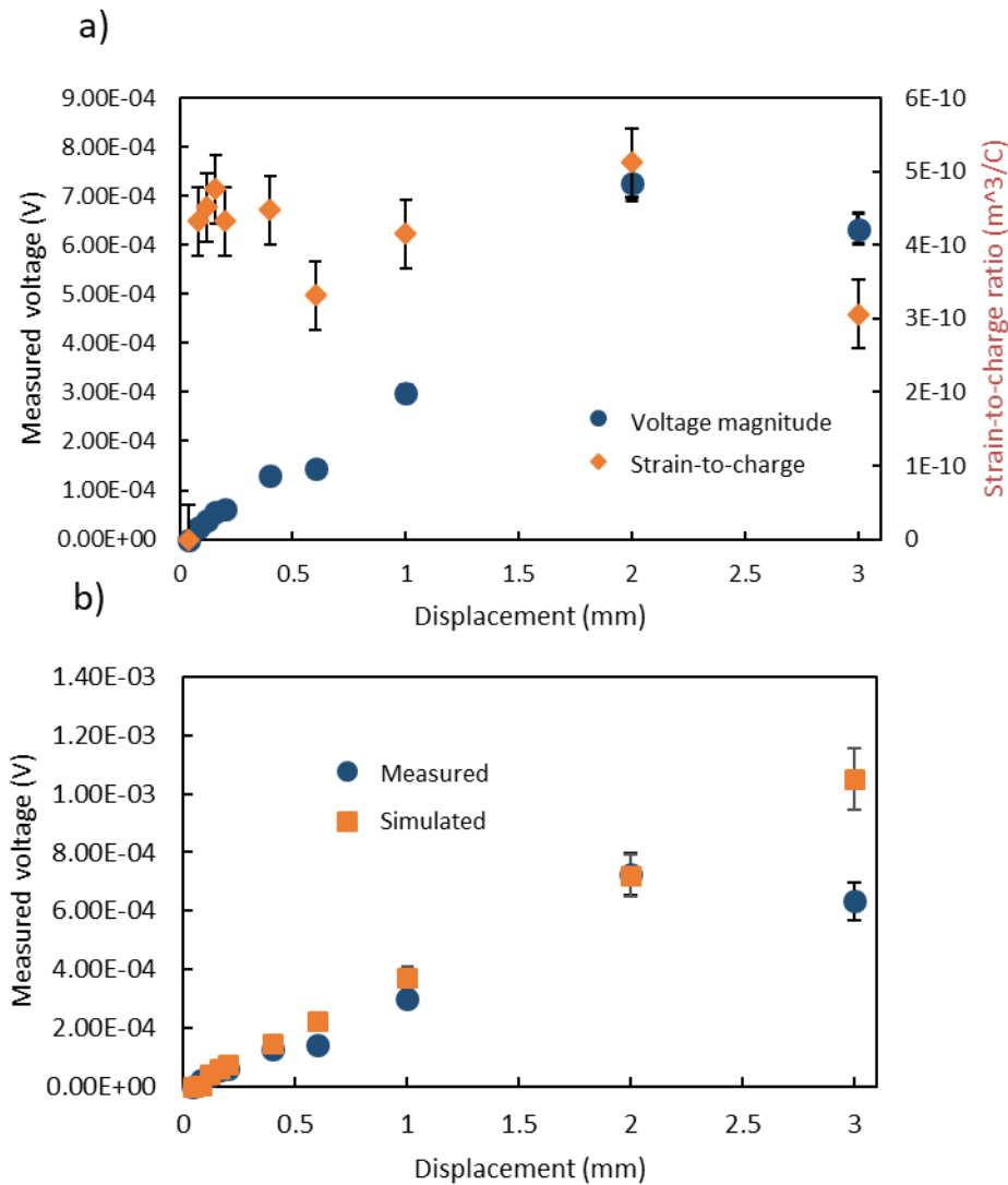
Fig. 10. a) Voltage magnitude and the strain-to-charge ratio as a function of magnitude when the frequency of displacement is constant at 3 Hz, b) Comparison between simulation and experiment of the magnitude of output voltage
