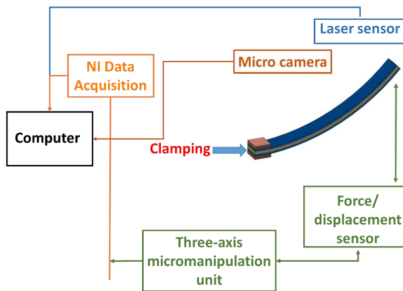
Fig. 12. Experimental setup to measure the damping ratio of the trilayer actuator and the blocking force
