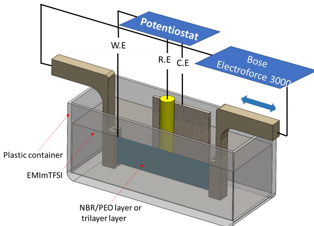
Fig. 10. Young's moduli of the NBR-PEO layer alone - and of a trilayer structure as a function of oxidation state - were measured using a Bose Electroforce 3000 dynamic mechanical analyzer
