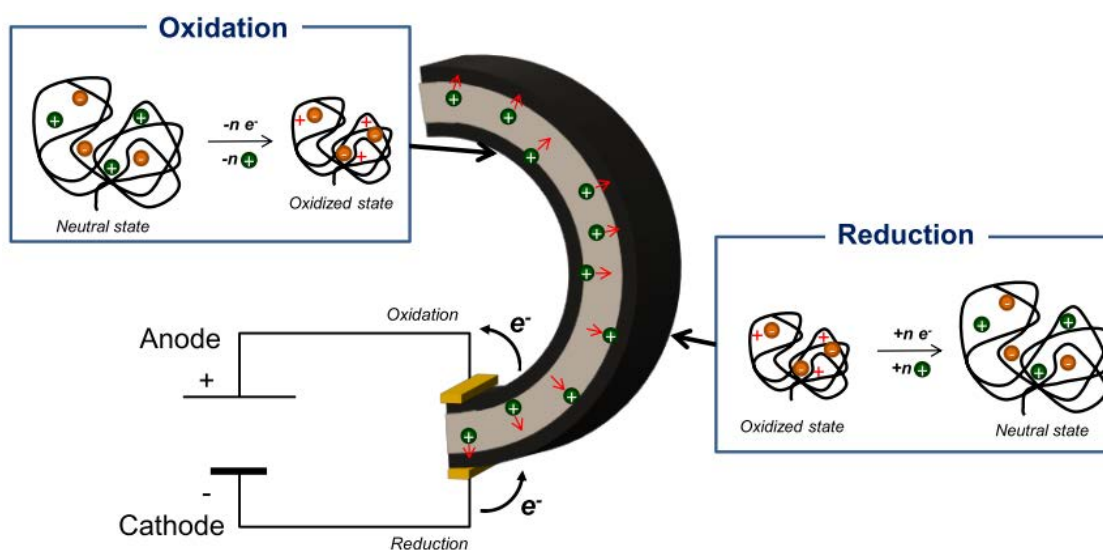
Fig. 3. Bending actuation mechanism of PEDOT-based trilayer actuators. The anode contracts due to ion expulsion and the cathode expands due to cation incorporation, leading to bending.
