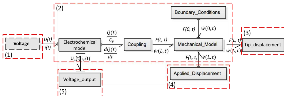
Fig. 6. Global Word BG model, where (1) and (3) represent the input voltage and the tip displacement, respectively, as the trilayer structure in actuation mode; the (4) and (5) are the input displacement and the voltage output, respectively, when the trilayer is operated as a sensor, (2) is the global BG model
