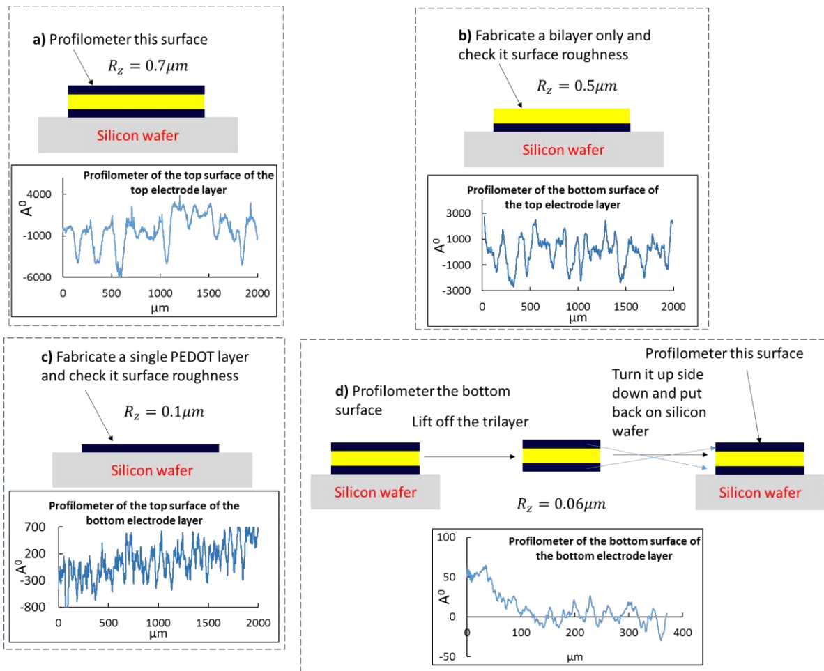
Fig. 5. Surface roughness measurement apparatus
