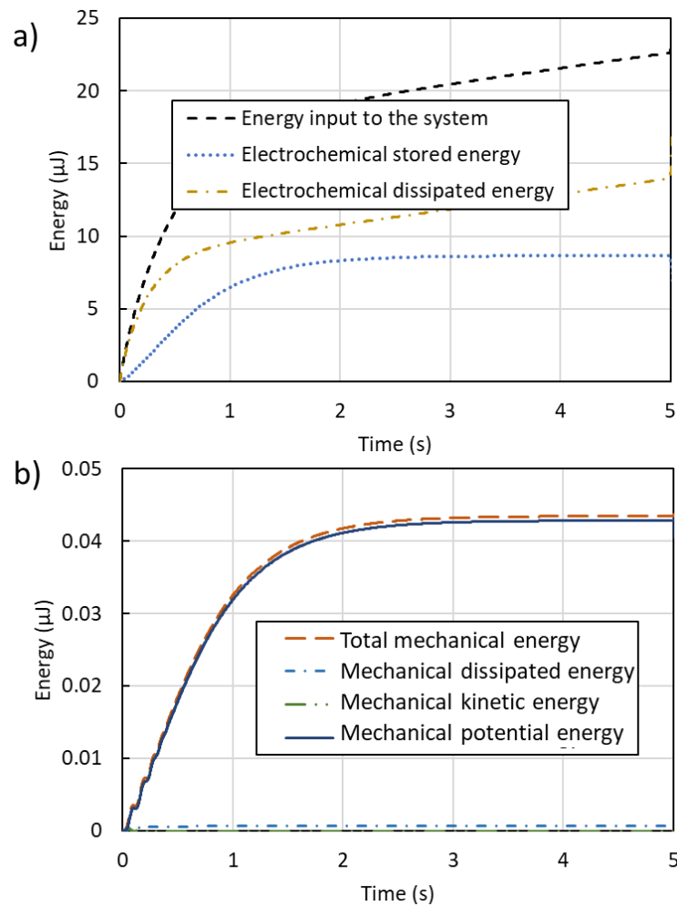
Fig. 23. Evolution of energy over half a period of applied voltage: a) In the electrochemical part, b) In the mechanical part.
