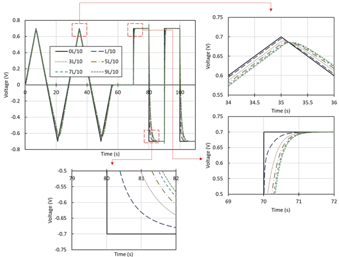
Fig. 18. Modeled voltage drops along the length of the beam due to the existence of electrical resistance of PEDOT electrodes. The black curve is the voltage seen at the fixed end of the cantilever where electrical contact is made. The dashed green line is the predicted voltage as seen at 0.9 of the length, and the others are in between.
