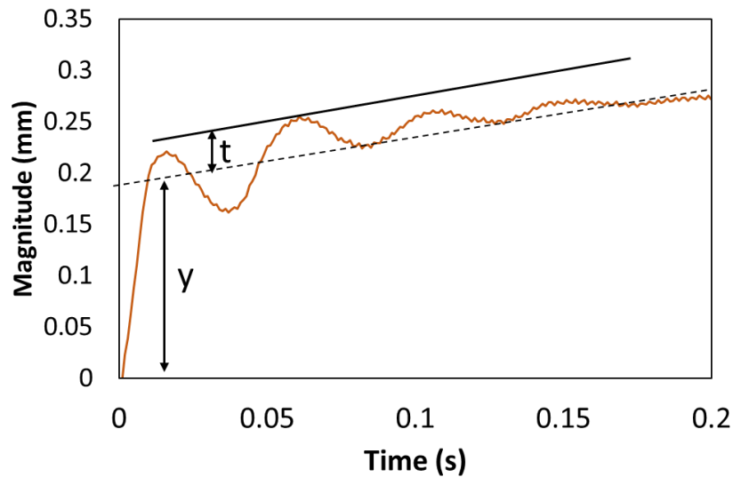
Fig. 13. Beam vibrating as function of time.
