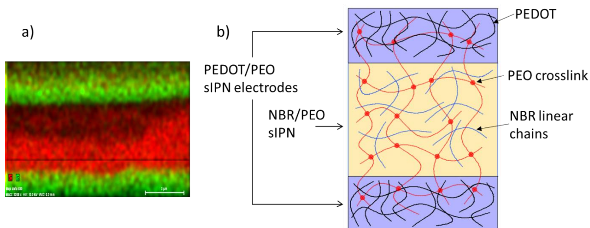
Fig. 17. a) The EDX of the trilayer structure, b) The anticipated morphology of the trilayer structure PEDOT:NBR/PEO:PEDOT
