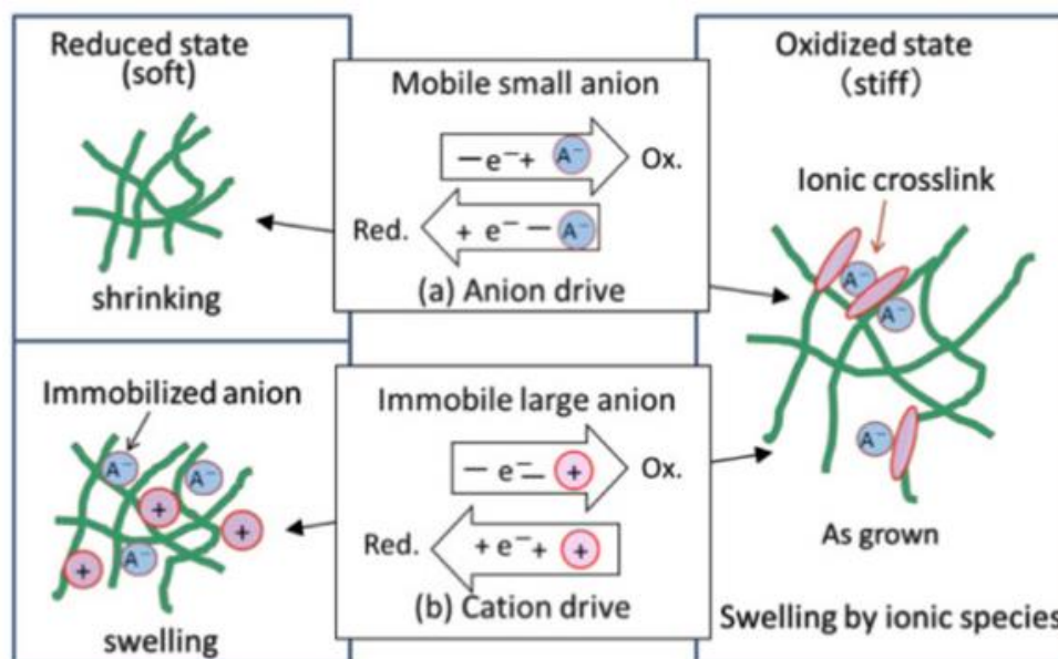
Fig. 1. Actuation mechanism of conducting polymer actuators: a) anion driven mechanism, b) cation driven mechanism [6] (Reprinted with permission from Springer Nature). The ovals represent positive electronic charge on the backbone.
