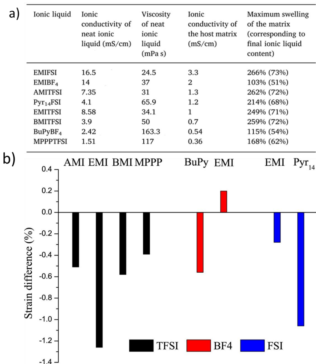
Fig. 8. a) properties of ionic liquids incorporated in NBR/PEO matrix, and b) strain differences calculated for PEDOT-NBR/PEO-PEDOT actuator swollen with different ionic liquids [42] (Reprinted with permission from Elsevier).
