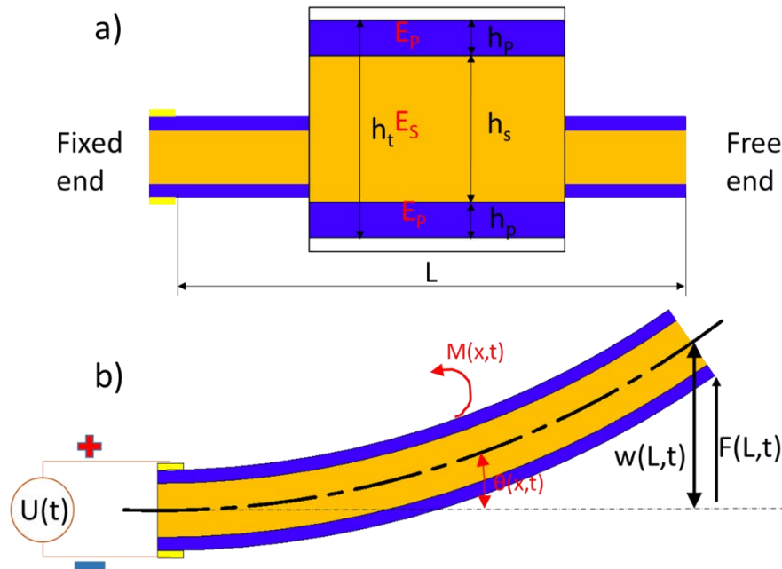
Fig. 2. a) a CP actuator in neutral state and its dimensions (shown in the magnified section in the middle), and b) a voltage excitation induces a tips displacement w(L, t) and an angular rotating angle \theta(x, t) of the actuator, which is equivalent to an external force F(L, t) or a moment M(x, t) , respectively. The Young's moduli of the PEDOT electrodes and the NBR/PEO layer are E_p and E_s , respectively.
