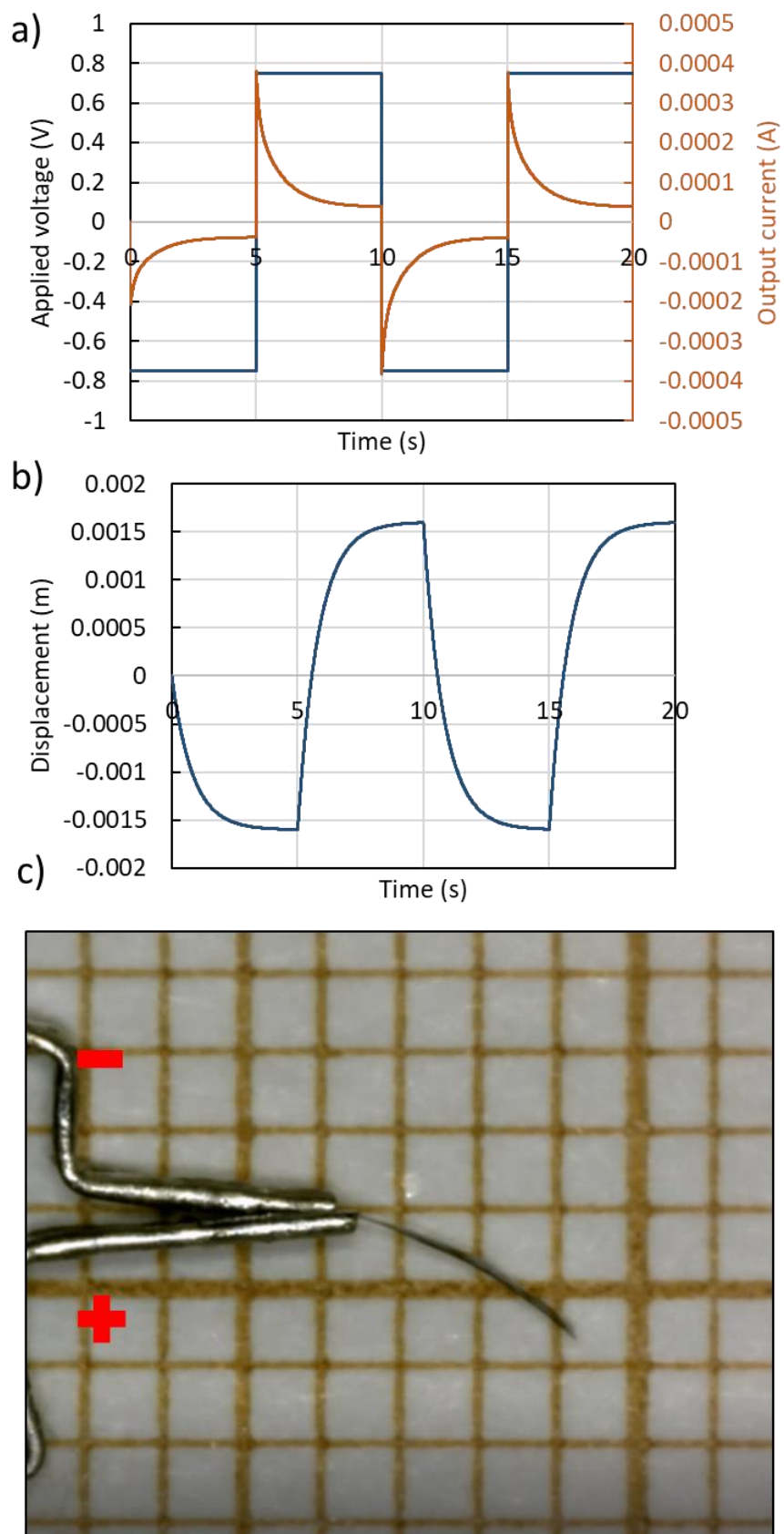
Fig. 1. Actuator behavior under a step voltage a) The applied step voltage and the response current, b) Bending response of the actuator, c) A picture of the bending actuator (length x width x thickness = 4 mm x 1 mm x 0.017 mm), the + and - indicate the polarity of the applied voltage.
