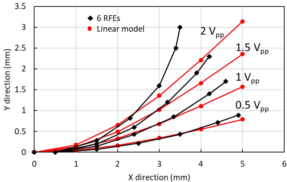
Fig. 15. Comparison between the linear model and the nonlinear model in bending displacement of the actuator in response to the step input voltage with various magnitudes
