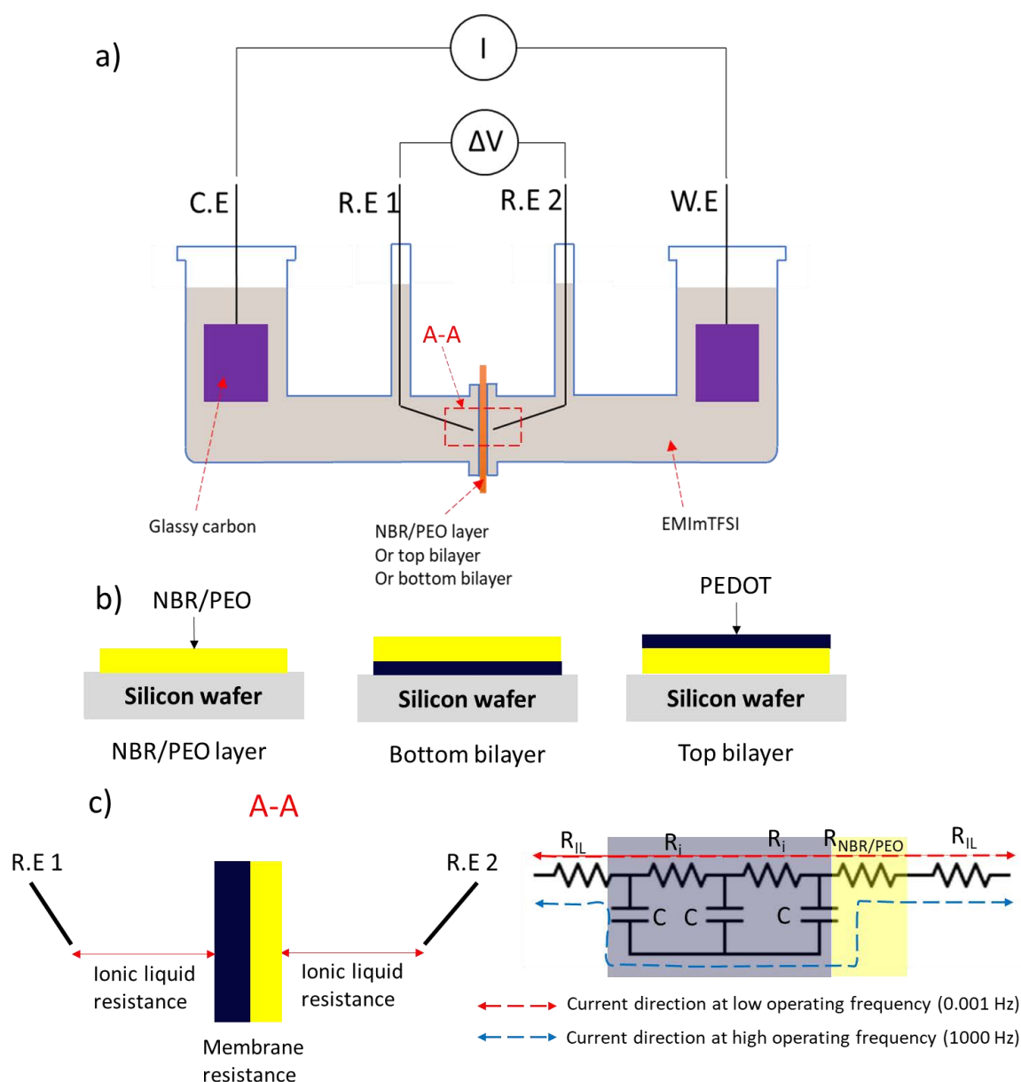
Fig. 2. a) EIS measurement using 4-point setup, b) NBR/PEO layer, bottom bilayer, and top bilayer configuration, and c) a zoomed image of an area in the red rectangular A-A and its equivalent circuit showing the current direction at low and high operating frequency.
