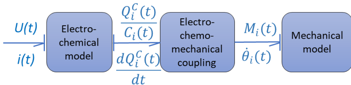
Fig. 3. Trilayer actuator Words BG model.
