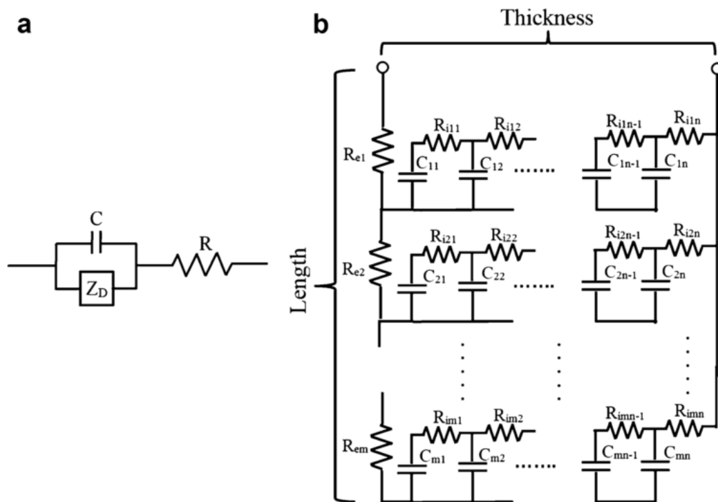
Fig. 1. a) The equivalent electrical circuit of the diffusive elastic model, which includes: a double layer capacitance C , electrolyte resistance R , and the impedance associated with ionic charge transport dominated by diffusivity Z_D , b) Example of an equivalent electrical circuit including a finite diffusion element C_{jk} and R_{ijk} , a resistance R_{ej} , and capacitance at the interface between the solution and the polymer
