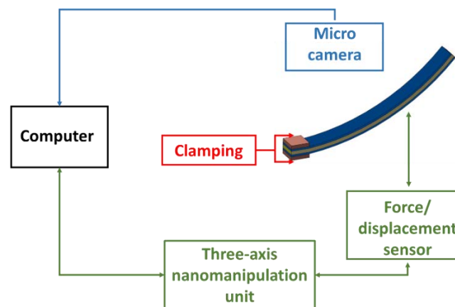
Fig. 8. Experimental setup to measure the decaying of blocking force of the actuator in response to a step displacement
