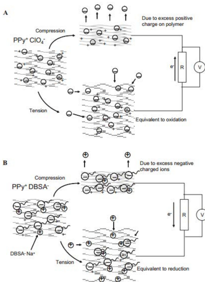
Fig. 3. Schematic diagram illustrating the net ion transport expected in both the “Deformation Induced Ion Flux” model and based on elastic energy considerations [2] (Reprinted with permission from John Wiley and Sons). In the first case compression of the polymer leads to an increase in ion concentration within the polymer, and a net flux of ions out. In the second, it is the compressive stress that squeezes ions out.
