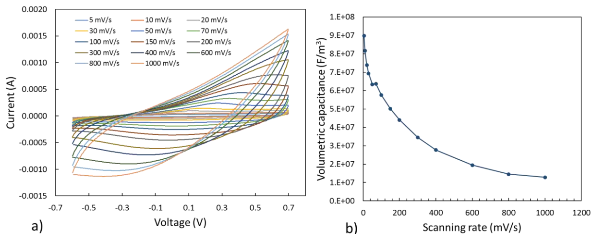
Fig. 7. a) Cyclic voltammograms of PEDOT electrodes obtained in neat EMImTFSI within a potential window of -0.6 V to +0.7 V with different scan rates: b) Volumetric capacitance of PEDOT electrodes as function of the scanning rate.
