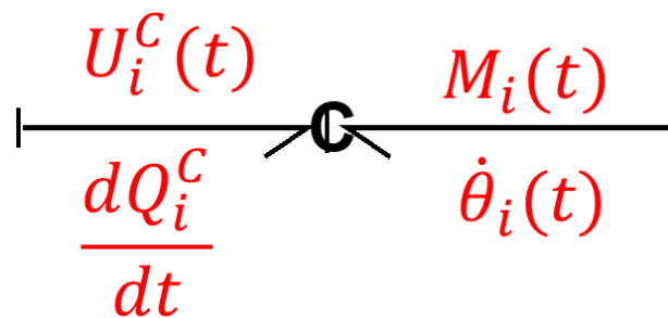
Fig. 6. Coupling between electrical sub-system and mechanical sub-system.
