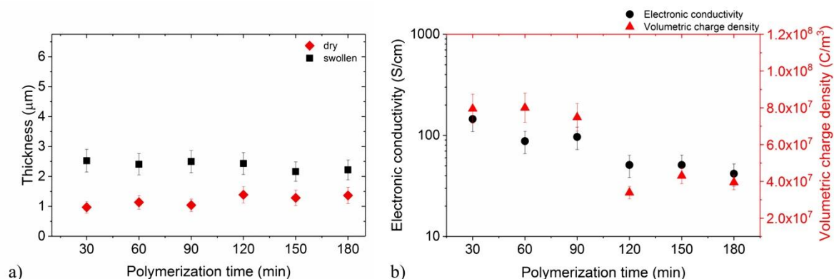
Fig. 3. Effect of EDOT VPP time on PEDOT electrode's thickness (a-■/◆), electronic conductivity (b-●), and volumetric charge density (b-▲). mPEG content: 10 wt%; spin coating speed/acceleration/duration of oxidant solution: 2500 rpm/1000 rpm s -1 /30 s; EDOT VPP temperature: 40 °C.
