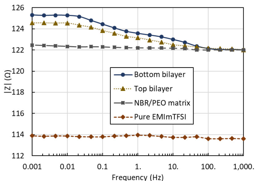
Fig. 3. Impedance values obtained from EIS measurements of a pure EMImTFSI, a top bilayer of NBR/PEO-PEDOT, a bottom bilayer of PEDOT-NBR/PEO, and a single NBR/PEO layer.
