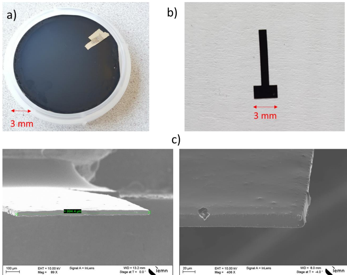
Fig. 16. a) The wafer after drying process, the white trace on the top right indicating the area has been peeled off for characterization: EDX and SEM, b) the resulting trilayer actuator after laser patterning process, the dimensions of the trilayer are length x width = 5 mm x 1 mm c) SEM images of the trilayer after swollen in EMITFSI
