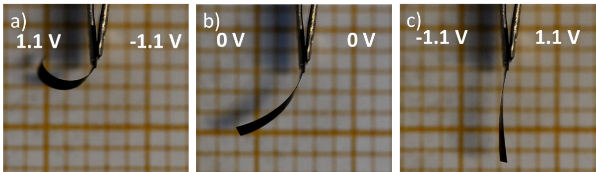
Fig. 16. Trilayer actuator under voltage excitation: a) Top PEDOT electrode voltage: -1.1 \text{ V} , Bottom PEDOT electrode: 1.1 \text{ V} , b) neutral state, c) Top PEDOT electrode: 1.1 \text{ V} , Bottom PEDOT electrode: -1.1 \text{ V} .
