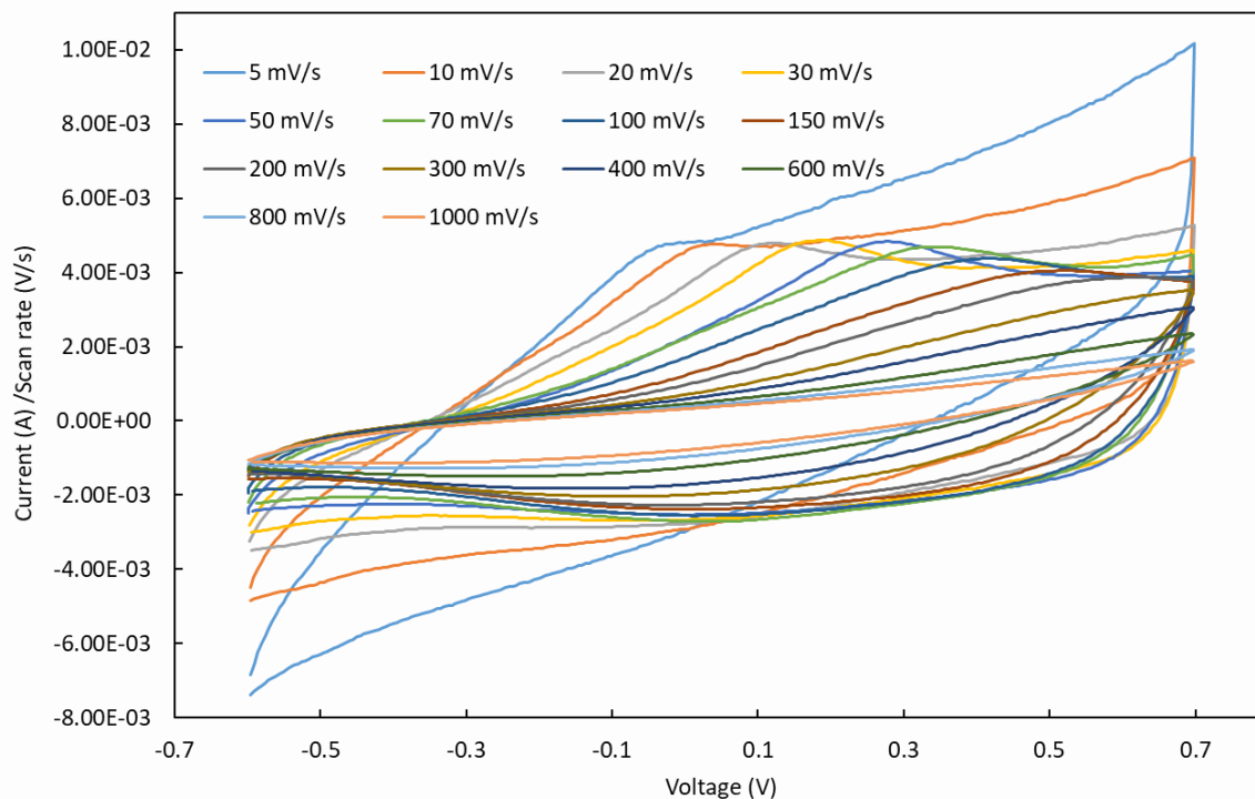
Fig. 6 Cyclic voltammograms of PEDOT electrodes obtained in neat EMImTFSI within a potential window of -0.6 V to +0.7 V with different scan rates. The vertical axis indicates the current (A) scaled by the scanning rate (V/s).
