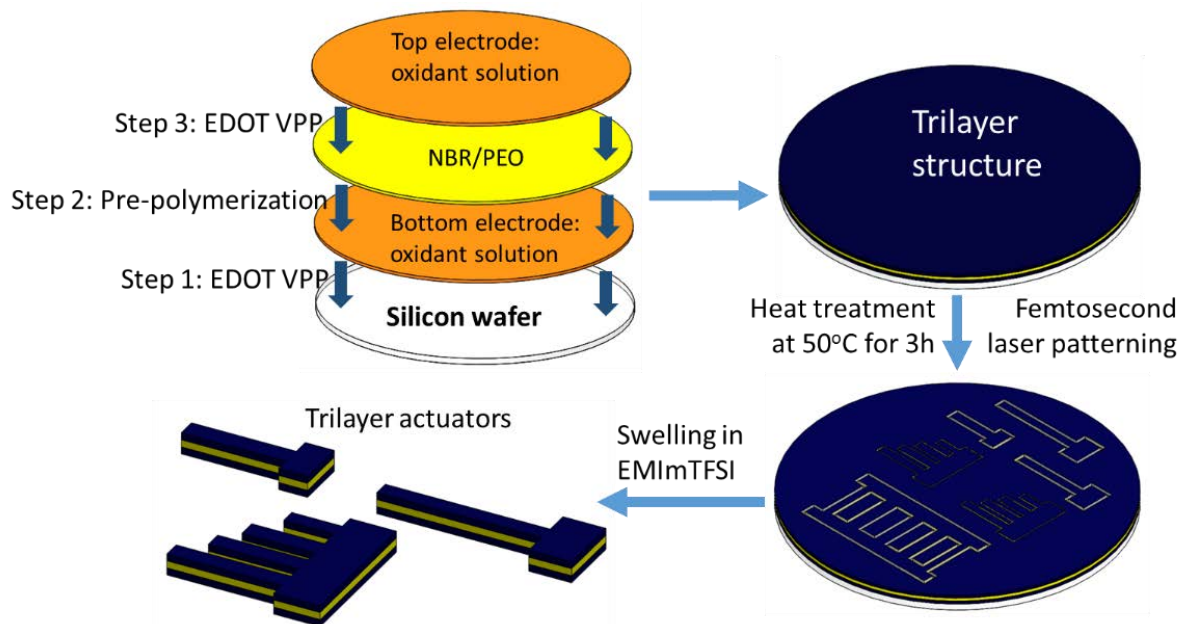
Fig. 13. Microactuator fabrication process showing the multilayer process followed by laser micromachining
