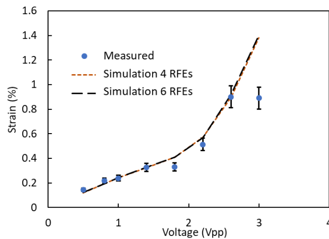
Fig. 19. Comparison between the simulations and the experiments on the strain as a function of the magnitude of applied voltage at a constant frequency of 0.1 Hz
