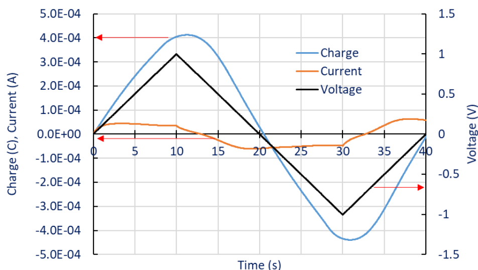
Figure 16. Current and charge response to a triangular input voltage.
