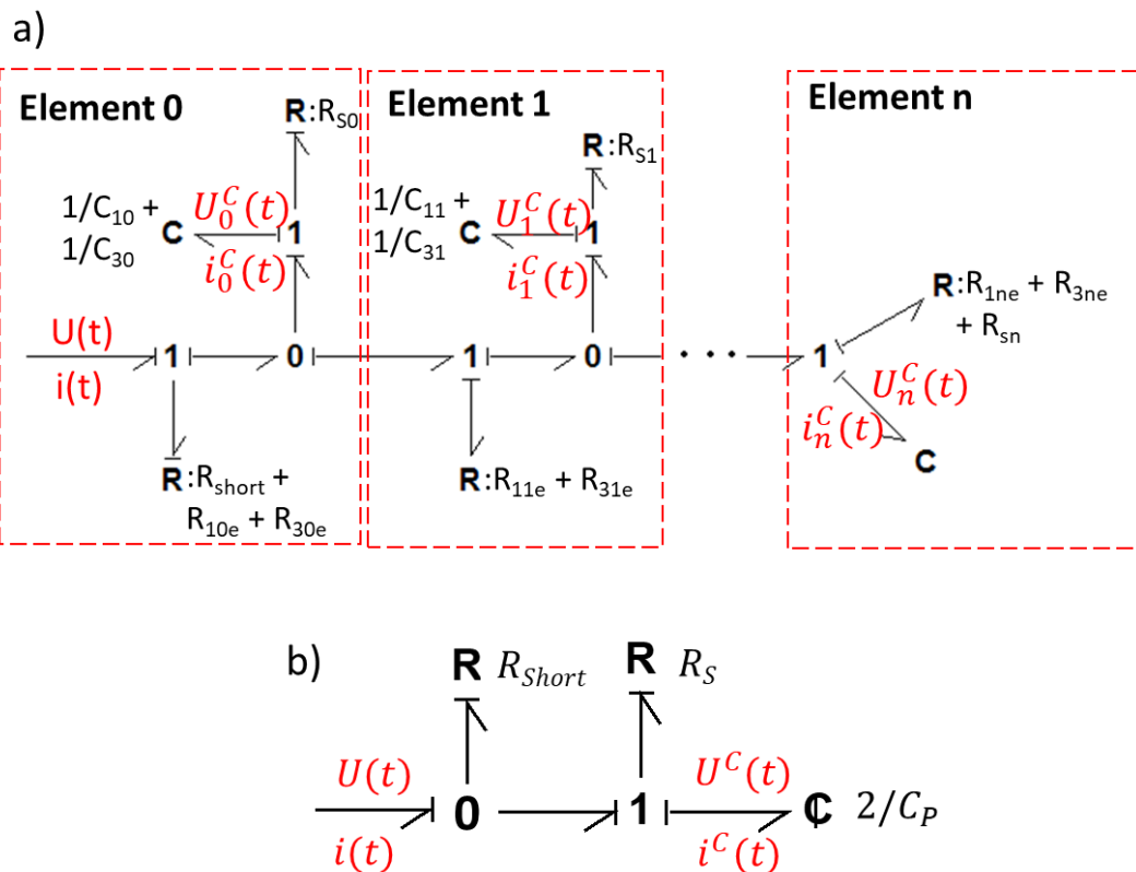
Fig. 5. BG representation of a) the nonlinear electrochemical model, b) the linear electrochemical model.
