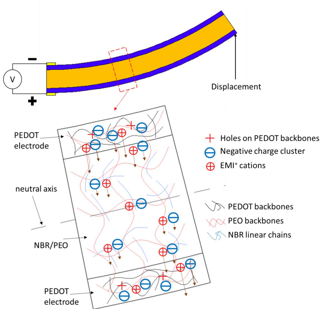
Fig. 8. A qualitative model on sensing mechanism of the trilayer structure: an input displacement causes a flux of cations and anion through the PEDOT electrodes and NBR/PEO layer, the direction of arrows indicates the moving direction while the length of arrows implies the ions velocity
