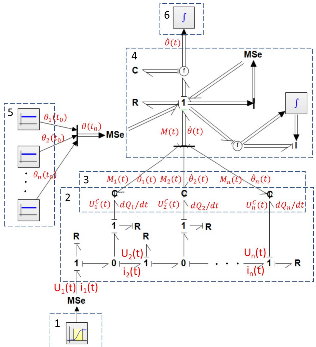
Fig. 11. CP actuator global model: 1. Voltage source, 2. Electrochemical model, 3. Coupling between electrochemical and mechanical part, 4. Mechanical model, 5. Boundary conditions: initial stress, 6. Displacement output.
