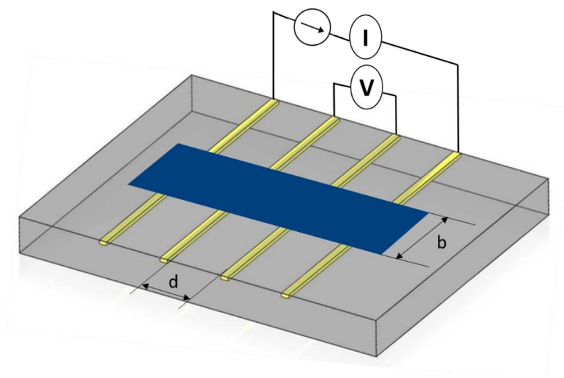
Fig. 5. A built in-house four-line probe to measure the electronic conductivity of the PEDOT electrodes, where the distance between two copper lines is d = 2 \text{ mm} .
