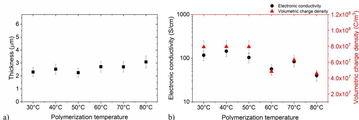
Fig. 4. Influence of EDOT VPP temperature on PEDOT electrode's thickness (a-■), electronic conductivity (b-●), and volumetric charge density (b-▲). mPEG content: 10 wt%; spin coating speed/acceleration/duration of oxidant solution: 2500rpm/1000rpm s -1 /30s; EDOT VPP time: 30 min.
