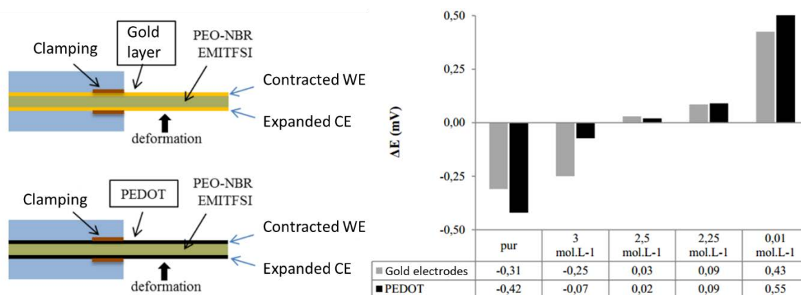
Fig. 5. Schematic experiments and comparison of output voltage in two different trilayer configurations: Gold-NBR/PEO-Gold, and PEDOT-NBR/PEO-PEDOT with the dimension of L = 15\text{mm} , b = 5\text{mm} , h_t = 0.17\text{ mm} at various EMITFSI-PC concentrations, under a 2% applied strain [11] (Retrieved from https://tel.archives-ouvertes.fr/tel-01413677 . By permission from author.). In this case a positive voltage suggests anion motion.
