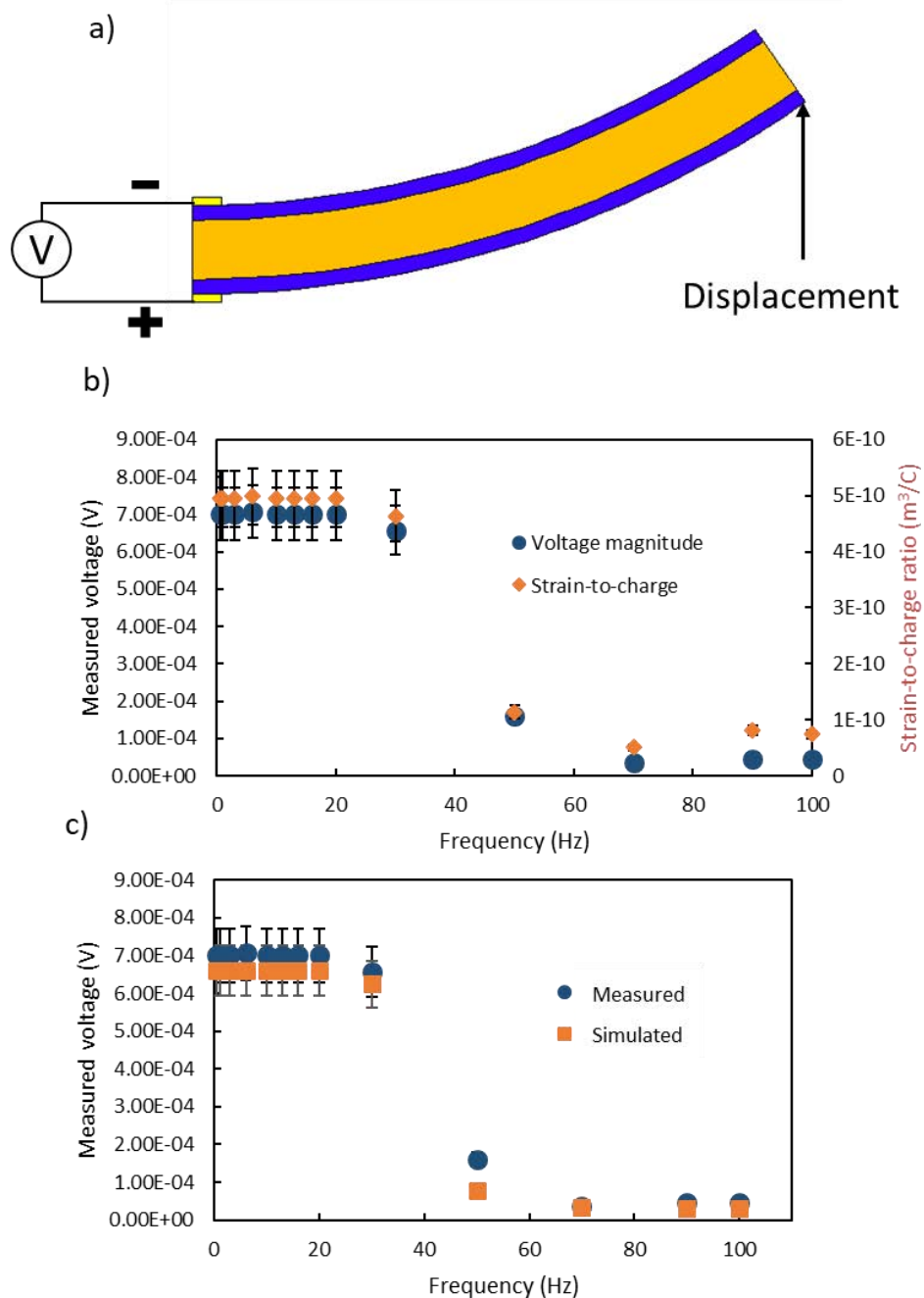
Fig. 9. a) Schematic of a trilayer transducer under a displacement excitation and the produced voltage polarity b) Voltage magnitude and the strain-to-charge ratio as a function of frequency when the magnitude of the sinusoidal displacement is constant at 2mm, c) Comparison between the simulation and the experiment of the magnitude of output voltage
