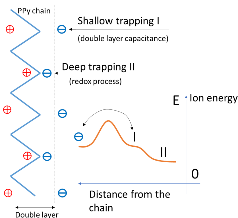
Fig. 4. A possible model taking into account two electrochemical doping process: some ions (II), deeply trapped near the polymer chains are released at only very low potentials. Other ions (I) are shallowly trapped, they form a double layer at a certain distance from the chain. (Reproduced with permission from [10], The Electrochemical Society.)
