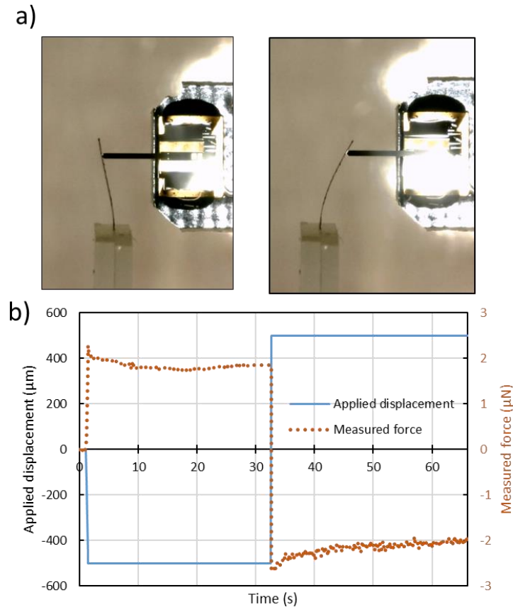
Fig. 12. a) Experiment of applying step displacement, and b) The decay of force response of the beam as a function of time.
