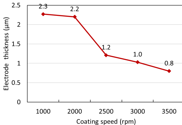
Fig. 12. Relation between the rotational speed of the spin-coater for deposition of the oxidant solution on a silicon wafer and the thickness of the PEDOT electrode, where the mPEG content is 10% of oxidant solution
