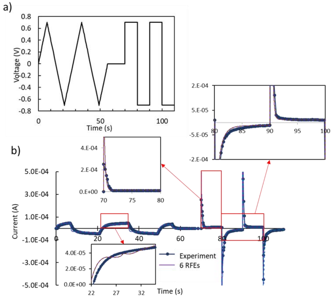
Fig. 17. a) Triangular wave and rectangular wave applied voltage, b) Measured and simulation current response
