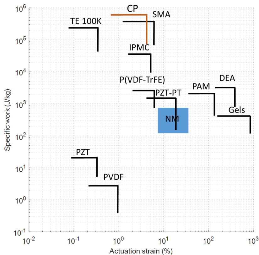
Fig. 2. Dependence of specific work on actuation strain for various artificial muscles.
