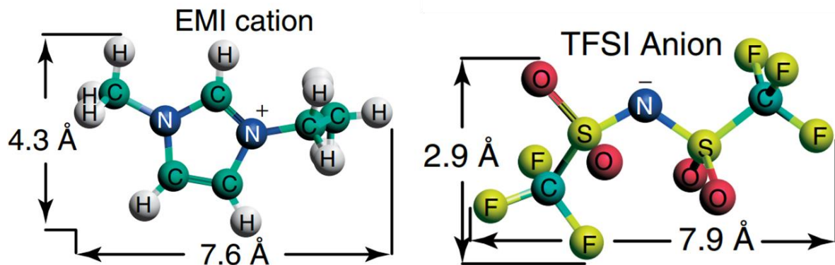
Fig. 7. 3D molecular structure and size of EMI cation and TFSI anion (Adapted with permission from Ref. [14]. American Chemical Society, 2008.)
