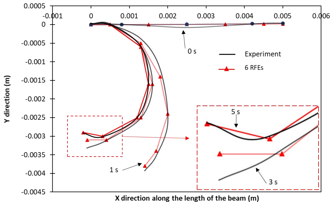
Fig. 21. Comparison between the experiment and the simulation in terms of the dynamic mechanical behavior of the beam subjected to a voltage excitation of 2.2 V pp at 0.1 Hz.
