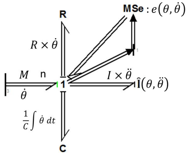
Fig. 9. Mechanical BG model.
