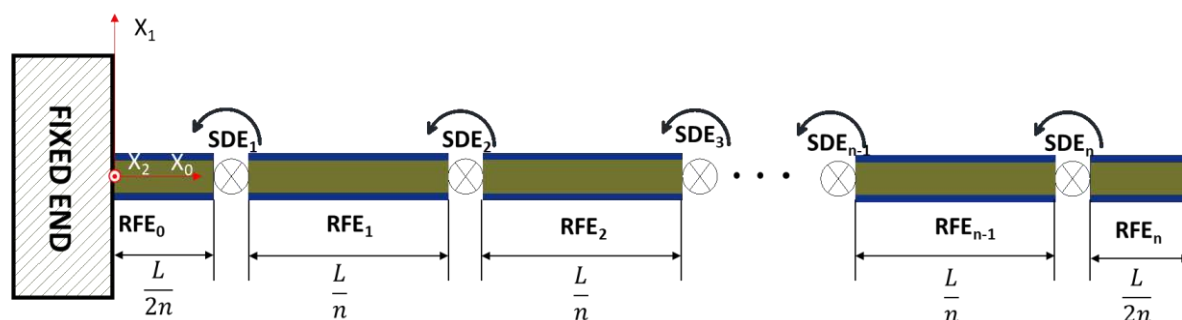
Fig. 7. Rigid Finite Element Model (RFEM) of a trilayer actuator, in which it is divided into (n+1) rigid elements: from RFE_0 to RFE_n , the elements each have a mass and are linked by a spring-damper element SDE_1 to SDE_n , shown in their initial positions. The integrated coordinator includes X_0 axis along the length of the actuator, X_1 axis perpendicular to the X_0 and X_2 axis perpendicular to the X_0X_1 surface.
