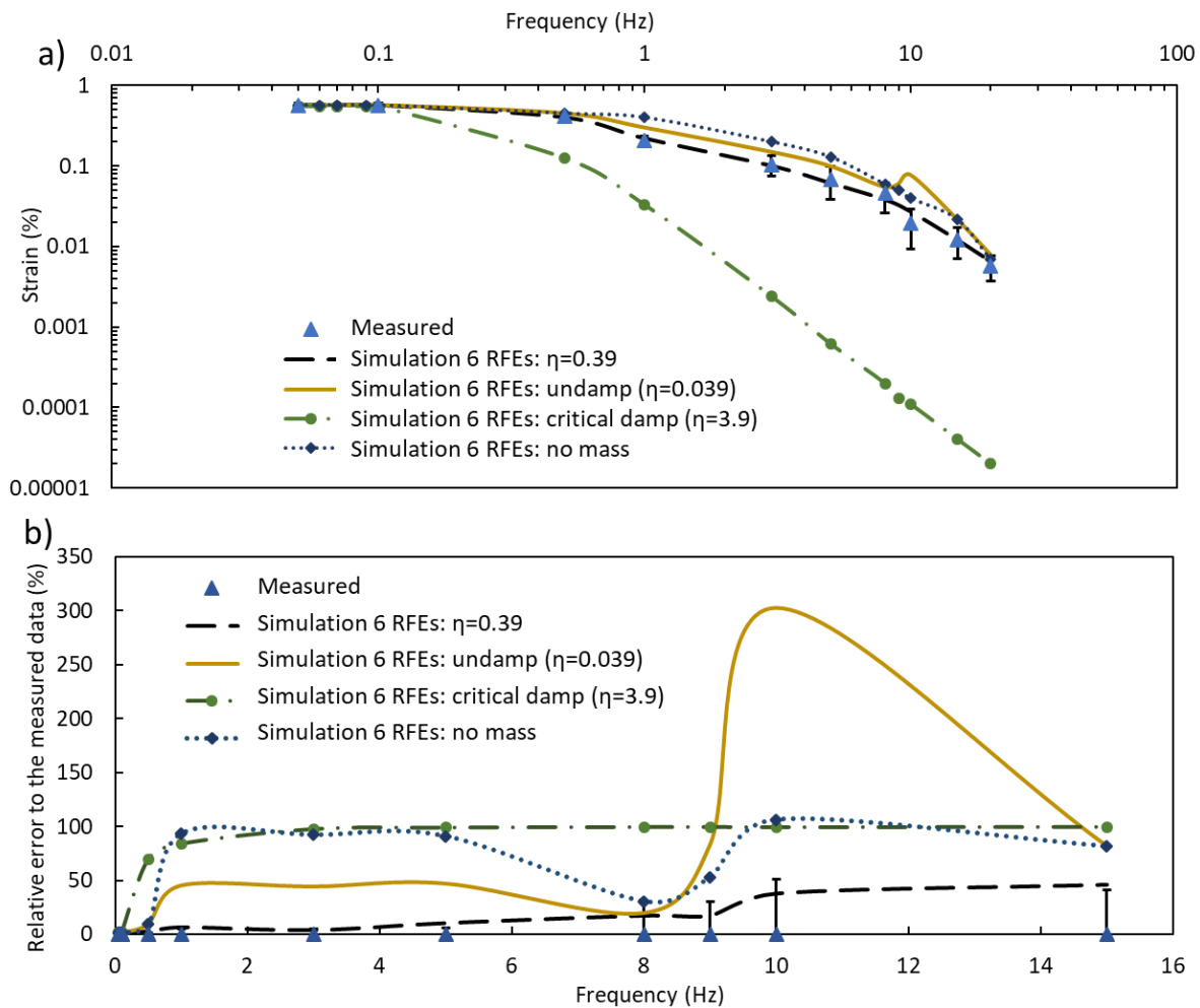
Fig. 20. a) Comparison between the simulations and the experiments on the strain as a function of the frequency of applied voltage at a constant magnitude of \pm 1.1 V, b) The relative error of the simulations compared to the measured data.
