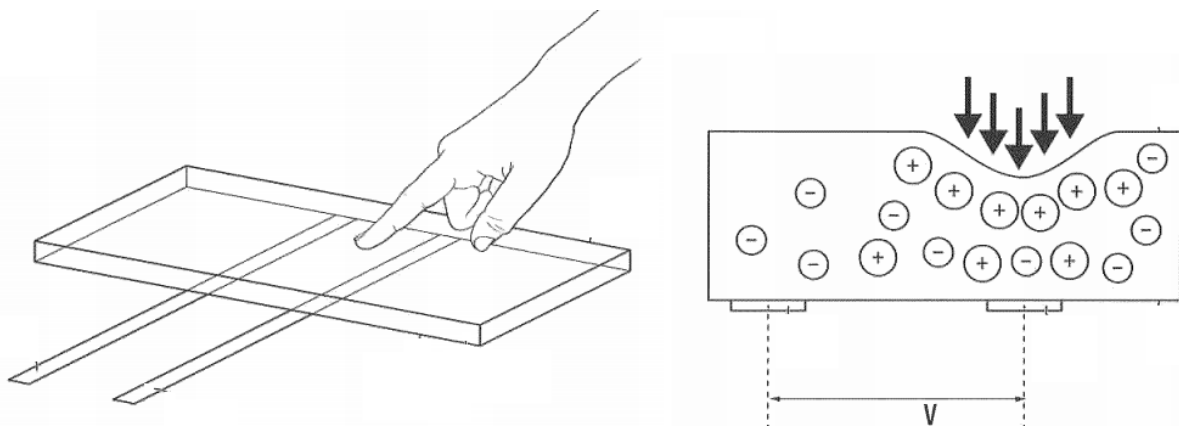
Fig. 4. Experimental scheme and induced voltage mechanism of a thin ionic conducting polymer film under an applied stress [10]
