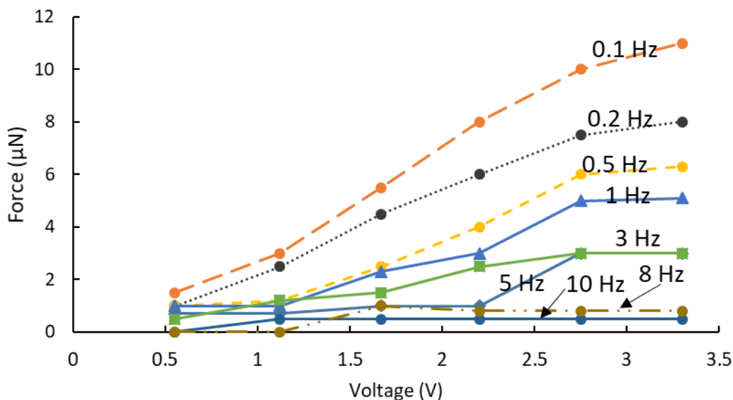
Fig. 14. Force generated as a function of the magnitude and the frequency of the applied voltage from a trilayer actuator of length x width x thickness: 6 mm x 1 mm x 0.017 mm.
