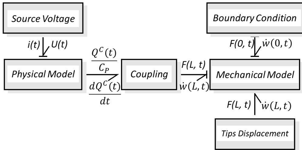
Fig. 12. Linear BG global model of CP actuators, where a source of voltage is employed as the input and the tips displacement of the beam is the output of the model.
