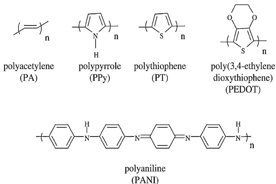
Fig. 3. Chemical structures of some typical conducting polymers.
