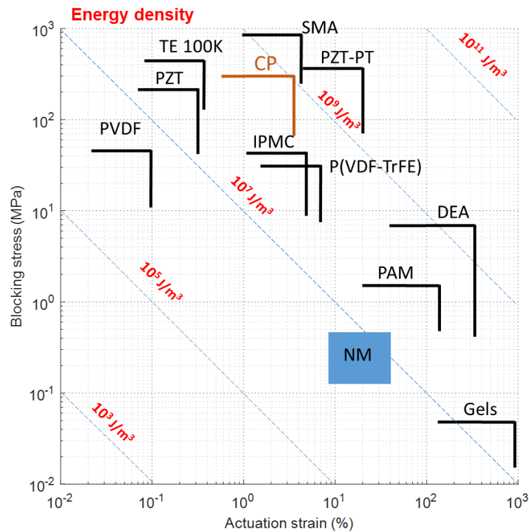
Fig. 1. Dependence of blocking stress on actuation strain for various artificial muscles. Abbreviations: PVDF - piezoelectric polymer [32], PZT - piezoelectric ceramic [33], TE 100K - Thermal expansion actuators 100K [34], SMA - shape memory alloy [35], CP - conducting polymer [36], IPMC - ionic polymer metal composite [37], PZT-PT - piezoelectric single crystal [33], P(VDF-TrFE) - relaxor ferroelectric polymer [38], DEA - dielectric elastomer [35], PAM - pneumatic artificial muscle [19], Gels - Gel actuators [39], NM - natural muscle [1].
