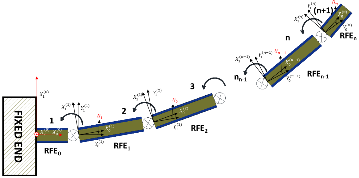
Fig. 8. Trilayer actuator in a bent state. The bending angle between the element (i-1) and the element i is \theta_i .
