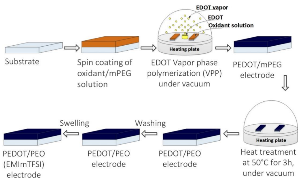
Fig. 11. Fabrication process of PEDOT electrodes [51]
