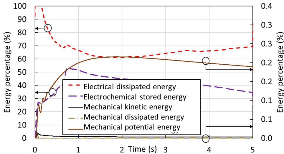
Fig. 24. Instantaneous electrical to mechanical coupling.
