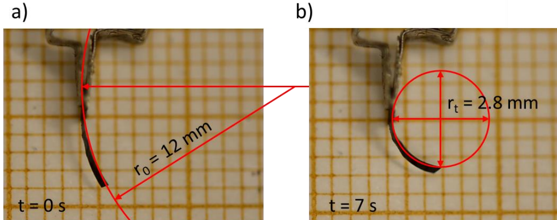
Fig. 15. Actuator at the a) neutral state where the bending radius is equal r_0 = 12 mm, and b) excited state where the bending radius is r_t = 2.8 mm. The orange square on the background of the pictures has the dimension of 1 \times 1 mm.
