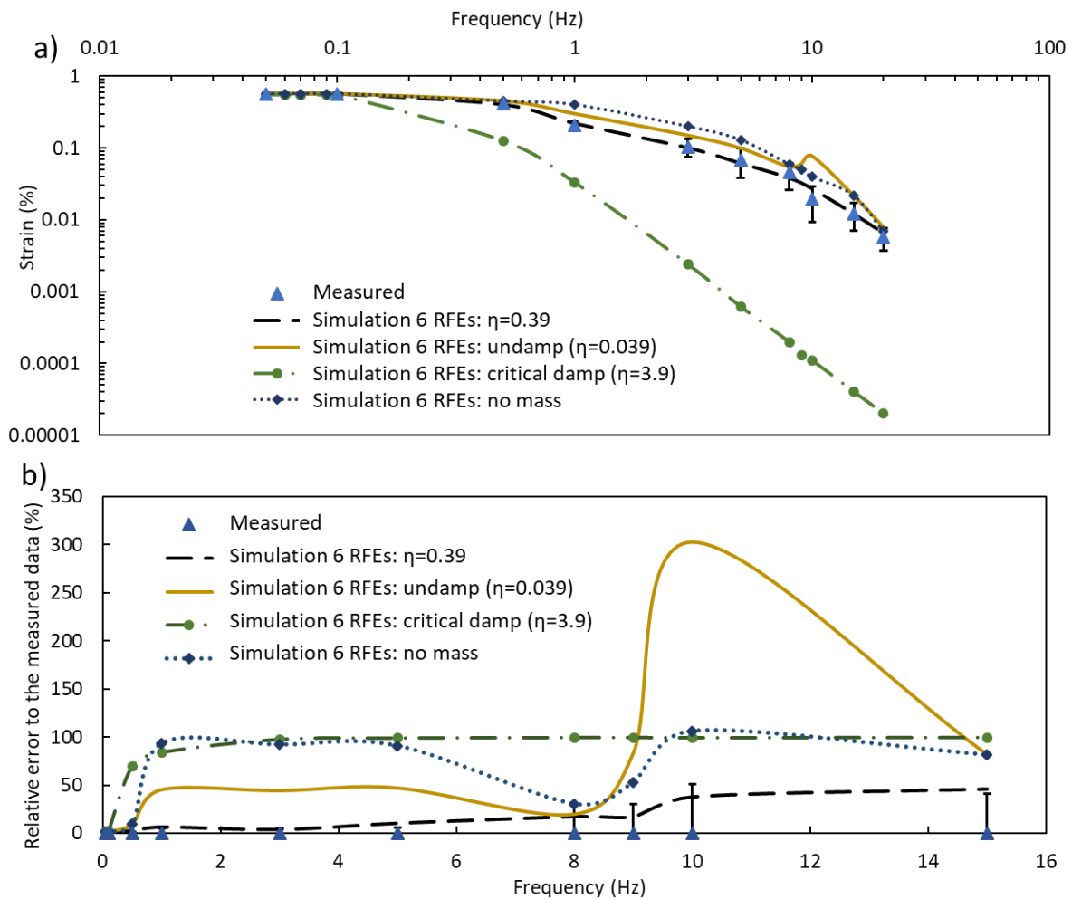
Fig. 20. a) Comparison between the simulations and the experiments on the strain as a function of the frequency of applied voltage at a constant magnitude of \pm 1.1 V, b) The relative error of the simulations compared to the measured data.
