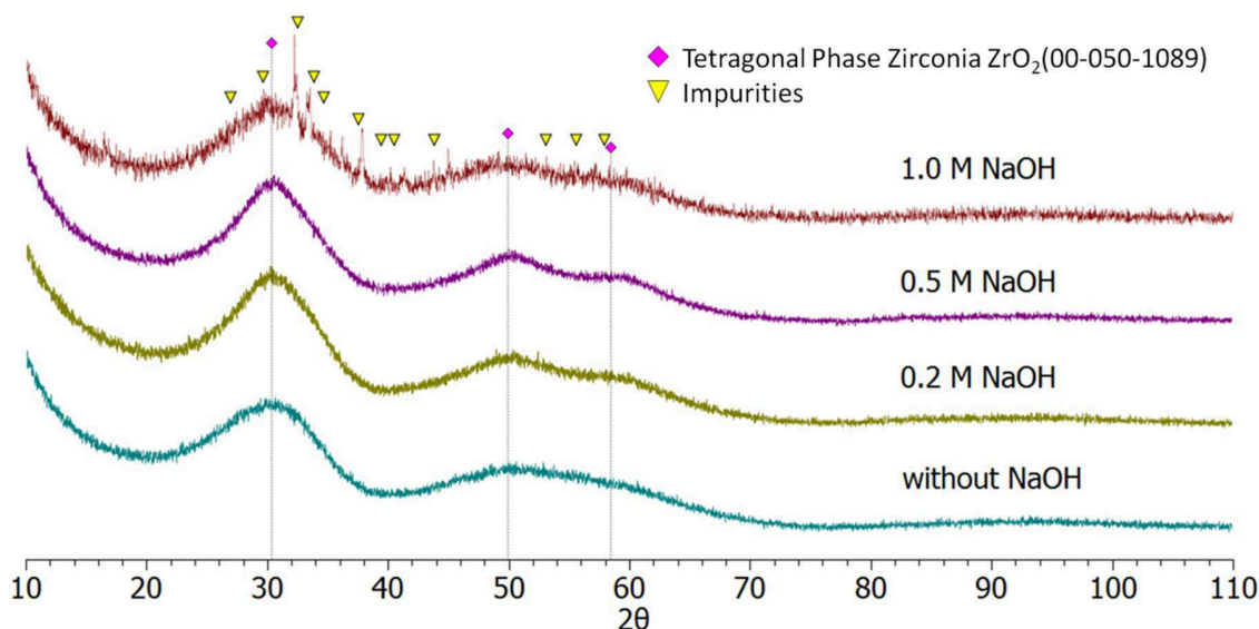
Figure 79: XRD patterns of samples obtained via a solvothermal technique at 210°C for 3 days using [Zr(O^iPr)_4 \cdot HO^iPr]_2 and anisole under varied amounts of NaOH (0.0, 0.2, 0.5, and 1.0 mol.L -1 )
