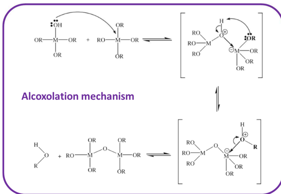
Figure 13: Oxolation and alcoxolation mechanisms for condensation step.
