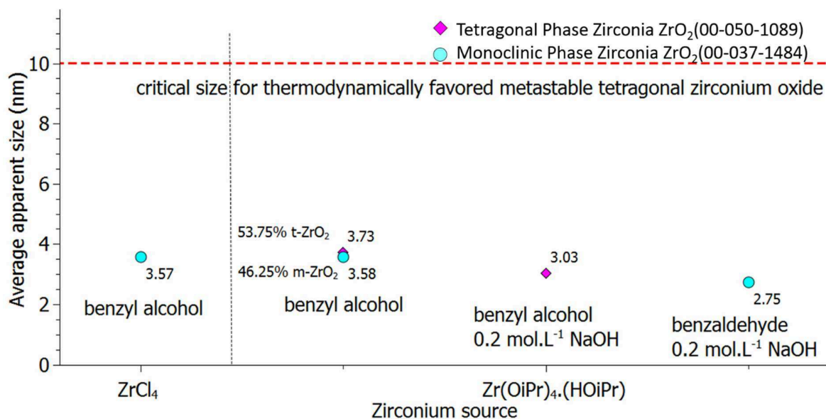
Figure 72: Average apparent size of the zirconia particles obtained using zirconium chloride ( ZrCl_4 ) precursor and zirconium isopropoxide-isopropanol adduct [Zr(O^iPr)_4 \cdot HO^iPr]_2 with or without the presence of sodium hydroxide under varied solvents prepared using solvothermal technique at 150^\circ C and 210^\circ C for 3 days.
