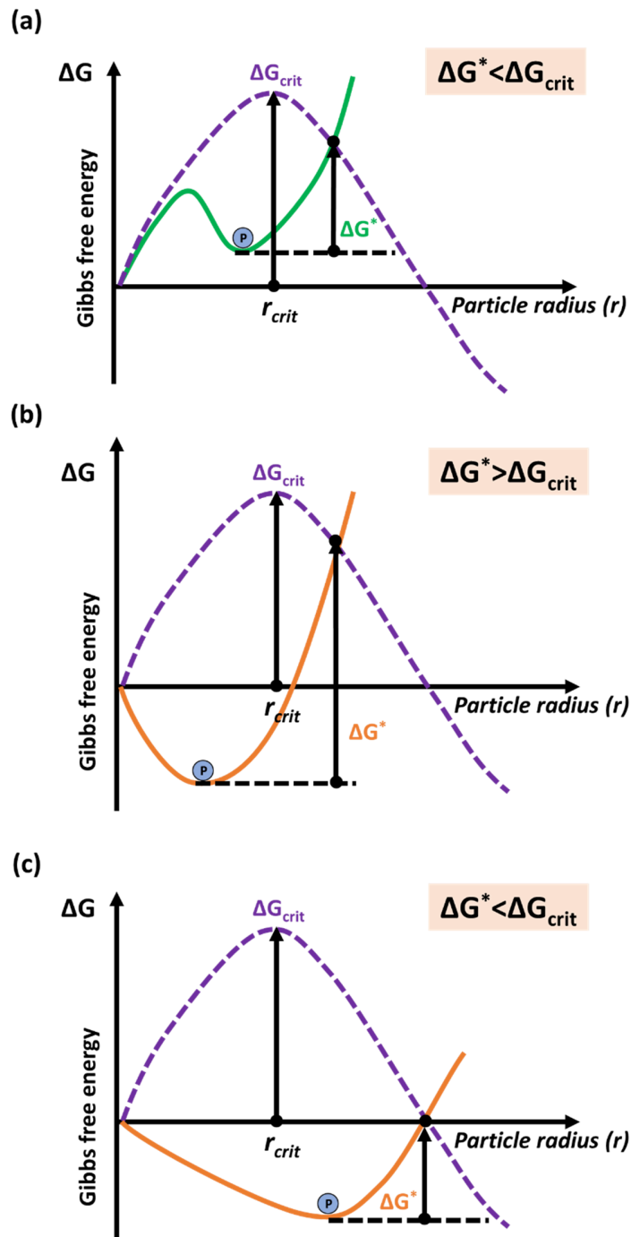
Figure 36: Thermodynamical rationale for (a) metastable and subcritical prenucleation cluster as relatively favorable intermediates to crystal nucleation, (b) small and stable cluster exhibiting a considerable increase in the energy barrier for the cluster-to-nucleus transition and favoring nucleation from bulk solution, (c) large and stable prenucleation clusters as a favorable building blocks to crystal formation.
