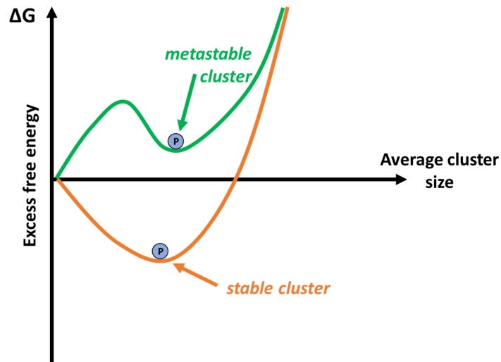
Figure 35: Excess free energy profile relative to the free ions in solution and normalized to the bulk surface energy for metastable and stable prenucleation cluster as a function of the average cluster size.
