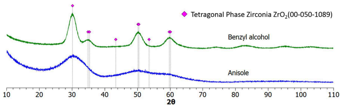
Figure 83: XRD diagrams of the samples obtained via a solvothermal technique at 210°C for 3 days using [Zr(O^iPr)_4 \cdot HO^iPr]_2 with 0.2 mol.L -1 NaOH in (a) benzyl alcohol and (b) anisole.
