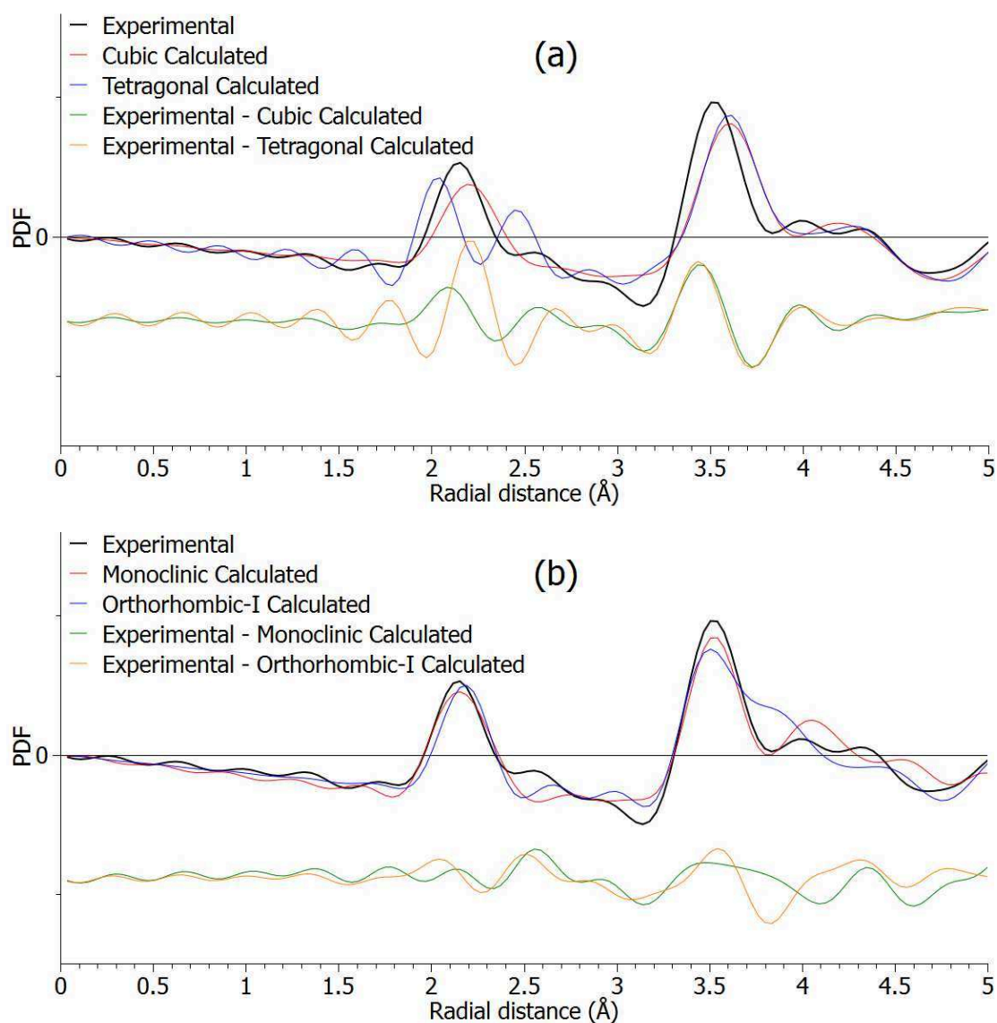
Figure 98: Experimental PDF of the zirconia particles produced at 210°C for three days in benzyl alcohol with 0.2 mol.L -1 NaOH compared with a refined (a) cubic and tetragonal and (b) monoclinic and orthorhombic I models within the range of 0 to 5 Å.
