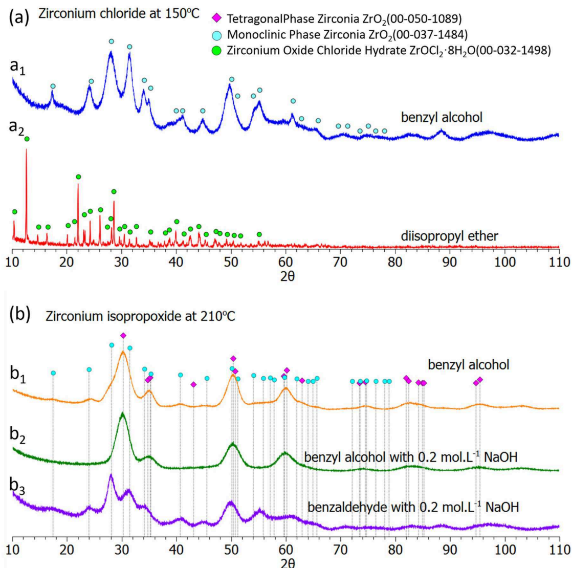
Figure 71: XRD patterns of samples obtained using ZrCl_4 precursor (a) and [Zr(O^iPr)_4 \cdot HO^iPr]_2 (b) under varied solvents coupled or not with the presence of sodium hydroxide and solvothermal technique for 3 days at 150^\circ C (a) or 210^\circ C (b).
