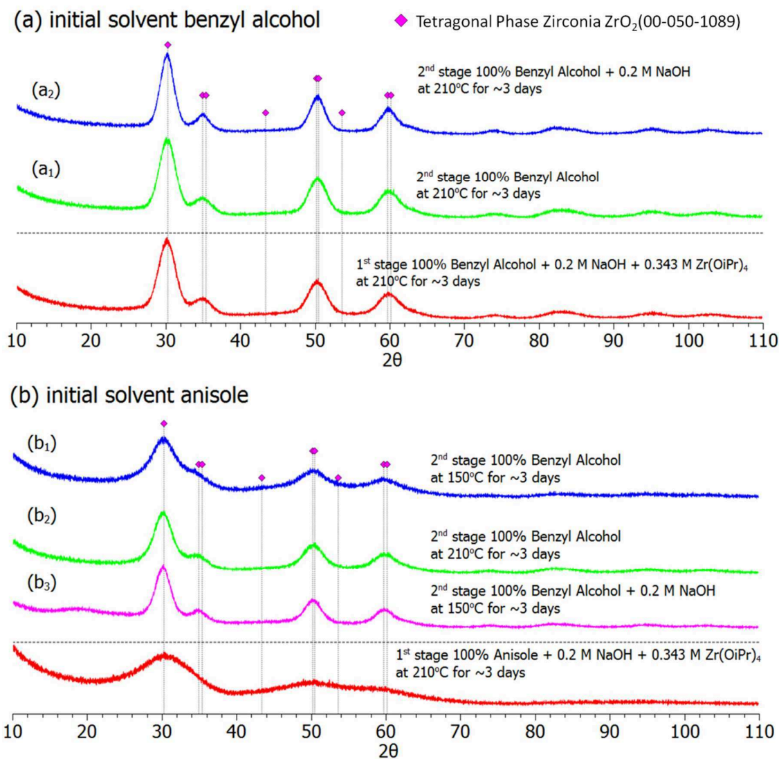
Figure 81: XRD patterns of samples prepared by dual stage synthesis using [Zr(O^iPr)_4 \cdot HO^iPr]_2 with 0.2 \text{ mol.L}^{-1} NaOH in (a) benzyl alcohol and (b) anisole at 210°C for 3 days for the first step and then, secondly in benzyl alcohol with or without 0.2 \text{ mol.L}^{-1} NaOH for the second step.
