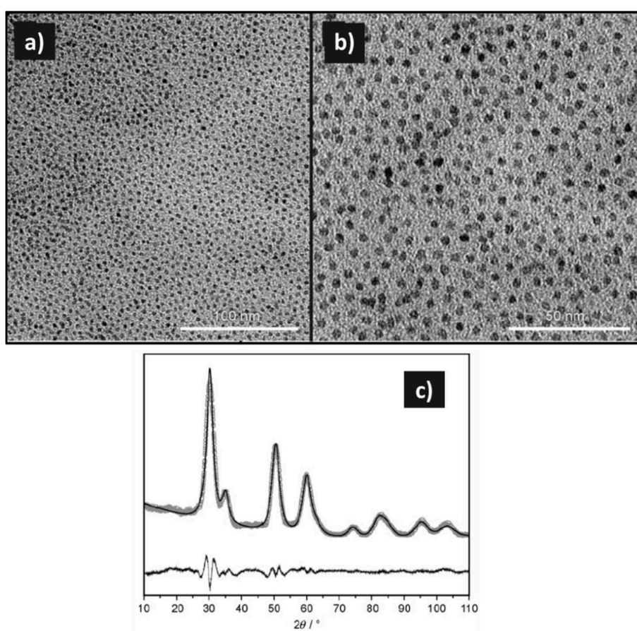
Figure 25: TEM images of ZrO 2 nanoparticles after post-functionalization with octadecanoic acid (a-b) and XRD diffraction pattern of as-prepared ZrO 2 nanoparticles (c) according to Garnweitner et al.
