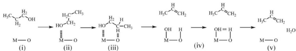
Figure 75: Schematic representation of the concerted E_2 elimination dehydration reaction involving surface oxygen (a) of the oxides. The steps are: alcohol adsorption on the Lewis acid site \text{M} ((i) \rightarrow (ii)), \beta -hydrogen transfer to a surface \text{O} (a (iii)), alkene formation and desorption (iv), water formation, desorption and catalyst regeneration (iv) \rightarrow (v).
