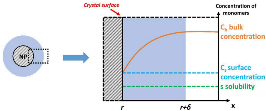
Figure 38: Schematic illustration of diffusion layer ( \delta ) near the surface of a nanocrystal (left) and plot of the monomer concentration as a function of the distance x (right) according Kwon et al. [65].
