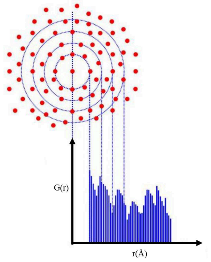
Figure 68: Scheme representing the pair distribution function G(r) .
