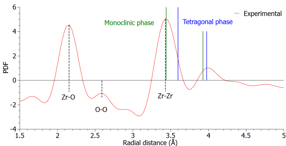
Figure 111: Experimental PDF of the zirconia particles produced at 210°C for three days in anisole compared with well crystallized zirconia tetragonal phase [88] and monoclinic phase [87].
