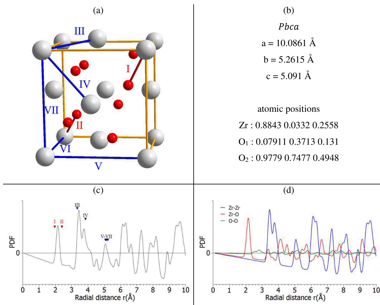
Figure 92: Structural model of the orthorhombic I phase zirconia (a) balls and stick representation, (b) parameter details of the phase [90], (c) PDF analysis of the phase and (d) interatomic distances of the model.
