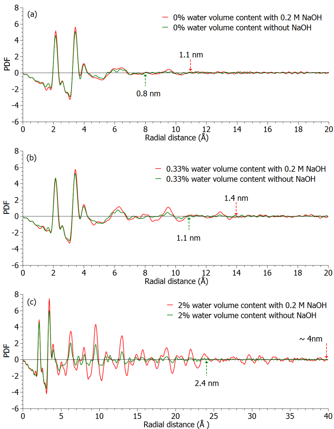
Figure 140: (a) Experimental PDF of the zirconia particles produced at 210°C in anisole without and with 0.2 mol.L -1 NaOH for (a) 0% water volume content, (b) 0.33% water volume content, and (c) 2% water volume content.
