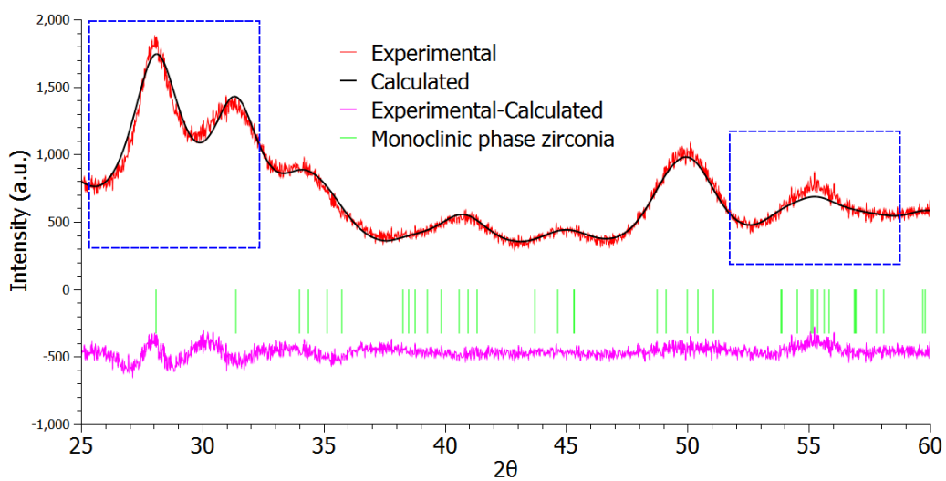
Figure 100: Rietveld refinement of the XRD diagram of the \text{ZrO}_2 sample examined at closer range.
