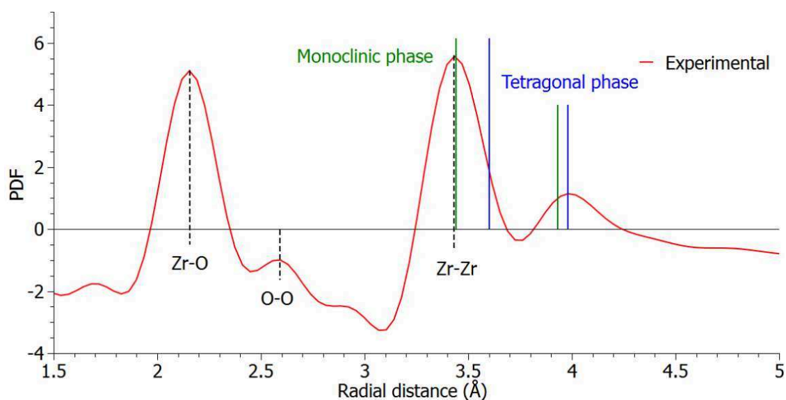
Figure 107: Experimental PDF of the zirconia particles produced at 210°C for three days in anisole with 0.2 mol.L -1 NaOH compared with well crystallized zirconia tetragonal phase [88] and monoclinic phase [87].
