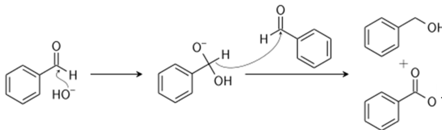
Figure 70: Chemical equation for the disproportionation of benzaldehyde in alkaline medium namely Cannizzaro reaction.
