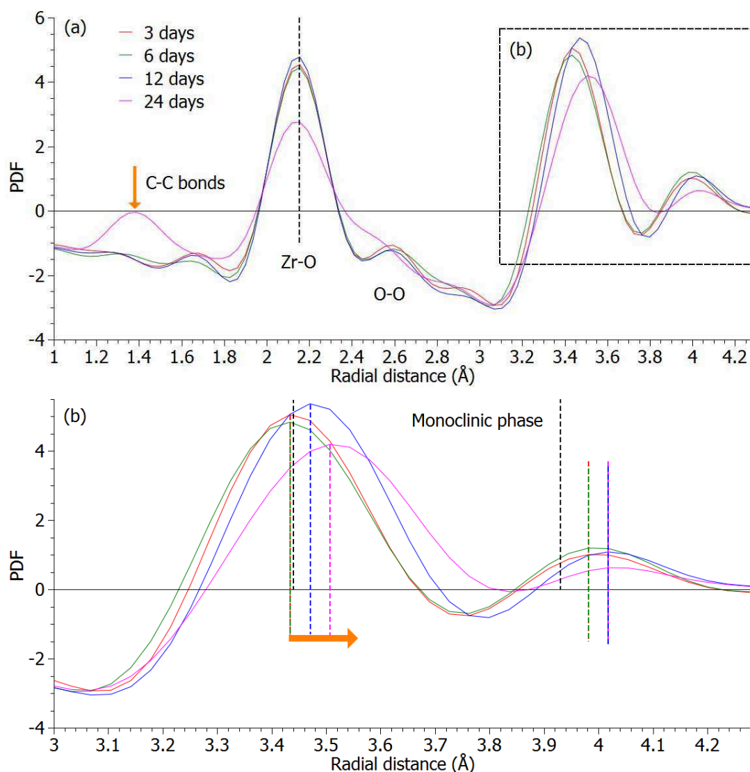
Figure 120: Experimental PDF of the zirconia particles for varied solvothermal ageing period prepared at 210°C in anisole without NaOH compared with well crystallized zirconia monoclinic phase [87].
