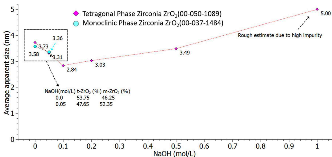
Figure 74: Average apparent size of the samples obtained via a solvothermal technique at 210°C for 3 days using [Zr(O i Pr) 4 ·HO i Pr] 2 in benzyl alcohol with different amounts of NaOH.
