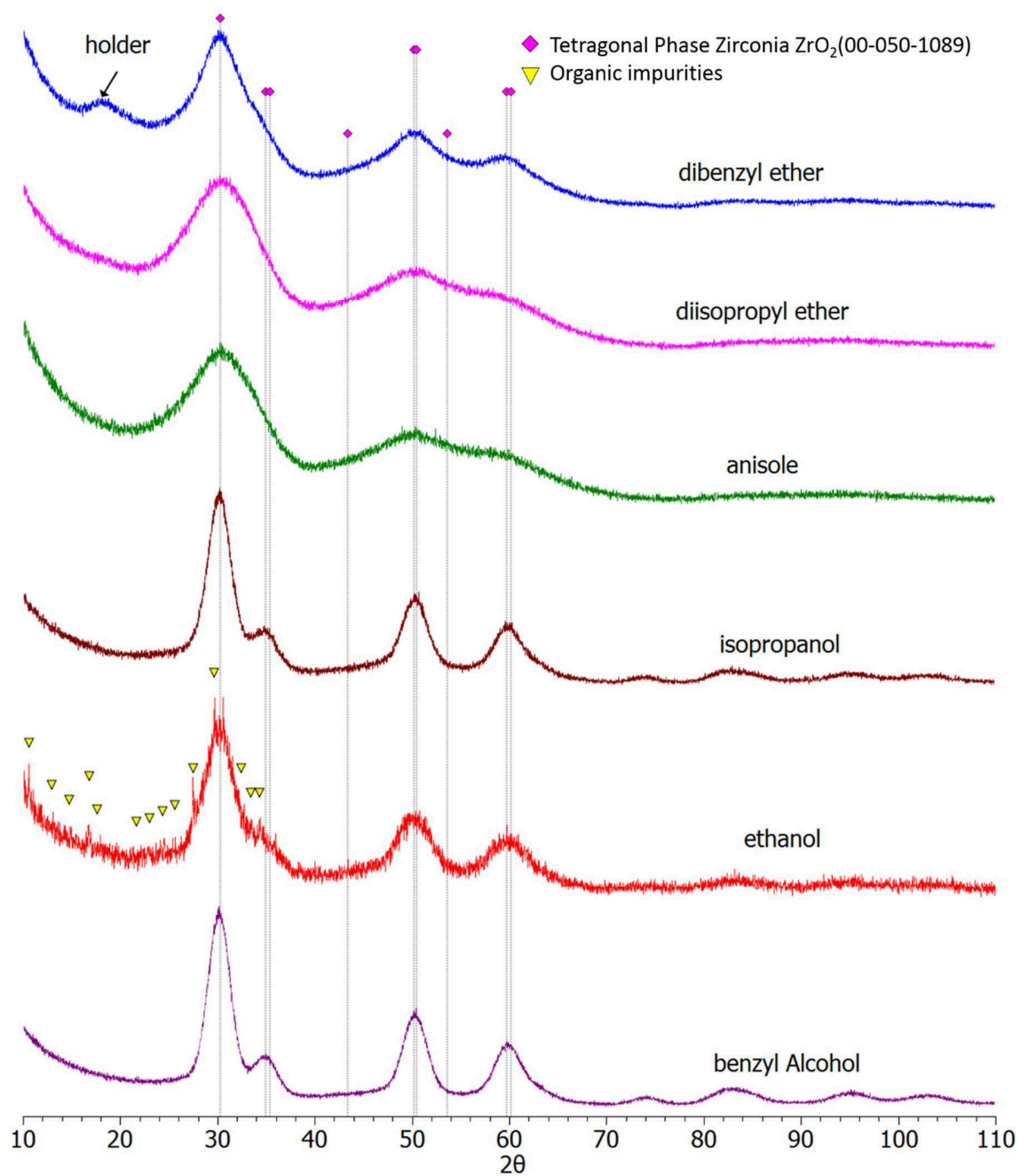
Figure 151: XRD patterns of zirconia samples prepared via a solvothermal technique at 210°C for 3 days using [Zr(O^iPr)_4 \cdot HO^iPr]_2 and 0.2 \text{ mol.L}^{-1} NaOH under various solvents.
