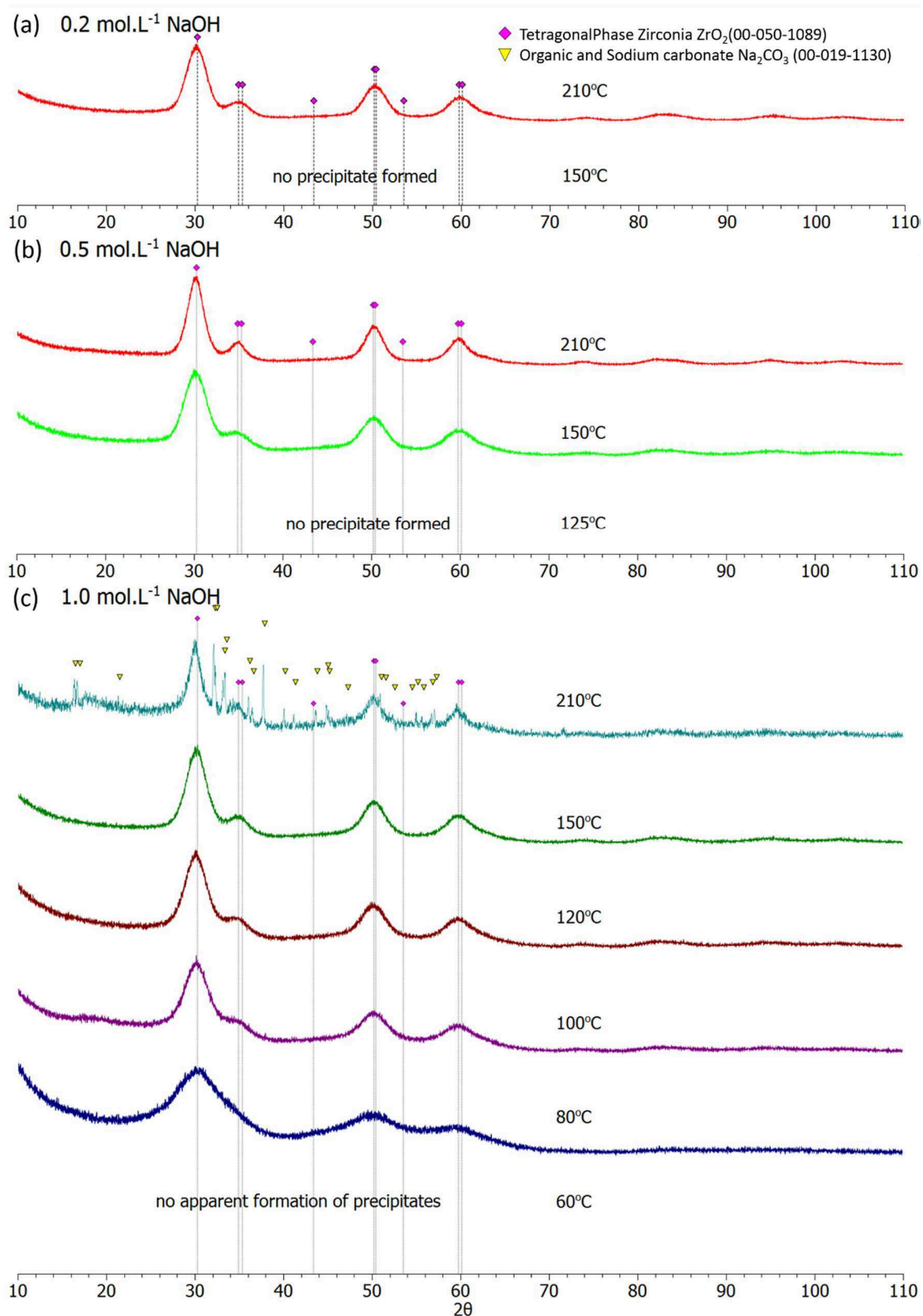
Figure 76: XRD patterns of samples obtained via a solvothermal technique under varied synthesis temperature for 3 days using [\text{Zr}(\text{O}^i\text{Pr})_4 \cdot \text{HO}^i\text{Pr}]_2 in benzyl alcohol with (a) 0.2, (b) 0.5 and (c) 1.0 mol.L -1 NaOH.
