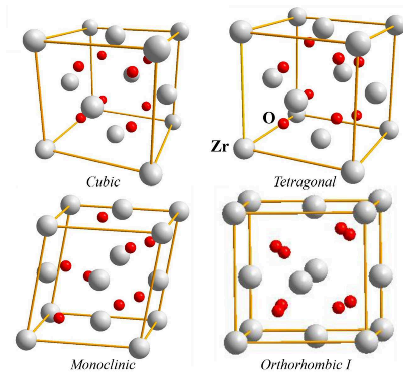
Figure 46: Graphical representation of fluorite-derived structures of zirconia.
