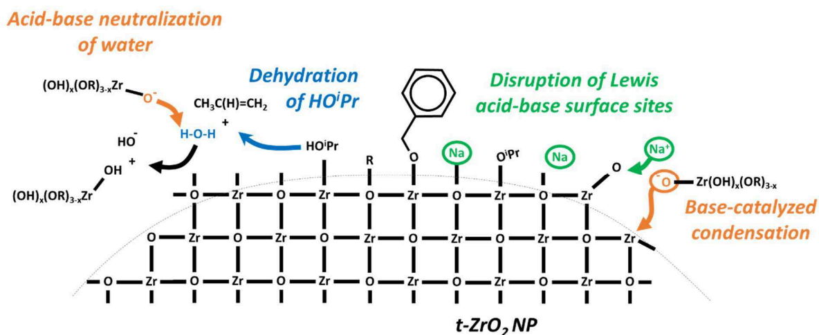
Figure 148: Schematic representation of the two types of inhibition or neutralization of water.
