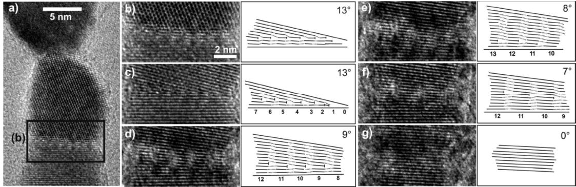
Figure 44: Rotations followed by interface relaxation, imaged during heating of 10 nm sized PbSe QDs at a temperature of 170 °C, increasing to 200 °C, over a time span of 23 min. (a) Triplet of attached quantum dots with interfaces. The two dots at the bottom fuse into a single crystal. (b-g) Details of the bottom interface. Lattice planes drawn from the images are shown on the right-hand side. (b) The dots are not aligned. (c) The top QD has rotated, so that both crystals now display the same line pattern with a mistilt of \phi=13^\circ . The interface is very sharp and involves only a few atomic layers, in which 7 interface dislocations can be identified (displayed schematically on the right-hand side of the image). (d) The mistilt has decreased to \phi=9^\circ through a reduction of the number of interface dislocations to 4. Also the interface area broadens as the dislocations evolve and produce strain fields also in atomic layers further away from the interface. (e,f) Further decrease of the mistilt to 8 and 7^\circ accompanied by a decrease of the number of dislocations. (g) There are no dislocations left; the crystals have fused into a single crystal according van Huis et al. [70].
