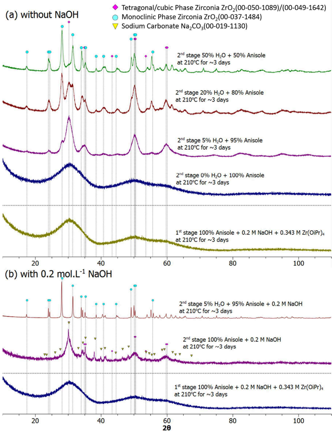
Figure 153: XRD patterns of zirconia samples prepared via dual-stage strategy at 210°C for (3+3) days using [Zr(OiPr)_4 \cdot HOiPr]_2 (a) without and (b) with 0.2 mol.L -1 NaOH in anisole prepared using solvothermal technique with varied amounts of water.
