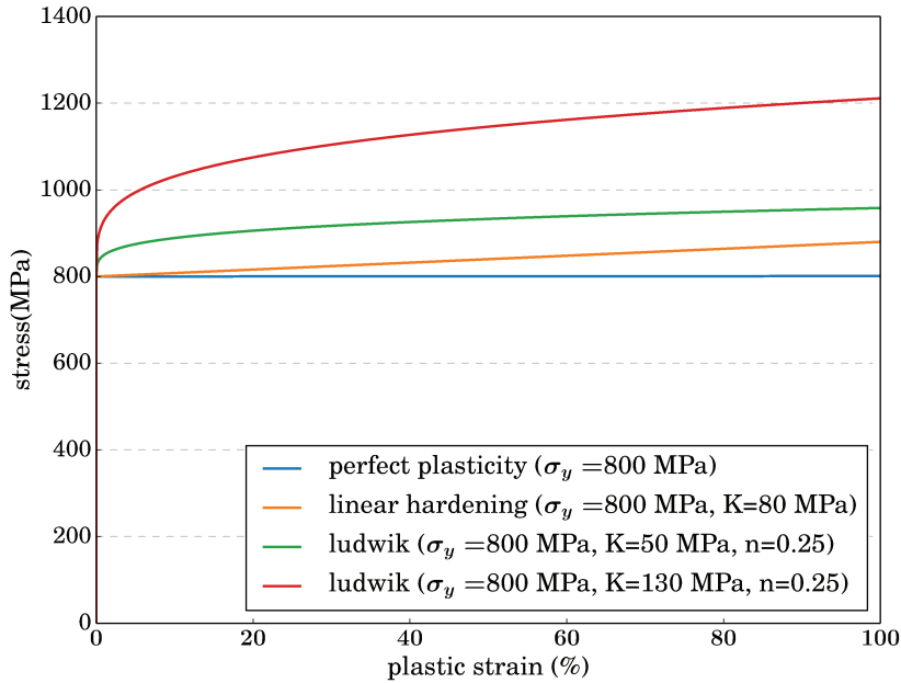
FIGURE 3.3: Different elastic-plastic responses: Perfect plasticity, linear hardening and Ludwik law with different hardening moduli.
