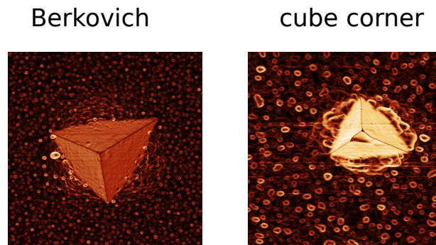
FIGURE 2.7: AFM micrographs of Berkovich (left) and cube corner (right) residual imprints on 400 nm gold thin film.
