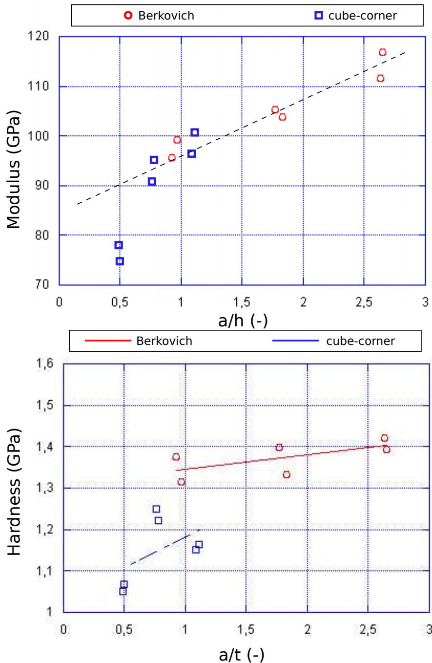
FIGURE 2.8: Indentation modulus and hardness as function of normalized equivalent contact radius \frac{a}{t} for 400 nm gold thin film deposited on silicon substrate. The red circles correspond to Berkovich indenter data while the blue squares correspond to cube-corner indenter data.
