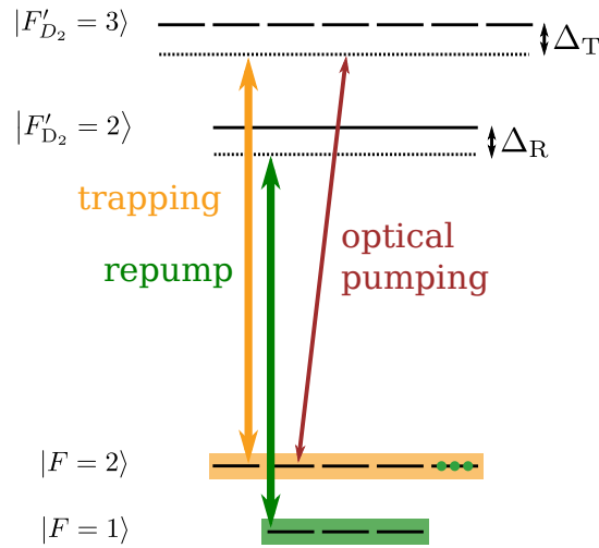
Figure 2.5: The atomic level scheme for the MOT preparation at ANU. During loading, the three retro-reflected two-inch cooling beams have a total power around 400 mW and 40 mW for repump light. At the end of the preparation sequence, the atoms are optically-pumped to the edge Zeeman state by a \sigma_+ -polarised beam, at the same frequency as the cooling beams. The optical pumping is accompanied by a resonant repump to leave the atoms in the ground state |g\rangle = |5S_{1/2}, F = 2, m_F = +2\rangle .
