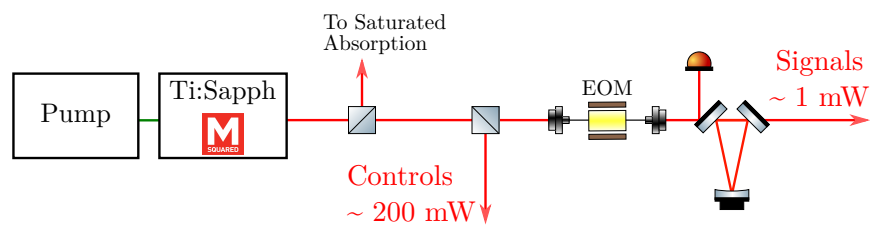
Figure 4.9: D_1 -light layout: The titanium-sapphire laser is frequency-locked on a saturated absorption channel (not depicted), and divided into control and signal channels. The signal channel goes through a fibre-EOM and the +6.8 GHz side-band is separated from the carrier on a ring cavity.
