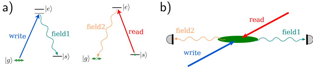
Figure 1.9: Principle of the DLCZ protocol. a) A write pulse, detuned from the excited state probabilistically generates a single photon in mode field 1, whose detection heralds a single collective excitation in |s\rangle . Subsequently applying a strong resonant read pulse deterministically produces a single photon in field 2. b) The geometry of the write and read beams to generate counter-propagating field 1 and field 2.
