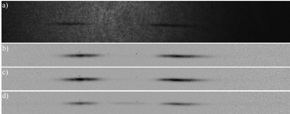
Figure 5.8: CCD images for a 4- \mu\text{s} imaging pulse during a 300- \mu\text{s} exposition time, corresponding to the duration of the whole SL experiment. Each measurement is constructed from ten images that are averaged to reduce shot-to-shot noise of the CCD camera. a) Single raw image capture showing a shadow where a spin wave has been written to the atoms. Averaged image over the ten acquisitions, hinting more precisely where spin-wave intensity |\hat{S}|^2 — and therefore absorption — is significant: b) after the optical pulse is initially encoded in the atoms, and after it has evolved into a steady state for spin waves c) with opposite phase, d) with the same phase.
