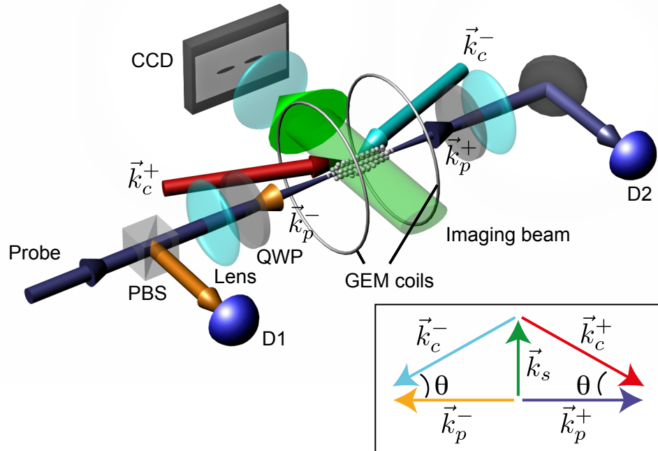
Figure 5.5: The experimental schematic for the SL pulse generation in an ensemble of cold ^{87}\text{Rb} atoms. The spinwave is created by storing a probe pulse via the gradient echo memory technique with forward control field. The magnetic field gradient over the ensemble is controlled by a set of coils (GEM coils). A backward control field couples to a backward probe, counter-propagating with its forward counterpart. Forward and backward probe and control beams are denoted by their wave vector \vec{k}_{(p,c)}^{\pm} . An imaging beam resonant with |s\rangle \rightarrow |5^2P_{3/2}(F'=2)\rangle is used for the absorption imaging of the spinwave. Detector D1 measures the backwards probe field; D2 measures the forward probe field; QWP is a quarter-wave plate and PBS is a polarizing beamsplitter. Inset: The angles between the forward (backward) probe field and the forward (backward) control field are set to be \theta \approx 6 mrad, where the phase matching condition \vec{k}_p^+ - \vec{k}_c^+ = \vec{k}_p^- - \vec{k}_c^- = \vec{k}_s is satisfied. Here, \vec{k}_s denotes the spin-wave wave vector. Please note that the convention for probe and control colour fields slightly differs in this figure from [Everett2017].
