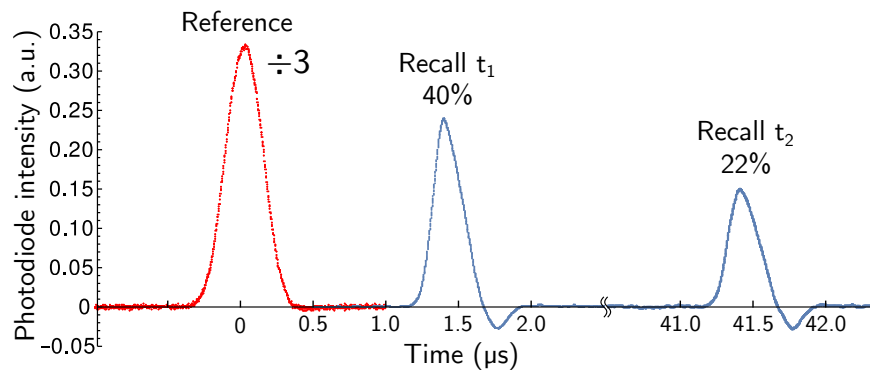
Figure 4.12: Efficient memory for a a 360-ns 1/e^2 -width signal (in red, scaled down). Recalls at times t_1 = 1.5 \mu\text{s} and t_2 = 41 \mu\text{s} (blue) are shown with their storage-and-retrieval efficiency. The decay of the memory efficiency corresponds to a delay-bandwidth product of 160.
