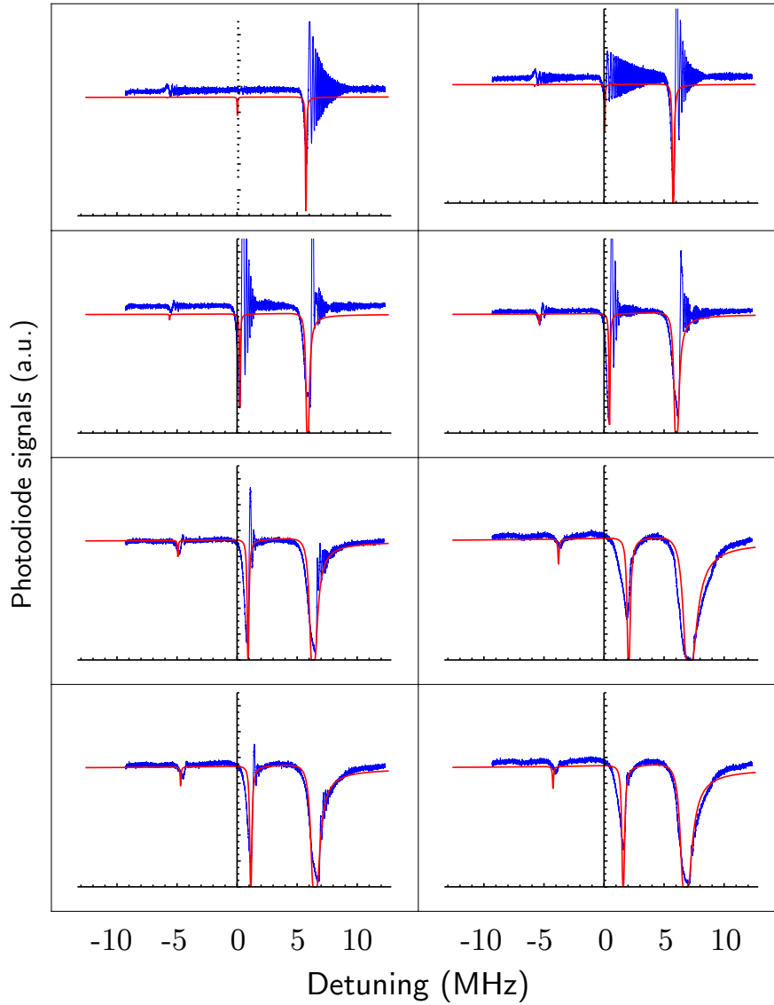
Figure 2.9: Raman line profiles in the ANU cold atomic ensemble, for increasing control field power (for left to right, and top to bottom). The blue curve corresponds to the experimental photodiode signal when the probe frequency is swept over the detuning shown in the x -axis. The theoretical absorption profile, in red, is manually tuned to match all the experimental curves, which provides a measurement of the OD, as well as the correspondence between the control field power and its Rabi frequency as seen by the atoms. In this case, the OD is found to be equal 250, along with the following set of parameters: \Gamma = 6.066 MHz, \gamma_{gs} = 8 kHz.
