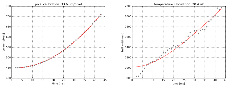
Figure 2.12: a) Position of the atomic centre of mass with time of flight. Knowing the mass of the atoms, a free-fall model gives access to the pixel scale for the imaging system. b) The width of the atomic cloud with the time of flight indicates the cloud temperature from a Boltzmann statistics.
