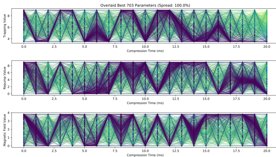
Figure 2.15: Overlaid best parameters for 703 sequences optimised by machine-learning. The darker a parameter region is, the more sequences had values of this parameter optimised in this range. Therefore the darkest line corresponds to a optimal run across all sequences, associated with a global minimum of the cost function.
