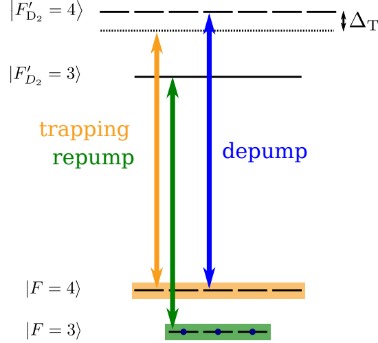
Figure 2.3: The atomic level scheme for the MOT preparation at LKB. During loading, the three retro-reflected two-inch cooling beams have a total power around 300 mW and the repump beams have 10 mW. At the end of the preparation sequence, the atoms are “depumped” to the lower ground state, in |g\rangle = |6S_{1/2}, F = 3\rangle , in a superposition of all the Zeeman sub-levels. This is performed by a depump beam resonant with the |s\rangle \rightarrow |6P_{3/2}, F' = 4\rangle transition, accompanied by the trapping beams relatively close to resonance and the repump off. The repetition rate of the complete sequence is 16 Hz.
