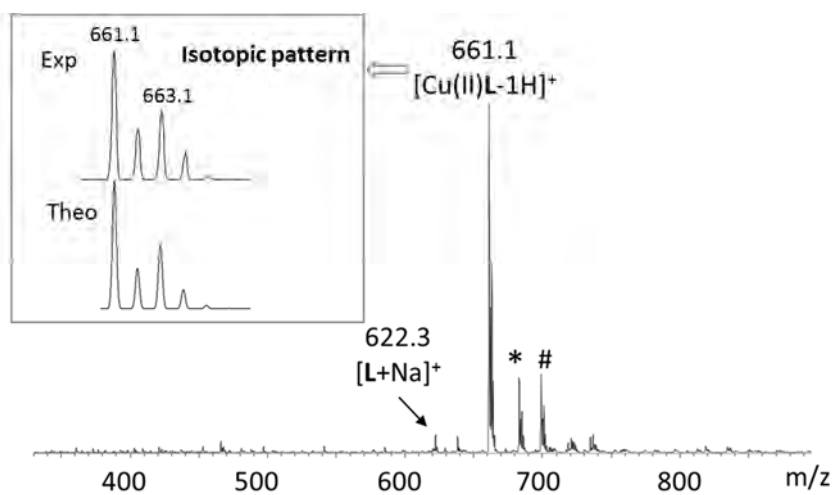
Figure S1. (+)ESI-MS spectrum of L (100 \mu M) with equimolar Cu(II)SO 4 , in ammonium acetate buffer (20 mM, pH 6.9). * Sodium adducts. # Potassium adducts.
