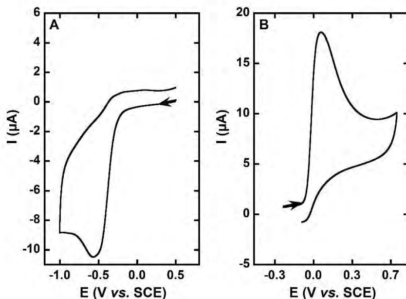
Figure S5. Cyclic voltammograms of O_2 (Panel A) and ascorbate (Panel B). [O_2] \approx 0.2 mM, [Asc] = 1 mM in [phosphate buffer] = 100 mM at pH 7.1. Scan rate = 100 mV \cdot s^{-1} ; WE = Glassy carbon, Ref = SCE, CE = Pt wire.
