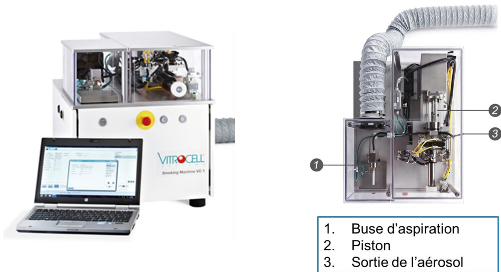
Figure 9. Smoking machine VC1 (d'après https://www.vitrocell.com/inhalation-toxicology/smoking-machines/vc-1 )
