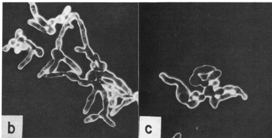
Figure 1 – temperature-sensitive mutants
