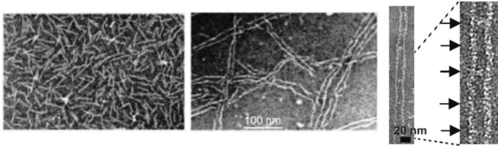
Figure 28 – Solutions of budding yeast septin filaments
