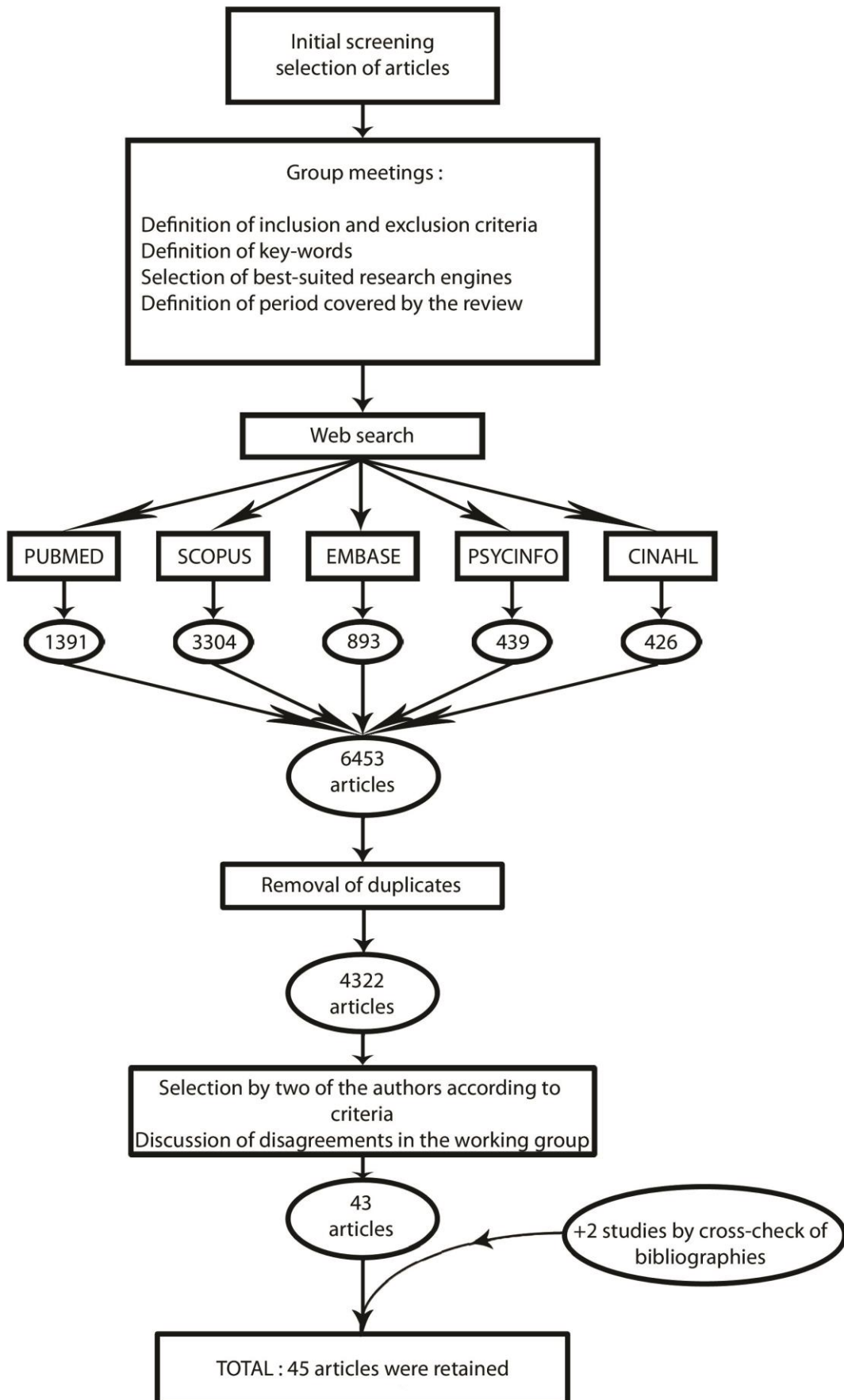
Figure 1 - Flowchart for selecting studies
