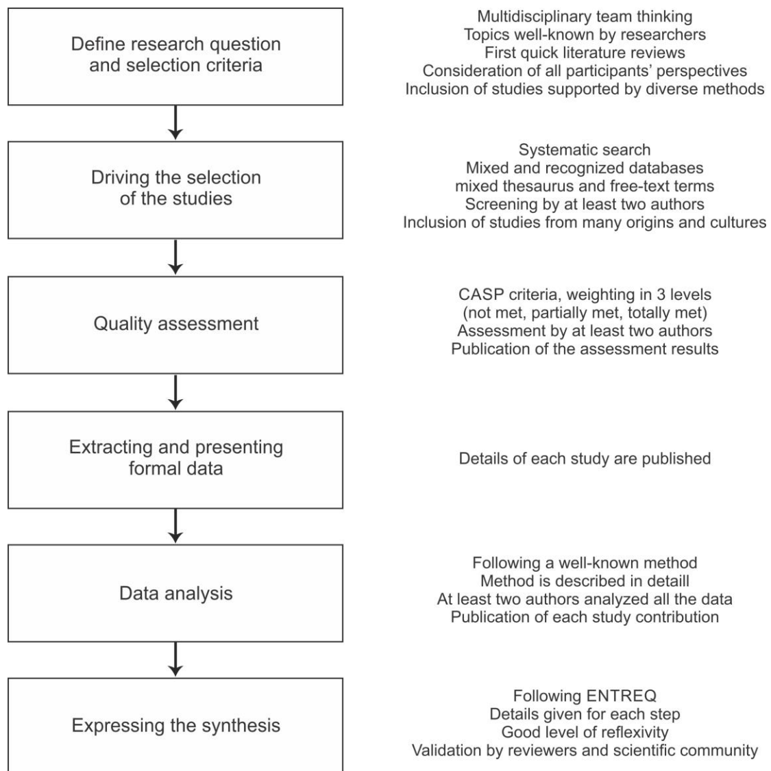
Fig 1 – Flowchart of the study process
