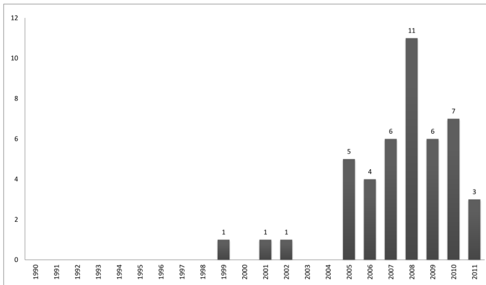
Fig 2 - Distribution in time for papers included in [55]
