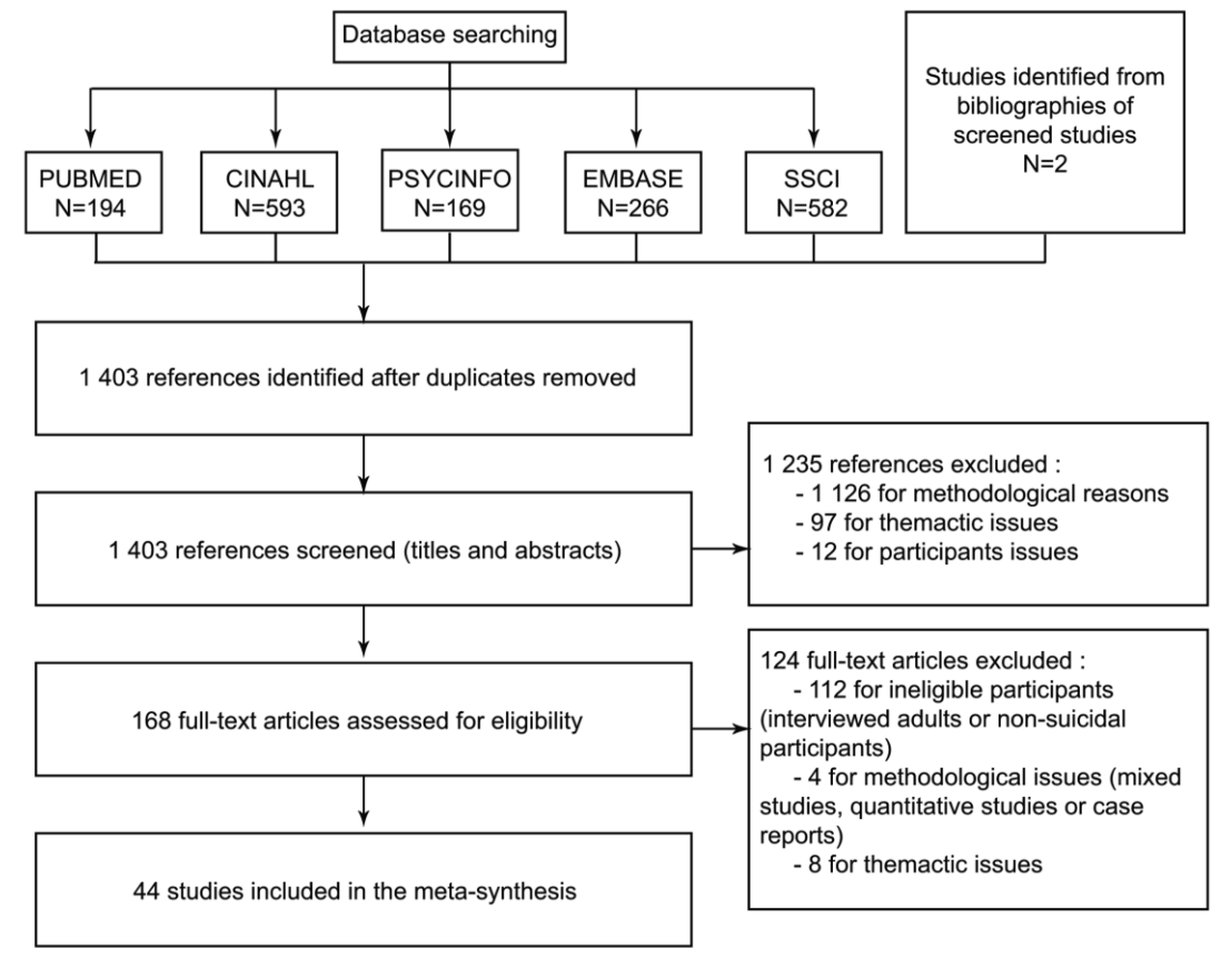
Fig. 1. Flowchart for selecting studies
