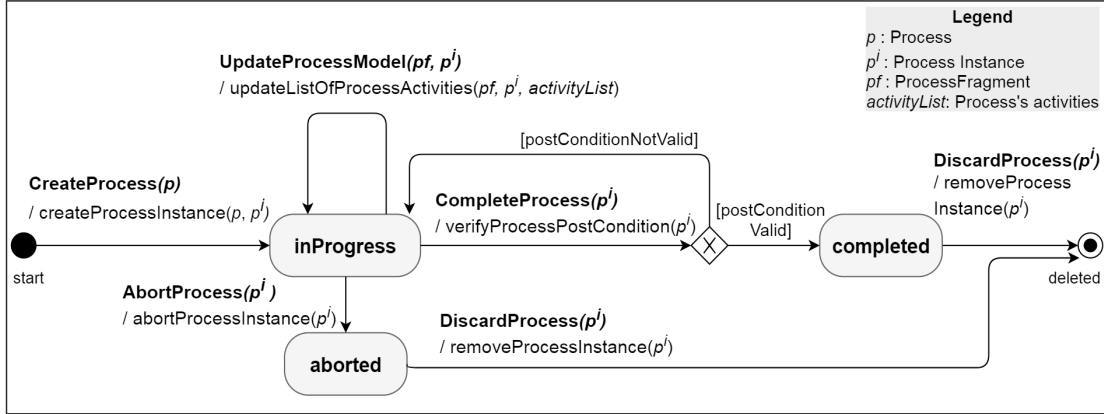
Figure 3.5: Process State Machine
