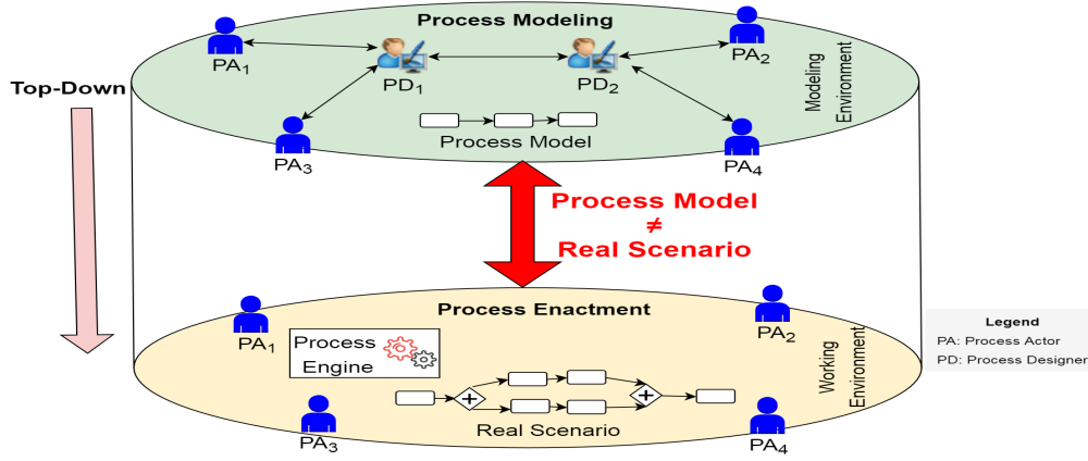
Figure 1.1: Activity-driven and top-down process management
