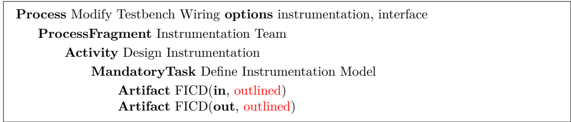
Figure 2.12: Invalid Model of constraint artifactStateNotSame
