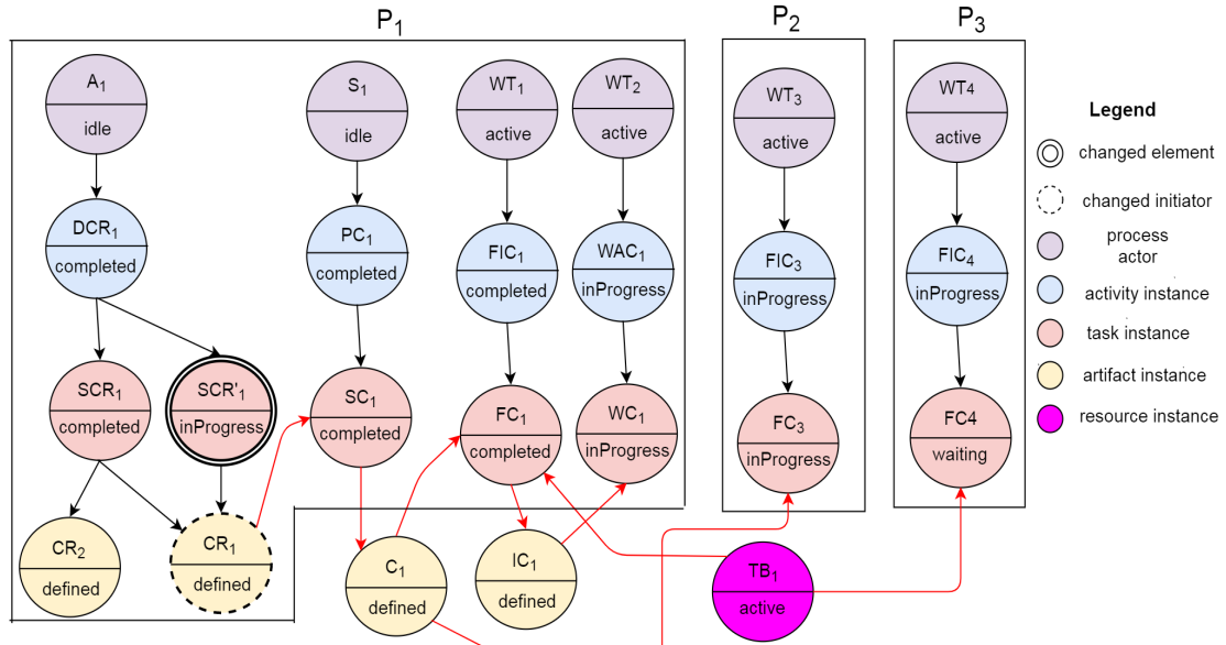
Figure 5.9: Execution Scenario \Delta
