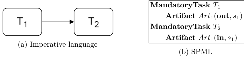
Figure 2.18: Sequence Pattern in SPML and imperative language
