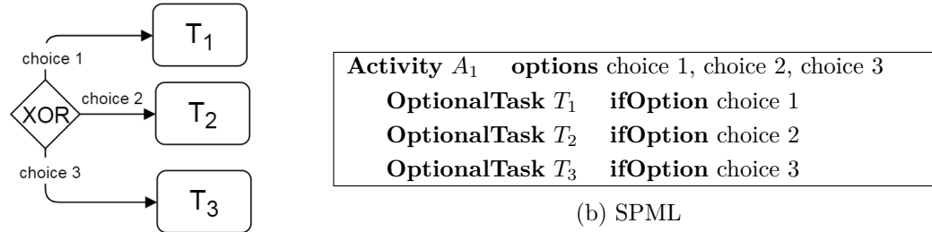
Figure 2.20: Choice Pattern in SPML and imperative language
