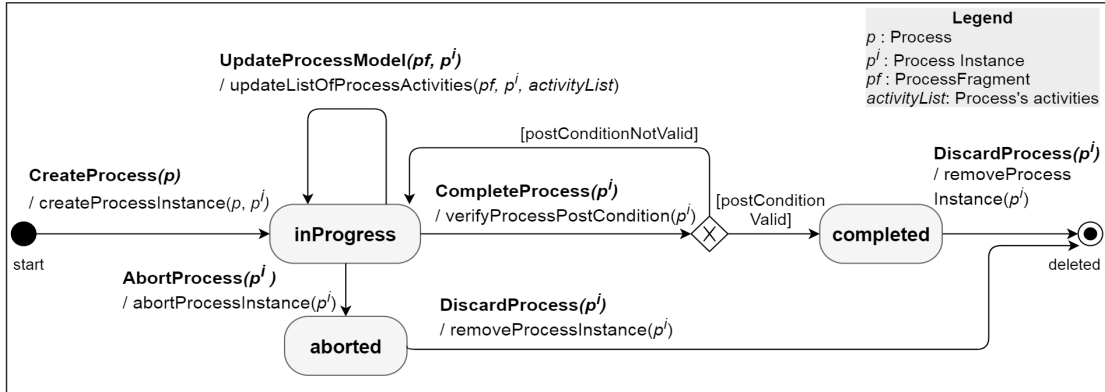
Figure 1.6: Process state machine
