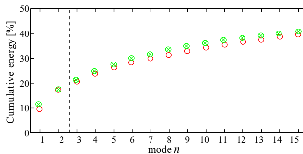
Figure 4.32 – Cumulative energy from POD decomposition of the velocity fields. 'o' red circle: multi-frequency forcing, '⊗' green crossed-circles: generalized feedback control.
