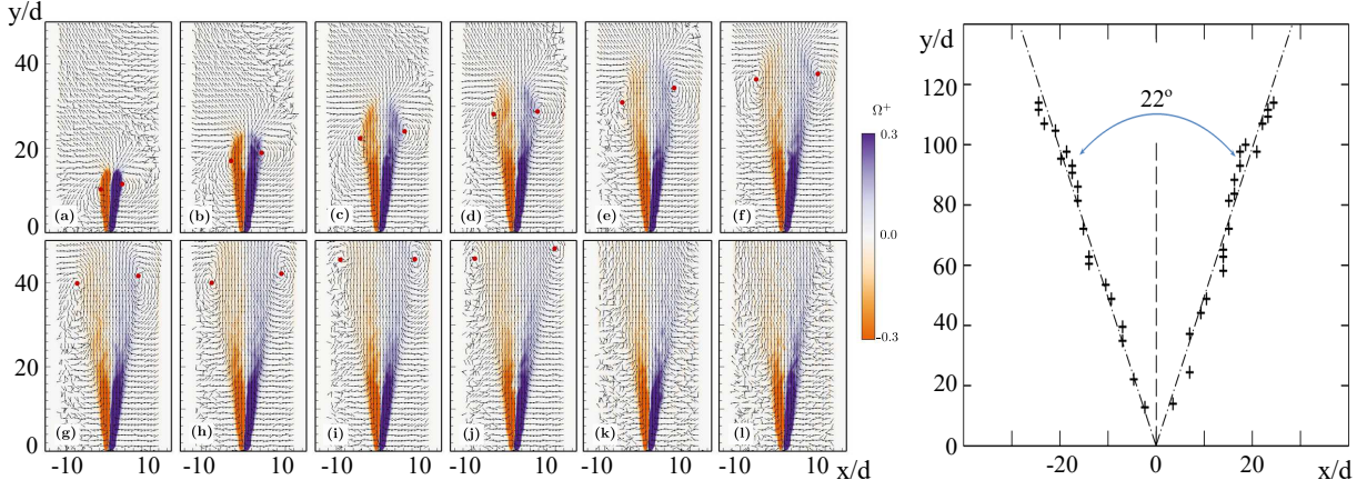
Figure 2.18 – Ensemble-averaged vorticity color plot with vectors superimposed, for a square signal of V_e=20 Volts, f_a = 1 Hz, (a) t/\mathbf{T}=0.01 , (b) t/\mathbf{T}=0.02 , (c) t/\mathbf{T}=0.03 , (d) t/\mathbf{T}=0.04 , (e) t/\mathbf{T}=0.05 , (f) t/\mathbf{T}=0.06 , (g) t/\mathbf{T}=0.07 , (h) t/\mathbf{T}=0.08 , (i) t/\mathbf{T}=0.09 , (j) t/\mathbf{T}=0.10 , (k) t/\mathbf{T}=0.20 , (l) t/\mathbf{T}=0.30 . The clockwise and counter-clockwise flow structures location are identified by the red points. Positions of phase-average vortex centres at each t=0.005\mathbf{T} of the transient injection cycle.
