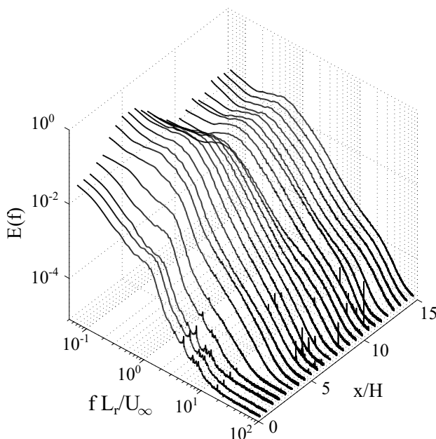
Figure 3.12 – Power spectra of wall-pressure fluctuations for different x/h locations at \text{Re}_H = 64200 .
