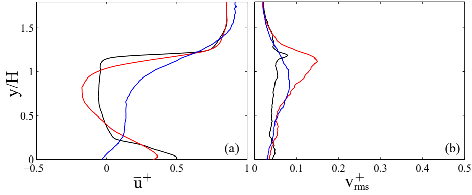
Figure 4.5 – (a) Time-averaged streamwise velocity ( \bar{u}^+ ), (b) Root-mean-square of the cross-stream velocity ( v_{\text{rms}}^+ ) profiles for various x/H positions ( x/H = '—' black line: 0.2, '—' red line: 0.6, '—' blue line: 1.5).
