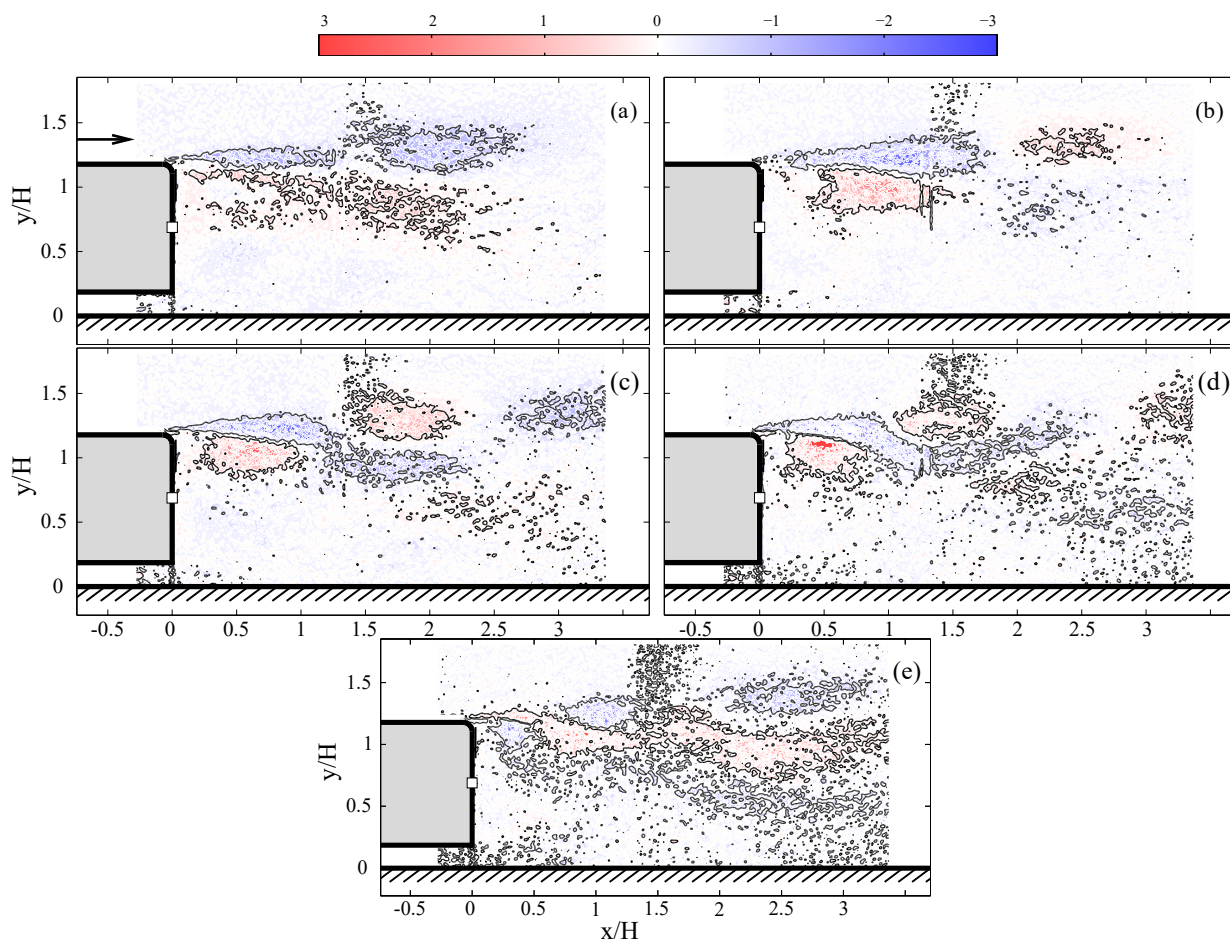
Figure 4.8 – Low-order POD velocity modes: (a) mode 1, (b) mode 2, (c) mode 3, (d) mode 4, (e) mode 5. Contour map shows the vorticity calculated from the corresponding POD velocity basis function and normalized with the step height and free-stream velocity ( \omega_z H / U_\infty ).
