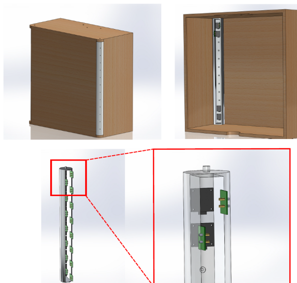
Figure A.2 – Simplified truck model with a movable cylinder equipped with 20 micro-blowers. Figures obtained from Minelli (2017)
