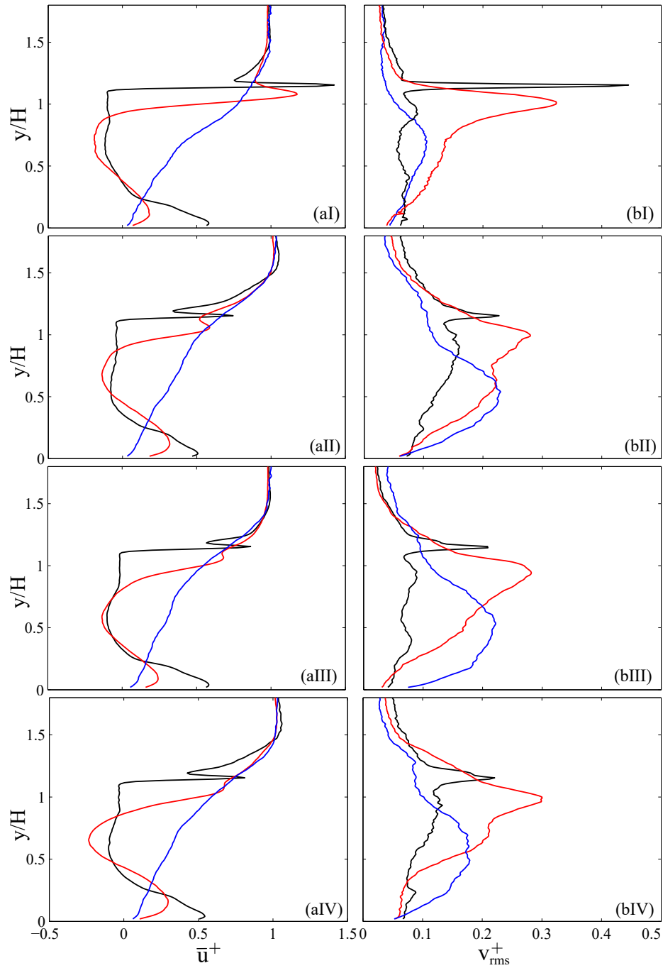
Figure 4.14 – (a) Time-averaged streamwise velocity ( \bar{u}^+ ) and (b) Root-mean-square of the cross-stream velocity ( v_{\text{rms}}^+ ) profiles for various x/H positions ('—' black line: x/H = 0.2 , '—' red line: x/H = 0.6 , '—' blue line: x/H = 1.5 ). (I) Case I: Steady blowing, (II) Case II: St_a = St_o/2 , (III) Case III: St_a = St_o , (IV) Case IV: St_a = 3St_o
