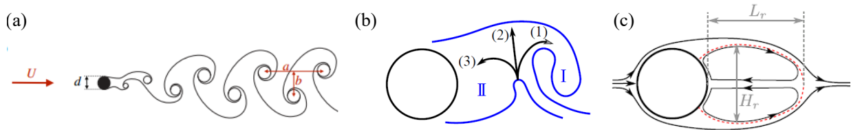
Figure 1.4 – (a) Schematic visualization of the Kármán vortex street (Eulalie, 2014), (b) Interaction of opposing shear layer (Gerrard, 1966), (c) Mean wake of a cylinder, obtained from (Li, 2017), '- -' red dashed line represents the recirculation bubble boundary. L_r and H_r are the bubble length and width, respectively.
