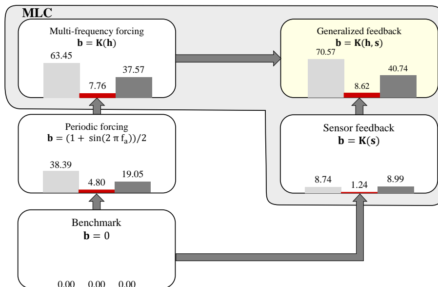
Figure 3.39 – Summary of both recirculation lengths and area; '■' dark red bars: external separation lengths L_r , '■' dark grey bars: internal separation length X_r and '■' light grey bars: separation area for all studied cases. Variations are in %
