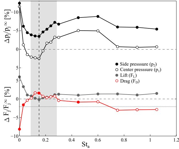
Figure 4.11 – Normalized and averaged variations of the rear pressures p_i ( p_1 and p_2 ), and forces F_i (lift F_L and drag F_D ) compared to the natural case p_i^\infty and F_i^\infty . These parameters are plotted as functions of the actuation frequency St_a at C_\mu=0.00678 for Re_H = 9 \times 10^4 . The dash-line denotes the worst control case ( St_o ), corresponding to the wake shedding. Note that for the steady blowing ( St_a = 0 ), the momentum coefficient is C_\mu=0.01355 due to the duty cycle of the forcing cases. Filled red dots represent the four cases studied.
