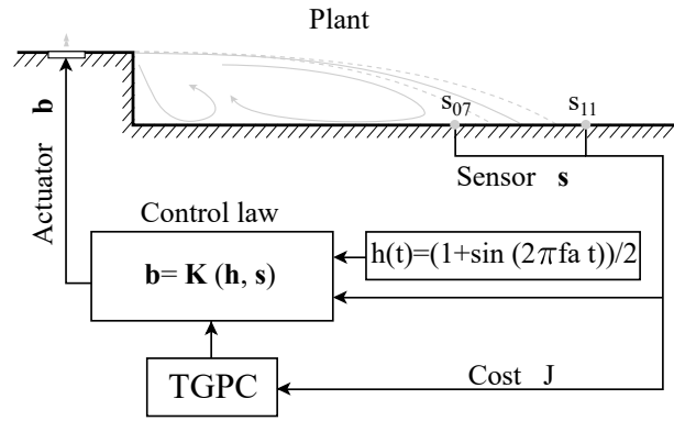
Figure 3.27 – Diagram of machine learning control architecture using tree-based genetic programming
