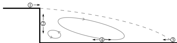
Figure 1.11 – Actuation positions based on theoretical mechanisms presented by Sujar (2014).
