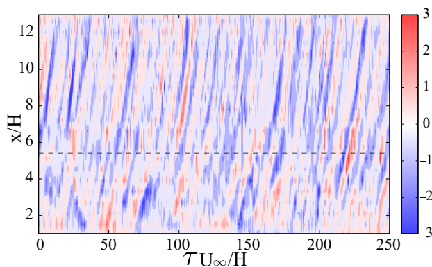
Figure 3.11 – Space-time contour plots of instantaneous wall-pressure fluctuations normalized by the rms pressure p/p_{\text{rms}} for \text{Re}_H = 64200 . '- - -' dashed line denotes the reattachment point.
