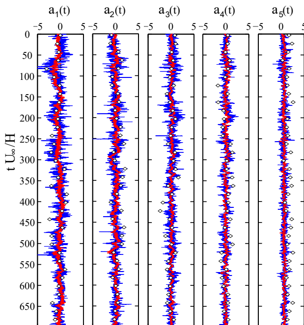
Figure 3.19 – Comparisons between the original ('◇' diamond symbol) and estimated MLSE ('—' red line) and MQSE ('—' blue line) temporal coefficients for the POD mode 1 to 5.
