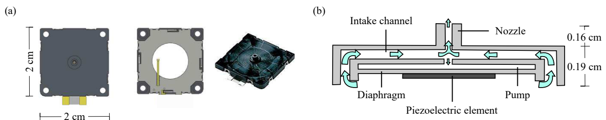
Figure 2.11 – (a) General characteristics of the actuator, (b) Cross-section of the micro-blower.
