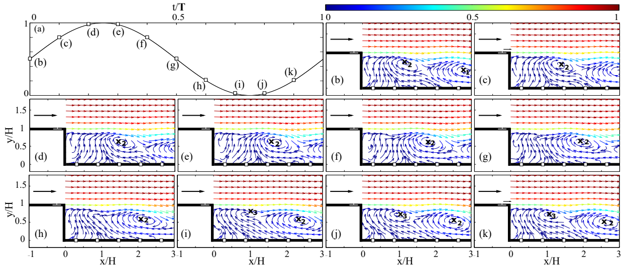
Figure 3.37 – Phase averaging of the (a) Jet velocity profile along the period \mathbf{T} for the optimal forced case. (b) to (k) temporal POD coefficient, a_i(t) , obtained from the MQSE for the 10 phases mentioned in (a). Vector lengths are normalized and equal to highlight the main flow structures. Colourbar represents the normalized velocity magnitude.
