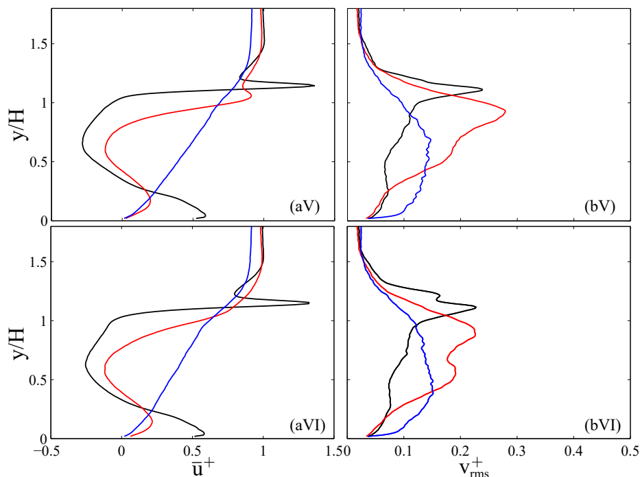
Figure 4.29 – (a) Time-averaged streamwise velocity ( \bar{u}^+ ) and (b) root-mean-square of the cross-stream velocity ( v_{\text{rms}}^+ ) profiles for various x/H positions ('—' black line: x/H = 0.2 , '—' red line: x/H = 0.6 , '—' blue line: x/H = 1.5 ). (V) Case V: Multi-frequency forcing; (VI) Case VI: generalized feedback control.
