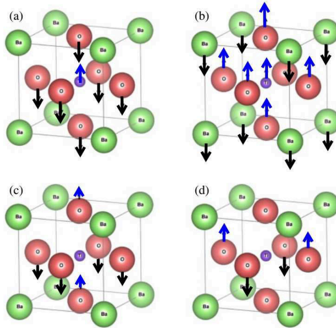
Figure 4.3: The classification of phonons in perovkites [95] depending on the involved atoms: (a) Slater n=1 (b) Last n=2 (c) Axe n=3 (d) \text{O}_4 torsional mode, n=4
