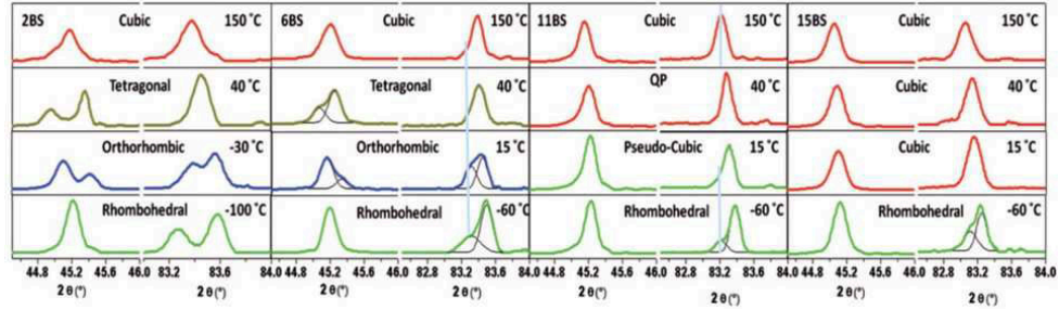
Figure 1.9: XRD patterns of Sn-rich compositions of \text{Ba}(\text{Sn},\text{Ti})\text{O}_3 at different temperatures, x(\text{Sn})=0.02; 0.06; 0.11; 0.15 [33]
