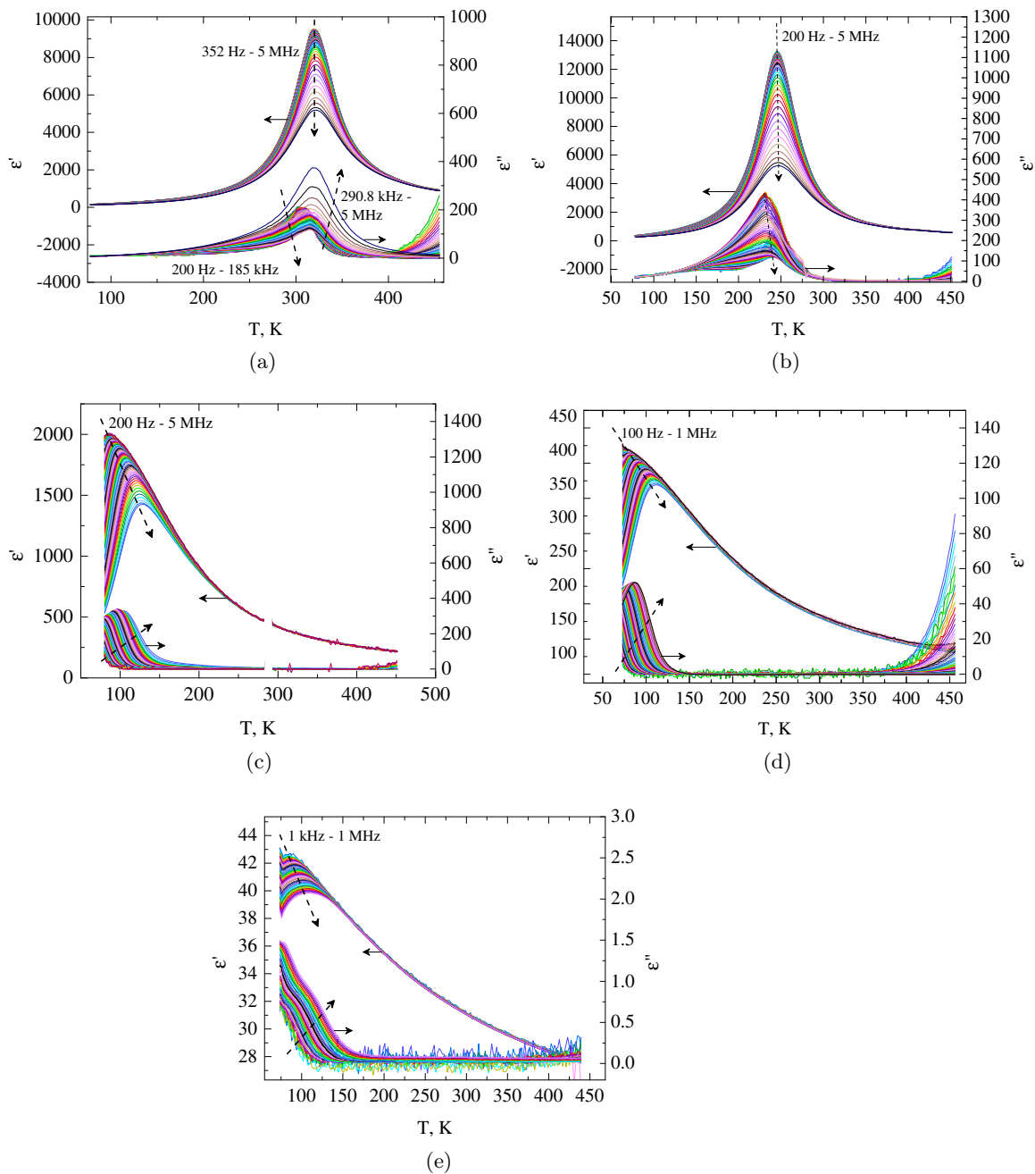
Figure 2.6: Dielectric permittivity and losses for BaSn x Ti 1-x O 3 with x(Sn): (a) 0.1, (b) 0.2, (c) 0.4, (d) 0.5 (synthesis with PVA) and (e) 0.8 (synthesis without PVA)
