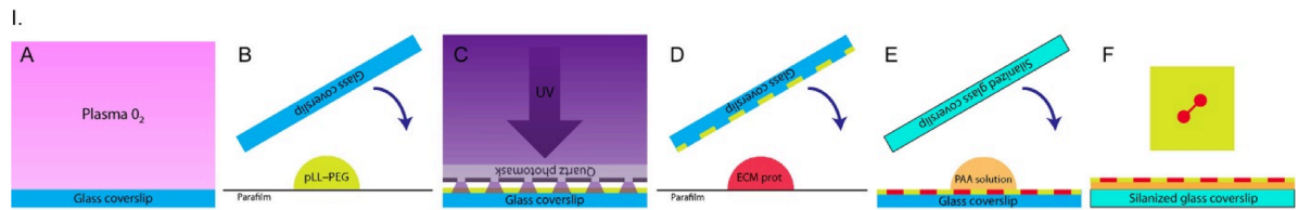
Figure 40: Schematic representation of creating micropatterns on top of soft hydrogels using the glass technique. A) Activation of a glass coverslip with plasma. B) Coating the activated glass coverslip with pLL-PEG. C) Burning of the polymer brush via local UV exposure through a photomask. D) Incubation with ECM protein solution (in our case fibronectin and fibrinogen). E) Polymerization of acrylamide solution in between the patterned glass coverslip and a silanized coverslip. F) After the peel-off, the final result is an adhesive micropattern of defined geometry on top of a soft polyacrylamide gel, which is attached to the silanized glass coverslip. [Figure taken from: (Vignaud 2014)]
