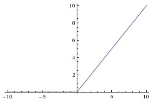
(c) ReLU
