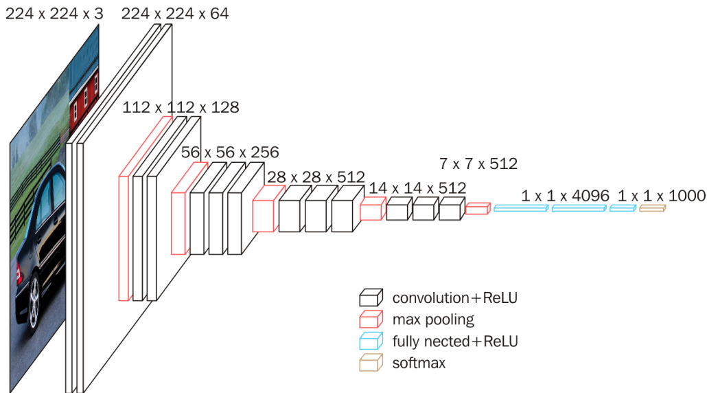
Figure 3.12 : Architecture VGG [5]
