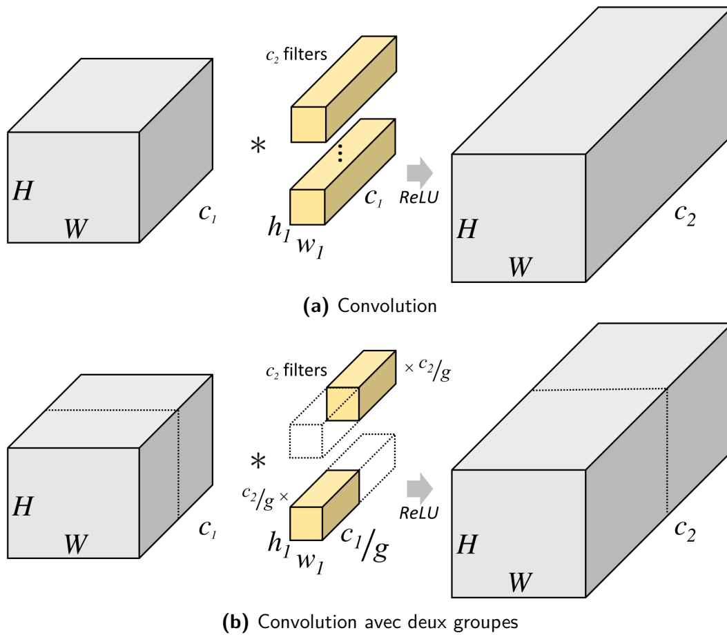
Figure 3.16 : Illustration des convolutions groupées (source [9])
