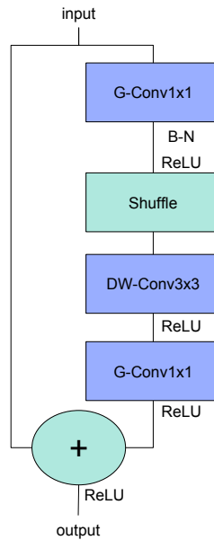
Figure 3.18 : Module “Shuffle” de ShuffleNet [10]
