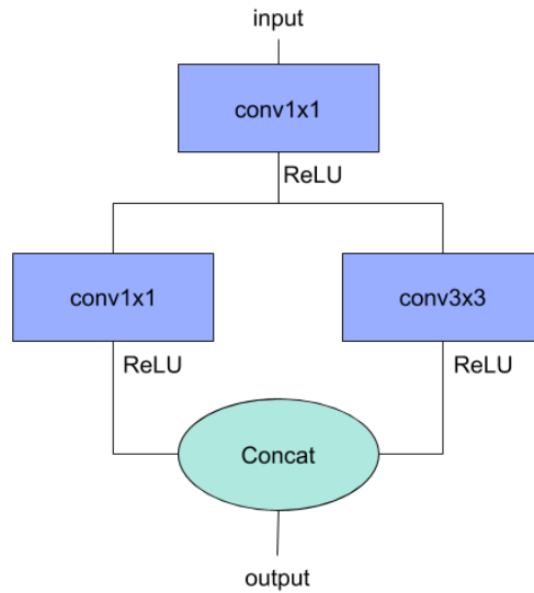
Figure 3.15 : Module “FIRE” de SqueezeNet [8]
