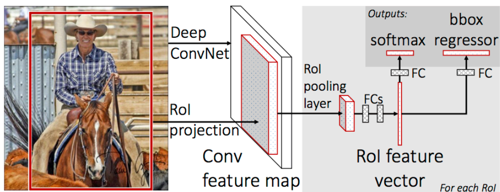
Figure 3.19 : Architecture Fast-RCNN [11]
