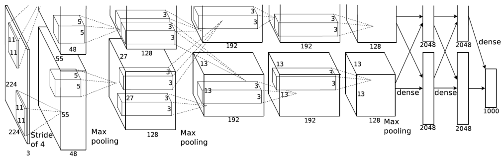
Figure 3.11 : Architecture AlexNet [4]
