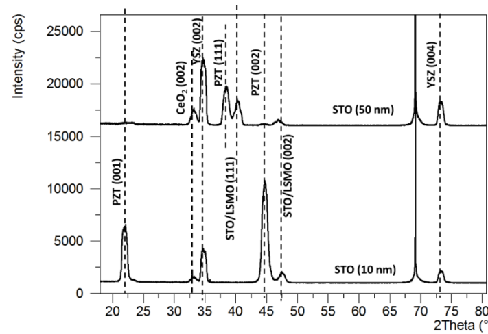
Figure III-7: XRD diagram of PZT films grown on LSMO/STO buffered CeO 2 /YSZ/Si with two different thicknesses of STO
