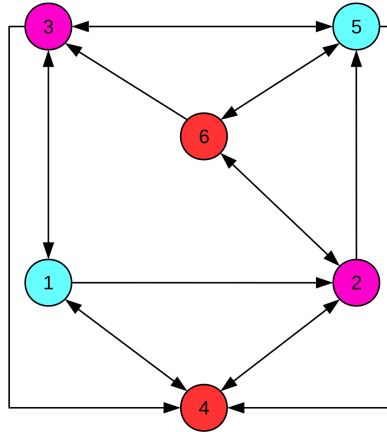
Figure 3.3 – Directed graph after coloring
