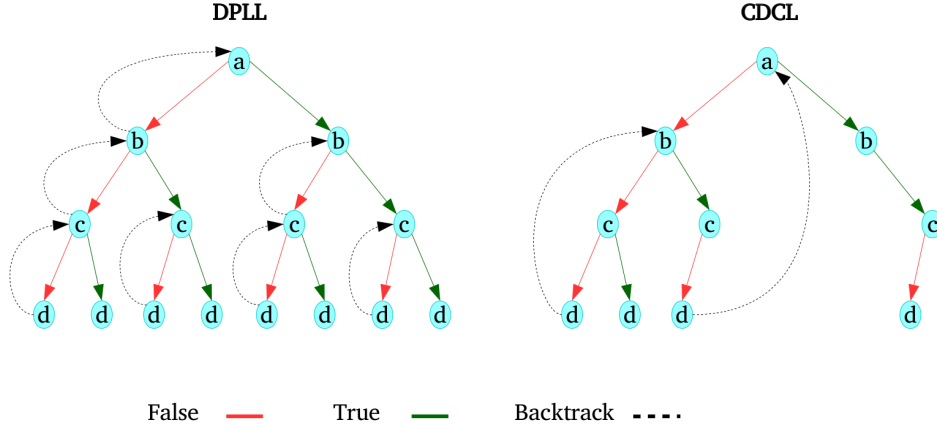
Figure 5.1 – Difference between CDCL and DPLL algorithms. The dashed arrows represent back-jumps. The red and green arrows denote false and true assignment.
