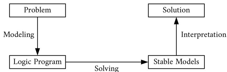
Figure 3.1 – ASP workflow
