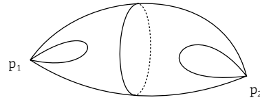
FIGURE 1.2 – Niveau f(y) = 1 .
