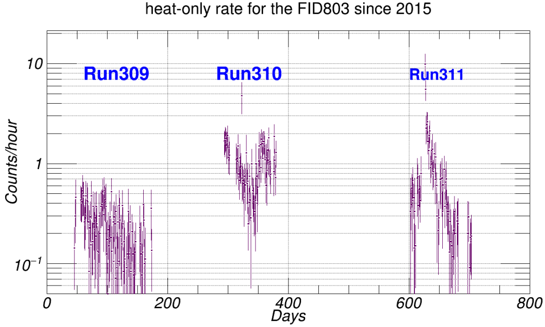
Figure 4.27 – Heat-only count rate of FID803 detector during run309, run310 and run311, for heat-only events with phonon energy above E_{\text{phonon}}^{\text{min}} = 15 \text{ keV} .
