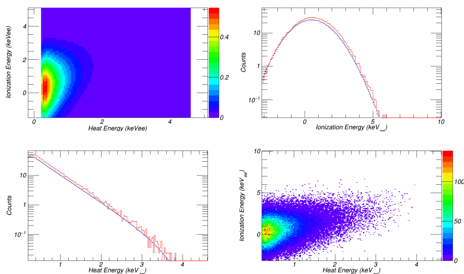
Figure 24 – Top, left: Probability Density Function for the expected signal of a WIMP in a FID800. It is expressed as a function of the two chosen variables of the analysis: E_{ion} and E_{heat} . Bottom, right: simulation of WIMP signals in the same parameter space. This figure allows to confirm that simulated data are in good agreement with the PDF. Top, right: ionization energy spectrum for fake data (in red) and providing from the PDF (in blue). Bottom, left: heat energy spectrum for fake data (in red) and from the PDF definition (in blue). The both are in excellent agreement, modulo one bin corresponding to the way they are filled.
