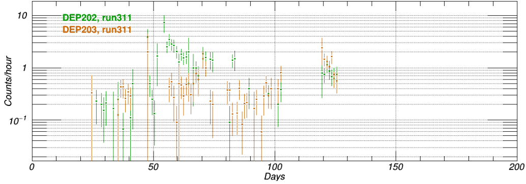
Figure 4.26 – HO rate for DEP detectors which have their NTD deported onto a sapphire slab: DEP202 in green and DEP203 in orange with phonon energy above E_{\text{phonon}}^{\text{min}} = 15 \text{ keV} .
