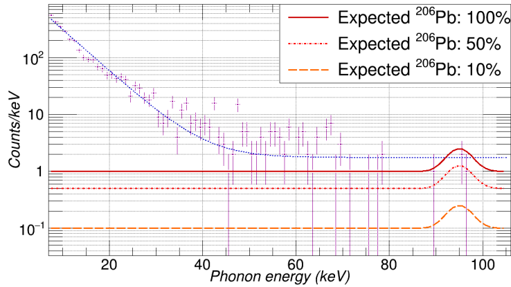
Figure 4.29 – Heat-only energy spectrum (in magenta) for FID803 detector during run309, fitted with a two exponential function (in blue). A function corresponding to a gaussian with a constant term associated to the lead recoil rate as described in chapter 5 is illustrated in dark red. The two other curves correspond to a scale applied on the lead rate (50% for light red dot curve and 10% for orange dashed curve).
