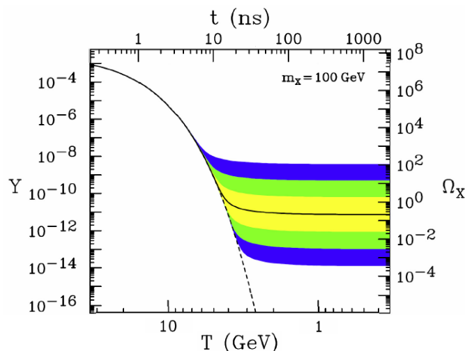
Figure 1.8 – Comoving density as a function of the temperature and resulting thermal relic density for a WIMP mass of 100 \text{ GeV}/c^2 . The annihilation cross-section corresponding to the correct relic density is the solid contour and the shaded zone are for cross-sections which differ by 10 , 10^2 and 10^3 from this value. The density of particle that remains in the thermal equilibrium is the dashed curve [33].
