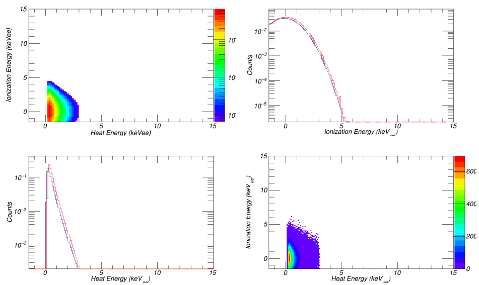
Figure 31 – Top, left: Probability Density Function corresponding to the heat-only background, expressed as a function of E_{ion} and E_{heat} . Bottom, right: simulation of heat-only events. This figure allows to confirm that simulated data are in good agreement with the PDF. Top, right: ionization energy spectrum for fake data (in red) and providing from the PDF (in blue). The both are in excellent agreement. Bottom, left: heat energy spectrum for fake data (in red) and from the PDF definition (in blue).
