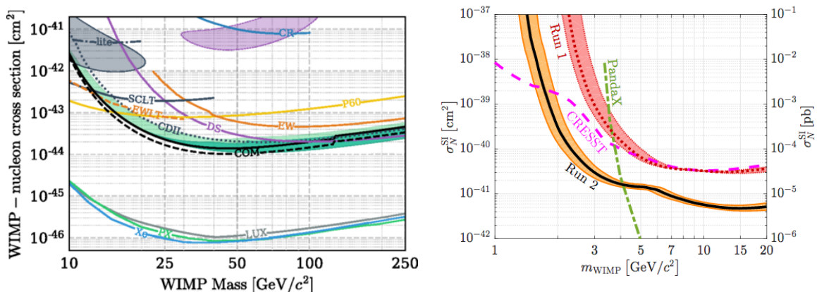
Figure 1.19 – Left: the 90% C.L. upper limit on the DM-nucleon cross-section (solid black) based on the single observed event in SuperCDMS dataset. The range of the pre-unblinding 68% (95%) most likely expected upper limits are shown as dark green (light green) bands. Closed contours shown are CDMS II Si (solid gray, 90% C.L.) and DAMA/LIBRA (dotted purple, 90% C.L.). Also 90% C.L. exclusion limits from other experiments are shown in the figure, taken from [65]. Right: Spin-independent WIMP-nucleon cross-section 90% upper limits from CDMSlite Run 1 (red dotted curve with red uncertainty band) and Run 2 (black solid curve with orange uncertainty band) compared to the other (more recent) most sensitive results in this mass region: CRESST-II (magenta dashed curve), which is more sensitive than CDMSlite Run 2 for m_\chi < 1.7 \text{ GeV}/c^2 , and PandaX-II (green dot-dashed curve) which is more sensitive than CDMSlite Run 2 for m_\chi \geq 4 \text{ GeV}/c^2 . The Run 1 uncertainty band gives the conservative bounding values due to the systematic uncertainty in the nuclear-recoil energy scale. The Run 2 band additionally accounts for the uncertainty on the analysis efficiency and gives the 95% uncertainty on the limit. Figure taken from [51].
