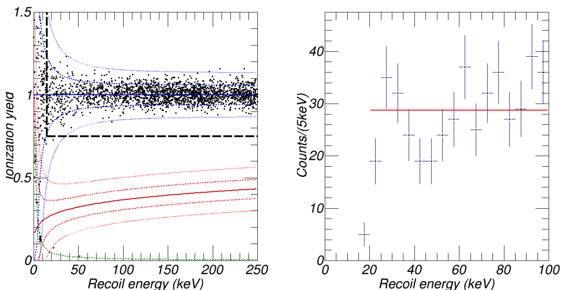
Figure 5.1 – Left: ionization yield as a function of the recoil energy (in keV) for fiducial events in FID803 detector during run309. In blue, the electronic recoil bands at 90% and 99.9% C.L. In red, the nuclear recoil bands at 90% and 99.9% C.L. The fiducial selection is illustrated with the dashed black lines. Right: recoil energy distribution (in keV) for fiducial gamma events and the corresponding fit with a constant term in red.
