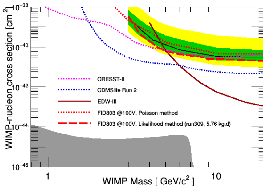
Figure 5.19 – WIMP-nucleon cross-section as a function of the WIMP mass. The black curve represents the sensitivity of the experiment for run309 for m_\chi \in [3; 20] \text{ GeV}/c^2 , with the error bands at 1\sigma and 2\sigma in green and yellow, respectively. The red dashed curve is the limit associated to the dataset of the run309. The previous limit obtained with the statistical method (section II.2.3) is also drawn as the dotted red line for comparison. The magenta curve corresponds to the CRESST results [54], the blue curve to CDMSlite Run2 [51] and the dark red curve to the previous EDELWEISS-III limit [92].
