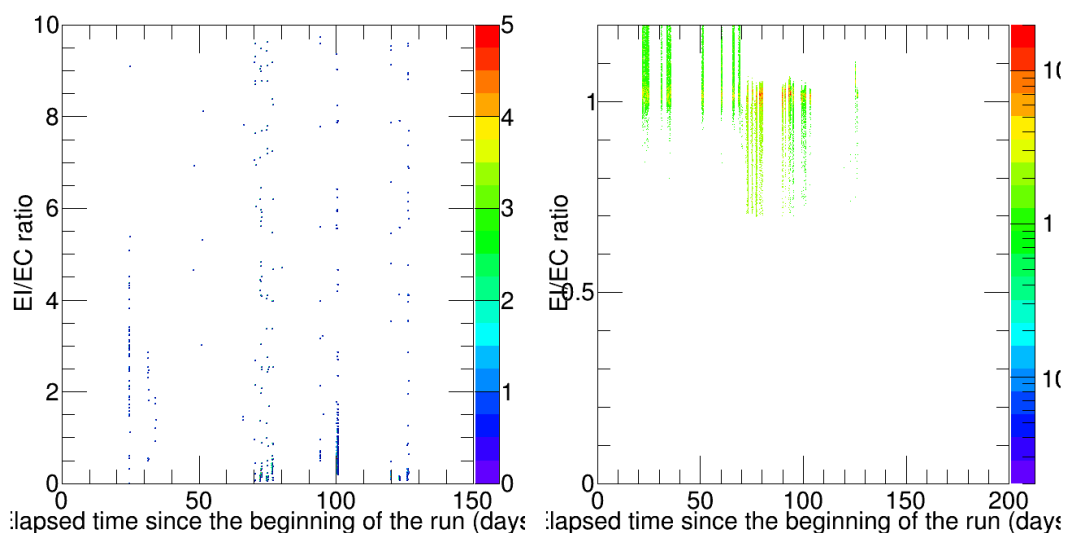
Figure 3.10 – Evolution of the ratio between ionization energy and heat energy as a function of the time of the run before (left) and after (right) the calibration of the heat channels. The ratio is centered around 1 after the calibration procedure.
