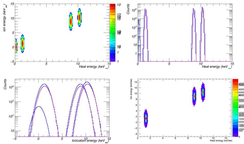
Figure 27 – Top, left: Probability Density Function corresponding to the cosmogenic peak background in the parameter space ( E_{ion}, E_{heat} ). Bottom, right: simulation of cosmogenic peak events in the same parameter space. This figure allows to confirm that simulated data are in good agreement with the PDF. Bottom, left: ionization energy spectrum for fake data (in magenta) and providing from the PDF (in blue). Both are in excellent agreement. Top, right: heat energy spectrum for fake data (in magenta) and from the PDF definition (in blue).
