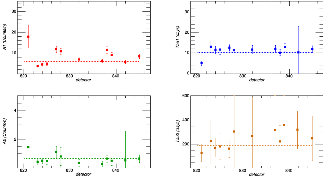
Figure 4.8 – Parameters of the fit f(t) = A_1 \cdot e^{-\frac{(t-t_0)}{\tau_1}} + A_2 \cdot e^{-\frac{(t-t_0)}{\tau_2}} applied on all heat-only count rates for run308 detectors, for E_{\text{phonon}}^{\text{min}} = 10 \text{ keV} . The two left plots correspond to the fitted amplitudes A_i whereas the right plots show the time constants \tau_i . Dashed lines are the average values of respective parameters.
