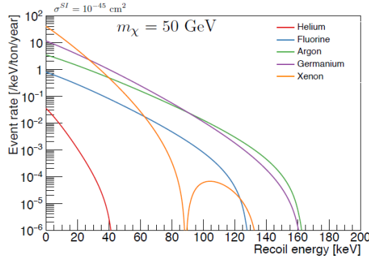
Figure 1.14 – Final recoil spectrum for a WIMP mass of 20 \text{ GeV}/c^2 with different target nuclei, taken from [57].
