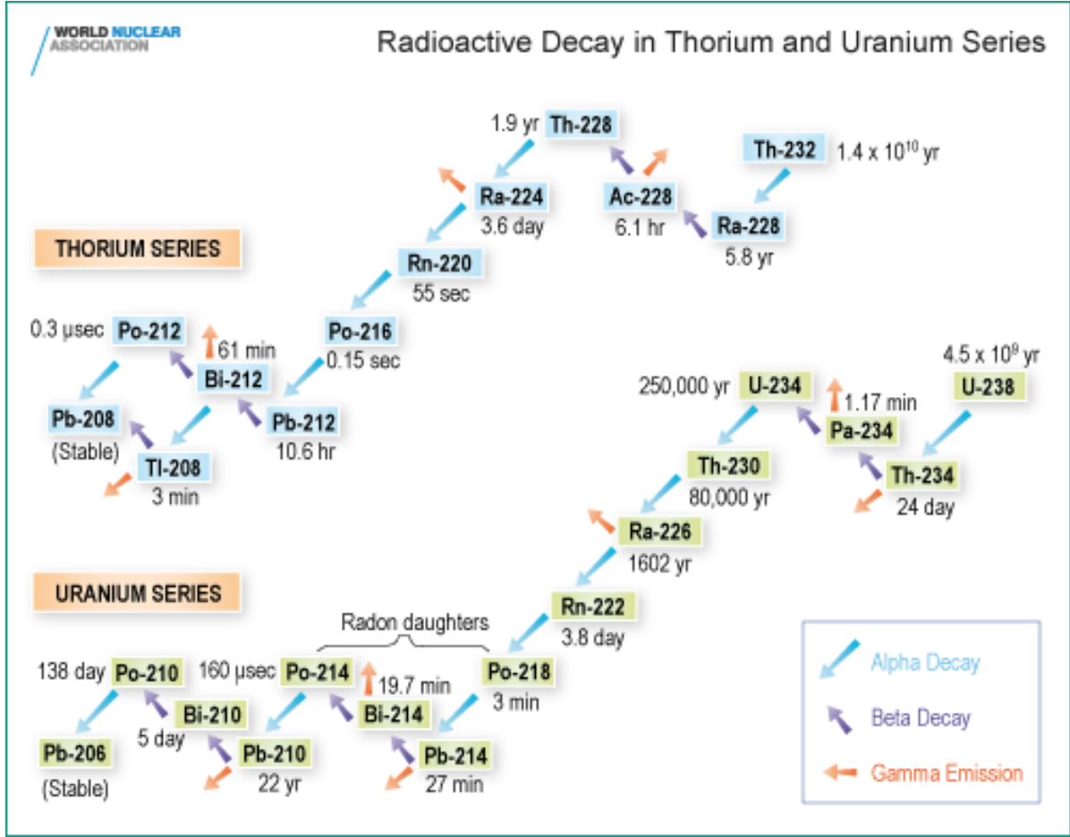
Figure 2.2 – ^{238}\text{U} and ^{232}\text{Th} radioactive chains, taken from [74]. The successive decays give \alpha , \beta and \gamma particles.
