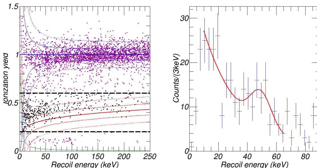
Figure 5.7 – Left: ionization yield as a function of the recoil energy (in keV) for surface events for FID803 detector in run309. In blue, the electronic recoil bands at 90% and 99.9% C.L. In red, the nuclear recoil bands at 90% and 99.9% C.L. The quenching selection Q \in [0.2; 0.6] is illustrated with the dashed black lines: rejected events are the magenta dots. Right: recoil energy distribution (in keV) for these events with the resulting fit of the beta function of Eq.5.13 in red.
