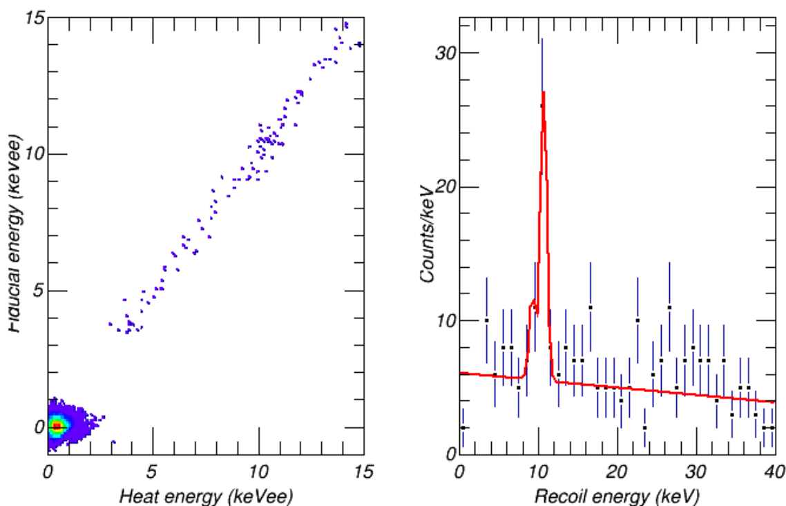
Figure 5.3 – Left: fiducial ionization energy (keV ee ) as a function of heat energy (keV ee ) for FID803 detector during run309. Events well-reconstructed (selection on the \chi^2 of the different channels) and occurring in the fiducial volume of the detector are used. Right: recoil energy spectrum for these events. A double-gaussian function is fitted on these data to determine the amplitude of the two peaks at 8.98 keV and 10.37 keV.
