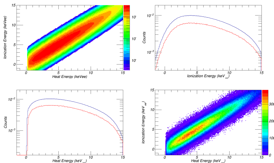
Figure 26 – Top, left: Probability Density Function corresponding to the tritium background in the parameter space (E_{ion}, E_{heat}) . Bottom, right: simulation of tritium events in the same parameter space. This figure allows to confirm that simulated data are in good agreement with the PDF. Top, right: ionization energy spectrum for fake data (in red) and providing from the PDF (in blue). Both are in excellent agreement. Bottom, left: heat energy spectrum for fake data (in red) and from the PDF definition (in blue), showing the same agreement.
