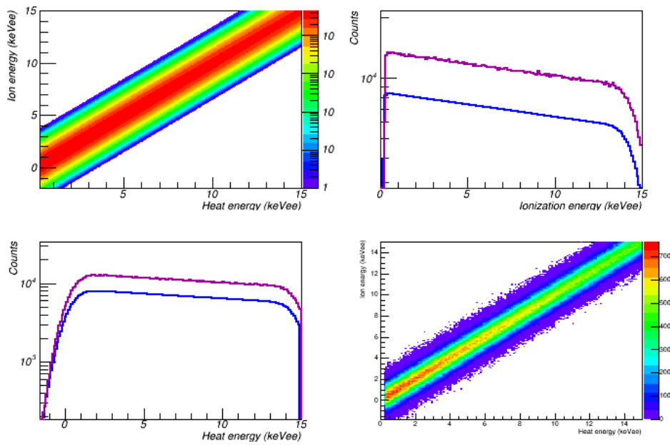
Figure 28 – Top, left: Probability Density Function corresponding to the \beta -background in the parameter space (E_{ion}, E_{heat}) . Bottom, right: simulation of \beta -events in the same parameter space. This figure allows to confirm that simulated data are in good agreement with the PDF. Top, right: ionization energy spectrum for fake data (in magenta) and providing from the PDF (in blue). Both are in excellent agreement. Bottom, left: heat energy spectrum for fake data (in magenta) and from the PDF definition (in blue), showing the same excellent agreement.
