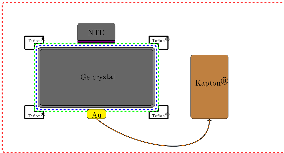
Figure 4.23 – Presentation of the different hypothetical sources of heat-only events on a FID detector. In gray, the Ge crystal surrounded by an amorphous layer of Ge. Electrodes in Al are represented in dashed blue lines. The surface treatment is illustrated by the green dashed block. The Ge NTD sensor corresponds to the small gray rectangle, attached with glue in violet. The gold pad is the block in yellow, linked to the bath (Kapton ® , in brown) by a thermal link (orange arrow). The white box represent the Teflon ® holders. The red box represents the vibrations from the environment and the cryostat impacting detectors.
