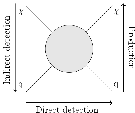
Figure 1.9 – Different processes for the detection of WIMP. The symbol \chi represents a dark matter candidate and the symbol q a SM particle. The circle corresponds to the interaction between these particles. From left to right, direct detection uses the scattering of WIMP on SM particles. From top to bottom, the annihilation of dark matter particles is used in indirect detection. From bottom to top, the production of dark matter particles is searched in colliders.
