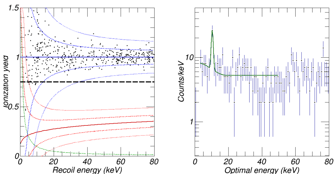
Figure 5.5 – Left: ionization yield as a function of the recoil energy (in keV) for fiducial events having an electronic recoil for FID803 detector in run309. The nuclear and electronic recoil bands are also drawn (in red and blue respectively). Right: spectrum of the optimal energy E_{opt} (in keV) as described by Eq.5.5. The tritium function described by Eq.5.11 is fitted on these data to determine the rate of this background for FID803 detector.
