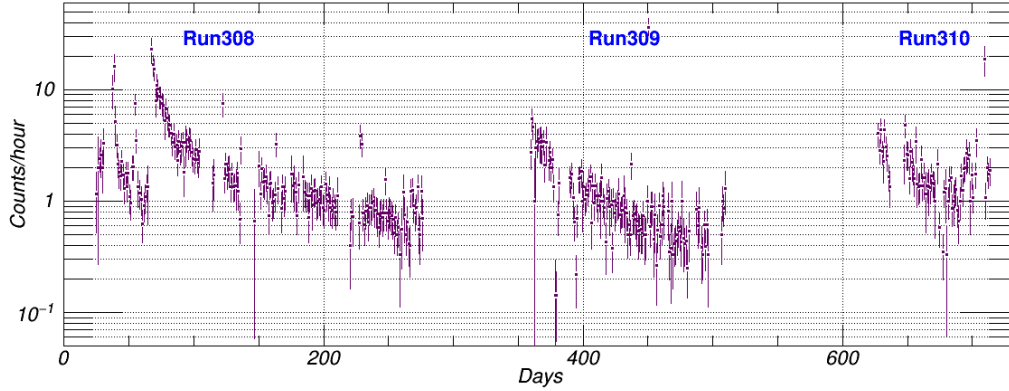
Figure 4.24 – Heat-only count rate since the beginning of the data taking for FID824 detector (which is in the cryostat since 2014, i.e run308) with phonon energy above E_{\text{phonon}}^{\text{min}} = 5 \text{ keV} .
