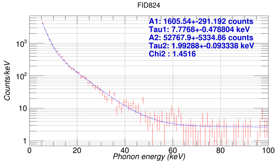
Figure 4.18 – Example of double exponential fit of the combined heat-only energy spectrum (run308, run309 and run310) for FID824 detector.
