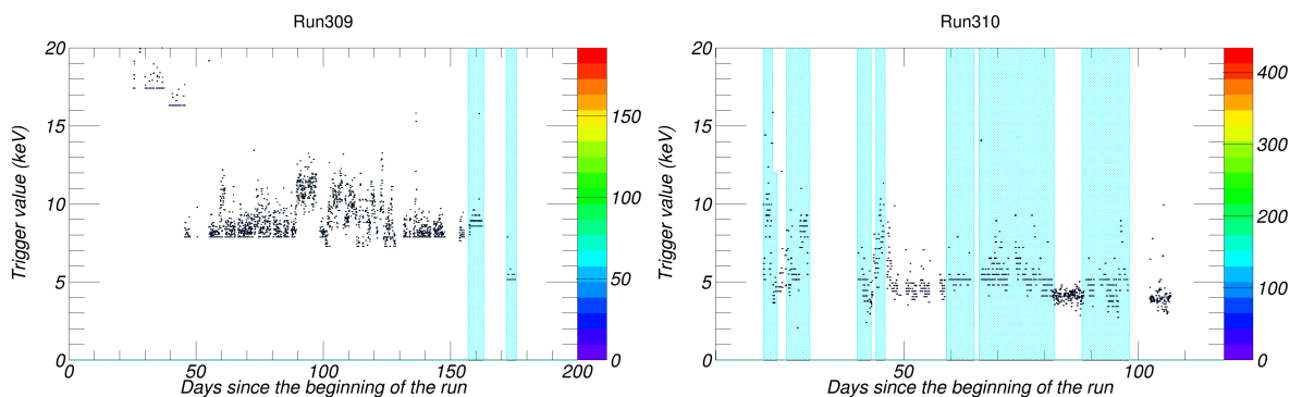
Figure 3.4 – Online trigger threshold as a function of the time of the cryorun, for run309 (left) and run310 (right). The cyan zones indicate time periods with high voltage bias for FID803 detector.
