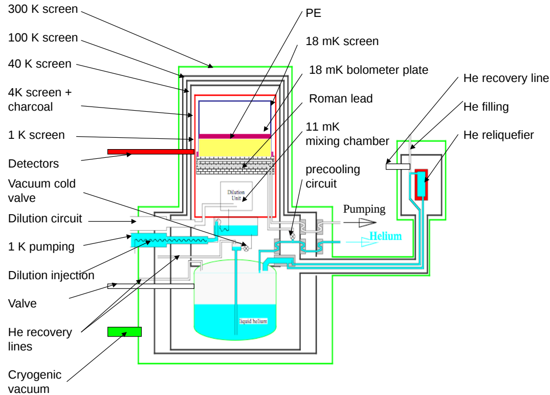
Figure 2.8 – Scheme of the EDELWEISS cryostat. The different screens corresponding to the 18 mK, 1 K, 40 K, 100 K and 300 K stage are represented.
