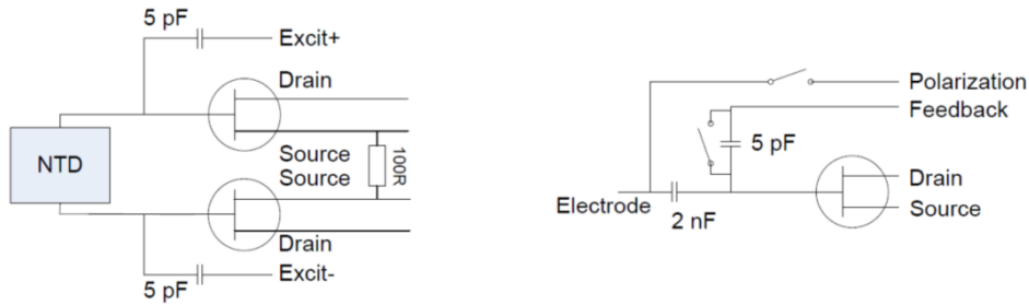
Figure 2.9 – Cold electronic readout for heat (left) and for ionization (right).
