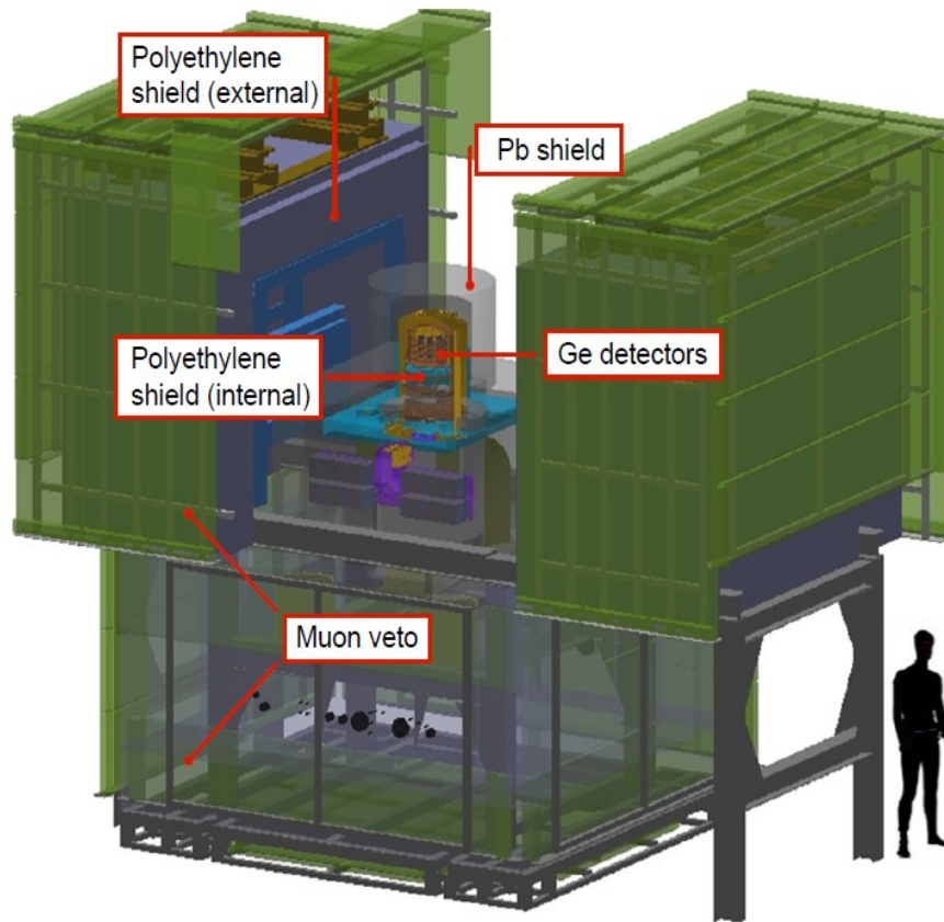
Figure 2.1 – Scheme of the EDELWEISS set-up. The muon veto (in green) is the outermost shell of the EDELWEISS shielding. PE (in violet) and lead (in gray) shields are installed between the muon veto and the cryostat (in orange).
