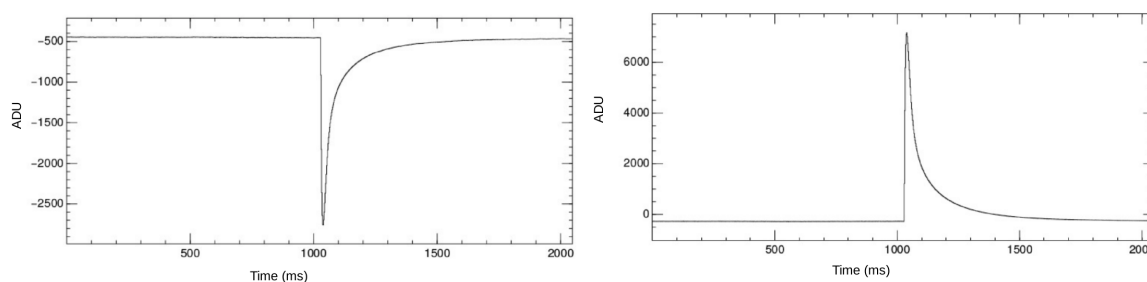
Figure 3.6 – Left: event measured by the NTD A. Right: same event measured by the NTD B. In both plots, the x-axis is in milliseconds and the y-axis in ADC units. The orientation of the pulse depends on the polarization sign imposed by the user.
