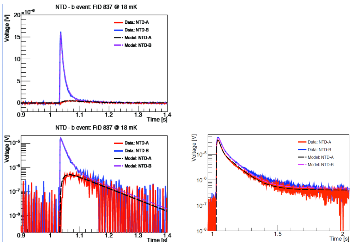
Figure 2.17 – Left: signal measured for an event occurring in one NTD (NTD B) with no signal in the other (NTD A). Top: linear scale. Bottom: log scale. Right: signal measured for an event occurring in the absorber and seen with nearly the same amplitude in both NTD. For all plots: in red, pulse recorded in the NTD A, in blue pulse recorded in the NTD B. Thermal model description of the response of each NTD are in black and magenta. In the two cases, the data and the model are in good agreement.
