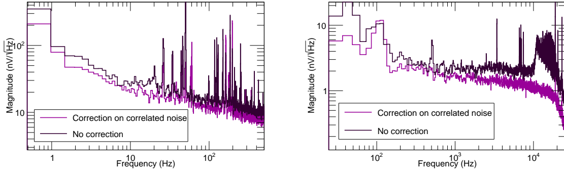
Figure 2.10 – Average noise amplitude (in nV/\sqrt{Hz} ) as a function of frequency of the ionization channel for an EDELWEISS detector. The black histogram corresponds to the noise before the correlated noise correction and the purple histogram to the noise after the correction. Left: frequencies below 500 Hz. Right: high frequency part.
