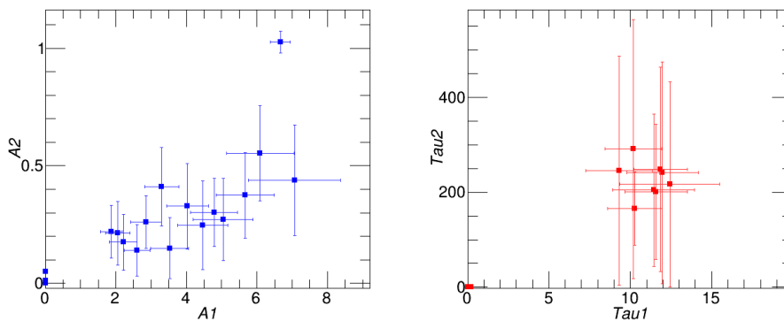
Figure 4.10 – Amplitude A_1 versus amplitude A_2 (left) and time constant \tau_1 versus time constant \tau_2 (right) for E_{\text{phonon}}^{\text{min}} = 10 \text{ keV} , obtained from fit results as presented in previous figures. A strong correlation is observed between the two exponentials.
