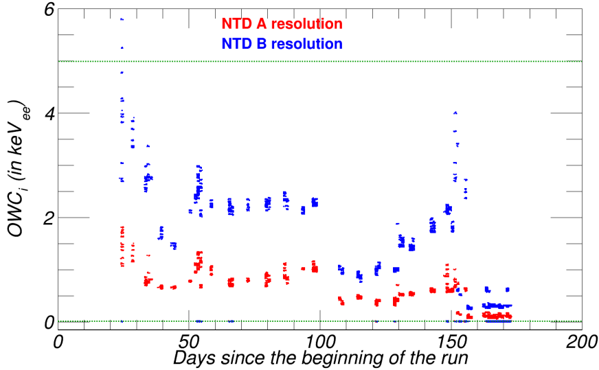
Figure 3.13 – Heat energy resolutions (FWHM) in \text{keV}_{ee} (NTD A in red, NTD B in blue) as a function of the time of the cryorun. The time selection quality cut of Eq.3.17 and Eq.3.18 removes 3% of the time, corresponding mostly to events above and below the interval between the two horizontal green dashed lines.
