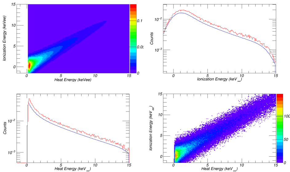
Figure 30 – Top, left: Probability Density Function corresponding to the neutron background in the parameter space (E_{ion}, E_{heat}) . Bottom, right: simulation of neutron events in the same parameter space. This figure allows to confirm that simulated data are in good agreement with the PDF. Top, right: ionization energy spectrum for fake data (in red) and providing from the PDF (in blue). Both are in excellent agreement. Bottom, left: heat energy spectrum for fake data (in red) and from the PDF definition (in blue), showing the same excellent agreement.
