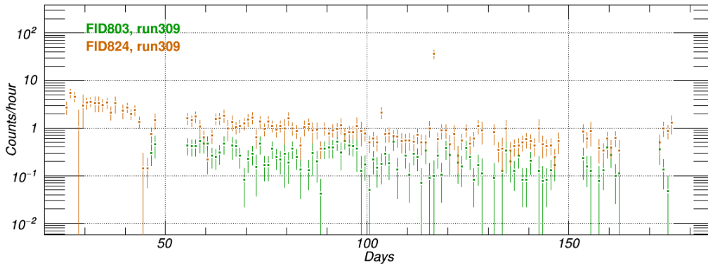
Figure 4.28 – HO rate for FID803 (in green) and FID824 (in orange) detectors in run309: FID824 has an amorphous layer of hydrogenated Ge ( \alpha\text{Ge} ) under its electrodes greater than FID803 but a lower HO count rate (with E_{\text{phonon}}^{\text{min}} = 10 \text{ keV} ).
