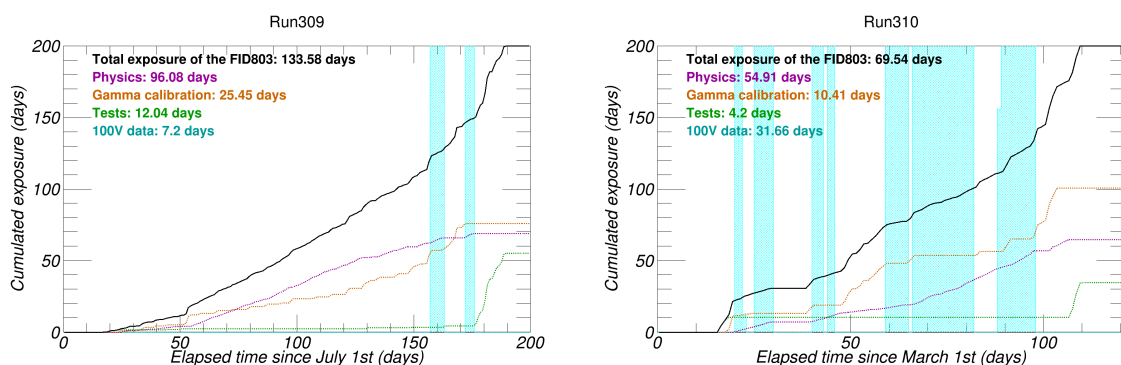
Figure 3.3 – Exposure of the data taking corresponding to run309 (left) and run310 (right) for FID803 detector. Calibration runs with a barium source exposure correspond to the orange curves. The magenta curves show the WIMP search data. The green curves correspond to runs dedicated to R&D purposes. The cyan zones indicate time periods with high voltage bias for FID803 detector.
