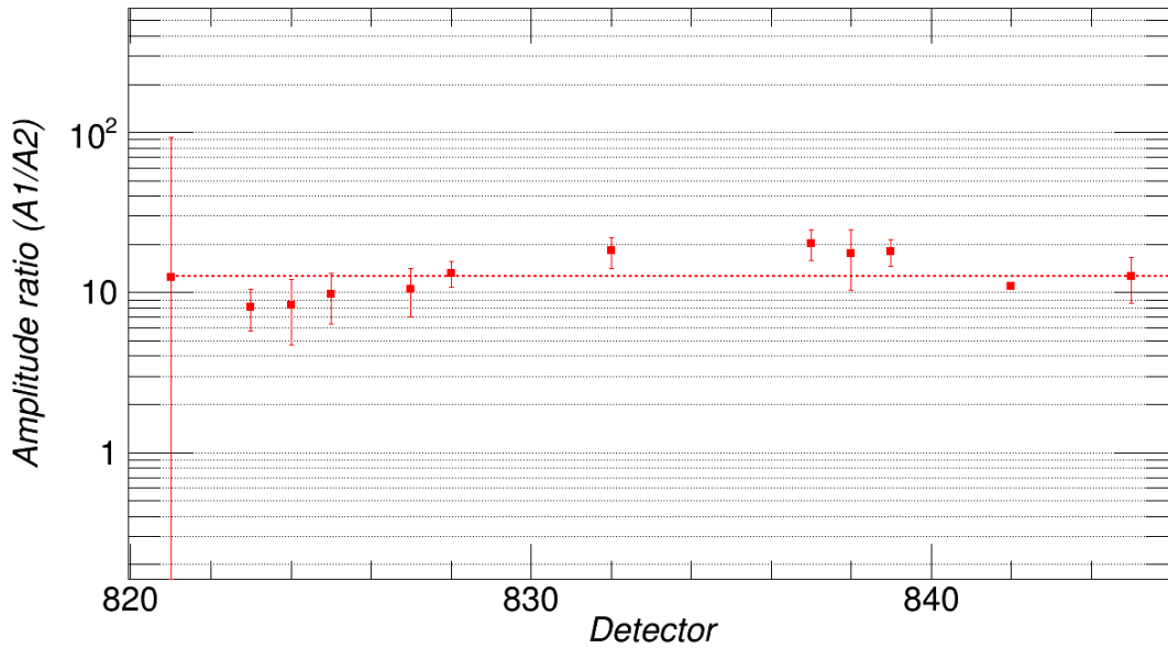
Figure 4.9 – Ratio of the amplitudes A_1 and A_2 of the two exponentials (Eq.4.4) as a function of the detector number, for E_{\text{phonon}}^{\text{min}} = 10 \text{ keV} . The average value of the amplitude is shown in red dashed line.
