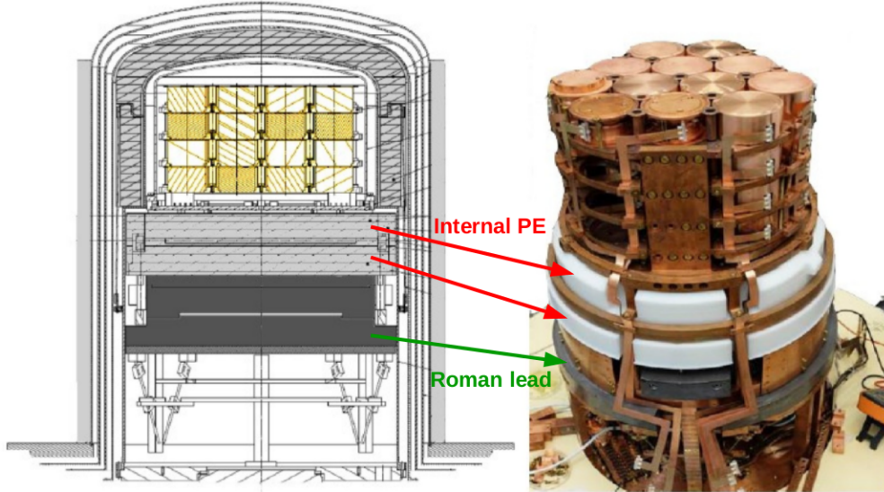
Figure 2.3 – Scheme of the upperpart of the cryostat and arrangement of detectors inside it. There is 12 towers, each tower can host up to 4 detectors. Internal polyethylene is visible in white (red arrows) in the right figure as well as the internal roman lead below PE (green arrow).
