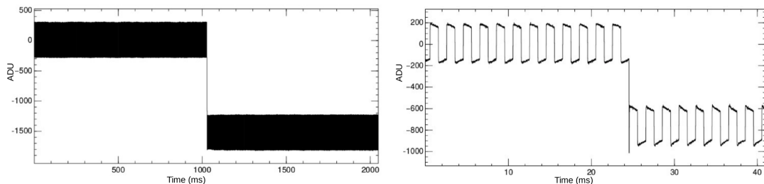
Figure 3.5 – Left: event measured by the electrode B, sampled at 1 kHz (so-called slow ionization). Right: same event measured by the electrode B, sampled at 100 kHz (fast ionization). The square-wave pattern visible on the 100 kHz ionization trace is induced by a cross-talk with the heat modulation. It is removed by subtracting the average pattern determined from the first half of the trace.
