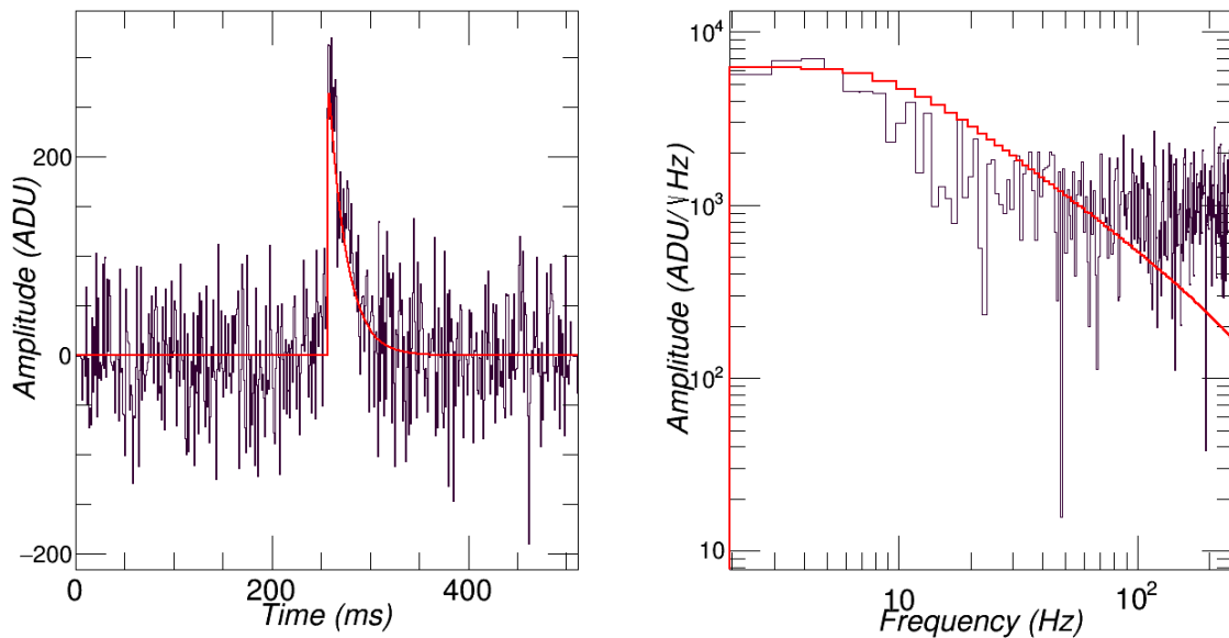
Figure 3.7 – Simulation of a recorded event and its template (in red) scaled with the amplitude resulting from the optimal filter (left) and their corresponding Fourier transforms (right).
