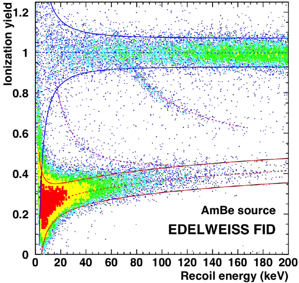
Figure 2.14 – Ionization yield as a function of the recoil energy for a FID800 detector from a neutron calibration using an AmBe source. The two red (blue) lines delimit the 90% C.L. nuclear (electronic) recoil band and the purple dashed lines correspond to inelastic scattering of neutrons on the first (13.28 keV) or the third (68.75 keV) excited state of ^{73}\text{Ge} .
