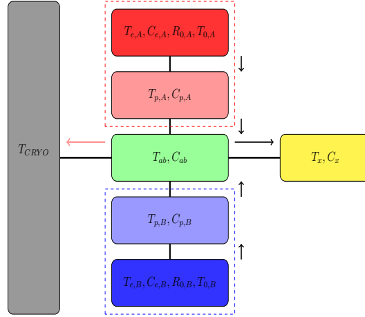
Figure 2.15 – Schematic of a FID800 detector. The gray block represents the temperature of the cryostat. Each NTD is represented by dashed block and have an electron bath and a phonon bath. The absorber bath is represented in green. Each element has a characteristic temperature T as well as a heat capacity C . A seventh element (in yellow) with a heat parasitic capacitance C_x has been required to fit correctly data.
