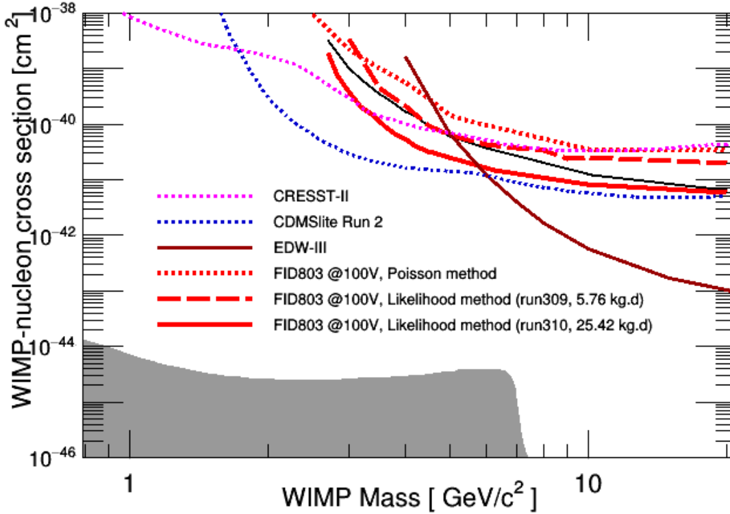
Figure 5.22 – WIMP-nucleon cross-section as a function of the WIMP mass. The red curve is the final limit obtained from this work and corresponds to the dataset of the FID803 detector in run310, with an exposure of 25.42 kg.day in high-voltage mode. The previous limits obtained for the same detector in run309 with the statistical method and the Likelihood analysis are also shown (red dotted curve and red dashed curve respectively) for comparison. The magenta curve corresponds to the CRESST results [54], the blue curve to CDMSlite Run2 [51] and the dark red curve to the previous EDELWEISS-III limit [92].
