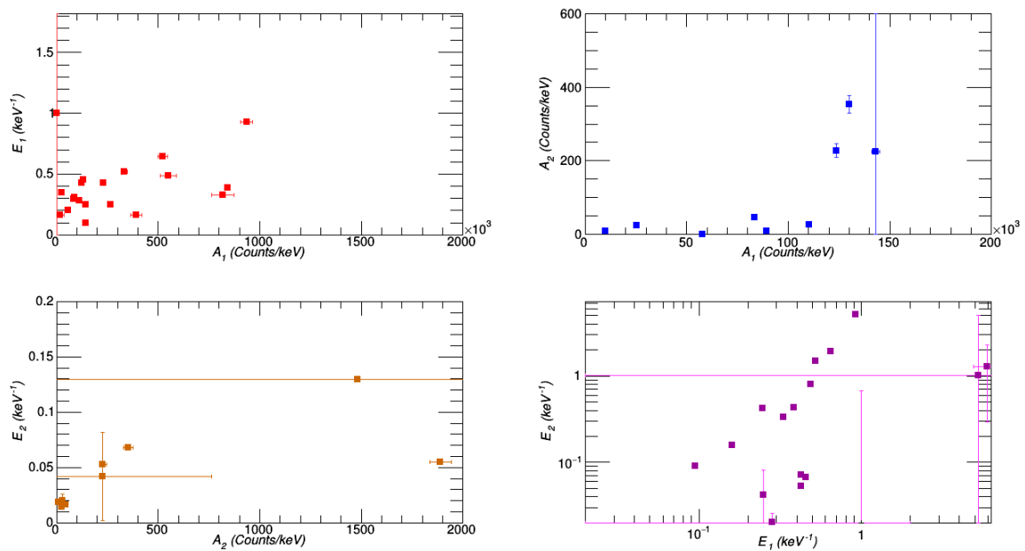
Figure 4.21 – Top, left: energy constant E_1 as a function of the amplitude A_1 . Bottom, left: energy constant E_2 as a function of the amplitude A_2 . Top, right: amplitude A_2 as a function of the amplitude A_1 . Bottom, right: energy constant E_2 as a function of the energy constant E_1 . A correlation is visible between these two parameters.
