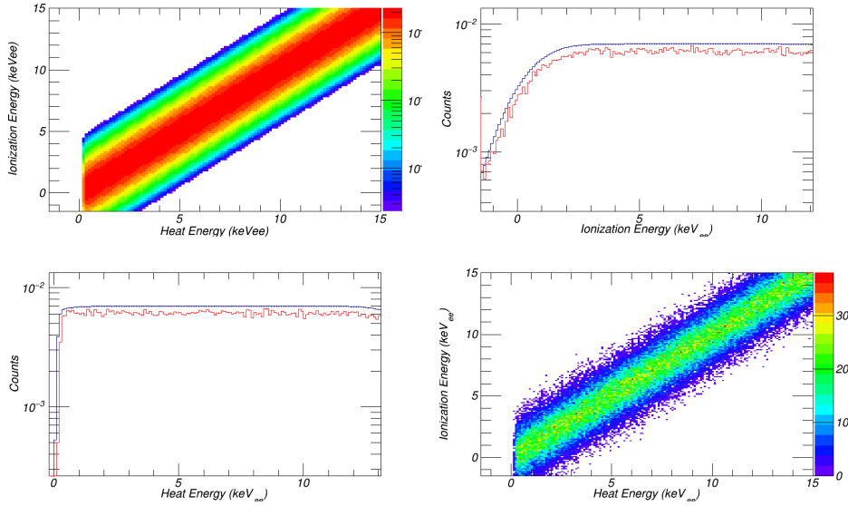
Figure 25 – Top, left: Probability Density Function corresponding to the \gamma -background in the parameter space ( E_{ion}, E_{heat} ). Bottom, right: simulation of \gamma -events in the same parameter space. This figure allows to confirm that simulated data are in good agreement with the PDF. Top, right: ionization energy spectrum for fake data (in red) and providing from the PDF (in blue). Both are in excellent agreement. Bottom, left: heat energy spectrum for fake data (in red) and from the PDF definition (in blue). The same agreement is observed.
