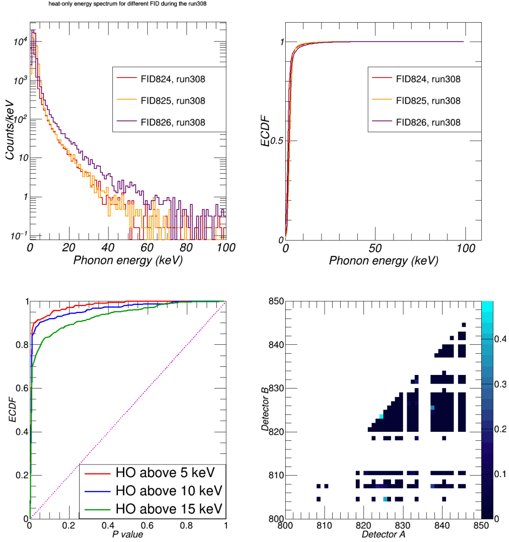
Figure 4.16 – Top, left: heat-only energy spectra of FID824 (red), FID825 (orange) and FID826 (magenta) detectors in run308. Top, right: ECDF of these three distributions. The main difference between these distributions corresponds to the phonon energy range E_{\text{phonon}} \in [0; 20] keV. Bottom, left: ECDF as a function of the p -values between different detectors with E_{\text{phonon}}^{\text{min}} equal to 5 keV (in blue), 10 keV (in red) and 15 keV (in green). The dashed violet line is the linear function ( f(x) = x ). It allows to conclude that the heat-only energy spectra are different whatever the detector independently of the E_{\text{phonon}}^{\text{min}} value. Bottom, right: p -values in the space of parameters ( \text{Detector}_A, \text{Detector}_B ), using E_{\text{phonon}}^{\text{min}} = 10 keV. The blue shades correspond to the obtained p -values (between 0 and 1). It is used to verify if a group of detectors show the same heat-only model.
