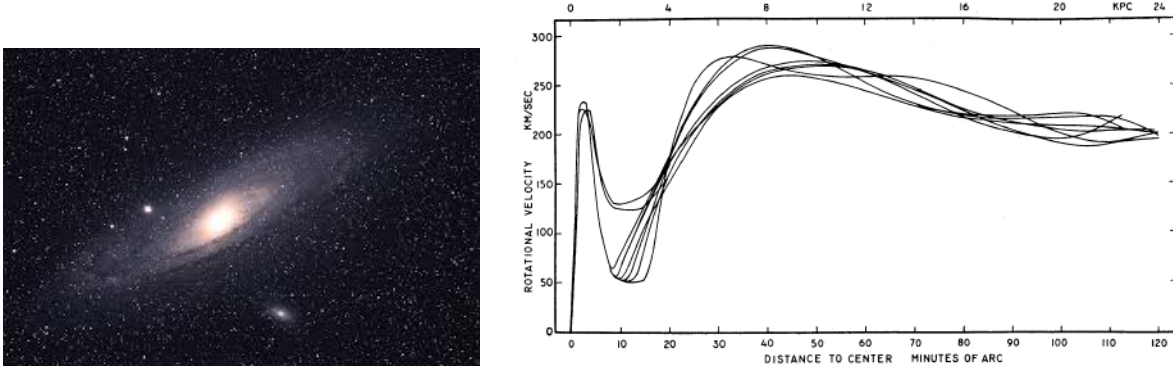
Figure 1.1 – Left: Andromeda’s galaxy (M31). Right: rotational curves measured by Rubin [6]. The velocity doesn’t decrease with the radius after exceeded the optical radius of the galaxy as it was expected. A missing mass could explain this phenomena.
