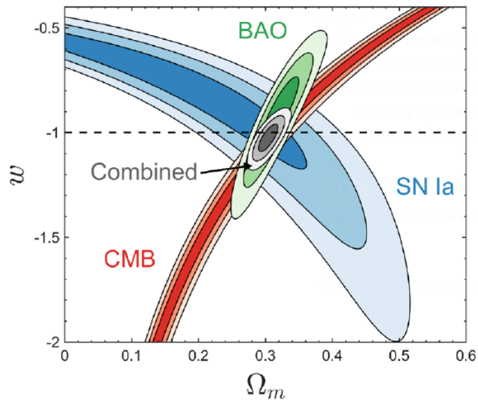
Figure 1.6 – Constraints on cosmological parameters using SNIa (in blue), BAO (in green) and CMB (in red) observations. It is expressed as a function of the matter density \Omega_m and the equation of state parameter w . Contours correspond to 68.3 % C.L., 95.4 % C.L. and 99.7 % C.L. of the analysis with the assumption of a flat Universe [17].
