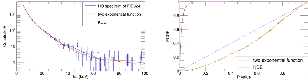
Figure 4.22 – Left: energy spectrum of FID824 detector for all heat-only events (run308, 309 and 310). Blue dots are data. In orange, the fit with two exponentials. In magenta, the Kernel function estimator. Right: comparison between the heat-only energy spectrum and its modelization with two exponentials (in orange), comparison between the heat-only energy spectrum and its Kernel estimator (in magenta). Both comparisons are realized using the Kolmogorov-Smirnov test.
