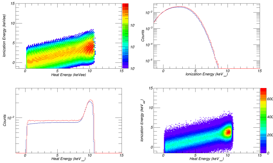
Figure 29 – Top, left: Probability Density Function corresponding to the ^{206}\text{Pb} background in the parameter space (E_{ion}, E_{heat}) . Bottom, right: simulation of ^{206}\text{Pb} events in the same parameter space. This figure allows to confirm that simulated data are in good agreement with the PDF. Top, right: ionization energy spectrum for fake data (in red) and providing from the PDF (in blue). Both are in excellent agreement. Bottom, left: heat energy spectrum for fake data (in red) and from the PDF definition (in blue), showing the same excellent agreement.
