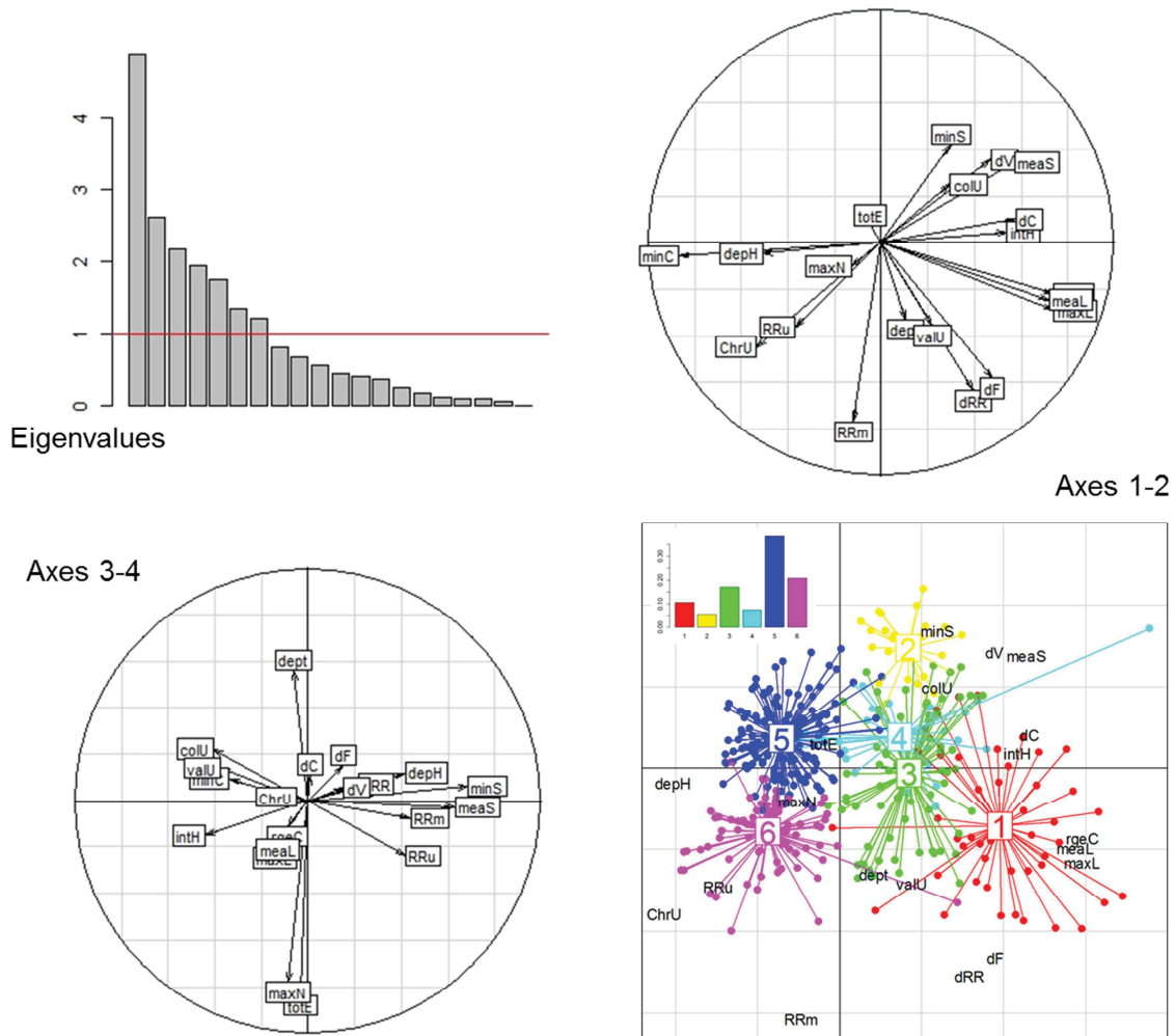
282 283 Figure 3: PCA analysis with a) histogram of the eigenvalues on the upleft ; b) correlation circle for 284 the two first axes on the upright ; c) correlation circle of the third and fourth axes on the 285 bottomleft ; d) projection of the soils on the the first axes on the bottomright (numbers and colors 286 indicate the different clusters obtained by HC – and the histogram indicates the frequency of the 287 clusters)
