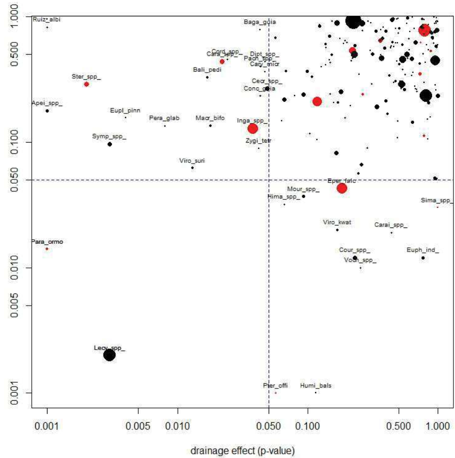
435 Figures 8: Representation of the significance of the soils and landscapes effects for the 199 species or group of species (SGS) available in the dataset. The 436 199 SGS are plotted regarding the p-value of the anova-like tests. Red plots indicate SGS which abundances are also significantly influenced by landscape. 437 The top figure indicates the results obtained when effects are tested independently. The down figure indicates the results obtained when landscapes 438 effects and soil effects are tested together including site-effects.
