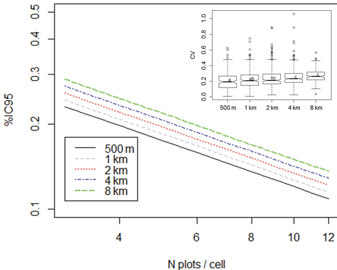
300 Figure 4: Estimation of coefficient of variation and confidence interval of local mean according 301 to grid resolution. 302 Inset boxplot shows CV of local biomass estimates according to grid resolution. Main part shows the 303 fitted values confidence interval of the local mean according to the model \log(\%IC_{95}) = -0.8155 - 304 0.54151 * \log(N) + 0.08024 * \log(R) from N=3 to 12 and R = 0.5 km to 8 km. 305
