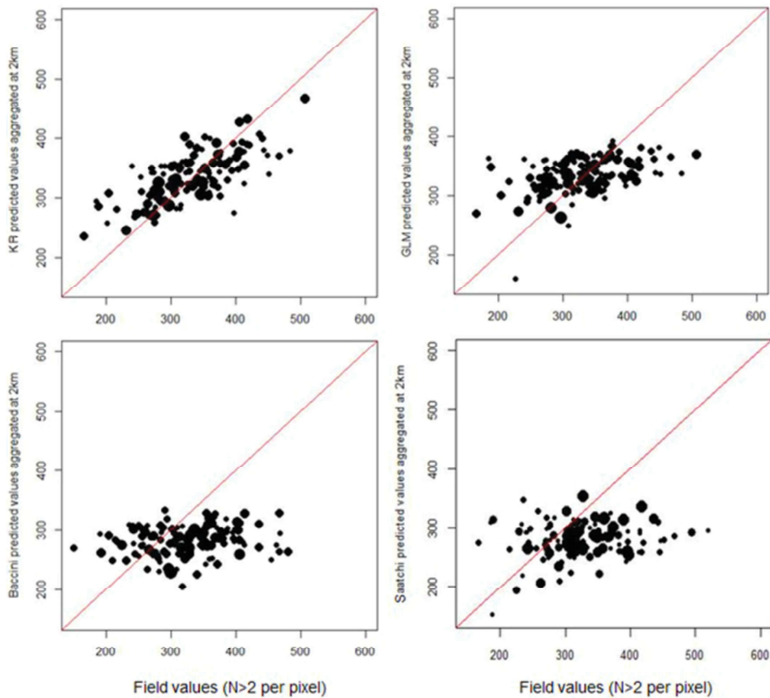
379 380 Figure 8: Comparison of validation data with AGB values predicted by the different maps at 2- 381 km resolution . 382 Aboveground biomass (AGB) values at cell level for the validation set of plots are compared to the 383 values predicted by the different maps at 2-km resolution : from the top left to the bottom right - KR, 384 GLM, Baccini [15] and Saatchi [16]. The red line indicates the 1:1 relationship (expected slope). The 385 size of the circles indicates the number of validation plots for each cell (from 3 for the smallest to 12 386 for the biggest).
