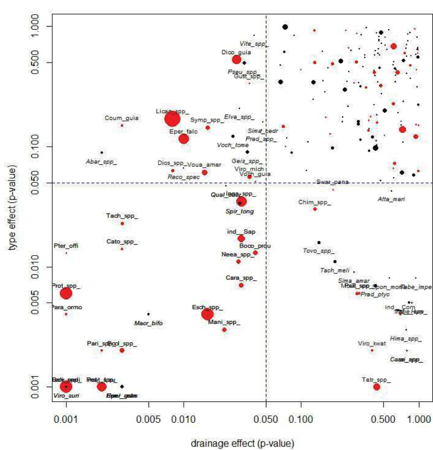
435 Figures 8: Representation of the significance of the soils and landscapes effects for the 199 species or group of species (SGS) available in the dataset. The 436 199 SGS are plotted regarding the p-value of the anova-like tests. Red plots indicate SGS which abundances are also significantly influenced by landscape. 437 The top figure indicates the results obtained when effects are tested independently. The down figure indicates the results obtained when landscapes 438 effects and soil effects are tested together including site-effects.
