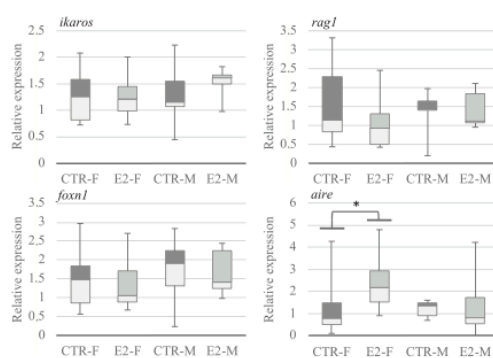
Fig. 3. Relative expression of thymic function-related genes, ikaros , rag1 , foxn1 and aire , in the thymus of sea bass, Dicentrarchus labrax , in females (F) and males (M) of E2-exposed (E2) and control (CTR) fish. Relative expression-levels are represented by box-and-whisker plots. The horizontal line inside each box indicates the median, top lines of the box are the 25 and 75 percentiles and the whisker limits depict extreme values. *, significantly different at p = 0.007 (Mann-Whitney U test).
