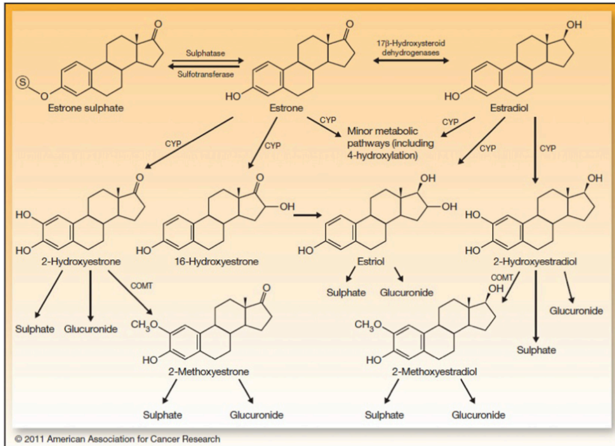
Figure 10: Endogenous oestrogen metabolism in human. Several cytochrome P450 enzymes such as CYP1A, CYP1B1, and CYP2A2 add hydroxyl group (-OH) to form different catechol oestrogens. Afterwards before excretion, catechol oestrogens are conjugated with sulfate or glucuronide acid or methylated to methoxyoestrogens by the catechol-O-methyltransferase (COMT). From Samavat and Kurzer (2015).
