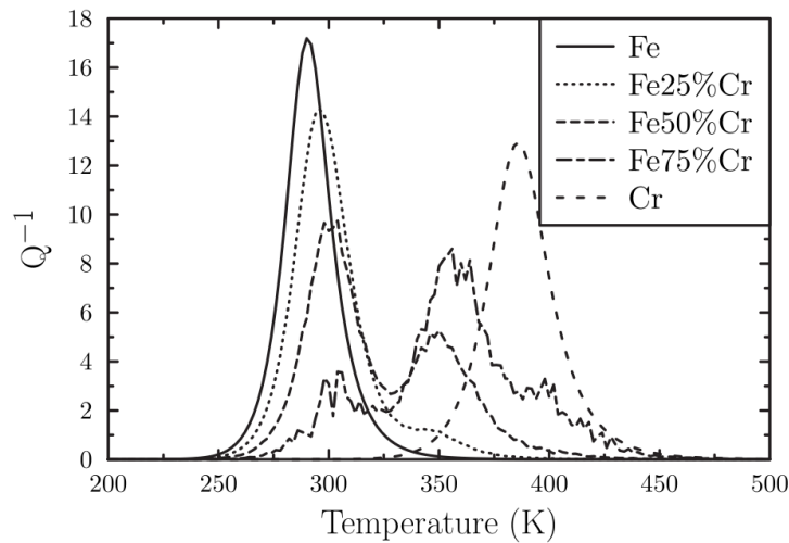
Figure 25: Calculated Snoek peak by Sandberg et al. [17].
