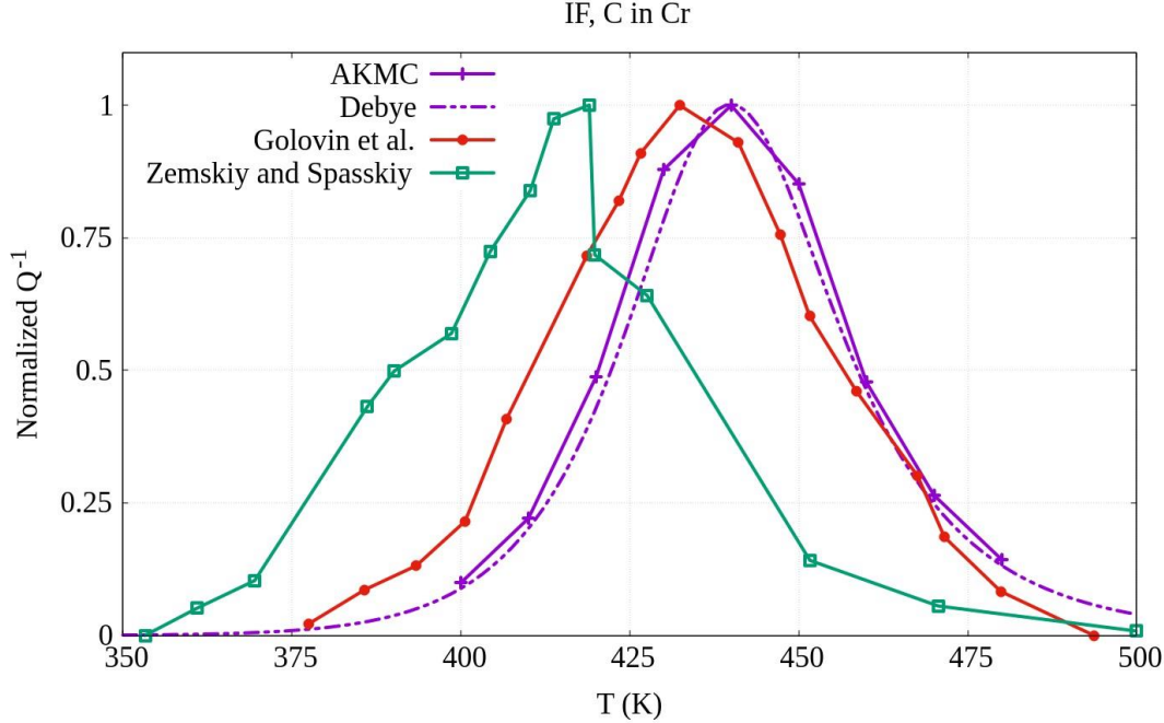
Figure 18: The Snoek peak in Cr-0.033%C, with f = 1 Hz and \sigma_0 = 0.131 GPa. Comparison between AKMC simulations, the Debye equation and the experimental results from Golovin et al. [67] and Zemskiy and Spasskiy [63].
