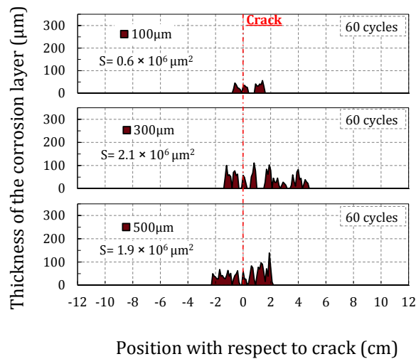
Figure I-27 : Corrosion products repartition obtained on specimens showing different residual crack openings and oriented horizontally with respect to rain
