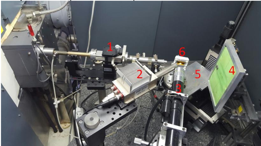
Figure I-1: Photograph of the assembly anode/XRD developed in LAPA (CEA/DSM/IRAMIS/SIS2M/LAPA) Legend: 1) X-Ray (Mo, \lambda K\alpha = 0,709 \text{ \AA} ), 2) X-Fluorescence detector 3) Optical microscope, 4) image plate (Fuji), 5) moving stage, 6) sample
