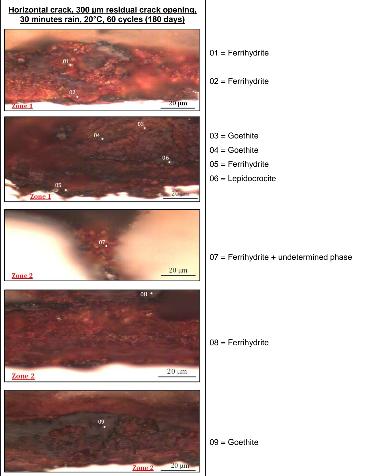
Figure 5-8: Corrosion layer observed at steel/mortar interfaces located far from the crack and deep in the crack in specimens having 300 μm crack oriented horizontally with respect to rain
