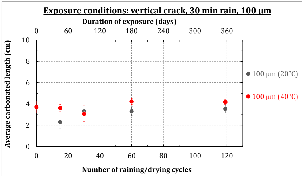
Figure I-71: Evolution of the carbonated steel/mortar interface length in specimens exposed to different temperatures (100 μm)
