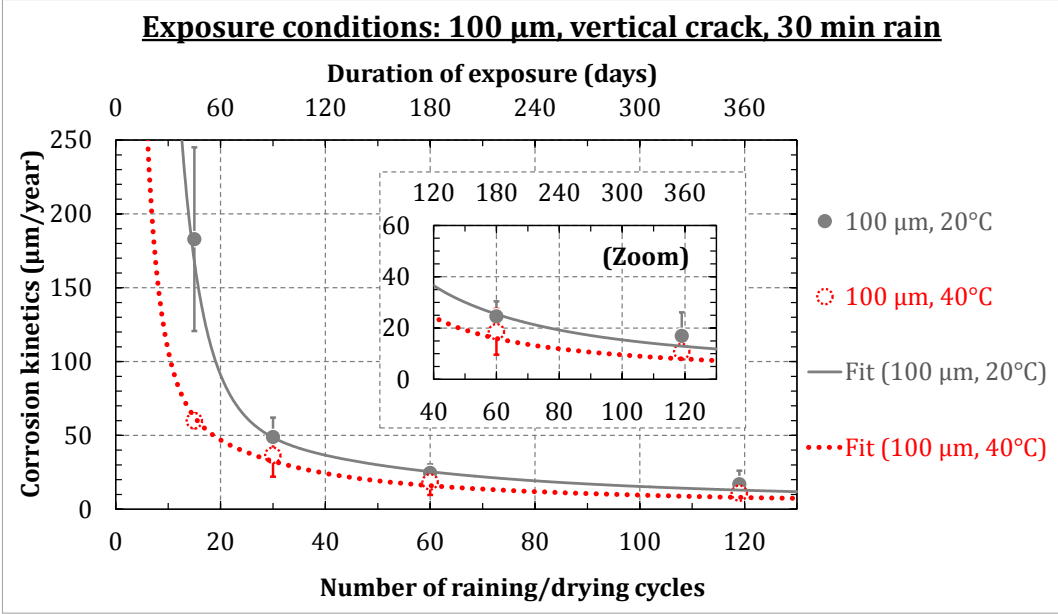
Figure 5-29: Corrosion rate evolution in specimens subjected to different temperatures during the corrosion test and showing 100 µm residual crack opening
