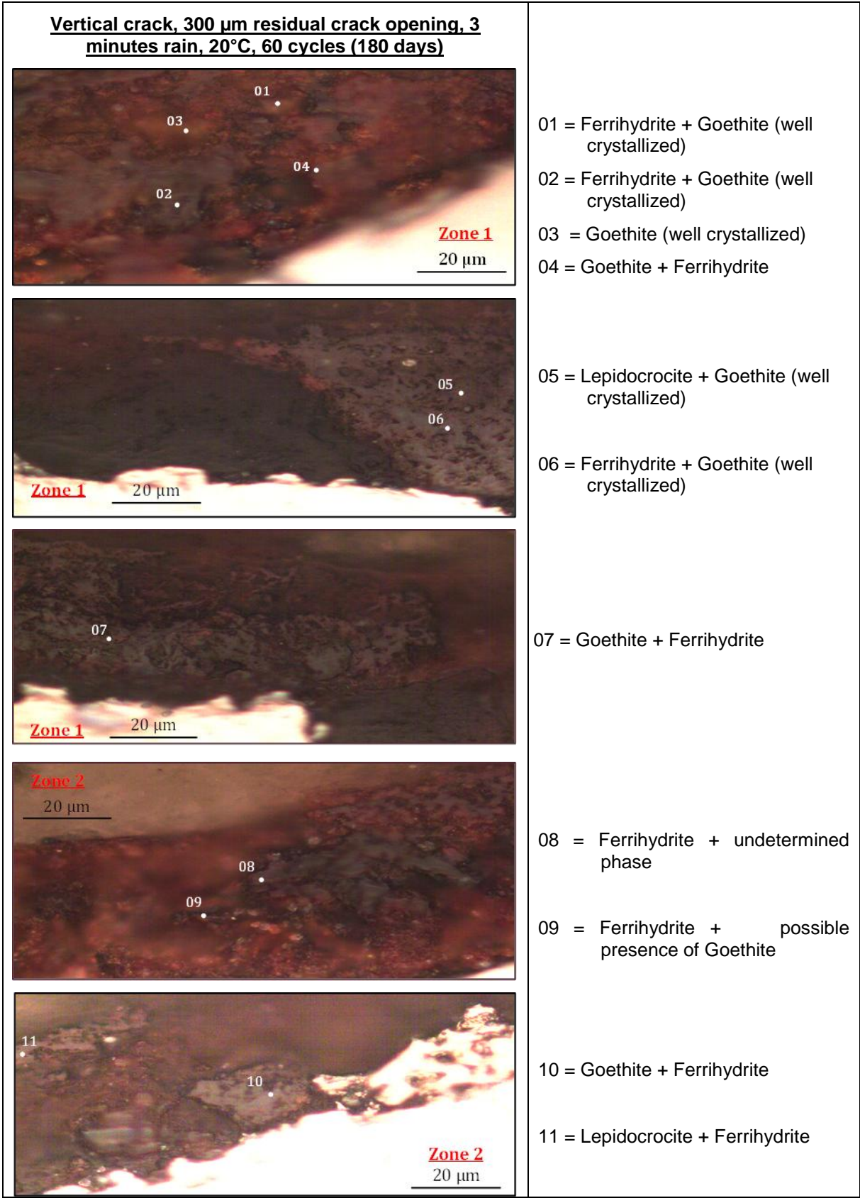
Figure 5-18: Corrosion layer observed at steel/mortar interfaces located far from the crack and deep in the crack in specimens having 300 μm residual crack width and exposed to 3 minutes rain in each raining/drying cycle.
