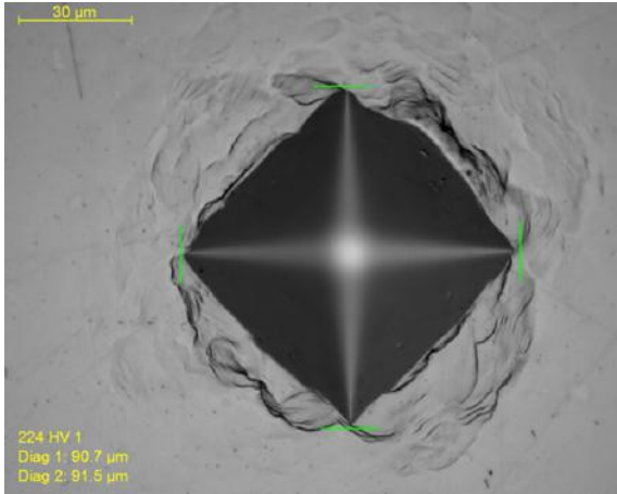
Figure 2-6: square footprint on the steel surface
