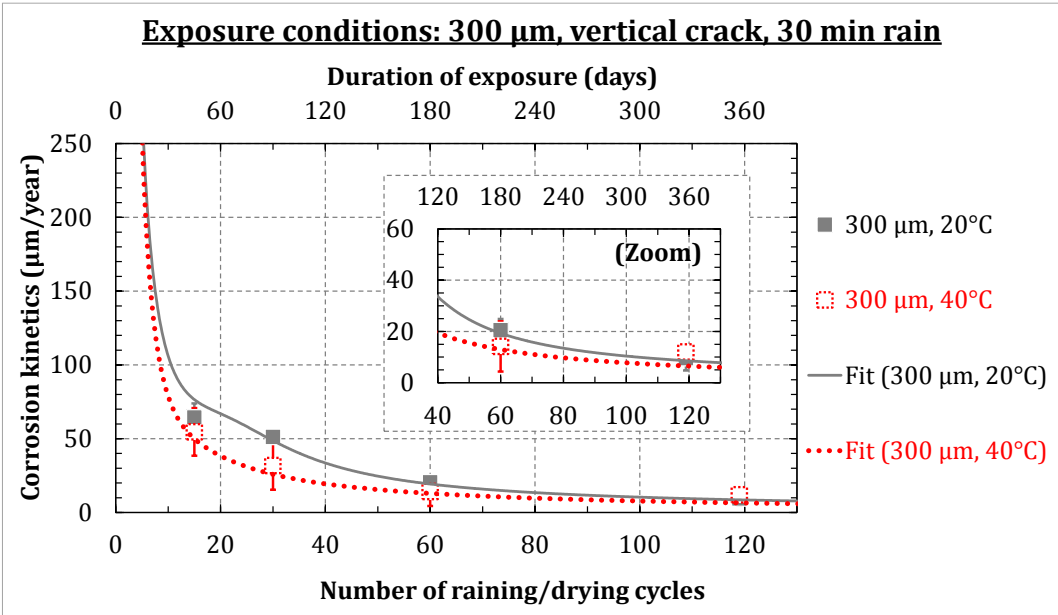
Figure 5-30: Corrosion rate evolution in specimens subjected to different temperatures during the corrosion test and showing 300 µm residual crack opening
