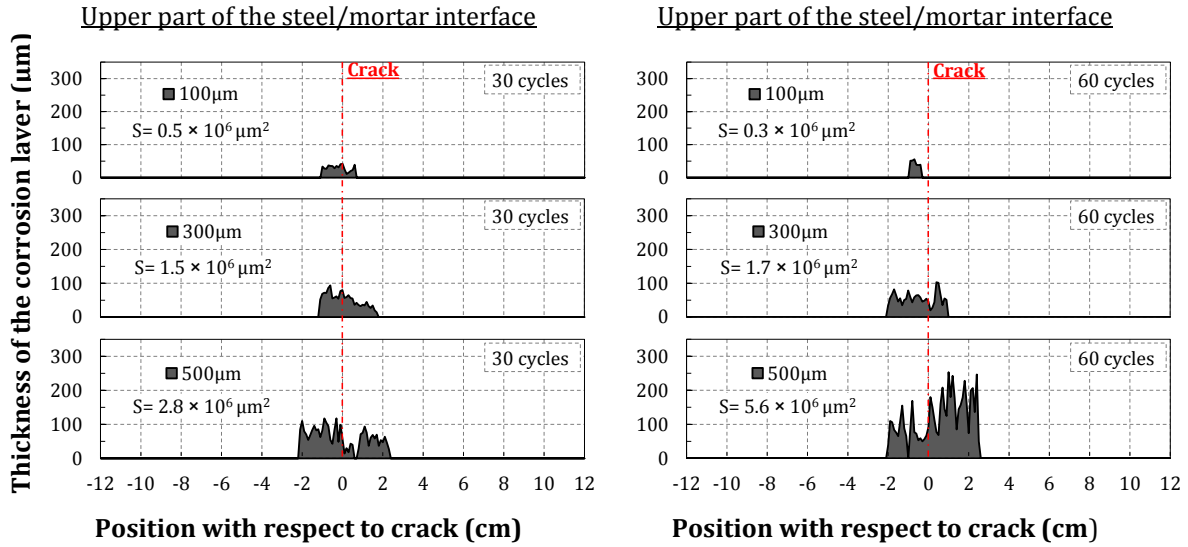
Figure 4-5 : Corrosion products repartition obtained on specimens showing different residual crack openings (optical microscopy)
