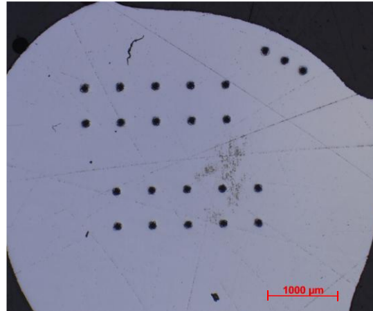
Figure 2-7: steel hardness measurements location
