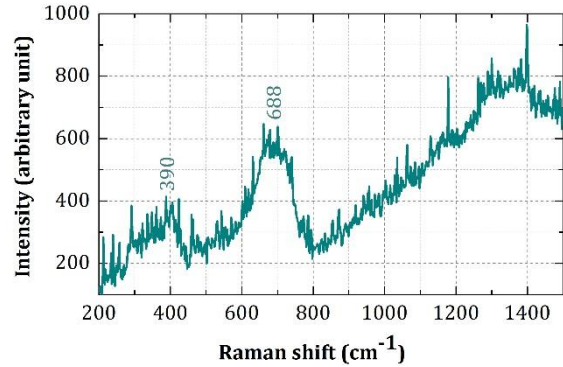
Goethite (Mortar (CEM I + slag)) (Vertical crack, 300 µm, 30 min rain, 20°C, 60 cycles, 180 days, zone 2, 04)
