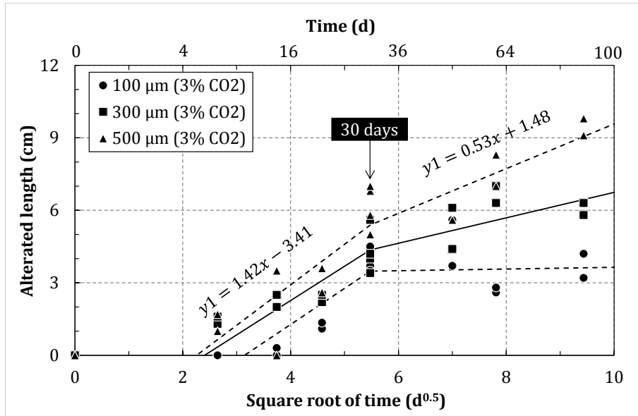
Figure 3-13: Carbonation length along the steel/mortar interface with respect to square root of time for three residual crack openings (100; 300; 500 μm)
