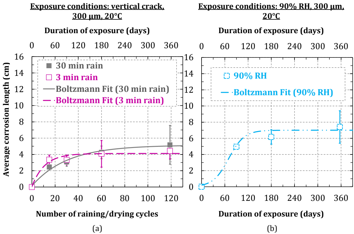
Figure 5-11: Corrosion length evolution with respect to raining/drying cycles and rain durations (visual inspection)
