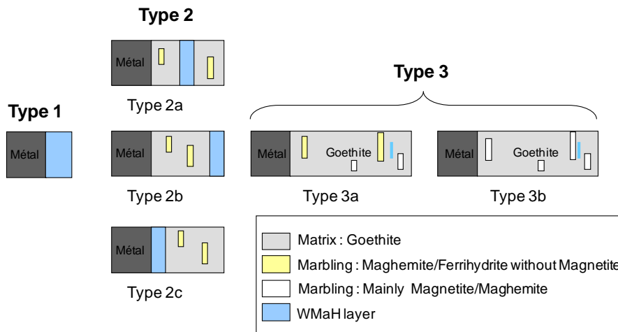
Figure 1-15: Hypothetical scenarios for the formation of long-term corrosion by carbonation patterns [59]
