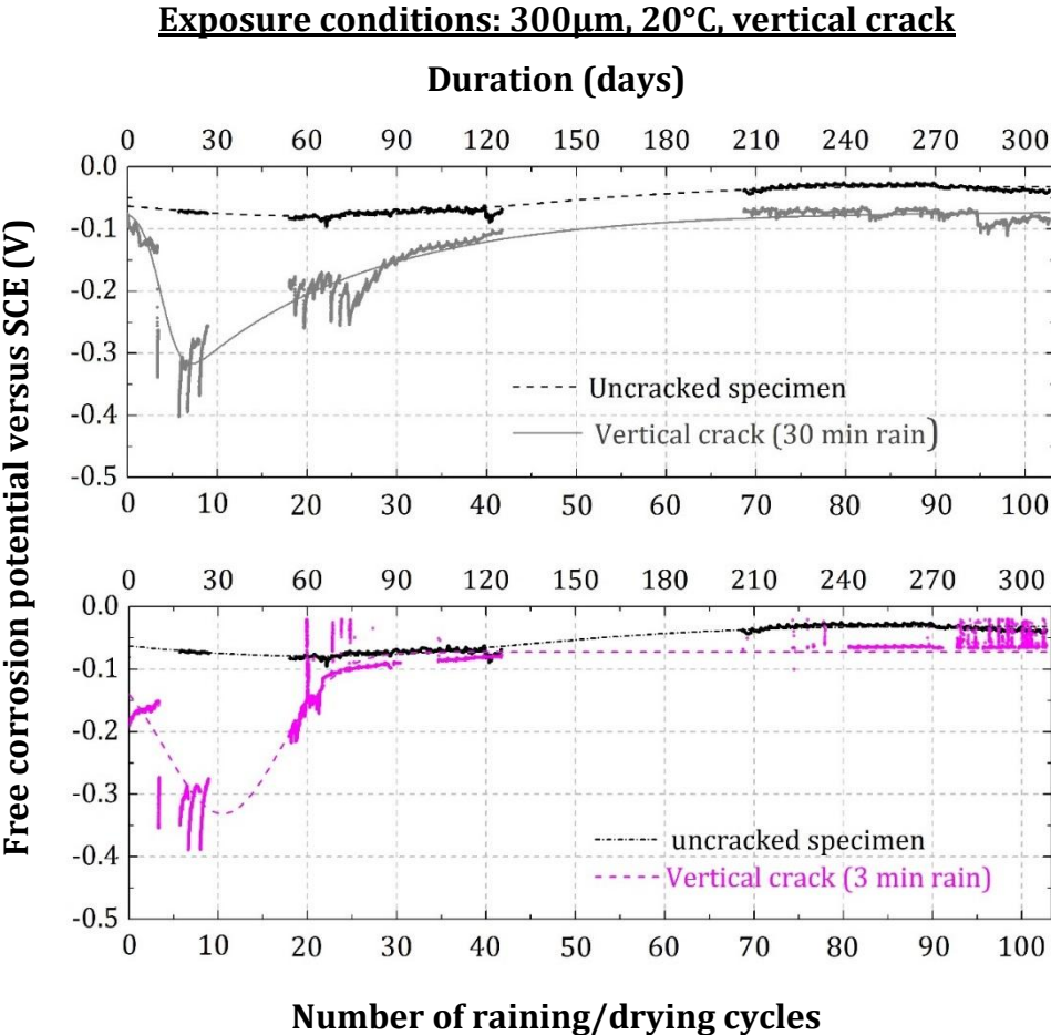
Figure 5-17: : Free corrosion potential (versus SCE) measured in specimens showing 300 µm residual crack width and exposed to different raining durations
