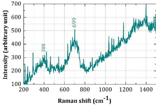
Ferrihydrite (Mortar (CEM I + slag)) (Vertical crack, 300 µm, 30 min rain, 20°C, 60 cycles, 180 days, zone 1, 03)
