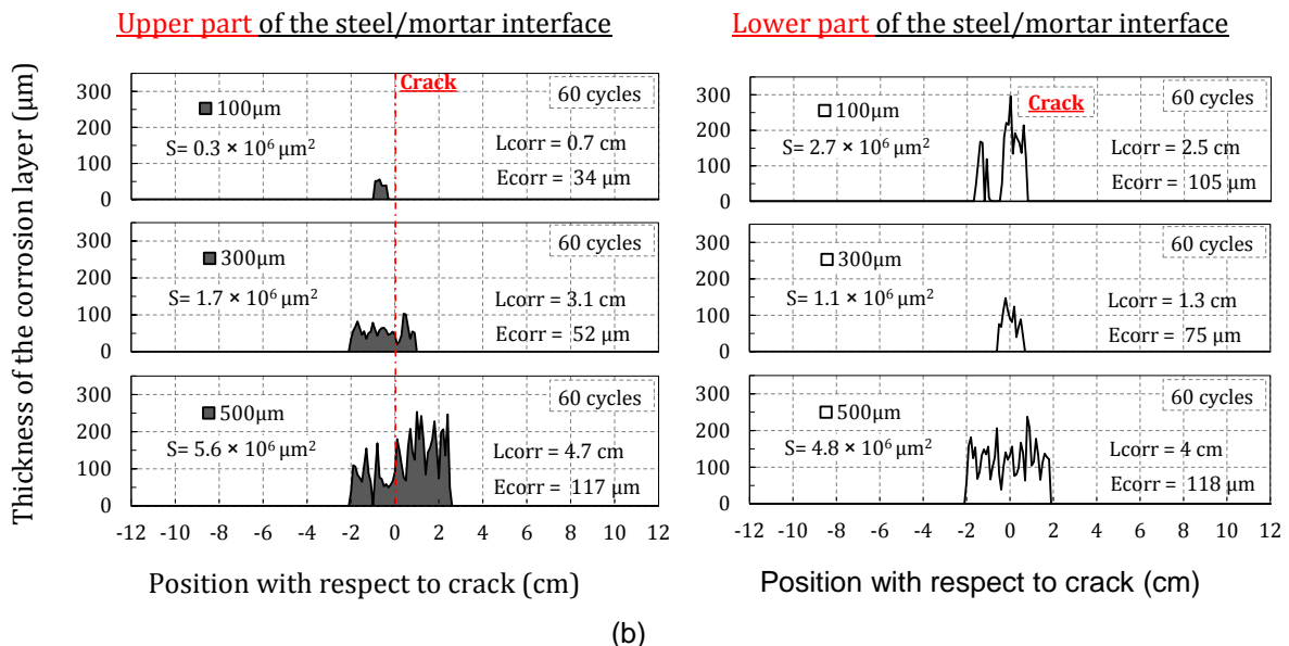
Figure 7-1 : Corrosion products repartition on the upper and the lower steel/mortar interfaces of specimens corroded in the reference test 5
