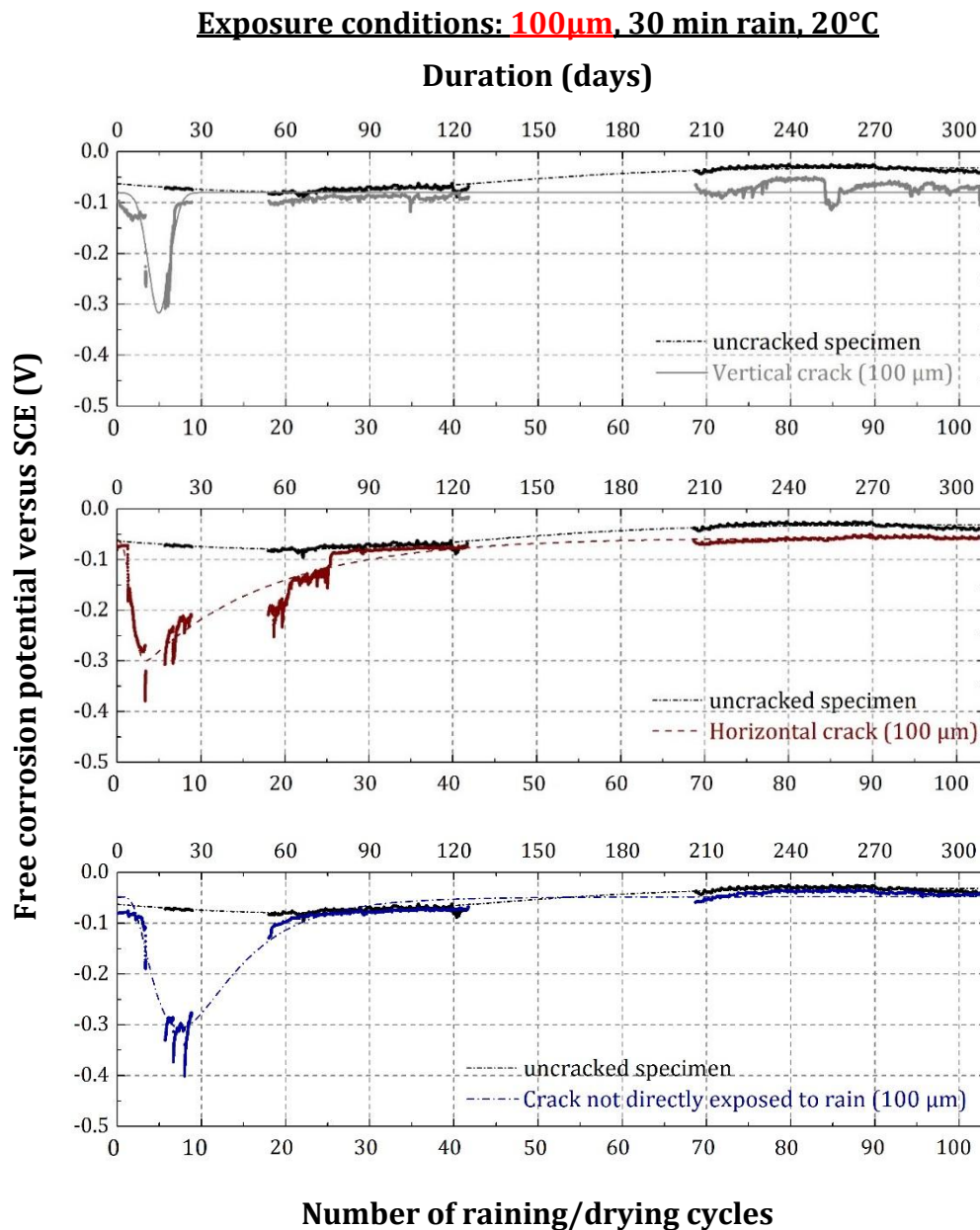
Figure 5-6: Free corrosion potential (versus SCE) measured in specimens showing 100 \mu\text{m} residual crack exposed in different directions with respect to rain
