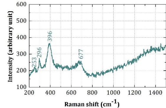
Goethite + Ferrihydrite (Mortar (CEM I + slag)) (Vertical crack, 300 µm, 30 min rain, 20°C, 60 cycles, 180 days, zone 2, 06)
