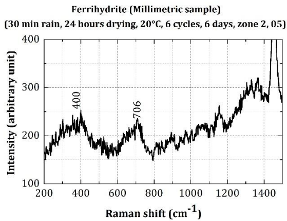
Figure I-59 : All the Raman spectra of corrosion products obtained on millimetric samples after 6 wetting/drying cycles
