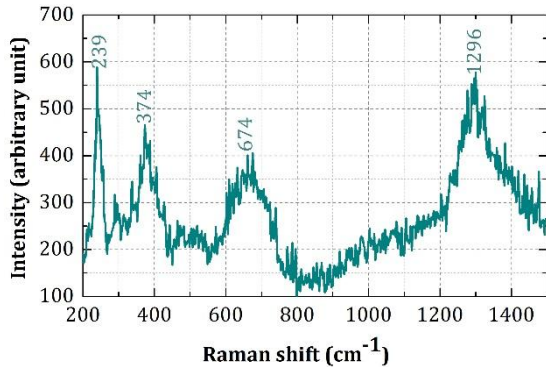
Goethite + Ferrihydrite (Mortar (CEM I + slag)) (Vertical crack, 300 µm, 30 min rain, 20°C, 60 cycles, 180 days, zone 2, 07)
