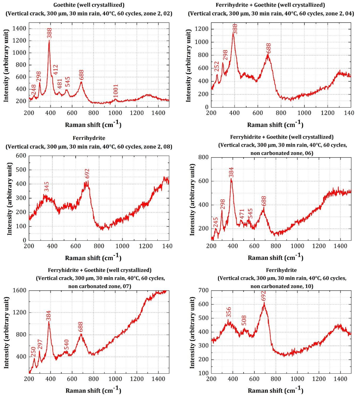
Figure 5-32: Some Raman spectra of corrosion products obtained on specimens having 300μm residual crack width corroded at 40°C under raining/drying cycles of 30 minutes rain each.
