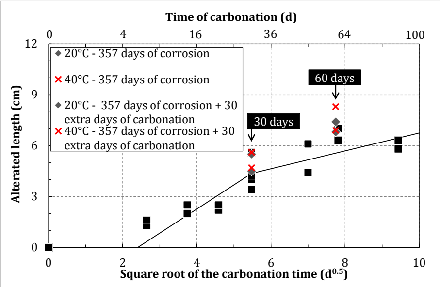
Figure 5-37: Evolution of the carbonation length along the steel/mortar interface with respect to the carbonation duration at 3%CO 2 of specimens showing 300 μm residual crack opening.
