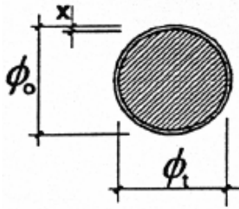
Figure 1-30: Residual reinforcing bar section for homogeneous corrosion [67]
