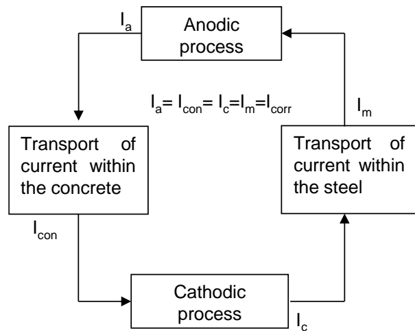
Figure 1-14: Electrochemical mechanism of steel corrosion in concrete (in [64])
