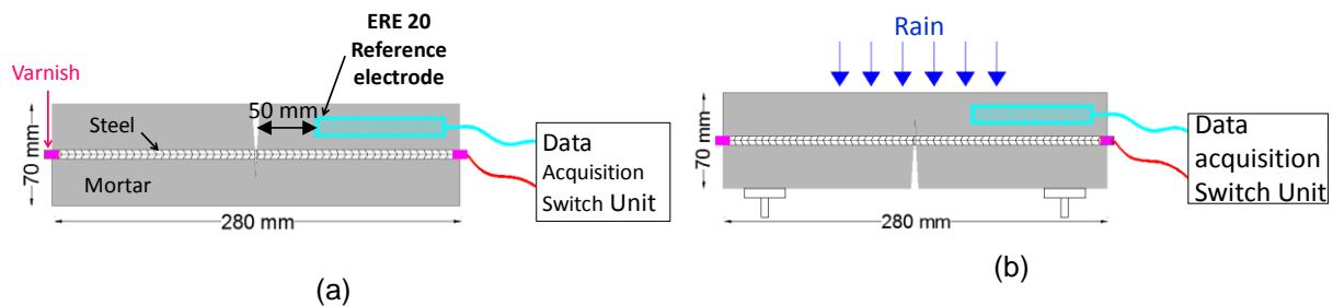
Figure 2-57: Electrochemical measurement
