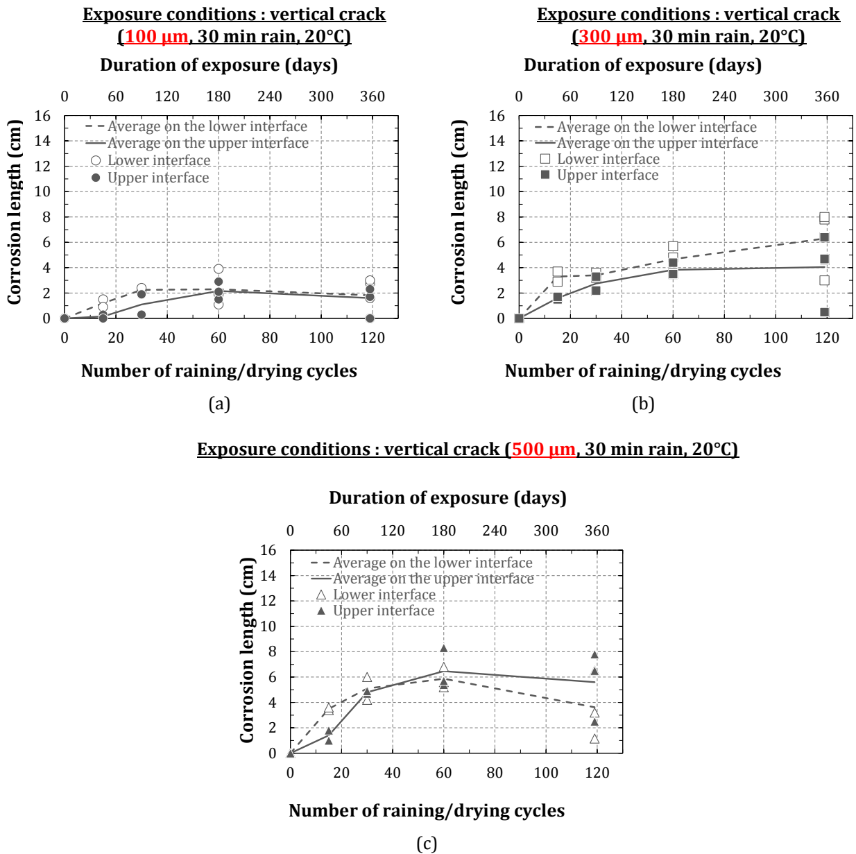
Figure 4-1 : Corrosion length along the upper and the lower steel/mortar interfaces measured during the visual inspection (naked eye)
