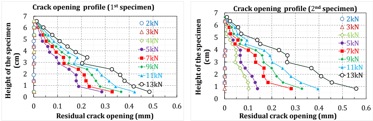
Figure 3-4: Crack opening profile over the entire height of two specimens
