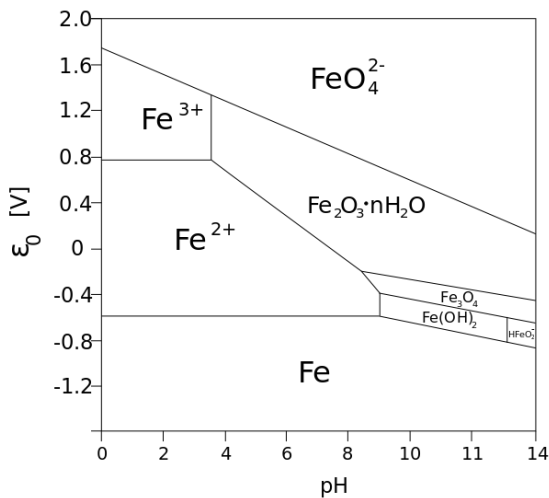
Figure 1-13: Pourbaix diagram for steel [63]
