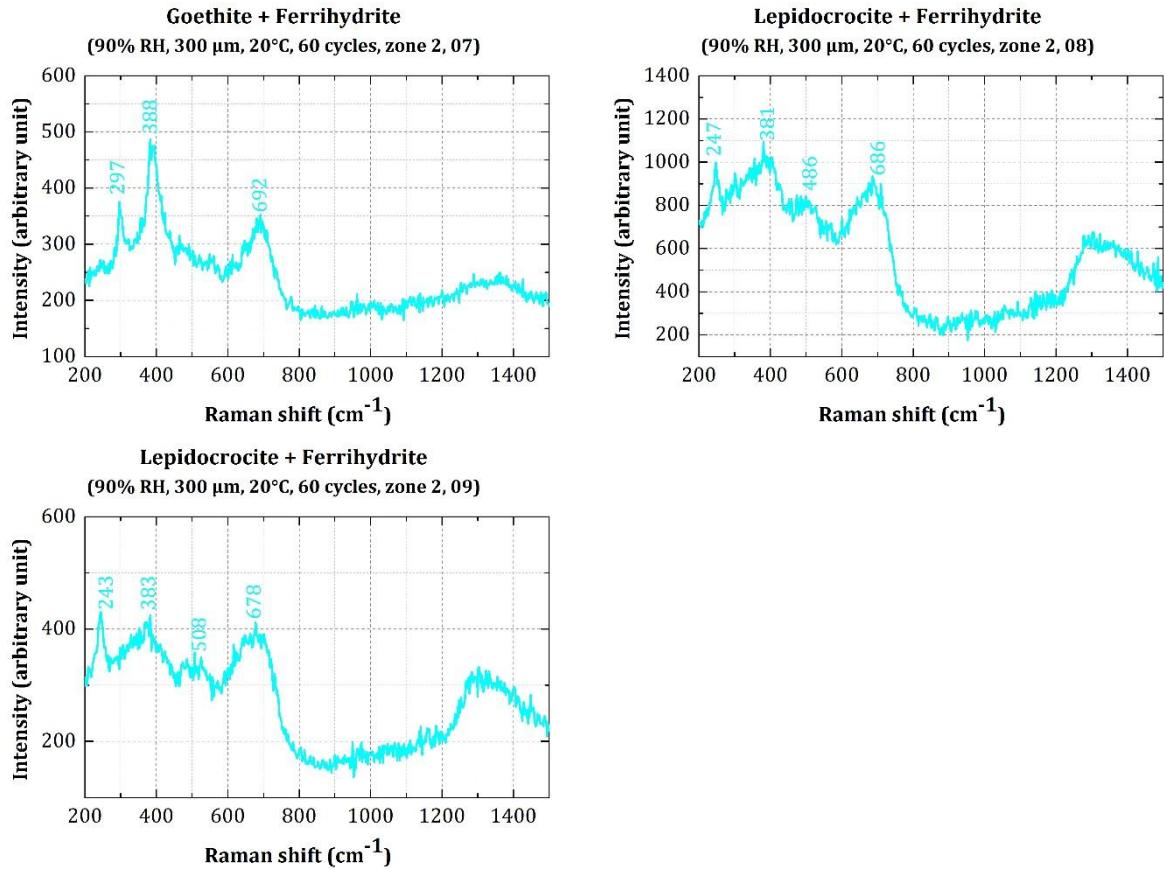
Figure I-54: All the Raman spectra of corrosion products obtained on specimens having 300 μm crack width and subjected continuously to 90% RH
