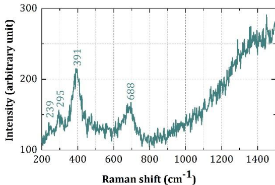
Figure I-63: All the Raman spectra of corrosion products identified in (CEM I + slag) mortar
