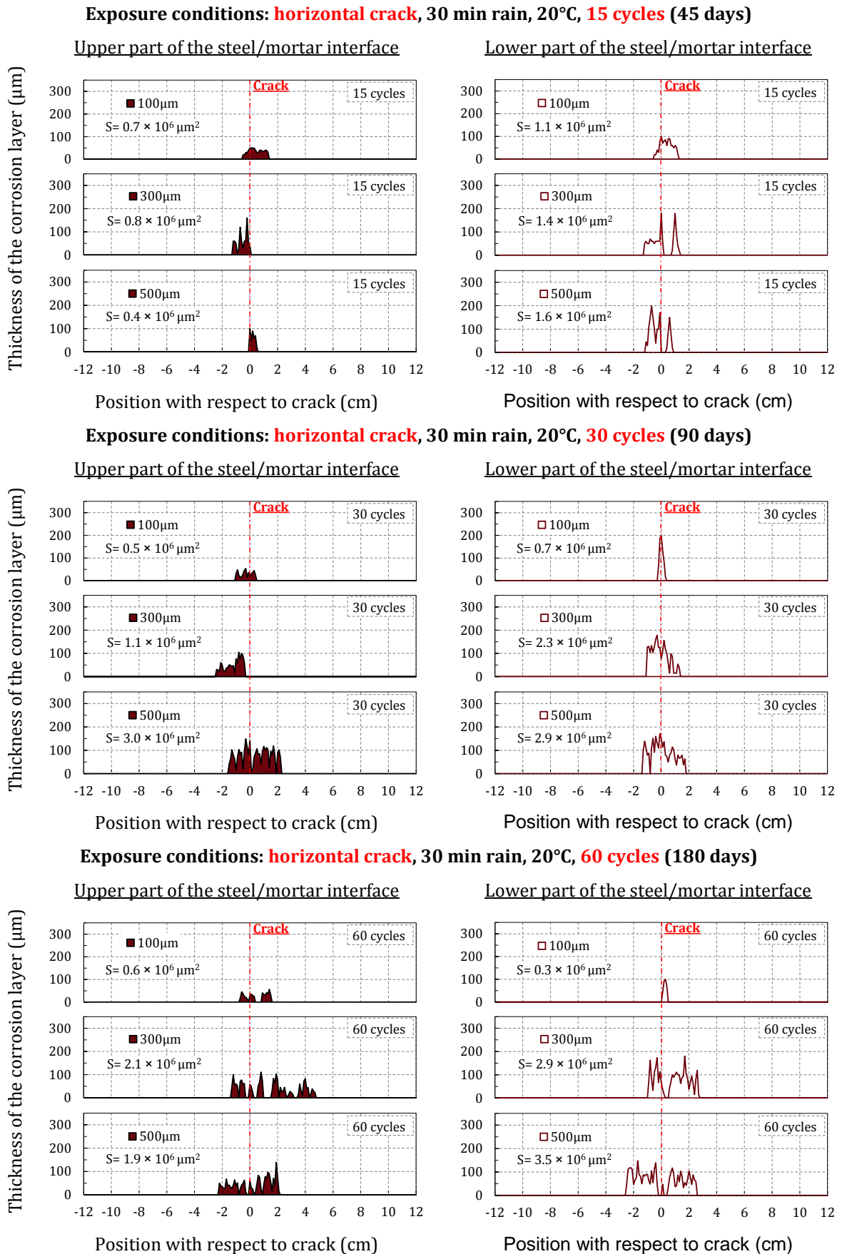
Figure I-39: Corrosion products repartition on the upper and the lower steel/mortar interfaces of specimens exposed horizontally with respect to rain (15, 30, 60 raining/drying cycles)
