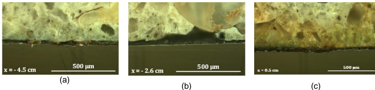
Figure 5-23: Loss section in the steel at different distances from the crack in a specimens exposed continuously to 90% RH for 180 days (optical microscopy)
