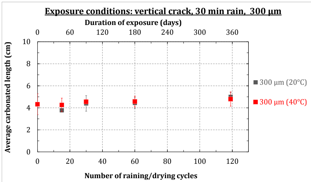
Figure I-72: Evolution of the carbonated steel/mortar interface length in specimens exposed to different temperatures (300 μm)
