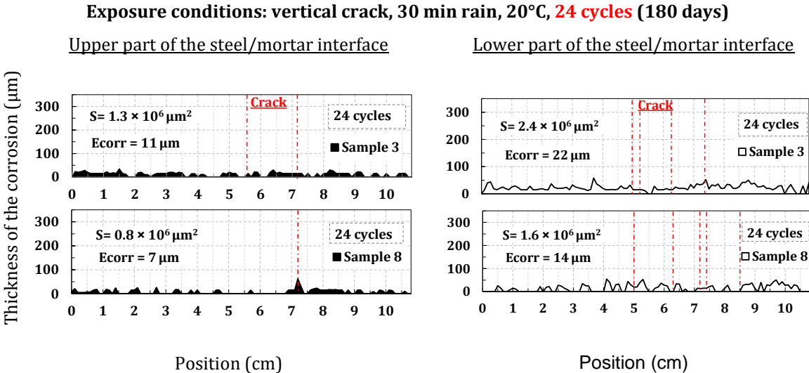
Figure 7-11 : Corrosion products repartition on the upper and the lower steel/mortar interfaces of both reinforcement layers embedded in a concrete slab subjected to 24 cycles.
