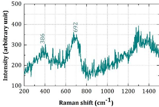
Lepidocrocite + Ferrihydrite (Mortar (CEM I + slag)) (Vertical crack, 300 µm, 30 min rain, 20°C, 60 cycles, 180 days, zone 2, 05)
