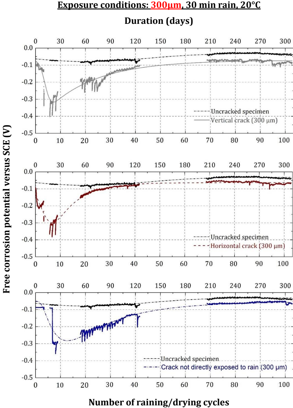
Figure 5-7: Free corrosion potential (versus SCE) measured in specimens showing 300 µm residual crack exposed in different directions with respect to rain
