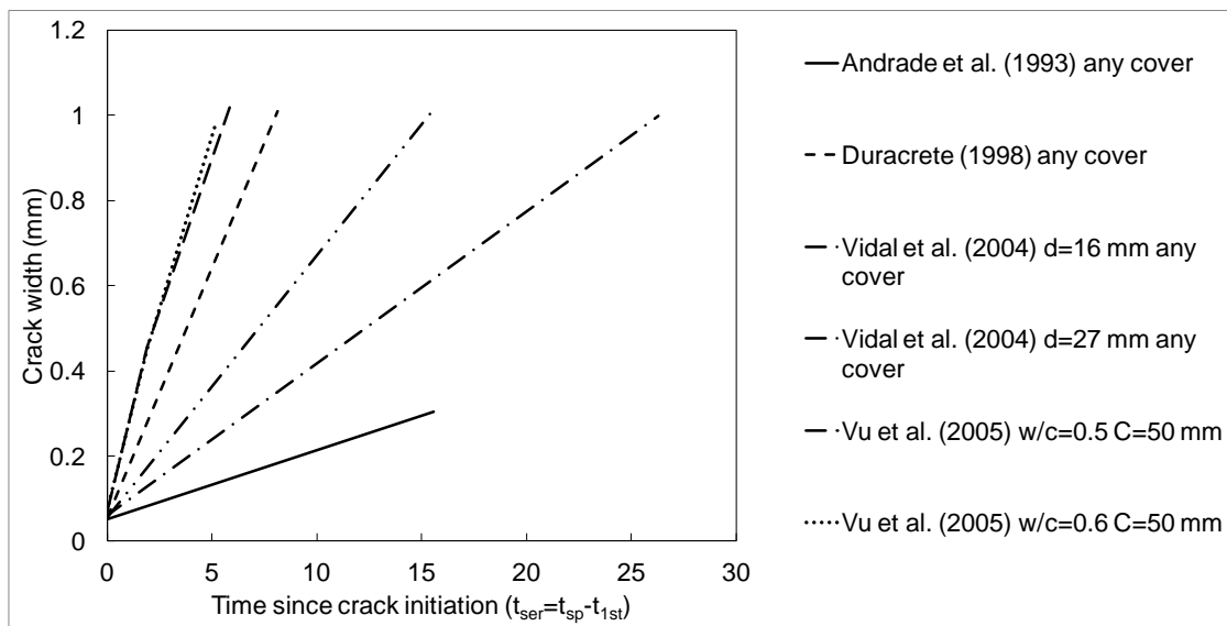
Figure 1-25: Comparison between different empirical models for estimating the crack width due to corrosion propagation in the case of chloride-induced corrosion [125]
