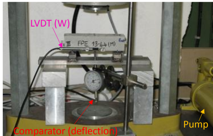
Figure 2-31: three point bending test on a 40x40x160 mm specimen
