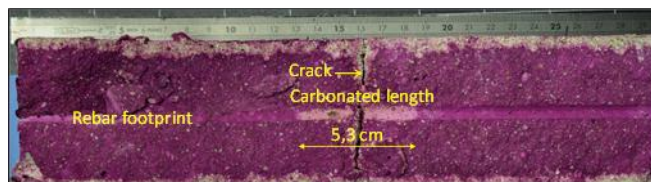
Figure 2-34: Alteration length of the steel/mortar interface for a cracked and carbonated specimen with a residual crack opening of 500 \mu\text{m}
