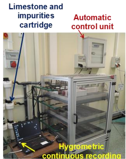
Figure 2-23: Real atomized device for humidification/drying cycles
