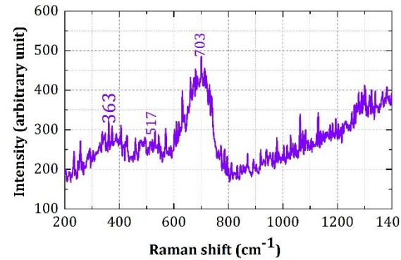
Ferrihydrite (Vertical crack, 300 \mu\text{m} , Saclay environment, 180 days, zone 1, 05)
