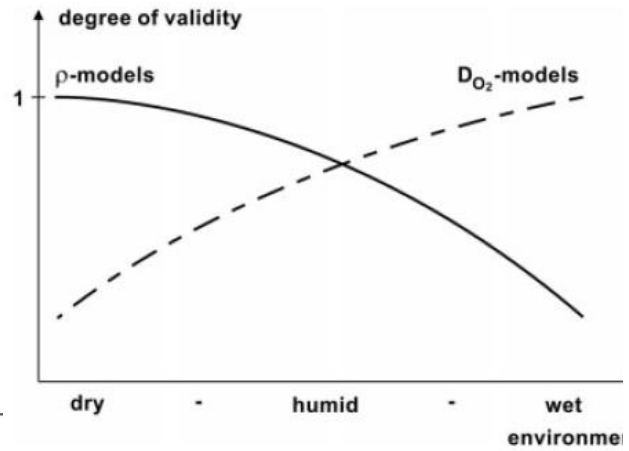
Figure 1-23: The controlling factors for the corrosion rate with regard to relative humidity
