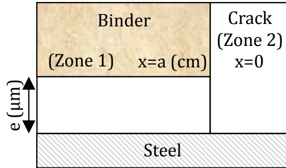
Figure 2-56 : Template for the schematic representation used to summarize the identified corrosion products
