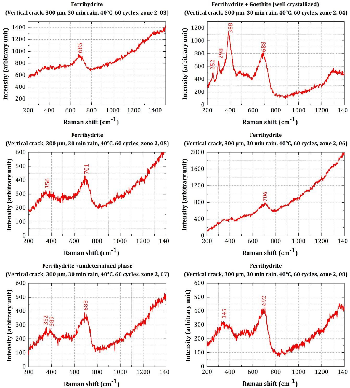
Figure I-55: All the Raman spectra of corrosion products obtained on specimens having 300 μm crack width and corroded at 40°C under raining/drying cycles of 30 minutes rain each (deep in the crack)
