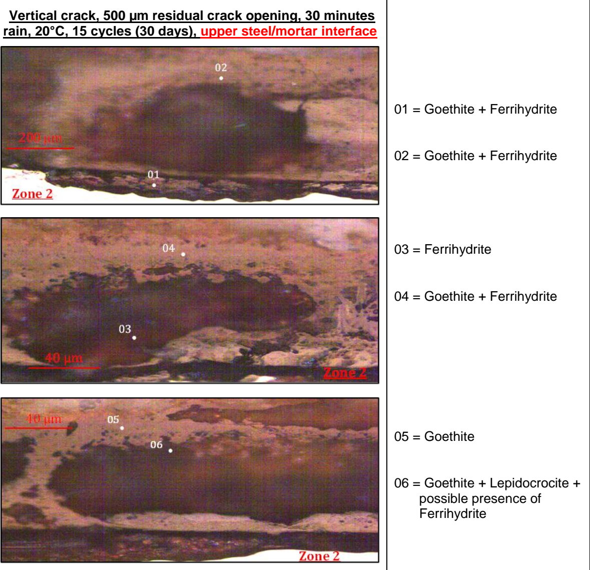
Figure 7-13: Corrosion layer observed at the upper steel/mortar interfaces located far from the crack and deep in the crack in specimens corroded in the reference test for 15 cycles ( W_r = 500 \mu\text{m} )
