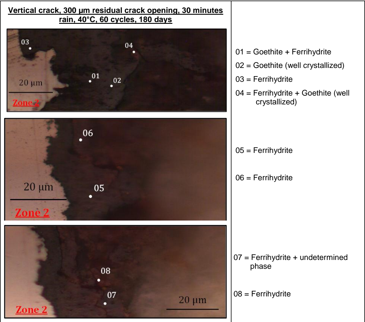
Figure 5-31: Corrosion layer observed at steel/mortar interface located deep in the crack in a specimen having 300 μm residual crack width and corroded under raining/drying cycles at 40°C
