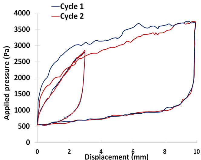
FIGURE 5.20: Stress variation over 2 cycles of charging/discharging for both \pm 3 mm and \pm 10 mm displacements
