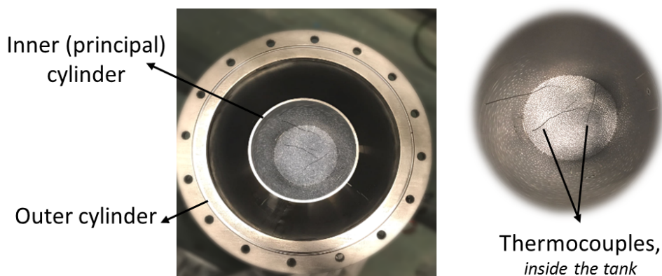
FIGURE 5.10: Top view of both cylinders showing the thermocouples inside the tank)
