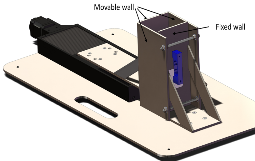
FIGURE 5.15: Schematic view of P'tit-Pousse installation
