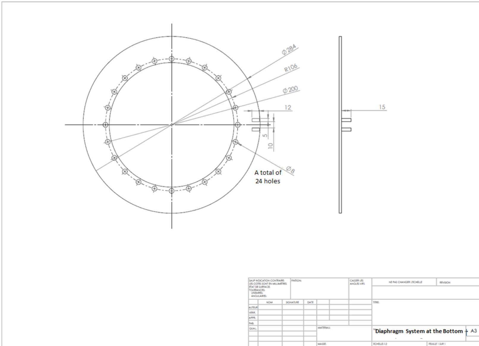
FIGURE B.6: Diaphragm system at the bottom of the tank
