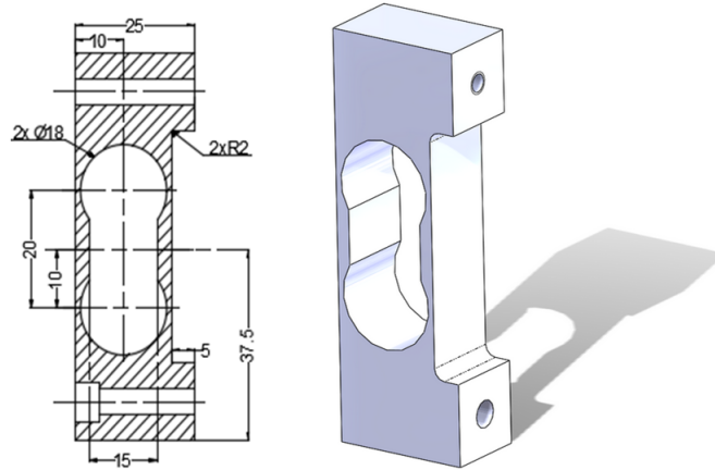
FIGURE 5.7: Dimensions of the force measurement device
