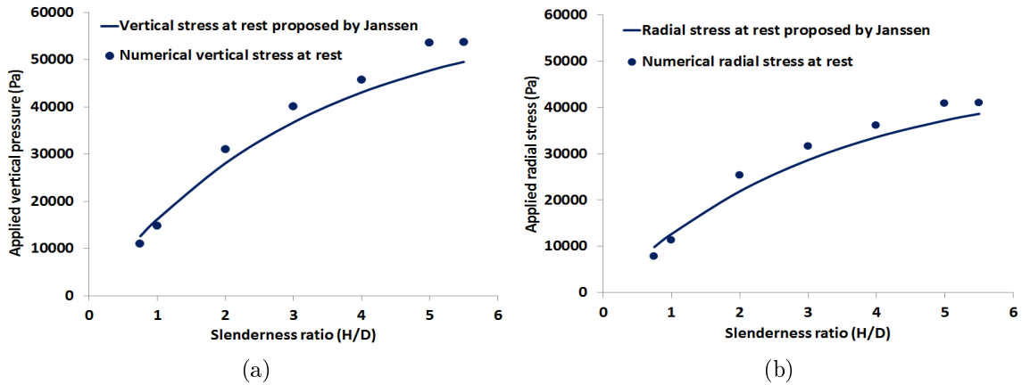
FIGURE 3.7: Influence of the slenderness ratio at rest: (a) on the vertical stresses (b) on the horizontal stresses
