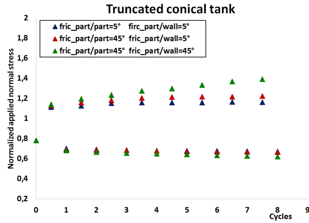
FIGURE A.4: Thermal stresses applied on truncated conical walls at different levels of friction
