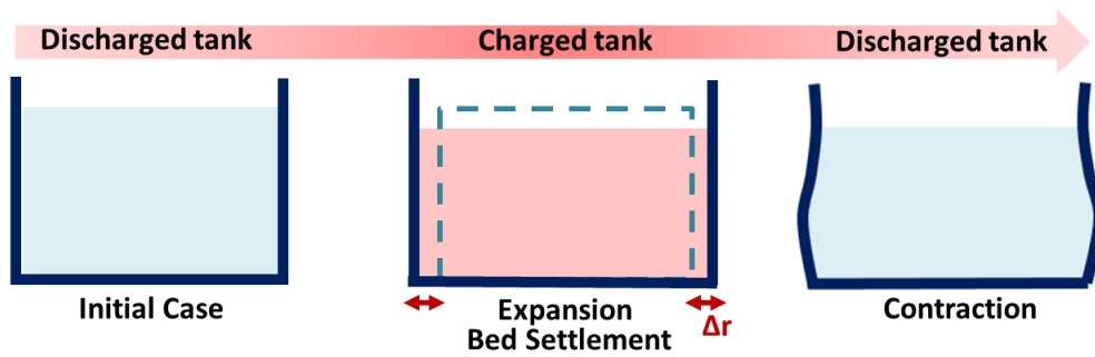
FIGURE 2.6: Illustration of the thermal ratcheting phenomenon when the tank expands more than the filler material
