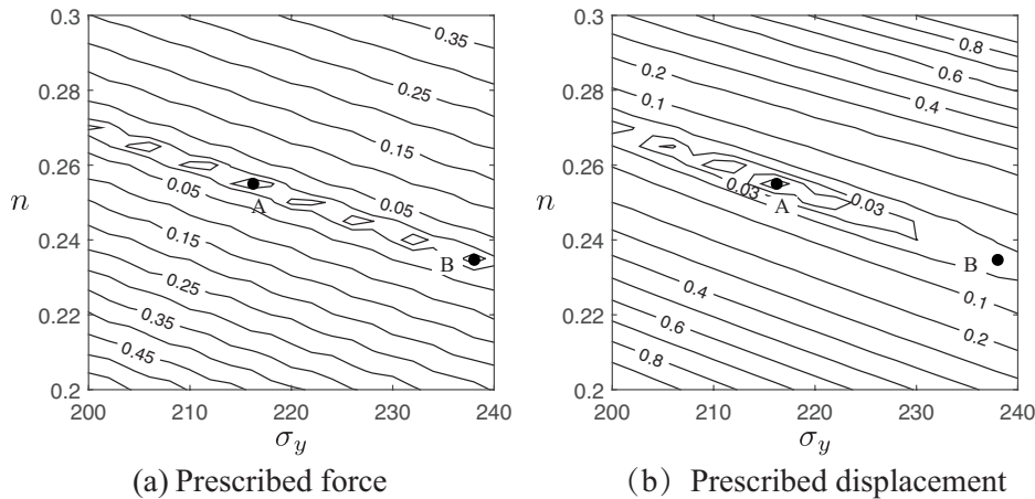
FIGURE 4.11 Objective function distribution when employing P - h curve snapshots with spherical indenter, p = q = 201 , w = 0 .
