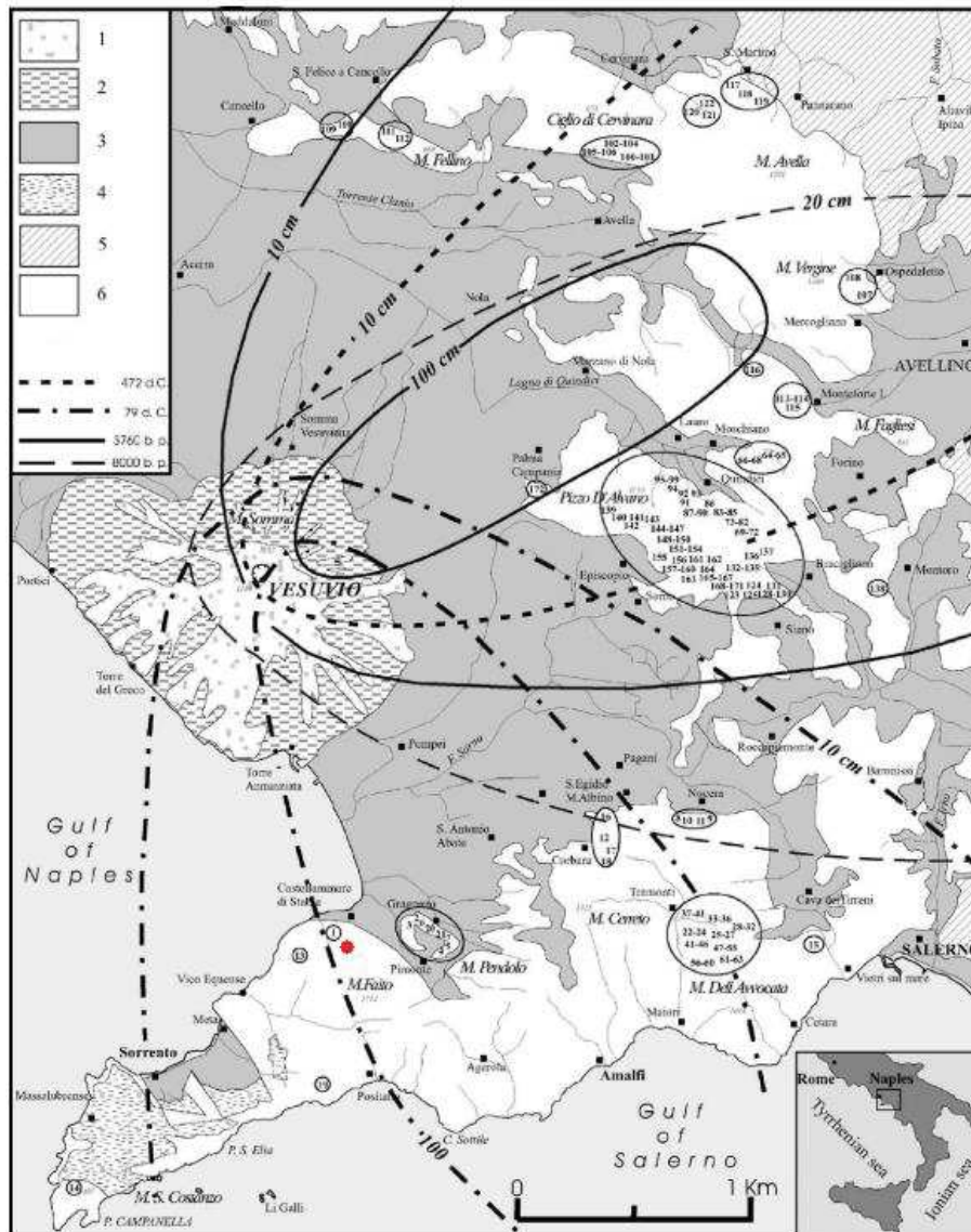
(1) Lavas; (2) Pyroclastic flow; (3) Pyroclastic fall and detrital-alluvial deposits; (4) Mio-Pliocene terrigenous deposits; (5) Miocene terrigenous deposits; (6) Mesozoic limestones ● Mount Faito test site
